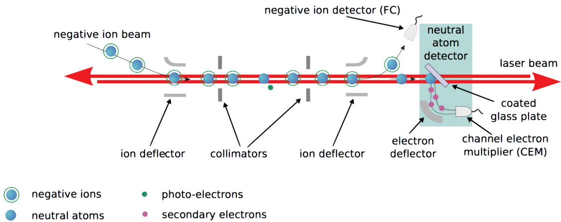
Figure 3.6: Figure from paper I showing a schematic principle of GANDALPH. A beam of negative ions is overlapped with a laser beam, arranged in either a co- or counter-propagating geometry. The neutral atoms produced in the photodetachment process impinge on a coated glass substrate where secondary electrons are created. These electrons are deflected 90° by means of an electrode where they are detected by a single channel electron multiplier. Remaining undetached ions are deflected towards a Faraday cup.
