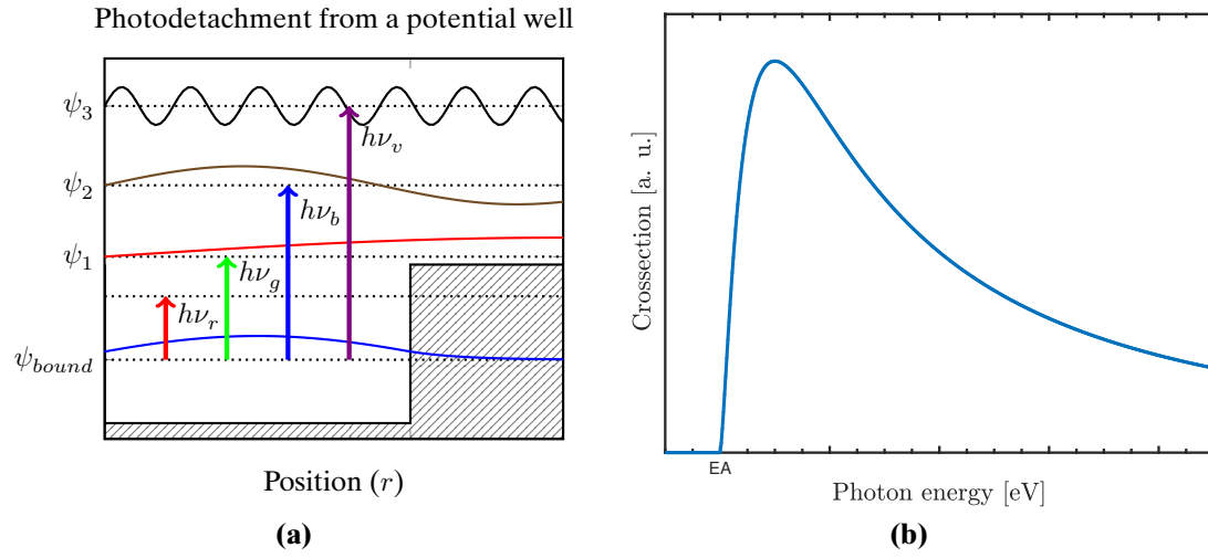
Figure 2.4: Figure (a) shows the photodetachment process of four separate cases of visible photon energies ( h\nu_v , h\nu_b , h\nu_g and h\nu_r ). The box potential is an approximation which can be used to qualitatively describe the overall behaviour of the total cross section which is shown in Figure (b). Particularly interesting is the peak value of (b) that coincide with the largest overlap between the initial ( \psi_{bound} ) and final ( \psi_b ) wave functions.
