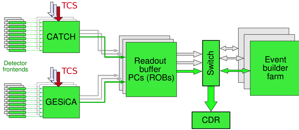
Figure 3.5: COMPASS data acquisition system. Digitized detector information is transferred to CATCH and for some detectors GESiCA modules. In case of a trigger signal from the trigger control system (TCS), the data are sent to readout buffer PCs. Via a GigaBit switch, the data are further transferred to the event builder farm, where the streams of information from one event are combined. Finally, the data are stored in the central data recording (CDR).
