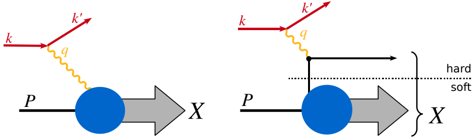
Figure 2.1: The diagram shows the lepton-nucleon scattering process, mediated by the exchange of a virtual photon, and the production of an undetected final state X . On the left hand side, a phenomenological picture of the DIS process is given, whereas the right figure shows the scattering process in the partonic picture. Therein, the photon scatters on one individual quark. This second approach is only valid in the Bjorken limit, where the concept of factorization can be applied.
