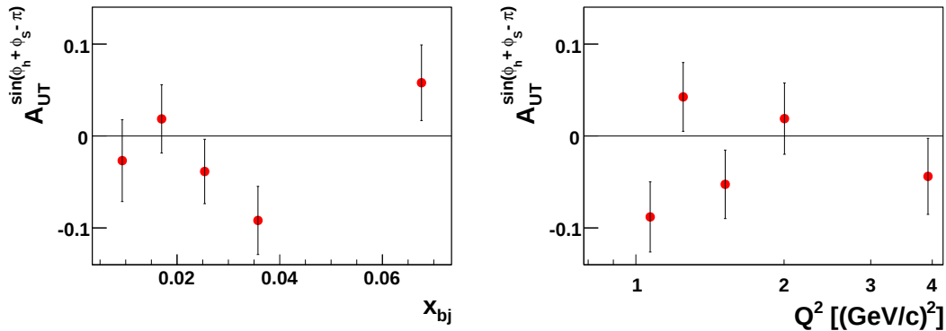
Figure D.1: Results for the amplitude A_{\text{UT}}^{\sin(\phi_h + \phi_S - \pi)} in certain ranges of the kinematic variables x_{\text{Bj}} and Q^2 .
