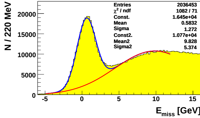
Figure 6.7: Distribution of the missing energy E_{\text{miss}} with all restrictions for the final data sample applied except those on this particular variable. This distribution was fitted with a function (blue), built as the sum of two Gaussian distributions, to determine the contributions of non-exclusive background events. The background contributions (red) in the kinematic range of the final data sample ( -2.5 GeV to 2.5 GeV) was estimated to be about 20%.
