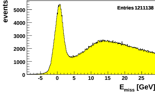
(a) Distribution of the missing energy with the restriction p_T < 0.3 \text{ (GeV/c)}
