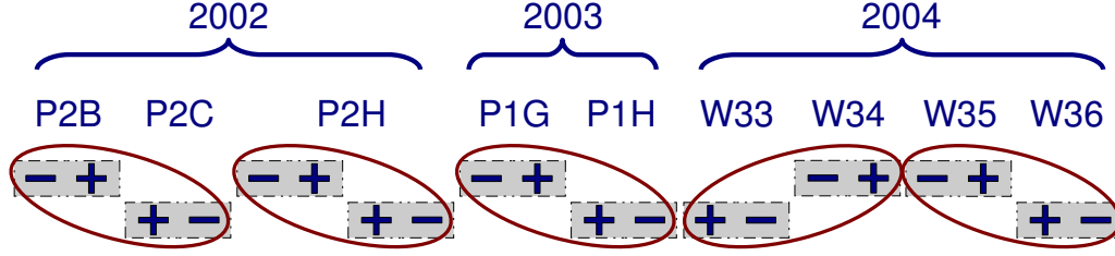
Figure 5.1: Grouping of the data recorded with the transverse-target spin configuration. The total, ten periods are combined to five double-periods, to which the Double Ratio method can be applied.
