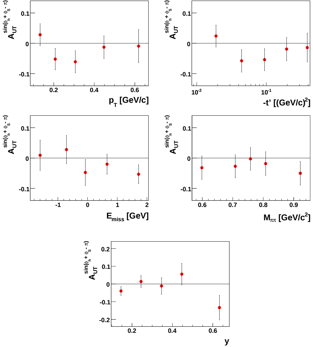
Figure D.2: Results for the amplitude A_{\text{UT}}^{\sin(\phi_h + \phi_S - \pi)} in certain ranges of the kinematic variables p_T , t' , E_{\text{miss}} , M_{\pi\pi} and y . Therein the range in the y -axis for the graph in y is widened.
