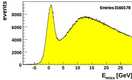
(c) Distribution of the missing energy with the restriction p_T < 0.7 \text{ (GeV/c)}
