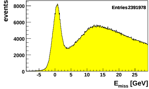
(b) Distribution of the missing energy with the restriction p_T < 0.5 \text{ (GeV/c)}
