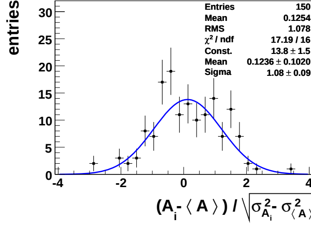
Figure 6.5: Pull distribution for the check of compatibility of the different periods. The fitted Normal distributions (with \text{RMS} = 1.078 ) validate the compatibility of results.
