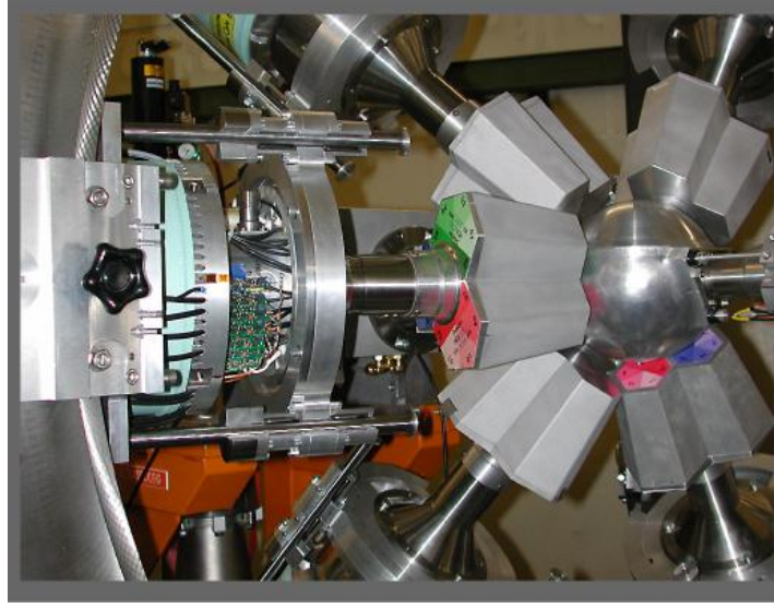
Figure 3.6: The MINIBALL array of HPGe detectors, in place at the end of REX-ISOLDE.
