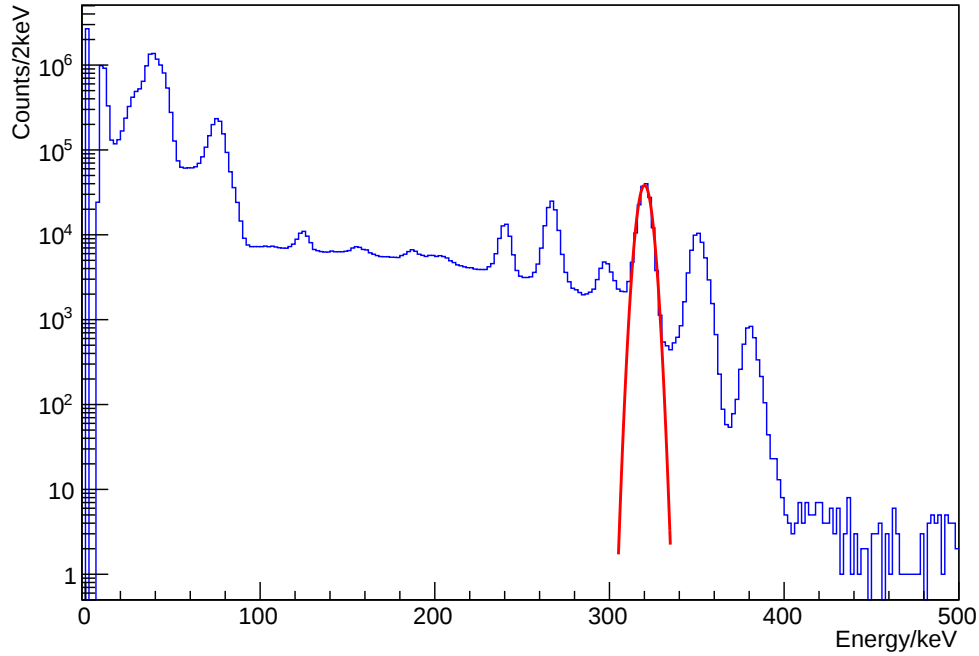
Figure 4.6: Total counts detected by SPEDE from all segments in approximately 40 minutes from a ^{133}\text{Ba} source. No HV or foils are present, and detector is cooled to approximately -30^\circ\text{C} . Position of fitted peak: 320.2(1)\text{ keV} , FWHM: 7.10(2)\text{ keV} .
