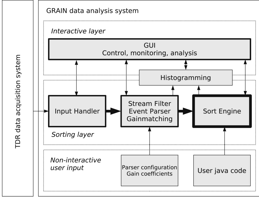
Figure 3.15: A schematic for the TDR DAQ system at the JYFL laboratory, Finland. This system was used to capture and process the events seen by SPEDE during in-beam testing.
