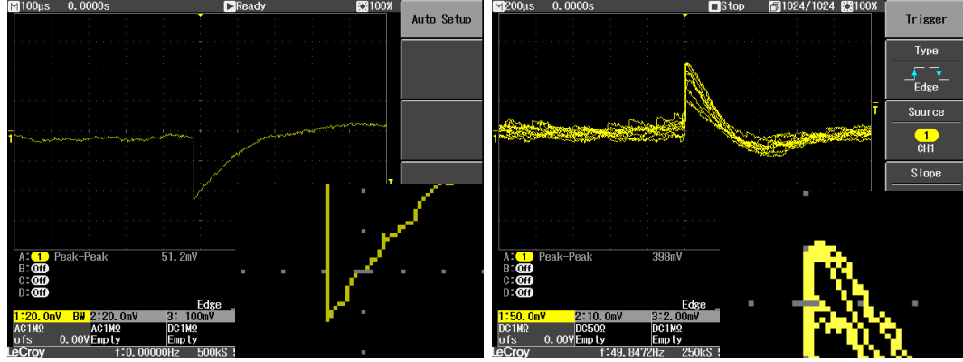
Figure 3.9: The pulse directly from the preamplifier is shown on the left, and from the GO box on the right, with each pulse zoomed in on the lower right of the picture. The top of the pulse from the GO box is elongated and appears flat before decaying, although the effect is slight and not an issue for pulse detection using Lyrtech electronics, which uses the initial sharp rise of the pulse for information. The two images are not directly comparable in terms of amplitude as the GO box has a gain of -2.5, and the time division for the scope has also been doubled to view pulses from the GO box.
