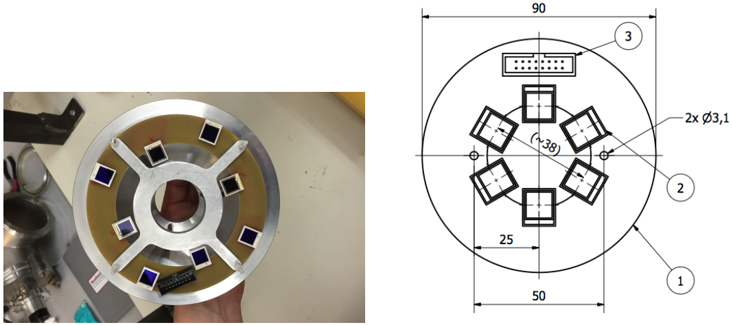
Figure 3.17: Left, the 8-PIN diode array particle detector used for the first part of SPEDE commissioning in February 2015. Right, the 6-PIN diode array particle detector used for the second part of SPEDE commissioning in May 2015, due to issues noted in the first commissioning run.
