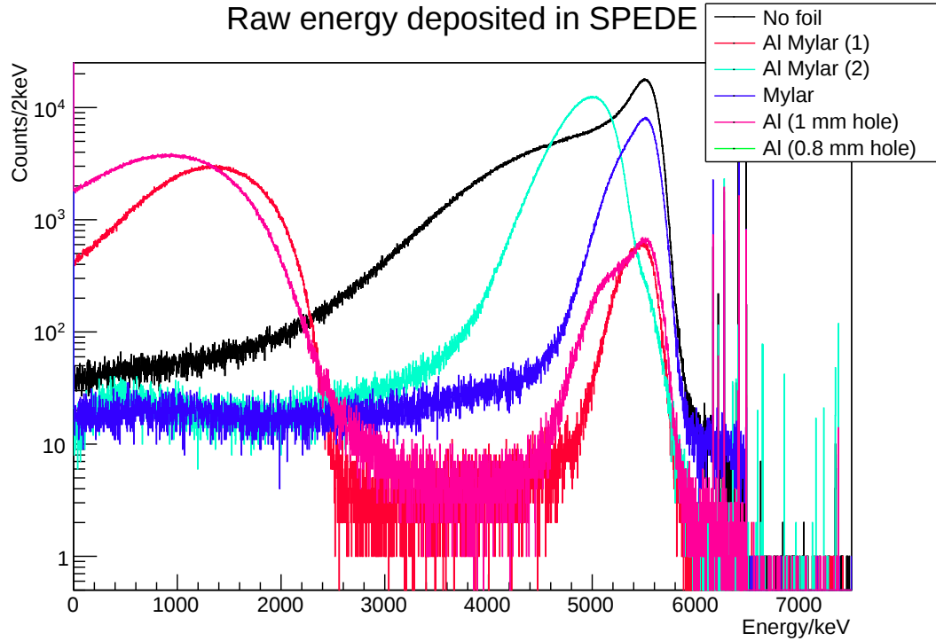
Figure 4.27: ^{241}\text{Am} after passing through various foils, used to determine foil thickness by looking at the attenuation of energy of the main peak.
