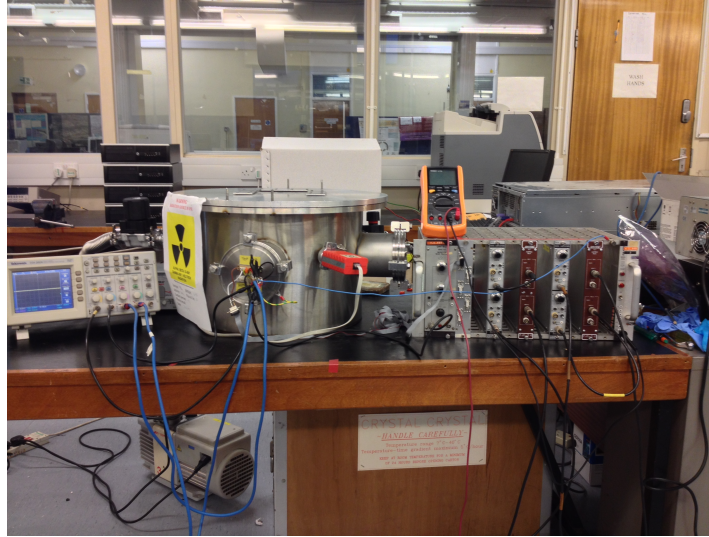
Figure 3.11: The setup used for initial testing of SPEDE in the Oliver Lodge laboratory, Liverpool
