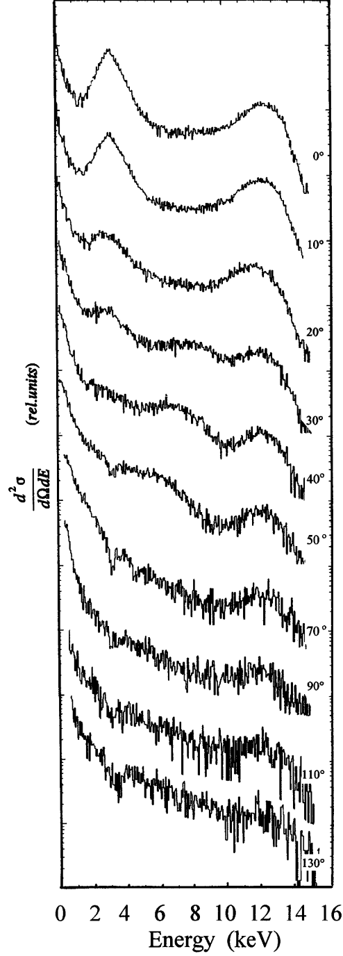
Figure 2.3: The \delta -electron distribution is not isotropic, and as can be seen is concentrated in the forward direction. The energy range is low, and drops quickly within the first 10 keV. Data is from [?].
