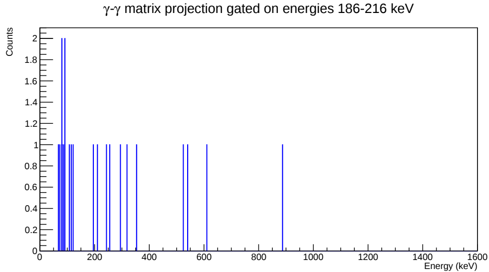
Figure 1.7: Taking Figure 1.5 and gating on the first peak, no coincidences with any other \gamma -ray energies are seen.
