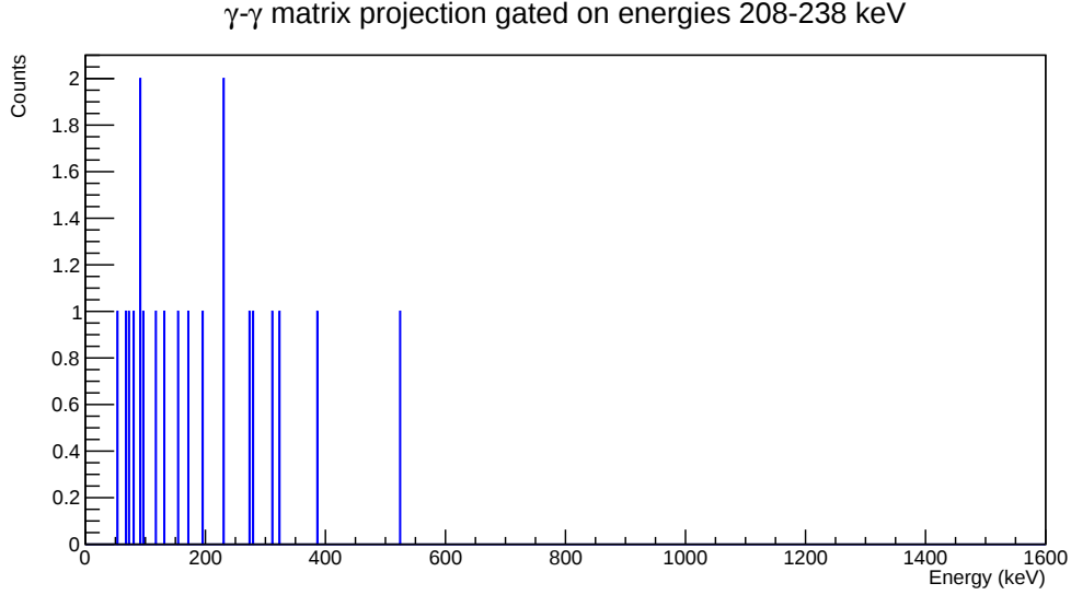
Figure 1.8: Taking Figure 1.5 and gating on the second peak, no coincidences with any other \gamma -ray energies are seen.
