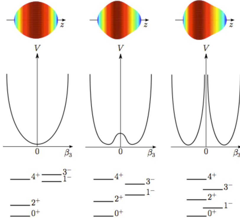
Figure 1.1: Nuclear potentials as a function of the octupole deformation parameter, \beta_3 ; from left-to-right, a quadrupole deformed nucleus with an octupole vibration averaging zero, an intermediate case with a small potential barrier separating two degenerate deformed minima and an ideal rigid deformation. Red colours indicate the shape raising out of the page, with bluer colours representing areas less raised. From [?].
