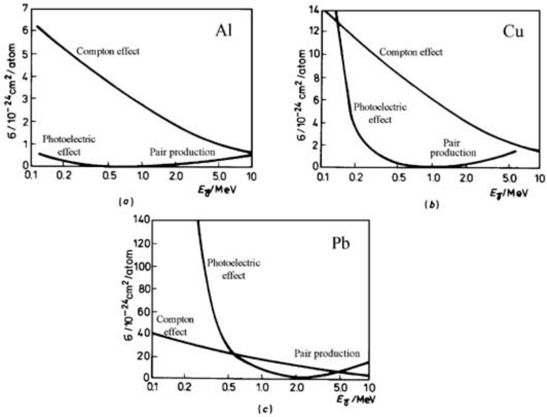
Figure 2.4: Photon interaction methods in aluminium (a), copper (b) and lead (c).
