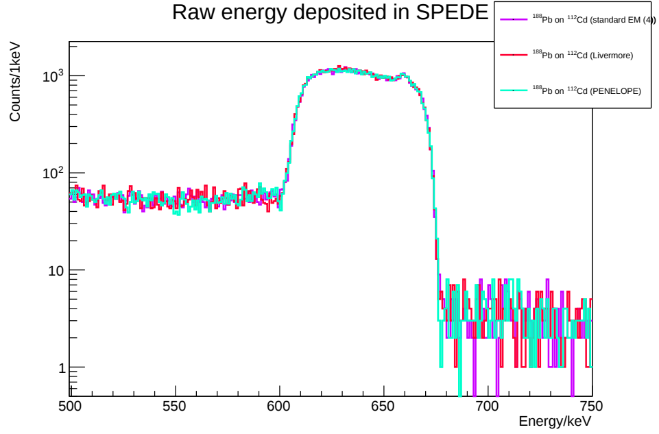
Figure 3.19: Simulated ^{188}\text{Pb} on ^{112}\text{Cd} using different energy libraries
