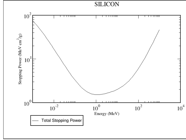
Figure 3.3: Stopping power of electrons in silicon, extracted from ESTAR.
