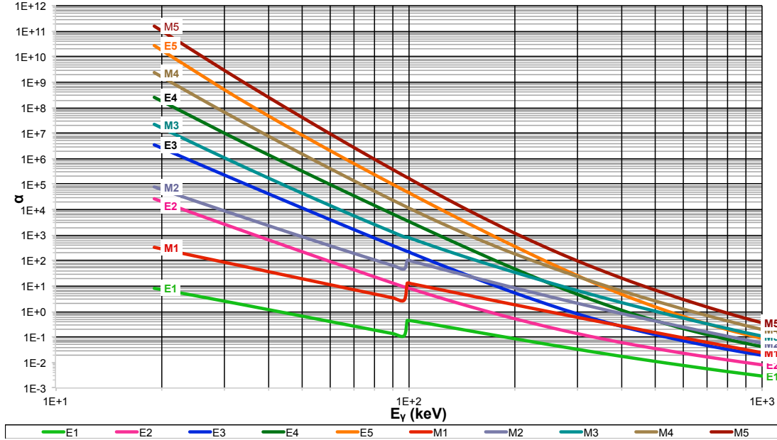
Figure 2.2: The data is the theoretical values for internal conversion in radon, as a dependence of energy, and also multipolarity of the transition. This dependency on the multipolarity comes from the fact that it is easier for an electron to carry more angular momentum from a nucleus and is thus the quicker, and therefore preferred, way for the nucleus to fall into the minimum of its potential well. Note the kinks in E1, M1, and M2 transitions, which are due to the K-shell binding energy. For nuclear transitions which lie below this energy, any converted electrons must come from a higher shell, such as one of the L shells, which are less likely to couple to the nucleus due to the quantum mechanical wavefunction of the electron-nucleus system resulting in the electrons spending less time in and around the nucleus. Similar kinks would be seen at the energies of the L-shells if the data had been available to plot; they are much less bound than the K-shell. Data is from [?].
