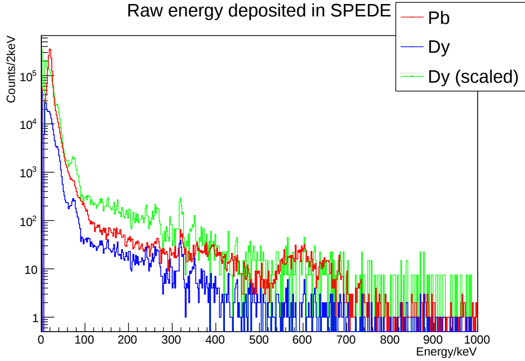
Figure 4.9: Total counts detected by SPEDE from all segments in approximately 12 minutes of ^{40}\text{Ar} on a ^{207}\text{Pb} (Red) and ^{160}\text{Dy} (blue) target. No foil is present. Note several peak-like areas over 500-750 keV. Peaks at lower energies can be attributed to contamination from ^{133}\text{Ba} .
