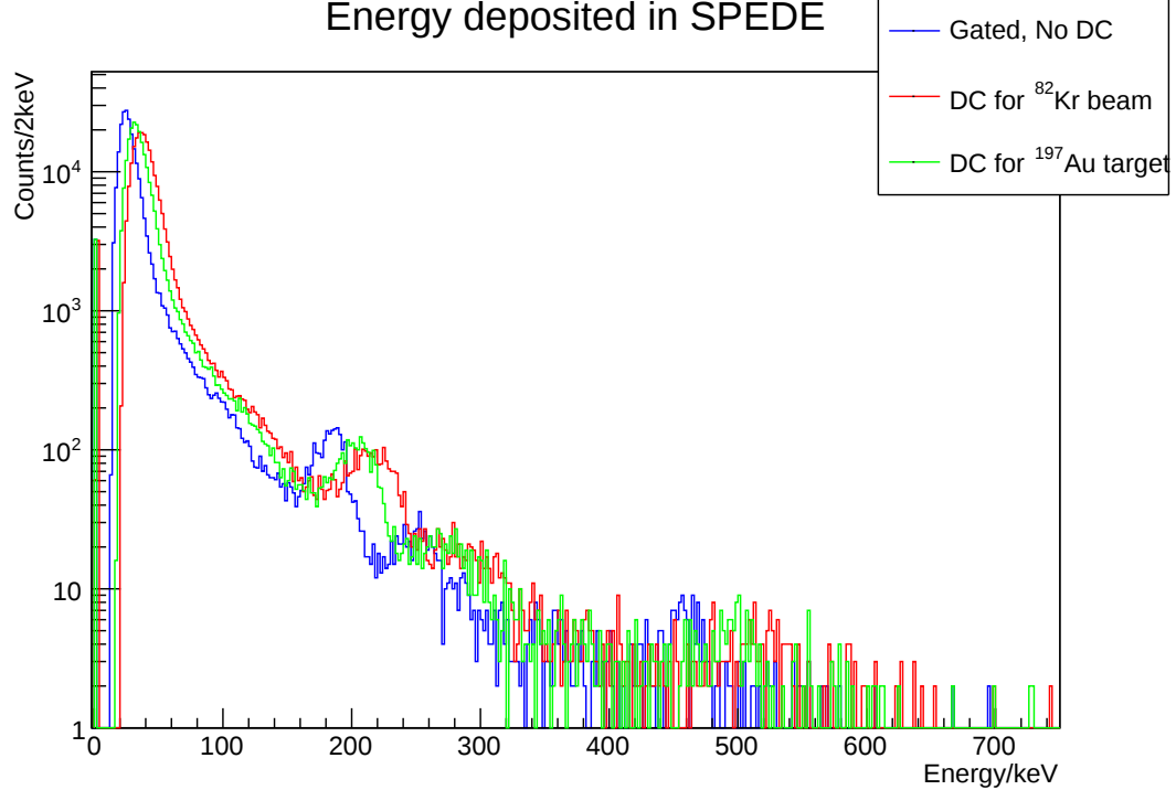
Figure 4.24: Compared to previous figures, the peaks, Doppler corrected for the target, appear much cleaner in this plot of ^{82}\text{Kr} on ^{197}\text{Au} with HV applied.
