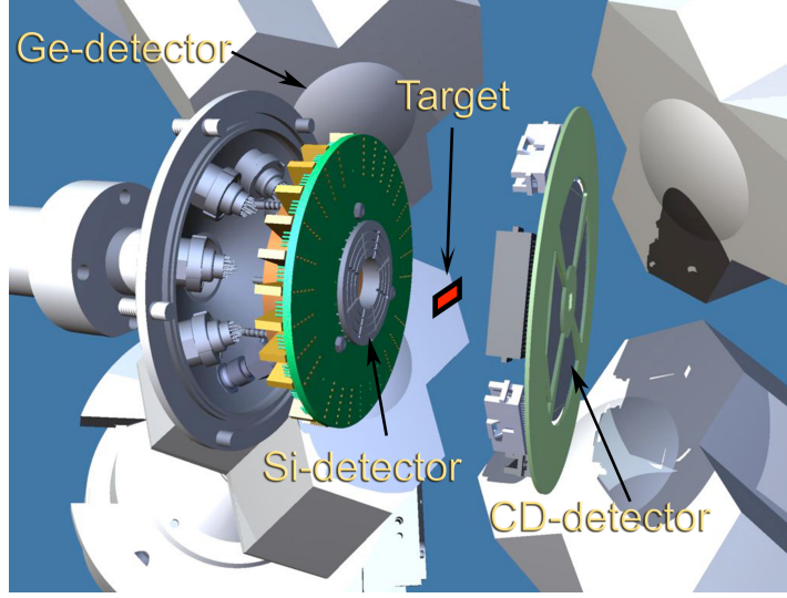
Figure 3.4: A computer-aided design (CAD) drawing of SPEDE is seen on the left of the picture. The beam enters from the left side, through the center of the detector, interacting with the target illustrated by the red box. Decays from excited nuclei are subsequently detected by SPEDE and the surrounding MINIBALL detectors. Particles are detected in the CD detector on the right.
