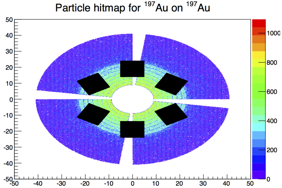
Figure 3.22: Here, the CD detector is shown in colour, with number of simulated hits of ^{197}\text{Au} on ^{197}\text{Au} given according to the colour scale on the right. A PIN diode array is shown in black on top of this CD illustrating the difference in cross-section for each detector setup.
