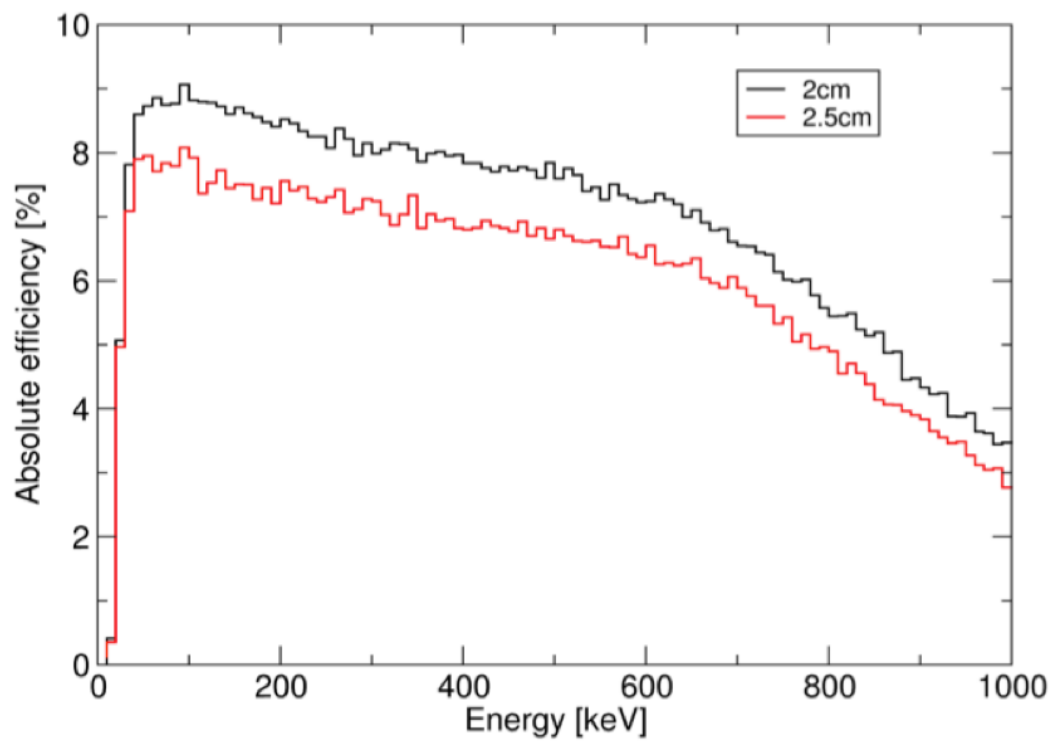
Figure 4.28: Simulated efficiency of SPEDE at 2 and 2.5 cm. An average efficiency of about 8% is seen across the region of interest, dropping rapidly at about 30 keV. Courtesy of D. Cox.
