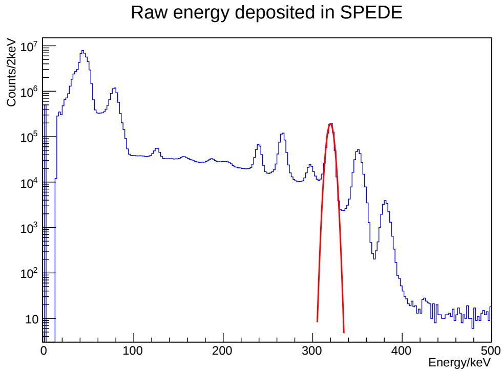
Figure 4.23: Total counts by detected SPEDE from all segments in approximately 170 minutes from a ^{133}\text{Ba} source. No HV or foils are present, and detector is cooled to approximately -^{\circ}30\text{C} . The resolution of each channel that make up this total plot ranged from 6.00 to 7.05 keV. Position of fitted peak: 319.9(4) keV, FWHM: 6.9(1) keV.
