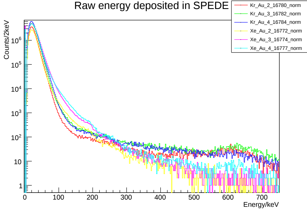
Figure 4.12: ^{132}\text{Xe} and ^{84}\text{Kr} beams incident on gold targets of various thicknesses
