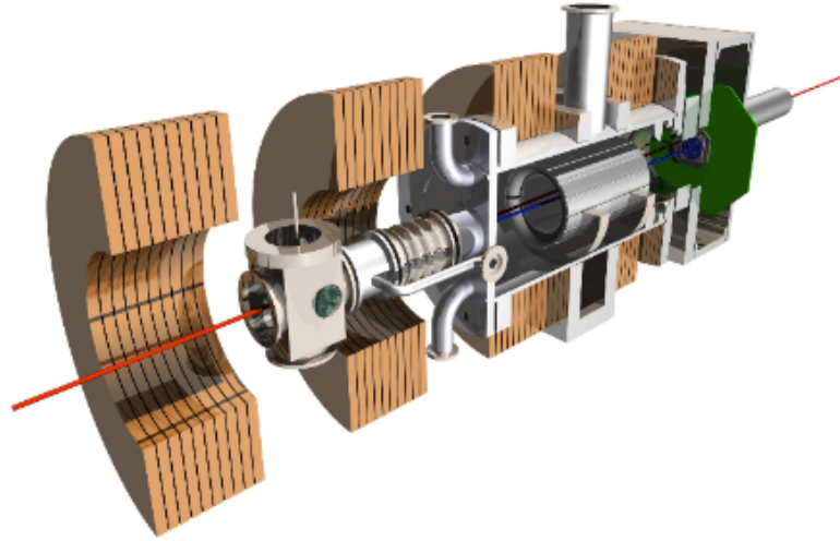
Figure 2.7: The SACRED detector
