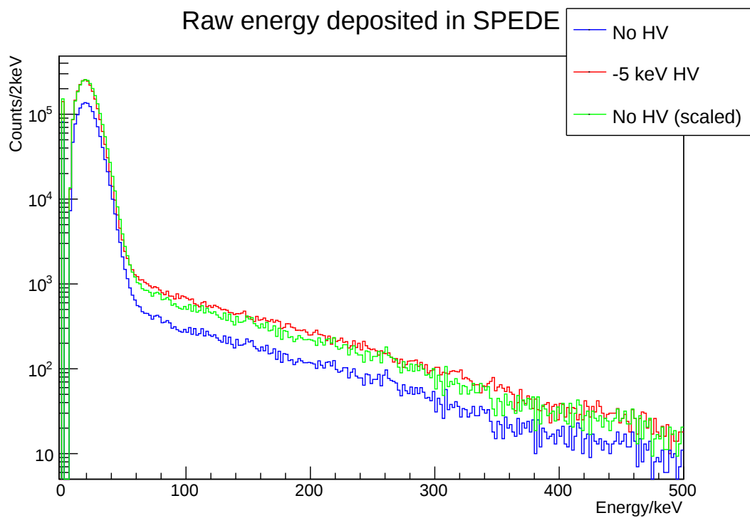
Figure 4.7: Total counts detected by SPEDE from all segments in approximately 3 minutes of ^{20}\text{Ne} on a ^{58}\text{Ni} target. An aluminised mylar foil is present. The blue line, illustrating data collected with no HV applied, is scaled to the bin with the maximum counts for HV at 19 keV, and shown by the green line.
