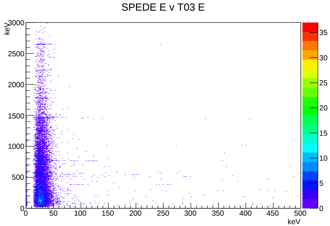
Figure 4.26: ^{82}\text{Kr} on ^{197}\text{Au} \gamma - e^- matrix. Note most coincidences appear in the left hand-side, implying they are random correlations with low-energy pileup within SPEDE, rather than true coincidences from higher-lying gamma-emitting states cascading and being internally converted.
