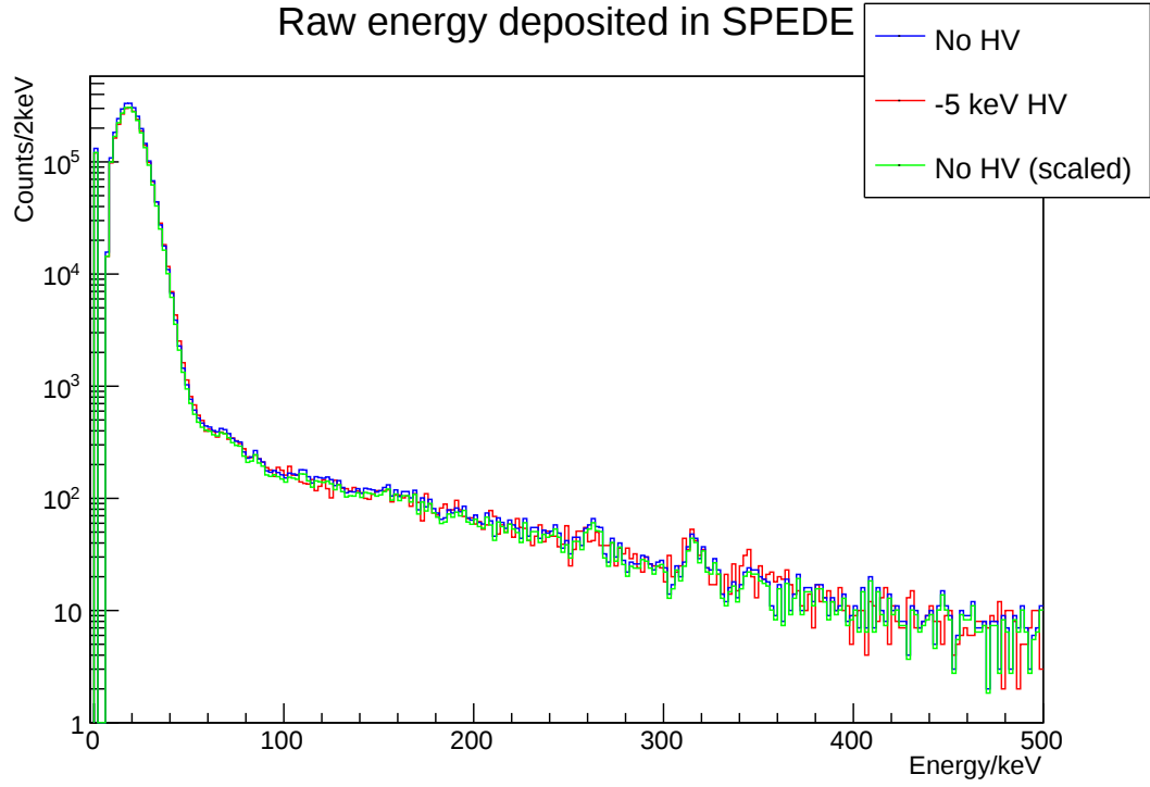
Figure 4.8: Total counts detected by SPEDE from all segments in approximately 4 minutes of ^{20}\text{Ne} on an empty target frame. An aluminised mylar foil is present.
