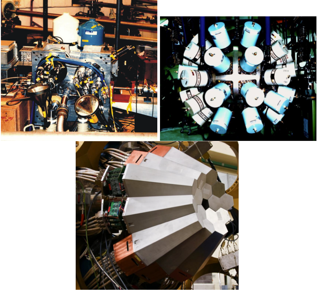
Figure 2.5: A variety of previous \gamma -detecting arrays are seen in the figure, clockwise from top-left: TESSA, EUROGAMII, AGATA.
