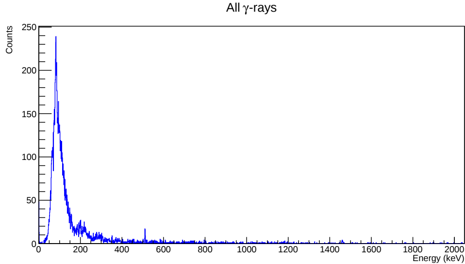
Figure 1.3: \gamma -ray spectrum showing all \gamma -rays detected by the MINIBALL array during the course of the experiment. The 511 keV annihilation peak is clearly visible. It is clear that there are a large number of background events. Conditions therefore need to be applied to clear spectra and make peaks visible.
