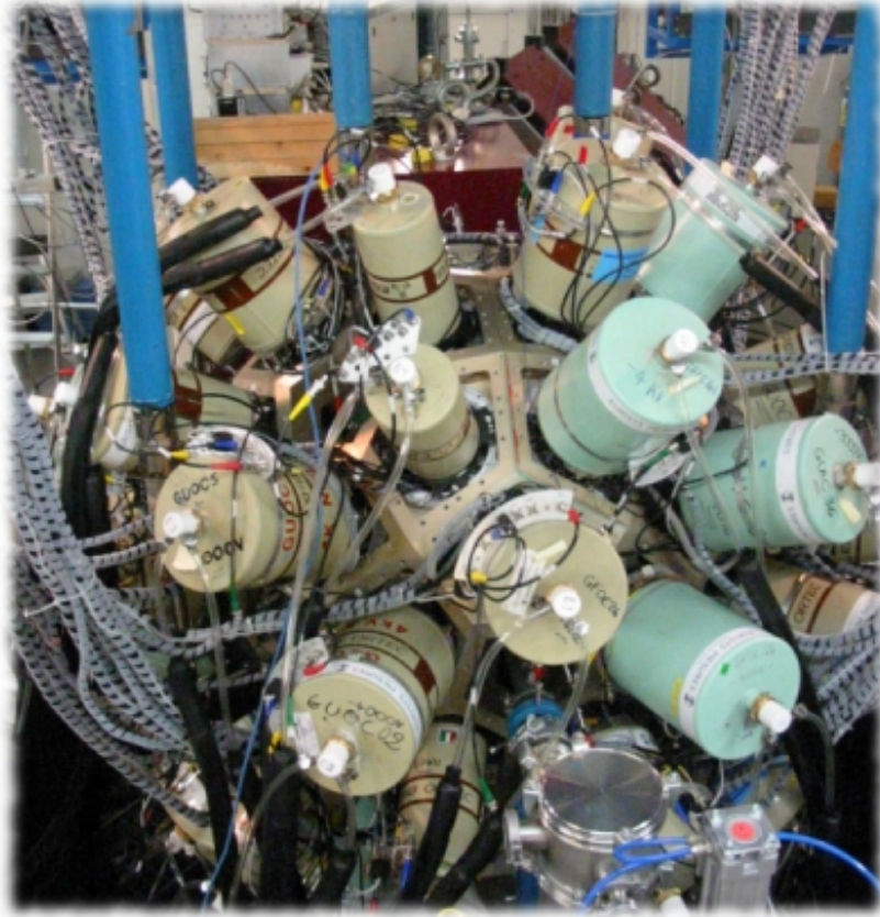
Figure 3.16: The JUROGAMII array
