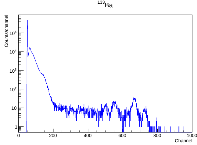
Figure 3.12: ^{133}\text{Ba} spectrum from SPEDE channel 1, during initial electronics testing, November 2013. This is uncalibrated; the peak corresponding to 320 keV at channel 665.73(45) has a FWHM of 22.61(98), which using a single point calibration would correspond to a FWHM of roughly 10.9 keV.
