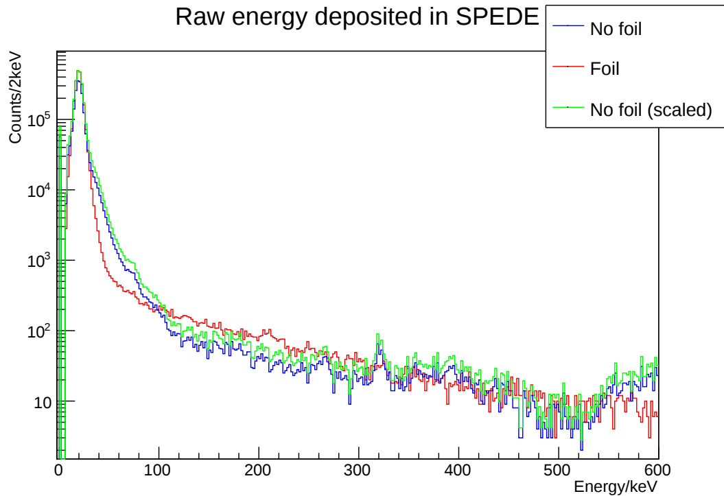
Figure 4.10: ^{40}\text{Ar} on ^{207}\text{Pb} , with & without foil
