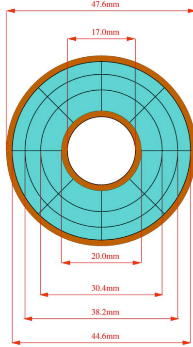
Figure 3.1: Inner and outer diameters of SPEDE are shown above. Detector segments are shown as blue areas between black lines, with guard rings illustrated by brown colouring.
