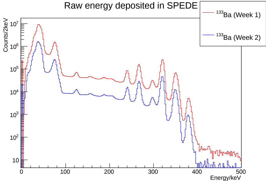
Figure 4.11: Total counts detected by SPEDE from all segments in approximately 280 minutes (week 1) and 60 minutes (week 2) from a ^{133}\text{Ba} source. No HV or foils are present, and detector is cooled to approximately -30^\circ\text{C} . Note the adjusted thresholds and the effect at low energy. Position of a fitted peak at 320 keV: 320.21(1) keV, FWHM: 7.29(8) keV (slightly worse than initial runs in November 2014).
