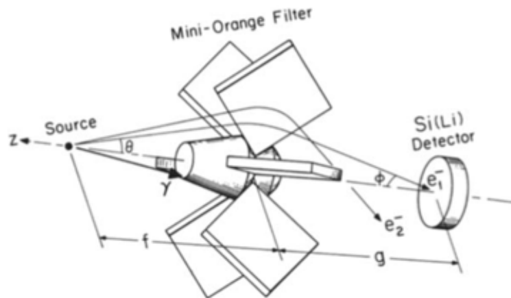
Figure 2.6: Typical layout of mini-orange type detector
