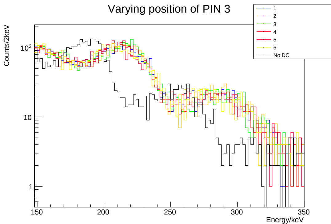
Figure 4.21: Effect of varying PIN position on Doppler correction
