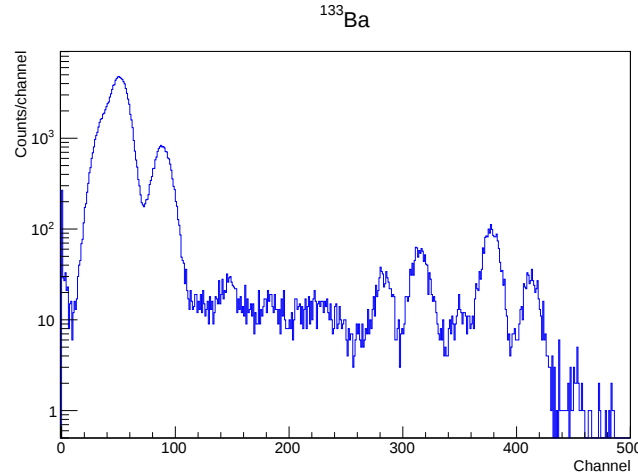
Figure 3.10: ^{133}\text{Ba} spectrum from preamplifier test, March 2013. This is uncalibrated; the peak corresponding to 320 keV at channel 377.59(19) has a FWHM of 13.99(35), which using a single point calibration would correspond to a FWHM of roughly 11.9 keV.
