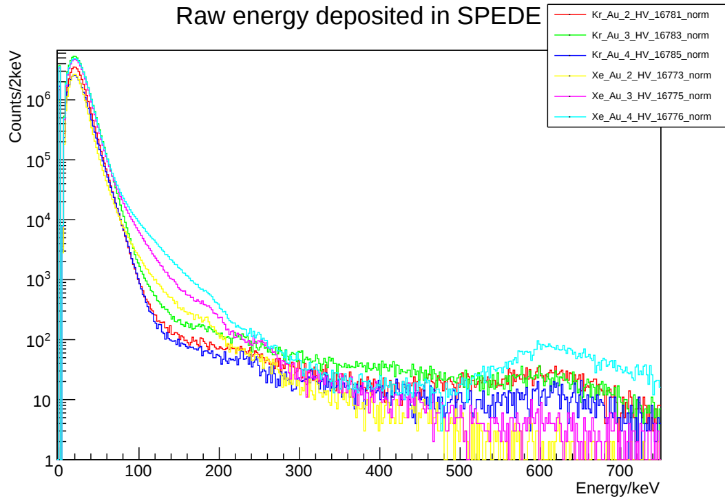
Figure 4.13: ^{132}\text{Xe} and ^{84}\text{Kr} beams incident on gold targets of various thicknesses (HV)
