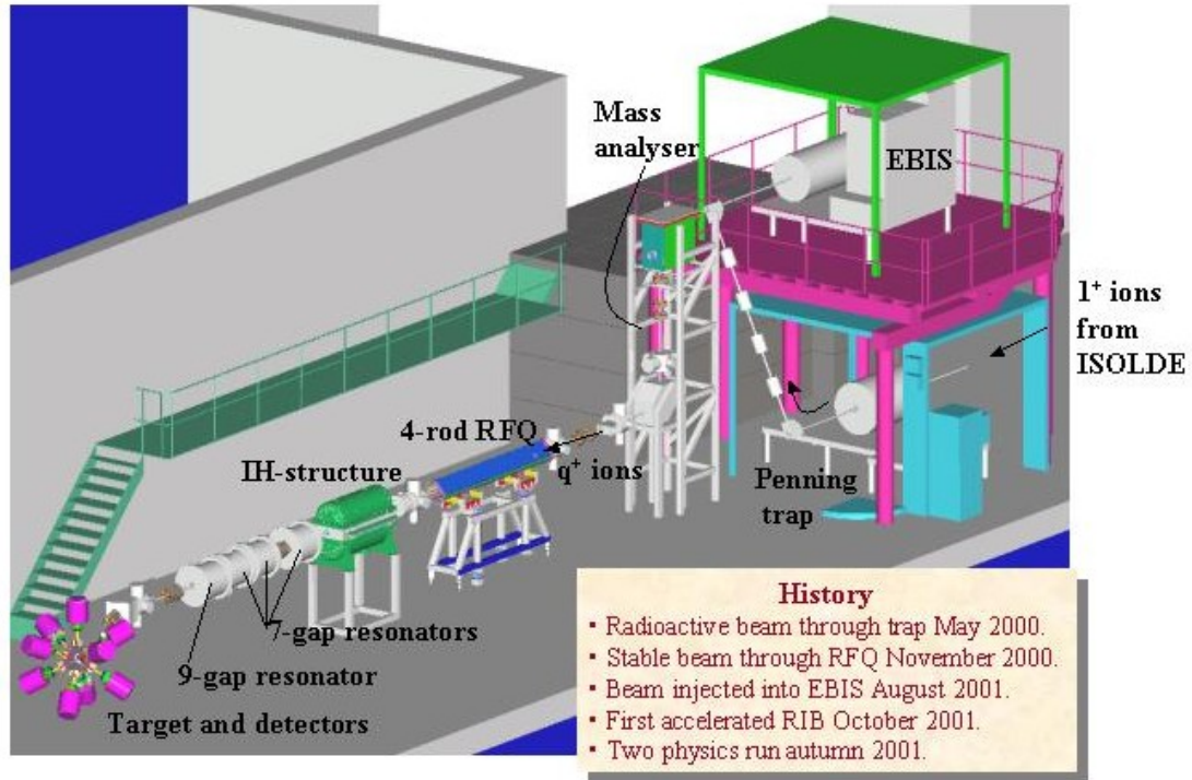
Figure 3.5: The beamline as it appears in the ISOLDE hall at CERN, with significant dates of development included.
