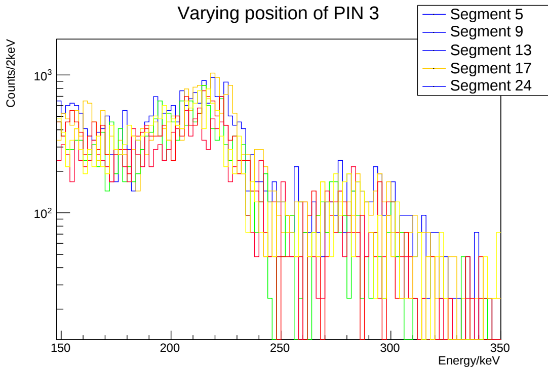
Figure 4.20: Doppler corrected spectra of selected SPEDE channels
