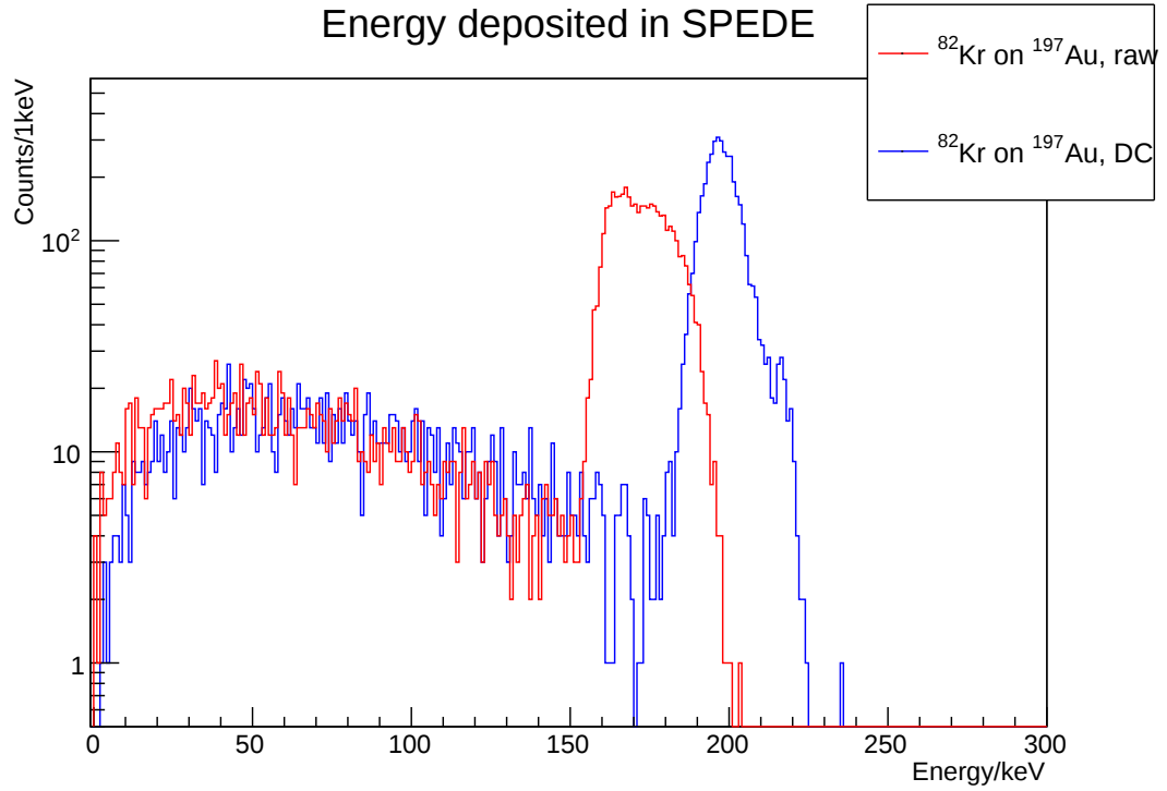
Figure 4.25: Here the simulation is seen, with HV on, of ^{82}\text{Kr} on ^{197}\text{Au} . The FWHM of the peak after Doppler correction is 11.9(4) keV.
