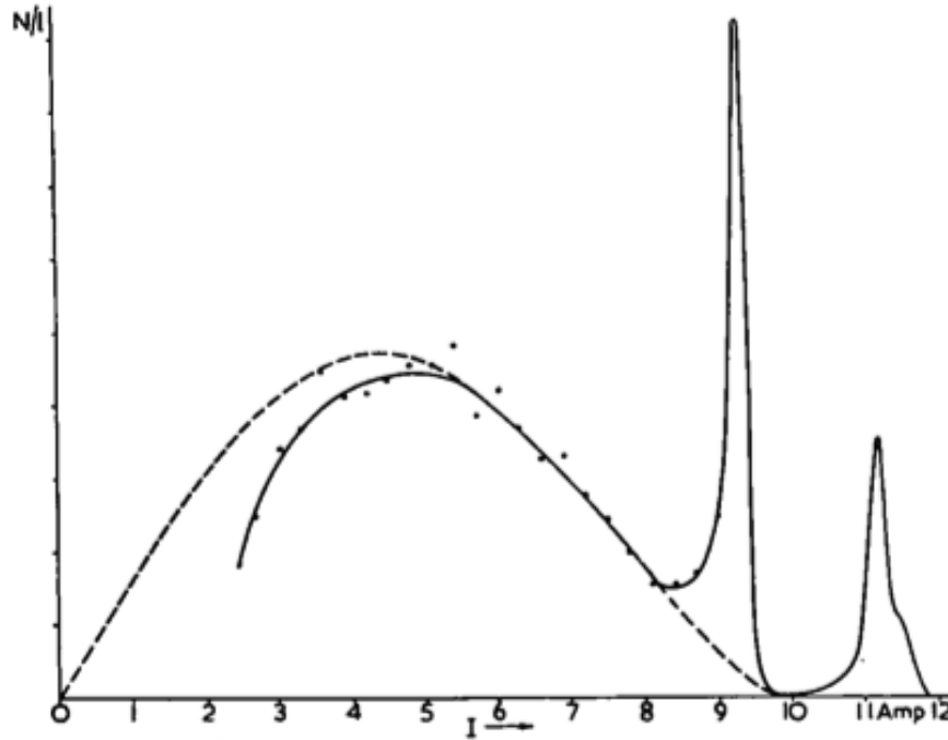
Figure 2.1: This plot shows the decay spectroscopy of ^{203}\text{Hg} . Here, a broad peak can be seen, corresponding to \beta -particles, with three peaks observable on the right-hand side. These correspond to the K-shell, L-shell, and (in the right tail of the L-shell peak) M-shell conversion electrons. Taken from [?].
