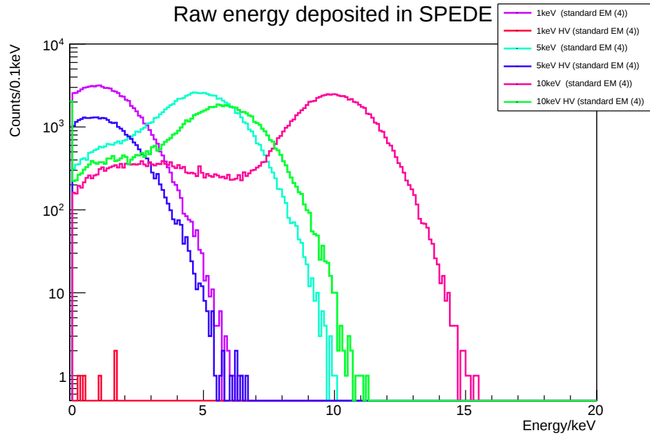
Figure 3.25: Here we can see three distributions using the standard electromagnetic libraries, both with and without high voltage applied. The shift is very clear, although it should be noted that both the 5 keV and the 10 keV distribution appear to shift by only 4 keV rather than the expected 5 keV. There is also a drop in the electron flux when voltage is applied, which is the expected behaviour.
