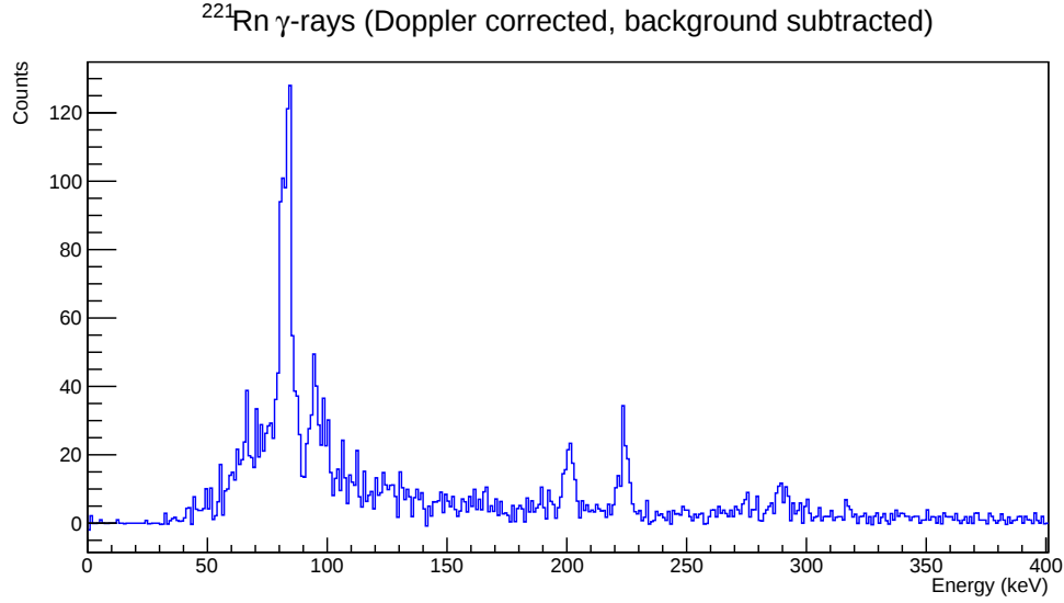
Figure 1.5: Background subtracted \gamma -ray spectrum of ^{221}\text{Rn} , Doppler corrected for ^{221}\text{Rn} . 3 peaks are clearly visible, at 200.42(26) keV, 223.55(25) keV, and 289.73(39) keV.
