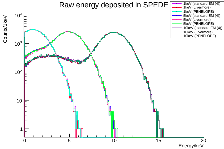
Figure 3.23: Simulated low-energy electron distributions, using different energy libraries. Only differences in the tails are seen clearly, which is a statistical quirk as there are very few counts in these bins.
