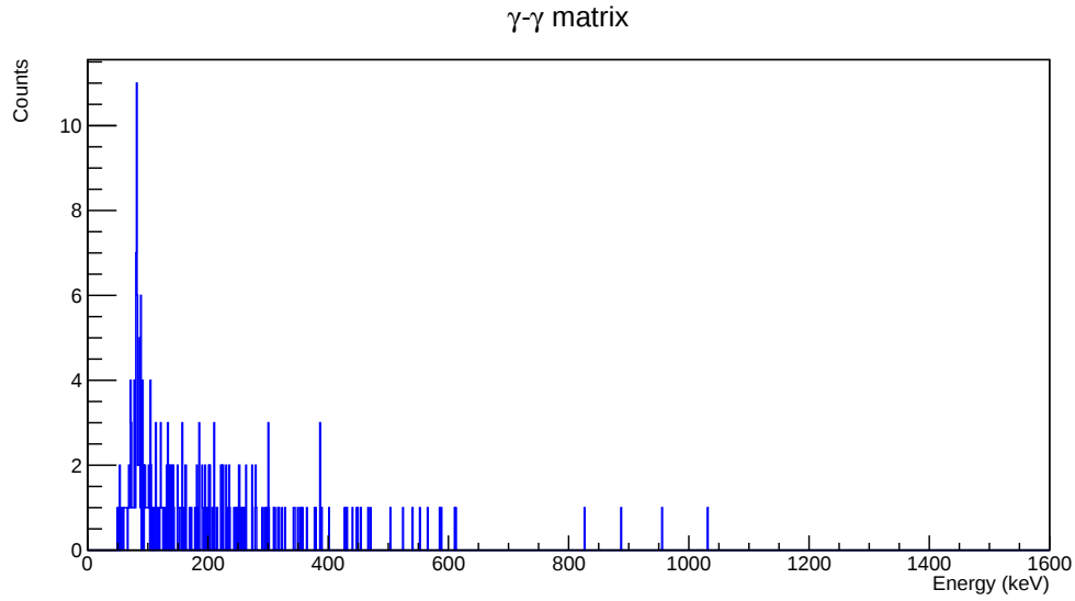
Figure 1.6: \gamma - \gamma matrix showing all coincident \gamma -ray events.
