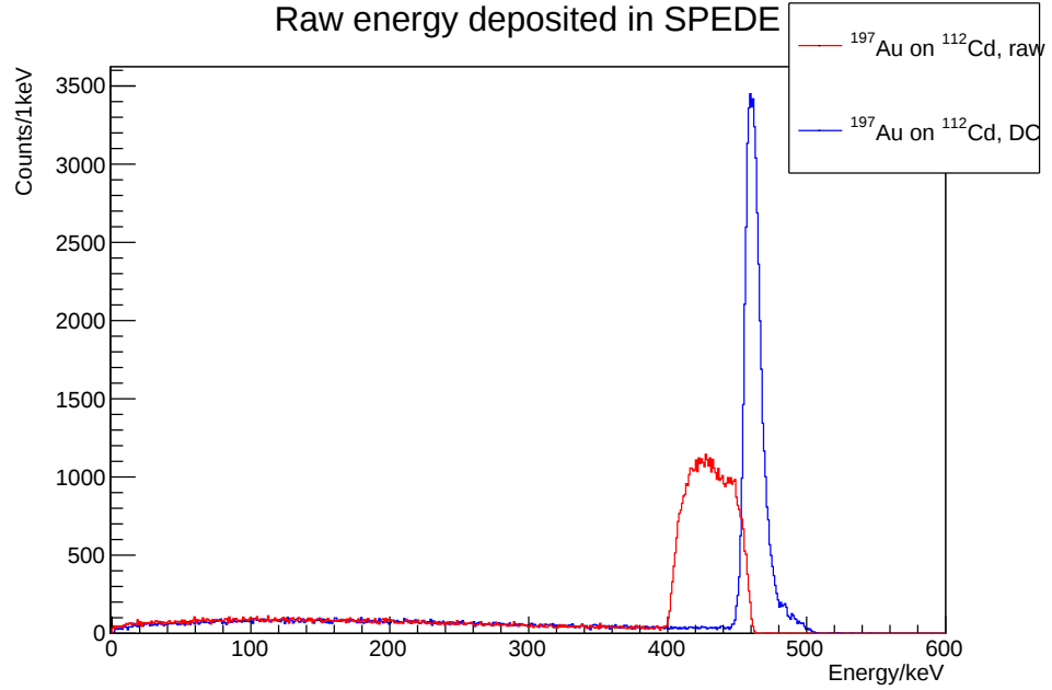
Figure 3.20: Simulated ^{197}\text{Au} on ^{112}\text{Cd} , with Doppler correction
