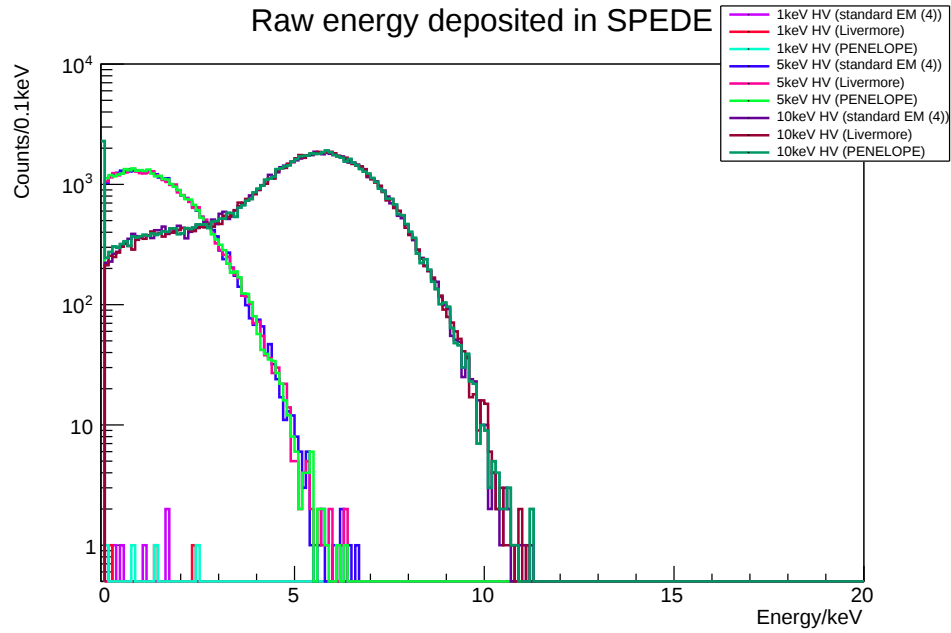
Figure 3.24: Low-energy electron distributions, using different energy libraries, with high voltage simulated. This is similar to Figure 3.23, but it is worth noting that the 1 keV distributions have very few counts seen. This is expected, and shows the high voltage is being applied in the simulation correctly.
