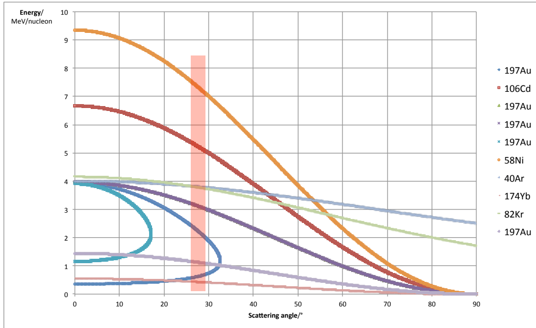
Figure 4.5: This plot shows the energy distribution with angle of scattered nuclei of various beams and targets used in SPEDE tests. Some nuclei, with inverse kinematics, are not seen by the particle detector and therefore can be used for clean gating of the other nucleus. The ideal beam and target combination would have a small change of energy at the position of the detectors, since the energy measurement of the recoiling nuclei was not very accurate, as well as a large separation in energy between the different nuclei. Particle identification can be avoided by using the same nucleus for the beam and the target material. The translucent box shows the approximate angle covered by the 6-PIN array.
