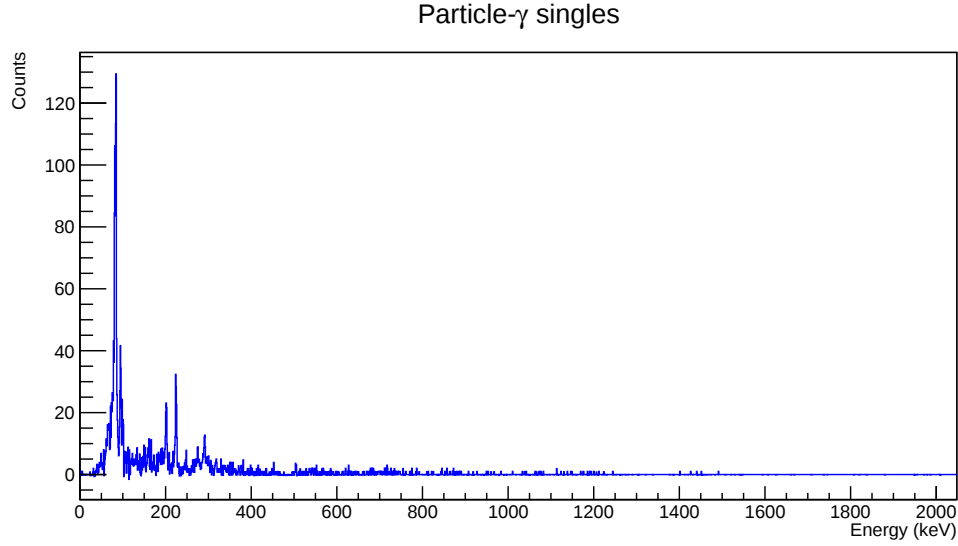
Figure 1.4: \gamma -ray spectrum showing all \gamma -rays in coincidence with a particle detected by the MINIBALL array during the course of the experiment.
