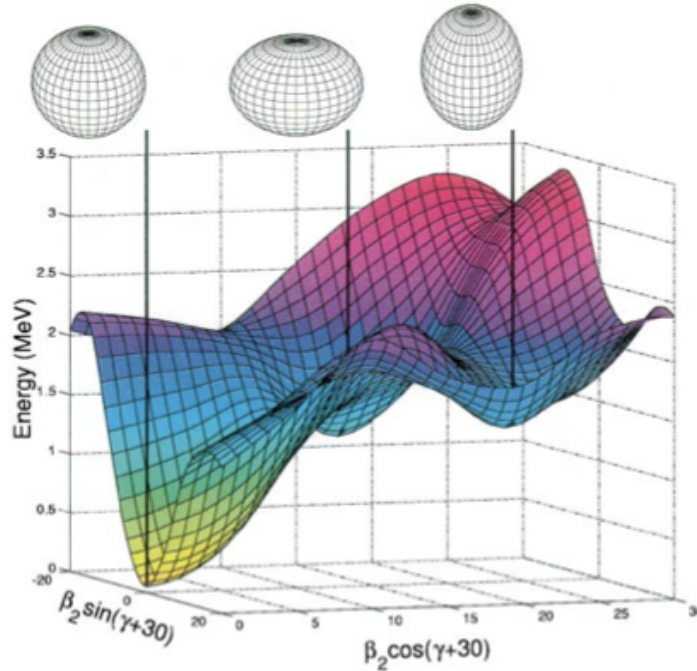
Figure 1.9: Calculated potential energy surface of ^{186}\text{Pb} . Spherical, oblate and prolate shape deformations are respectively indicated from left to right by the thicker vertical lines. Obtained from [?].
