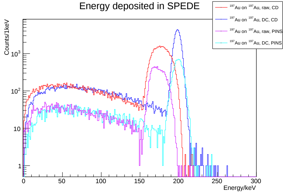
Figure 3.21: Simulated ^{197}\text{Au} on ^{197}\text{Au} , with Doppler correction, using different particle detectors. Using the CD detector, the number of electrons detected in coincidence with a particle is higher. Additionally, the resolution is slightly improved.
