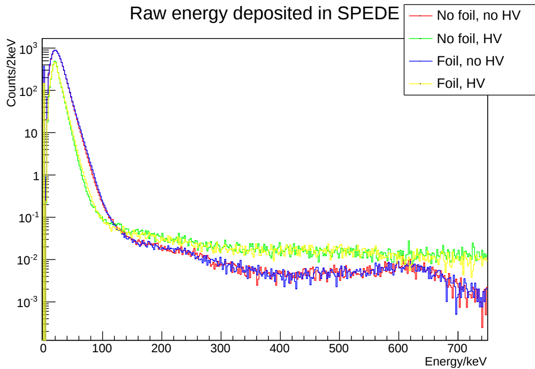
Figure 4.14: ^{84}\text{Kr} on ^{197}\text{Au} , with & without foil
