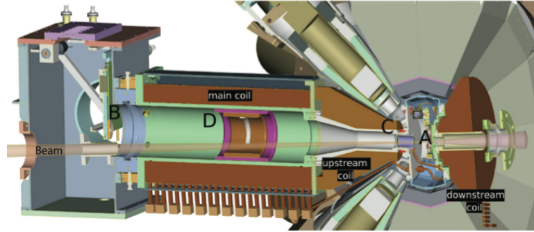
Figure 2.8: The SAGE detector
