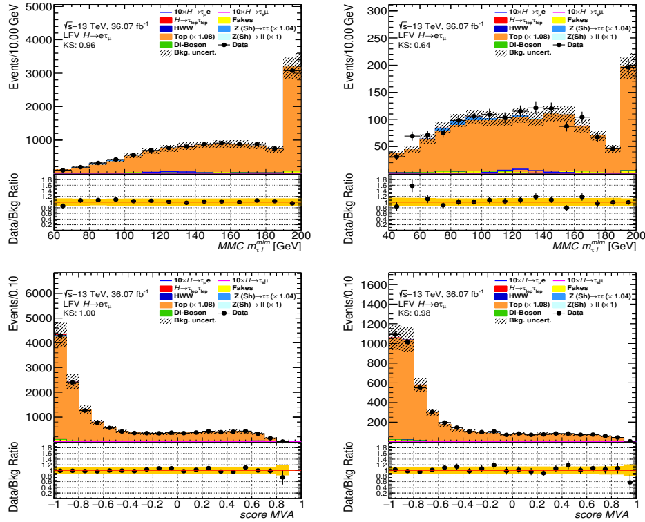
Figure 5.25: Top control region distributions of the MMC mass and the BDT score for e\tau_\mu events after non-VBF (left) and VBF (right) selection. Pre-fit normalization factors obtained in the baseline top control region have been applied. Error bands include the statistical uncertainties and the systematic uncertainties on the background normalization.
