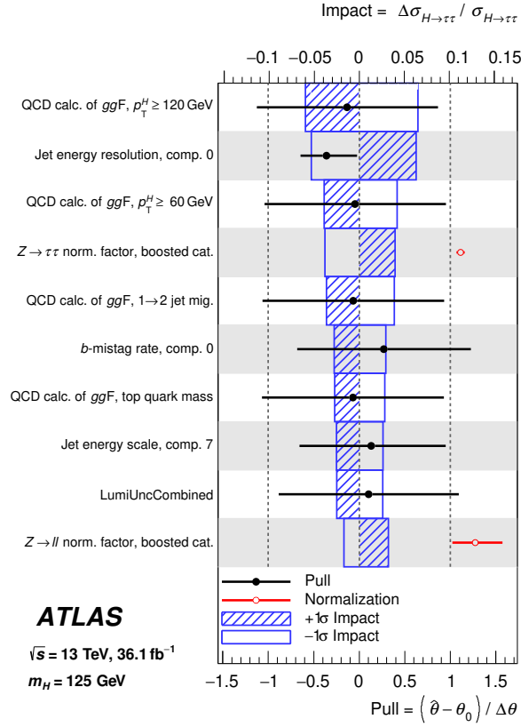
Figure 4.15: Fractional impact of systematic uncertainties in \sigma_{H \rightarrow \tau\tau} as computed by the fit. The systematic uncertainties are listed in decreasing order of their impact on \sigma_{H \rightarrow \tau\tau} on the y -axis. The hatched blue and open blue boxes show the variations of \sigma_{H \rightarrow \tau\tau} referring to the top x -axis (impact). The filled circles, referring to the bottom x -axis, show the pulls of the fitted nuisance parameters, i.e. the deviations of the fitted parameters \hat{\theta} from their nominal values \theta_0 , normalized to their nominal uncertainties \Delta\theta . The black lines show the uncertainties of the nuisance parameters resulting from the fit. Several sources of uncertainties such as the jet energy scale and resolution as well as the b -mistag rate are described by their principal components in the fit. The open circles, also referring to the bottom x -axis, show the values of the fitted Z \rightarrow \tau\tau and Z \rightarrow \ell\ell normalization factors in the boosted category. Their uncertainties do not include uncertainties in total simulated cross-sections extrapolated to the selected phase space. Reproduced from Ref. [117] under CC-BY-4.0 licence.
