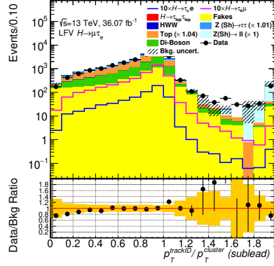
Figure 5.3: Distributions for the ratio between the electron ID track p_T and the electron cluster transverse energy. The baseline selection criteria, shown in Table 5.1, are applied except the p_T^{\text{track}}(\ell_2)/p_T^{\text{cluster}}(\ell_2) < 1.2 requirement. Error bands include the statistical uncertainties and the systematic uncertainties on the background normalization.
