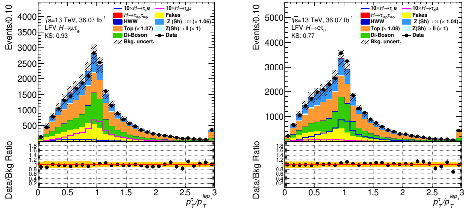
Figure 5.10: Kinematic distribution for the \mu\tau_e (left) and e\tau_\mu (right) final state for events passing the baseline selection. The p_T^{\tau}/p_T^{\ell_1} distributions are shown. Error bands include the statistical uncertainties and the systematic uncertainties on the background normalization.
