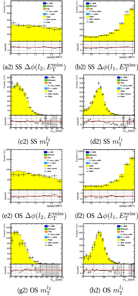
Figure A.17: The \Delta\phi(l_2, E_T^{\text{miss}}) , \Delta\phi(l_1, E_T^{\text{miss}}) , m_T^{l_2} and m_T^{l_1} distributions after the corrections in the \mu e channel SS (a2-d2) and OS (e2-h2) nominal b -veto region after the preselection. The errors are statistical only.
