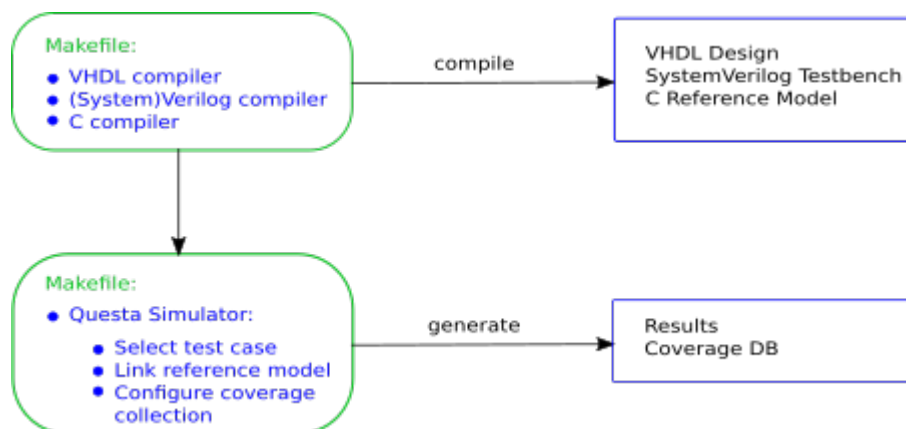
Figure 5.1: Simulation-based Verification Toolchain
