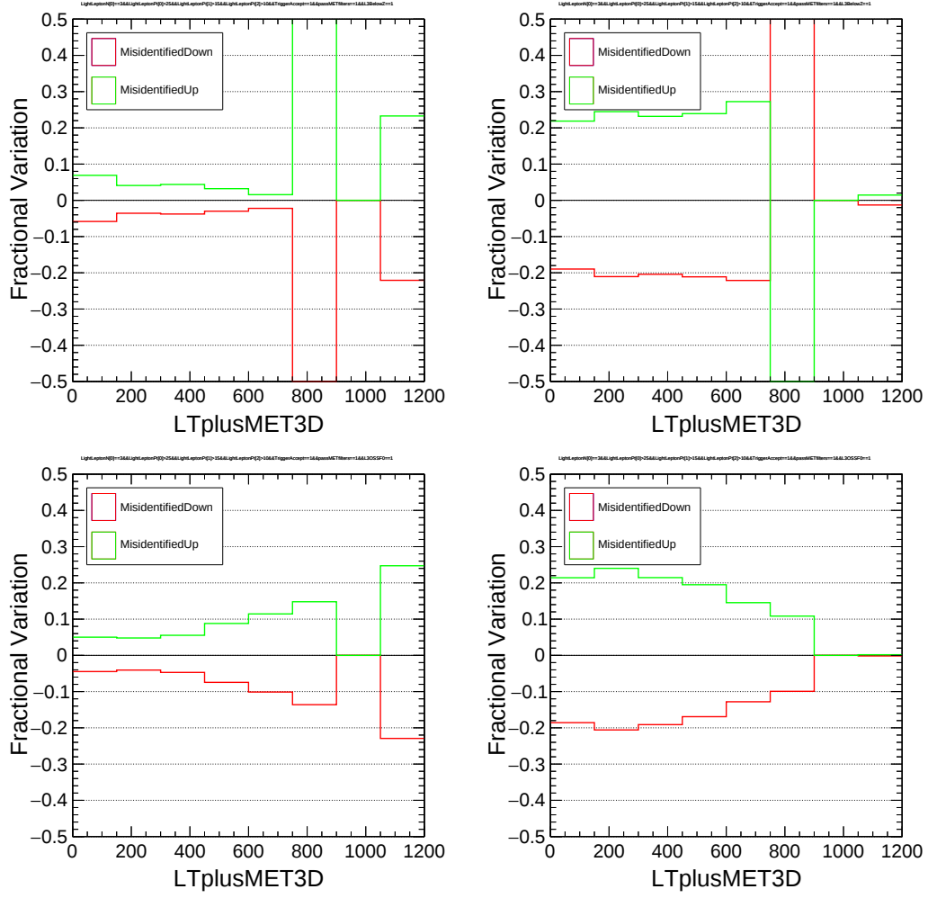
FIGURE 6.14: The relative variations of the misidentified lepton background estimate in data events in below- Z (upper) and OSSF0 (lower) trilepton signal regions as a function of L_T + E_T^{\text{miss}} . The up-down bands on the mean misidentified lepton background correspond to the independent variations of the electron (left) and muon (right) fake rates within their total respective uncertainties. Bins with variations greater than 30% correspond to those where the misidentified lepton background estimate is less than 0.1 event.
