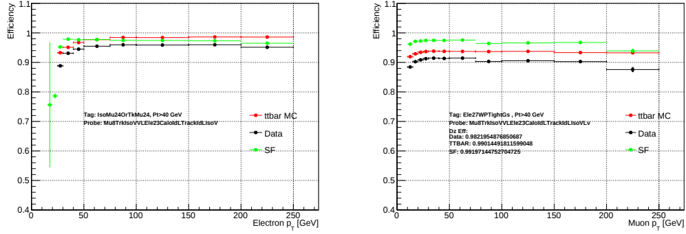
FIGURE B.3: Electron (left) and muon (right) leg efficiencies for the HLT_Mu8_TrkIso-VVL_Ele23_CaloIdL_TrackIdL_IsoVL trigger path as measured in events with a muon+electron pair in the full 2016 dataset and in MC, collected by a single muon or a single electron trigger, respectively. The DZ filter efficiency is found to be 0.98 in data and 0.99 in MC.
