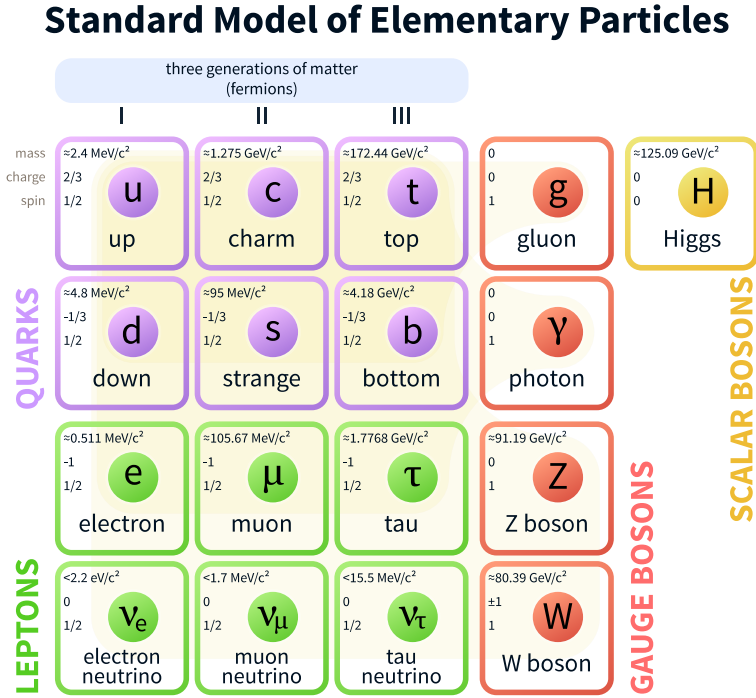
FIGURE 2.1: The SM particle content and their properties are listed here. The particles are grouped as lepton, quarks, gauge bosons and a scalar Higgs boson [1]
