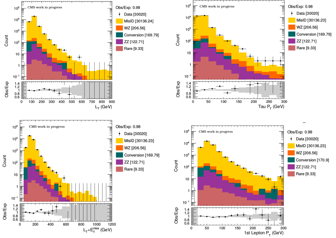
FIGURE 8.1: L_T (upper left), \text{Tau } p_T (upper right), L_T + p_T^{\text{miss}} (lower left), and first lepton p_T (lower right) distributions in L2T1 with p_T^{\text{miss}} < 50 \text{ GeV} CR (last bin includes overflow). Uncertainty bands in the ratio plots in the lower panel include statistical uncertainties only.
