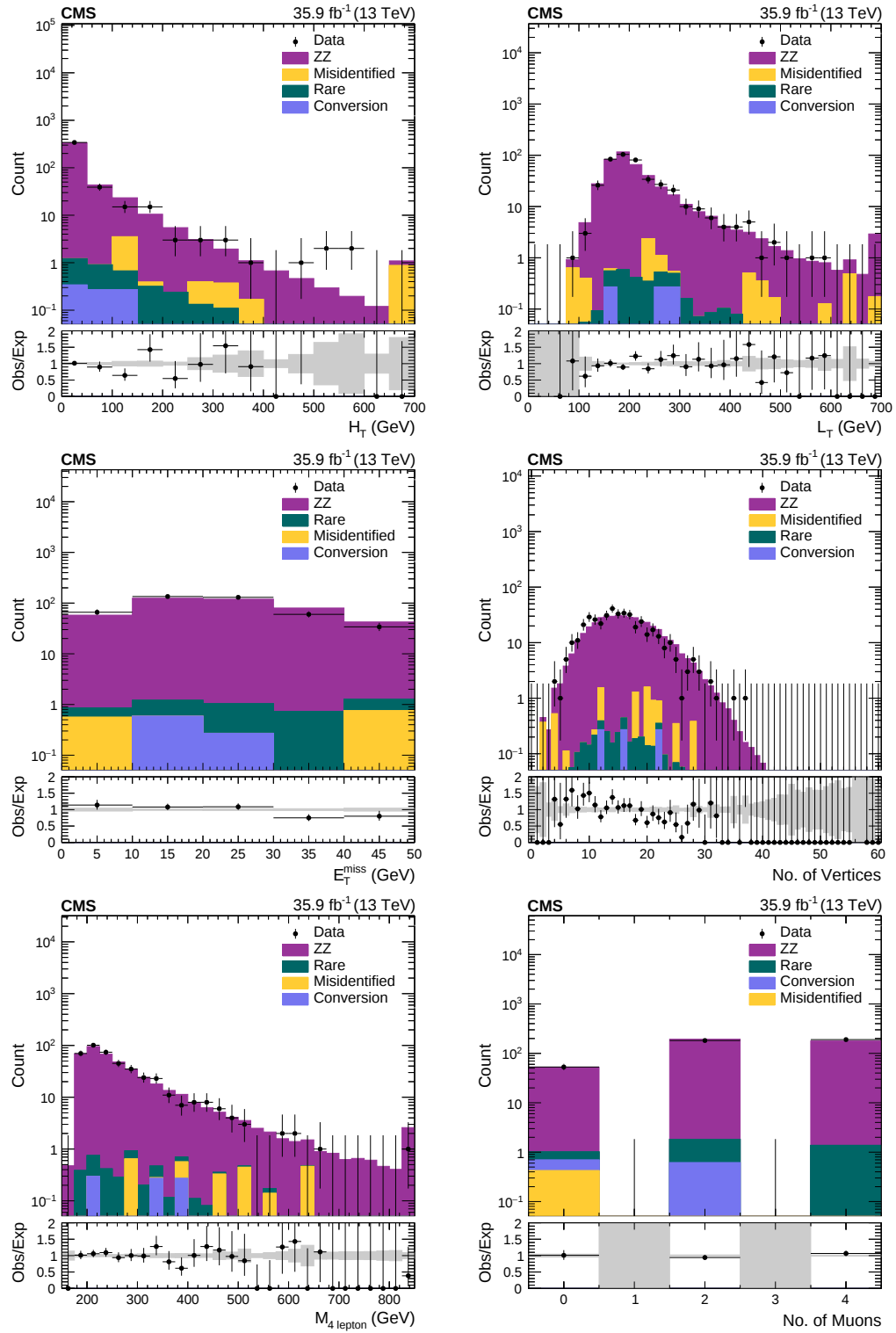
FIGURE 6.5: The H_T (upper left), L_T (upper right), E_T^{\text{miss}} (center left), primary vertex multiplicity (center right), M_{4\ell} (lower left), and muon multiplicity (lower right) distributions in the ZZ enriched selection of events. All plots include the ZZ cross-section normalization correction. The last bins include overflow events. The uncertainty bands in the ratio plots include statistical uncertainties only.
