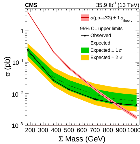
FIGURE 7.8: Observed exclusion limit at 95% CL on the production cross-section of \Sigma pairs, as calculated with the asymptotic CL_s mode of the Higgs Combination Tool. All systematic uncertainties listed in Table 6.5 are included.
