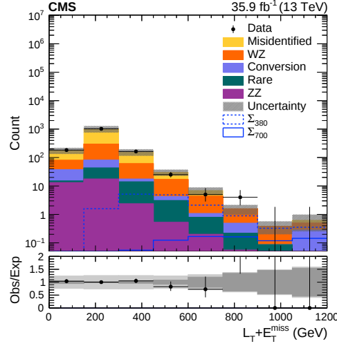
FIGURE 7.1: L_T + E_T^{\text{miss}} distribution for the 3 lepton, below- Z signal region as defined in Table 5.2. The expected yields of the Seesaw signal model with M_\Sigma = 380 GeV and M_\Sigma = 700 GeV are overlaid. The last bin includes overflow events. The uncertainty band includes systematic uncertainties listed in Table 6.5.
