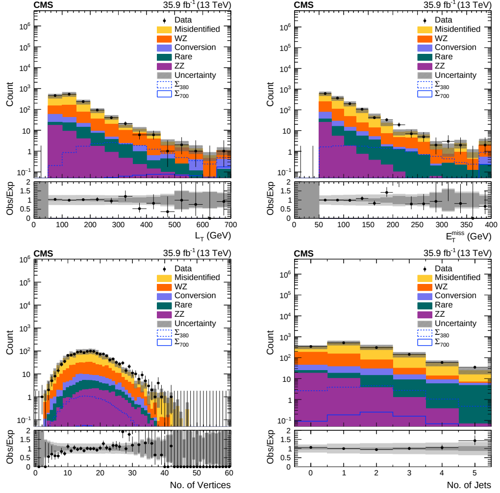
FIGURE 7.2: L_T (upper left), E_T^{\text{miss}} (upper right), primary vertex multiplicity (lower left), and jet multiplicity (lower right) distributions for the 3 lepton, below-Z signal region as defined in Table 5.2. The expected yields of the Seesaw signal model with M_\Sigma = 380 GeV and M_\Sigma = 700 GeV are overlaid. The last bins include overflow events, and the uncertainty bands in the ratio plots include statistical (dark) and systematic (light) uncertainties.
