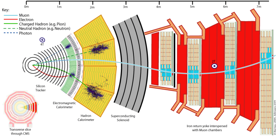
FIGURE 4.1: Various Particle Detection at CMS [10]
