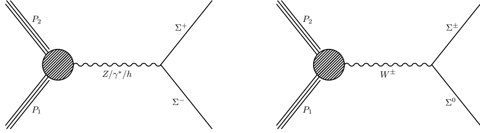
FIGURE 5.1: Examples of Feynman diagrams for heavy fermion production in the Type-III Seesaw model.
