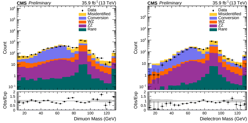
FIGURE 6.17: MOSSF distributions in the conversion electron dominated selection of events in \mu^\pm\mu^\mp e (left) and e^\pm e^\mp e (right) final states. Events in the \mu^\pm\mu^\mp e selection where M(2\mu) is below- Z ( < 81 GeV) is used to measure the photon-to-electron conversion rates, and those in the e^\pm e^\mp e selection is used to demonstrate the closure of the method in an orthogonal selection. All selections require E_T^{\text{miss}} < 50 GeV. Uncertainty bands in the ratio plots in the lower panel include statistical uncertainties only.
