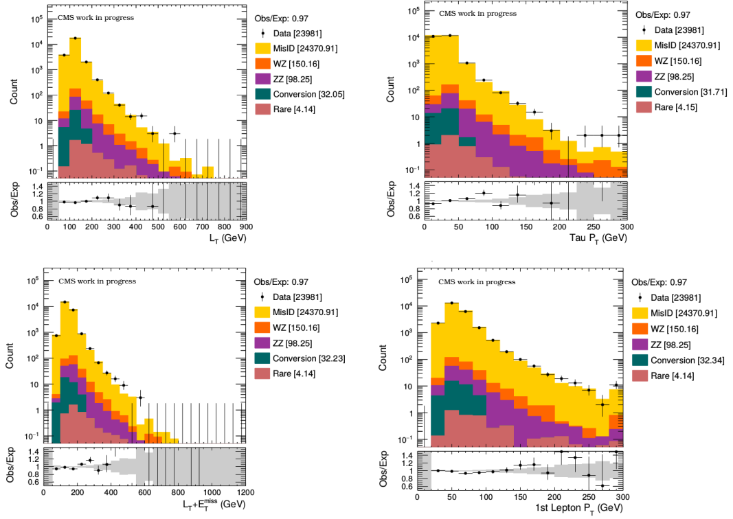
FIGURE 8.3: L_T (upper left), Tau p_T (upper right), L_T + p_T^{\text{miss}} (lower left), and first lepton p_T (lower right) distributions in L2T1 Off-Z with p_T^{\text{miss}} < 50 GeV CR (last bin includes overflow). Uncertainty bands in the ratio plots in the lower panel include statistical uncertainties only.
