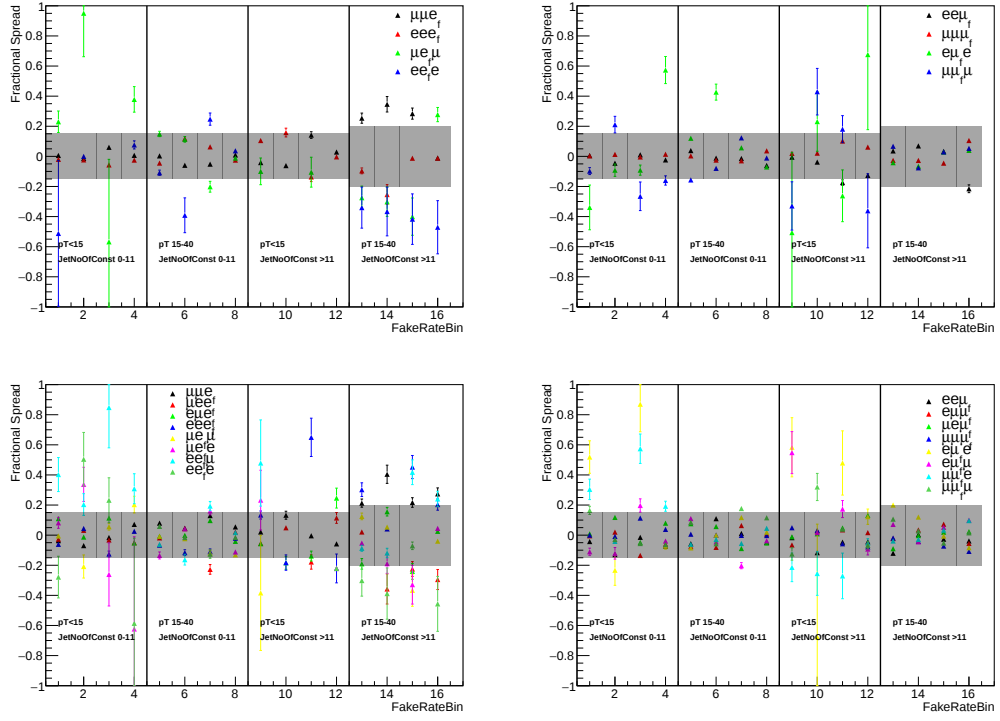
FIGURE 6.12: Flavor- p_T order dependent systematics on the electron (left) and muon (right) fake rates as measured in simulated DY+jets (upper) and t\bar{t} +jets (lower) events. In each plot, the enumerated labels on the x-axis represent different bins used in the parametrization of fake rates (such that each set of 4 consecutive bins correspond to a set of 4 |\eta| bins as presented in Appendix D) and the y-axis is the fractional change of the fake rate at a given flavor- p_T order scenario (as indicated in the legend, subscript f indicated the fake lepton) with respect to the inclusive fake rate in that bin. The gray bands represent the uncertainties assigned to the inclusive fake rates to account for these variations in each region (15-20%). These internal uncertainties mostly become relevant for the matrix method in the limit that process dependent (DY vs t\bar{t} ) variations on the fake rates become negligible, and therefore are utilized as minimum lower bounds on the MC based fake rate systematic uncertainties.
