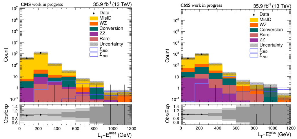
FIGURE 8.4: Partially un-blinded L_T + p_T^{\text{miss}} distributions in L2T1 Above Z(left), and L2T1 OSSF0 (right) signal regions. Uncertainty bands in the ratio plots in the lower panel include statistical as well as systematic uncertainties.
