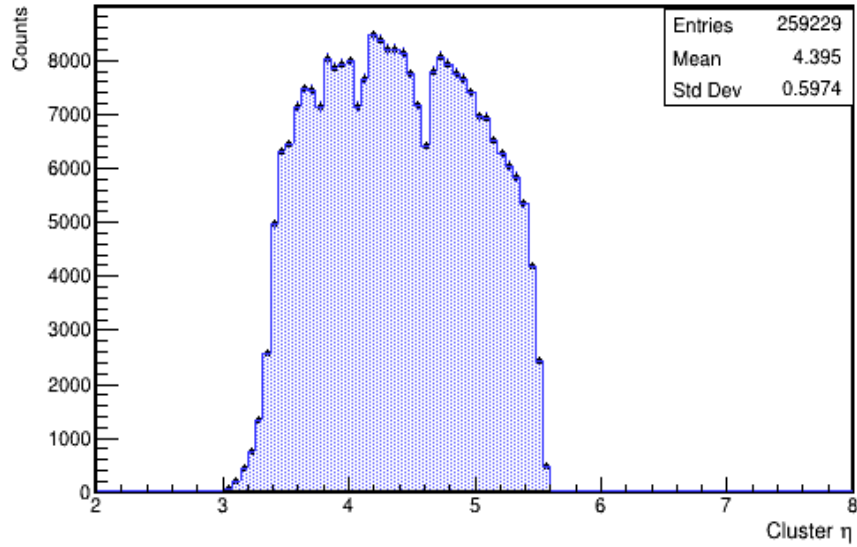
FIGURE 2.4: Pseudorapidity distribution of cluster in pp collision in FOAL
