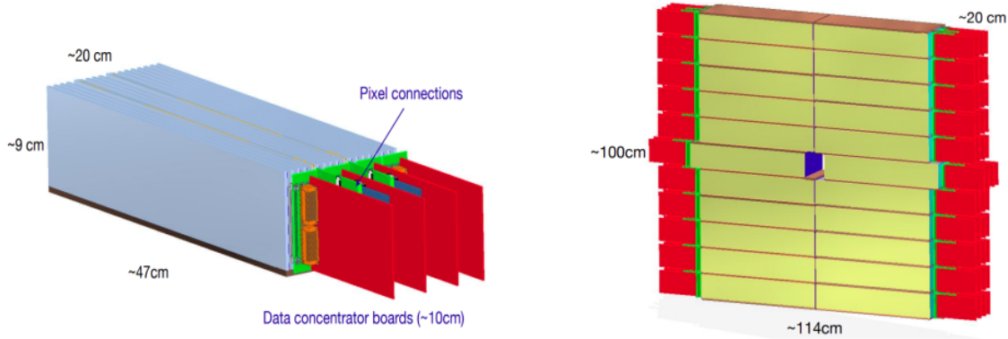
FIGURE 2.5: FoCal-E 22 modules, each 18 Pad + 2 Pixel layers
