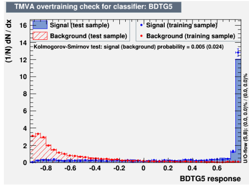
(c) nodeSize = 0.5%.
