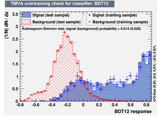
(b) adaBoostBeta = 0.2.
