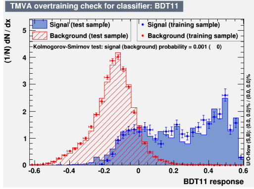
(a) adaBoostBeta = 0.5.
