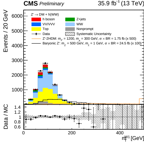
(a) m_T^{W1} .
