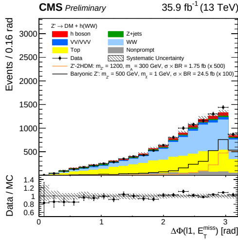
(c) \Delta\phi(E_T^{miss}, \ell_1) .
