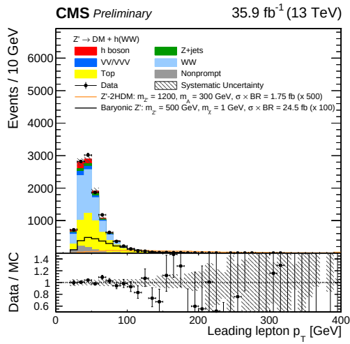
(e) leading lepton p_T .
