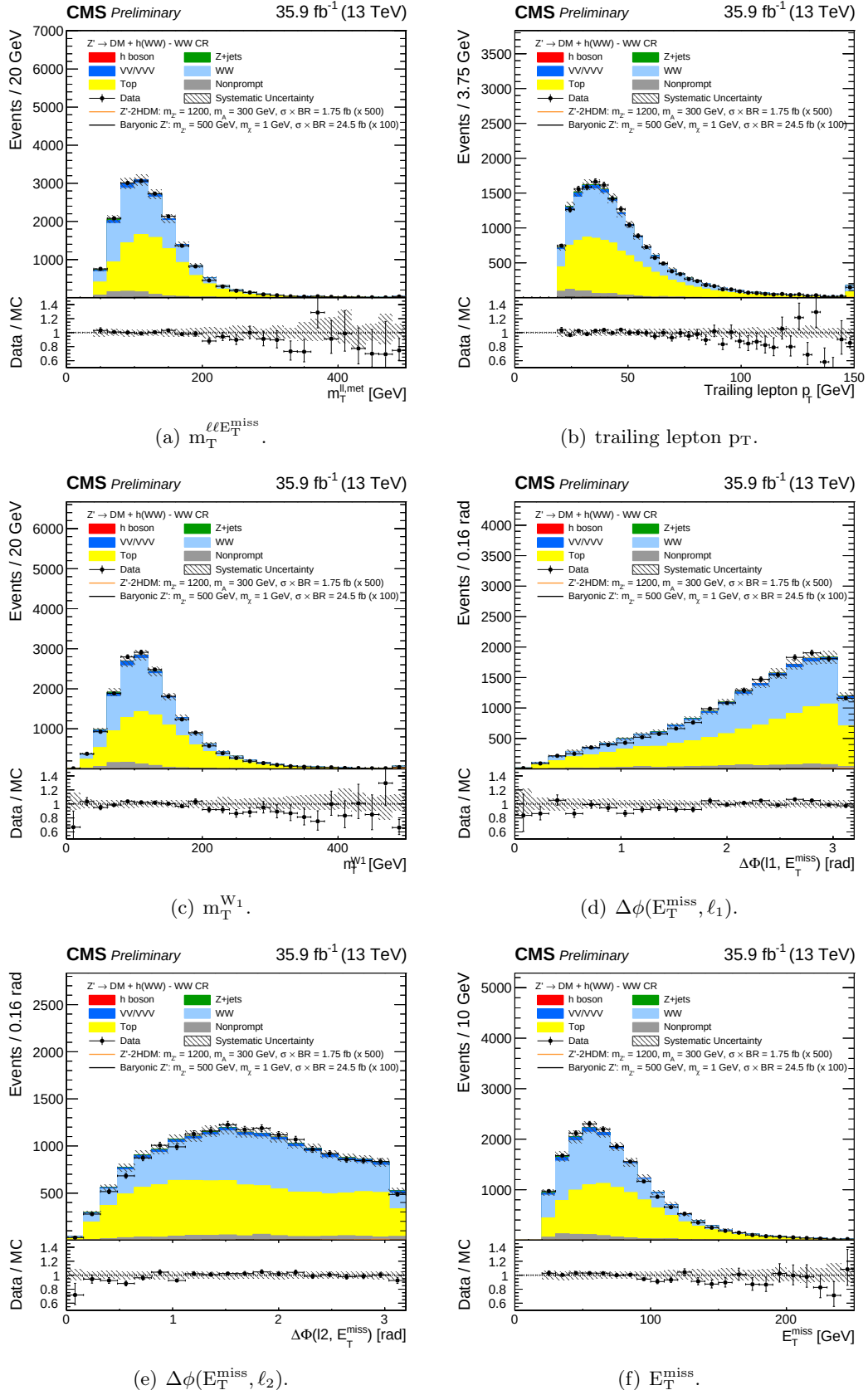
Figure 8.13: Control plots for several variables in the WW control region.
