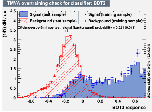
(c) nTrees = 2000 .
