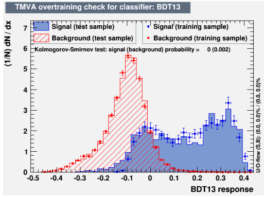
(c) adaBoostBeta = 0.8.
