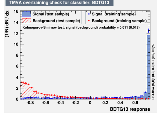
(b) baggingFraction = 1.
