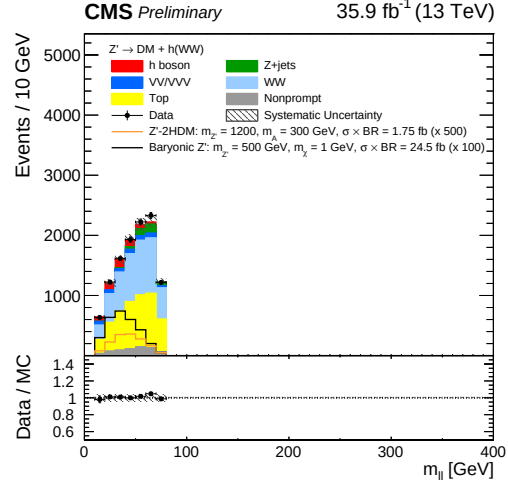
(b) m_{\ell\ell} .
