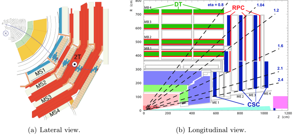
Figure 4.15: Schematic representation of the CMS muon system. The lateral view on the left (a) shows the typical trajectory of a muon. On the right (b), the view is presented in the rz -plane.
