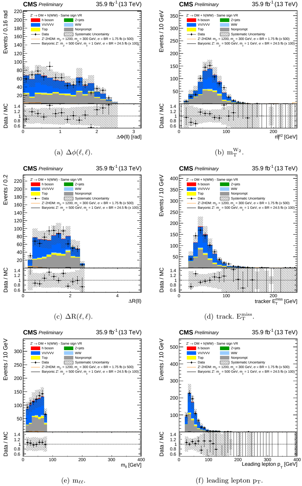
Figure 8.25: Control plots for several variables in the b-veto same-sign validation region.
