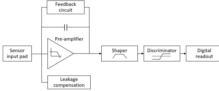
Figure 2.8. Block diagram of a typical front-end circuit implementation.
