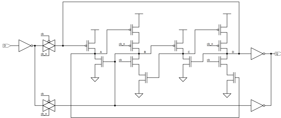
Figure 4.24. Example of a dual-interlocked (DICE) latch schematic [111].
