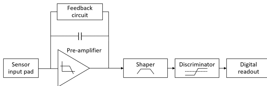
Figure 4.1. SSA analog front-end block diagram.
