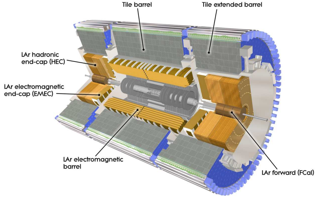
Figure 3.4: General cut-away view of the calorimeters [55].
