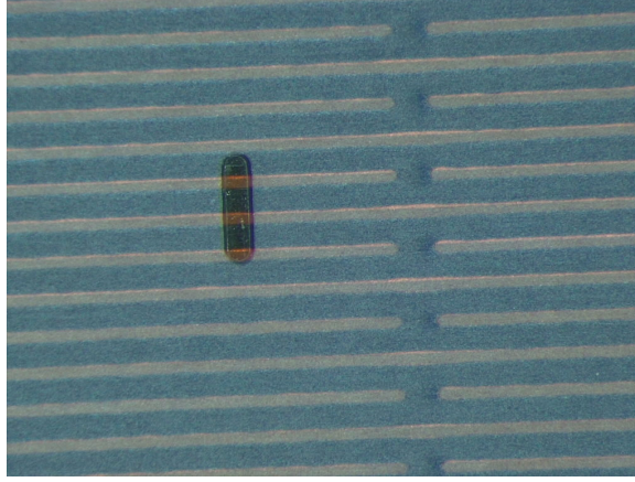
Figure 3.3 – Photo of a pillar on top of the readout panel of NSW Micromegas. The surface of this supporting pillar is about 1.2\text{ mm} \times 200\text{ }\mu\text{m} . The strips in shallow color are the resistive strips.
