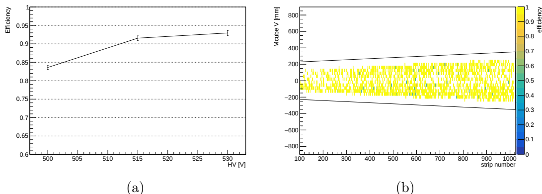
Figure 3.35 – The efficiency of M25 PCB1 Layer2 using 93 %Ar + 5 %CO 2 + 2 %iso-C 4 H 10 gas mixture. (a) HV scan of efficiency. (b) Efficiency map of M25 PCB1 Layer2 at 515 V.
