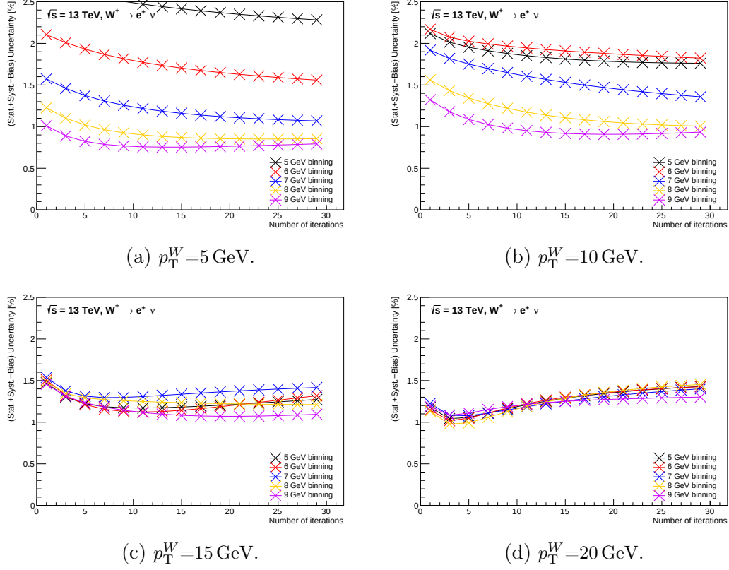
Figure 7.4 – Total uncertainty in various bin widths over different iterations for 13 TeV W^+ \rightarrow e\nu channel. The total uncertainty is interpolated to p_T^W=5, 10, 15, 20 GeV.
