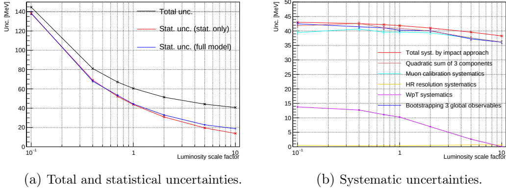
Figure 9.2 – Uncertainty decomposition for the profile likelihood fit based on muon p_T spectrum. For the total systematic uncertainty, the result of bootstrapping three global observables simultaneously is compatible with the quadratic sum of bootstrapping the three components individually.
