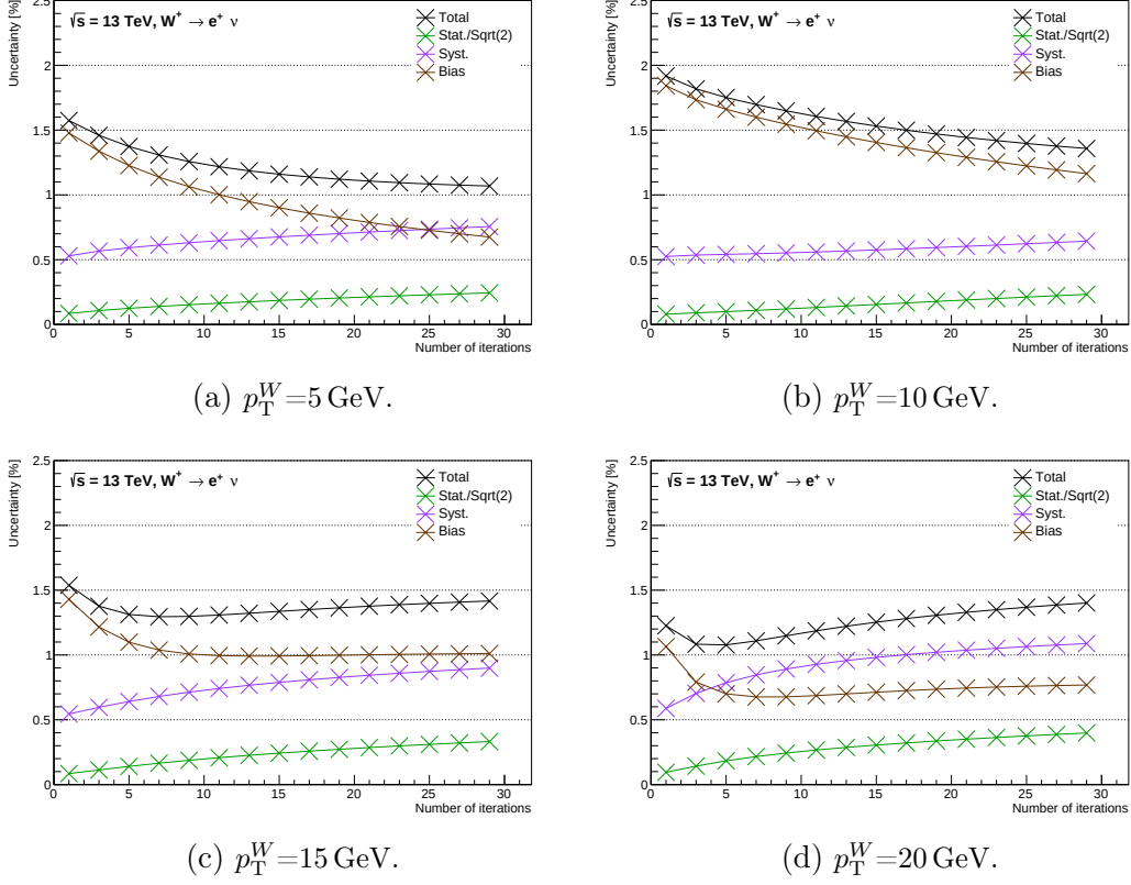
Figure 7.6 – Total uncertainty in various binnings over different iterations for 13 TeV W^+ \rightarrow e\nu channel. The total uncertainty is interpolated to p_T^W=5, 10, 15, 20 GeV.
