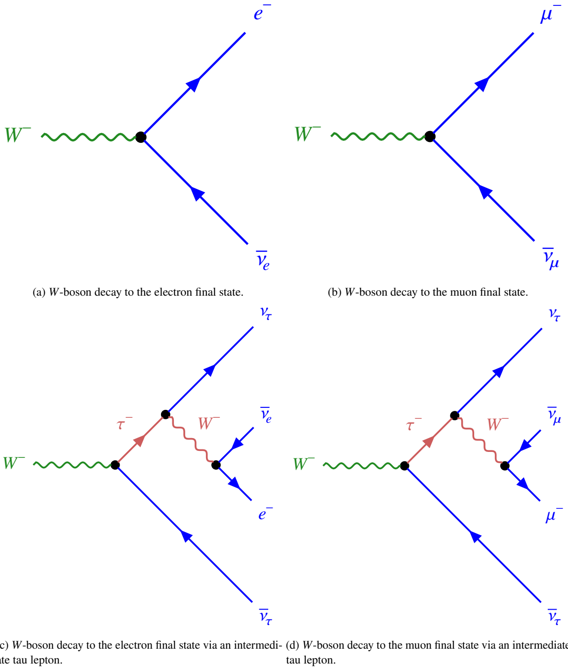
Figure 2.10: Feynman diagrams of the four possible leptonic decays of the W -boson containing a light lepton in the final state. Whereas (a) and (b) show the prompt decay of a W -boson (green) to a light lepton and the corresponding neutrino (both in blue), (c) and (d) show the decay via an intermediate tau lepton (red). Shown are only diagrams for negatively charged particles, whereas the decay chains for positively charged particles look similar.
