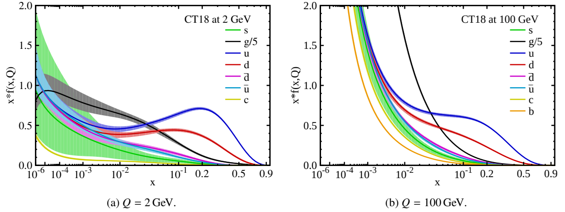
Figure 2.12: The PDFs of the CT18 global analysis at (a) Q = 2 \text{ GeV} and (b) Q = 100 \text{ GeV} for u, \bar{u}, d, \bar{d}, s = \bar{s} and g . The gluon PDF is scaled down by a factor of 5 (taken from [30]).
