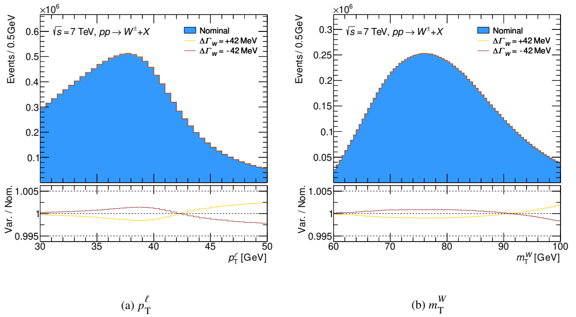
Figure B.2: Width templates for the nominal hypothesis and two width variations. Shown is the sum of all fitting categories of both processes initiated by a W -boson, W \rightarrow \ell \nu and W \rightarrow \tau \nu , for the kinematic distributions p_T^\ell (a) and m_T^W (b). The lower panel illustrates the ratio of the width variations compared to the nominal width template.
