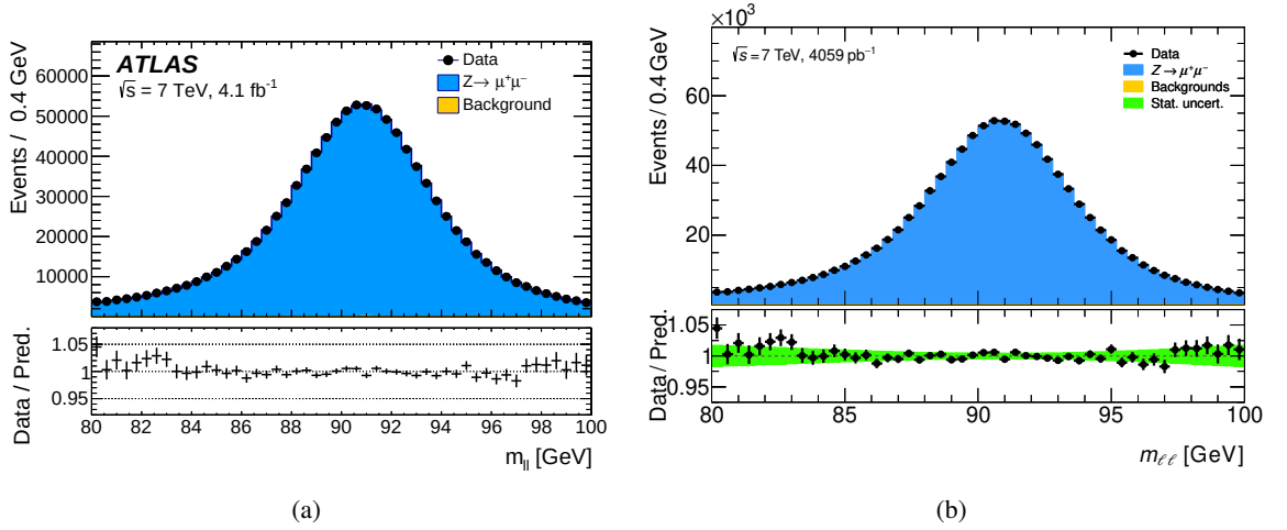
Figure 7.4: Comparison of the data to simulation agreement of the invariant dimuon mass in Z \rightarrow \mu\mu events between (a) the 2017 analysis (taken from [86]) and (b) the reanalysis. All corrections concerning the momentum calibration and the selection efficiency are applied to the simulation, whereas the sagitta bias correction is applied to data. The lower panel shows the ratio of data to simulation where the error bars indicate the statistical uncertainty and the green band represents the uncertainty caused by the limited simulation sample size.
