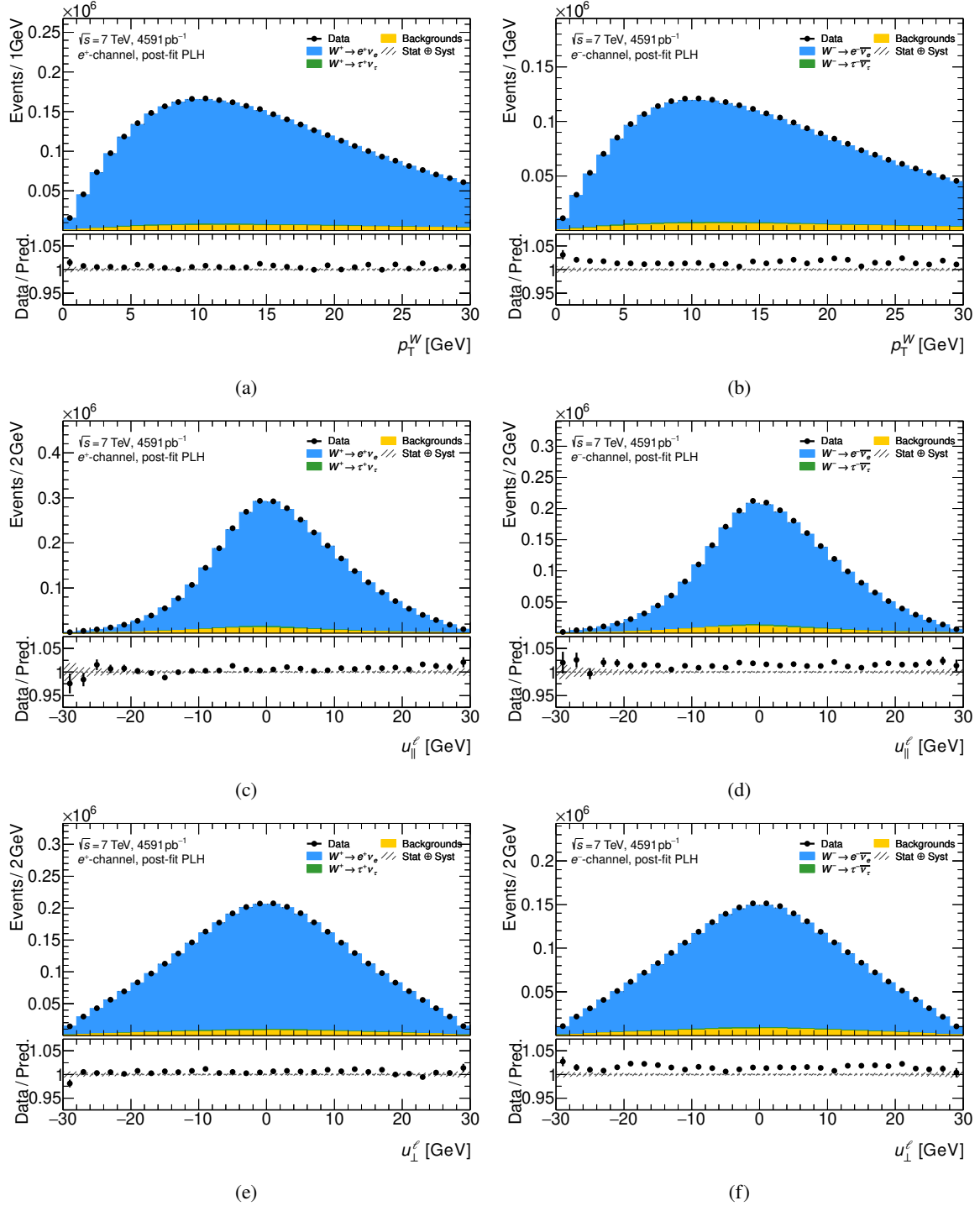
Figure F.9: Illustration of the post-fit recoil distribution in the electron channel for p_T^{\ell} fits of the W -boson mass. Shown are the distributions of p_T^W (a,b), u_{\parallel}^{\ell} (c,d), and u_{\perp}^{\ell} (e,f) for positively (a,c,e) and negatively (b,d,f) charged electrons.
