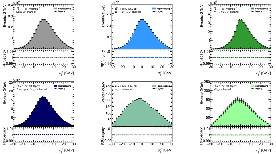
Figure C.9: Comparison between distributions published in the 2017 analysis (black dots) and the reprocessed samples (coloured filled areas) for muons with charge q = -1 and the observable u_{\parallel}^{\ell} . Shown are the distributions of the data sample and the five MC samples.
