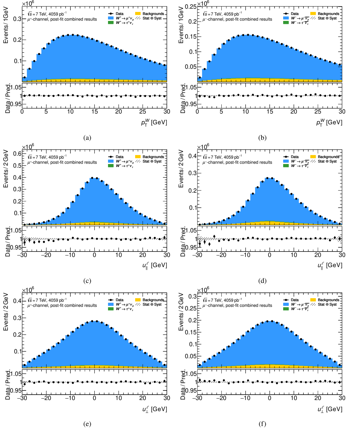
Figure F.23: Illustration of the post-fit recoil distribution in the muon channel for p_T^\ell fits of the lepton universality. Shown are the distributions of p_T^W (a,b), u_{\parallel}^\ell (c,d), and u_{\perp}^\ell (e,f) for positively (a,c,e) and negatively (b,d,f) charged muons.
