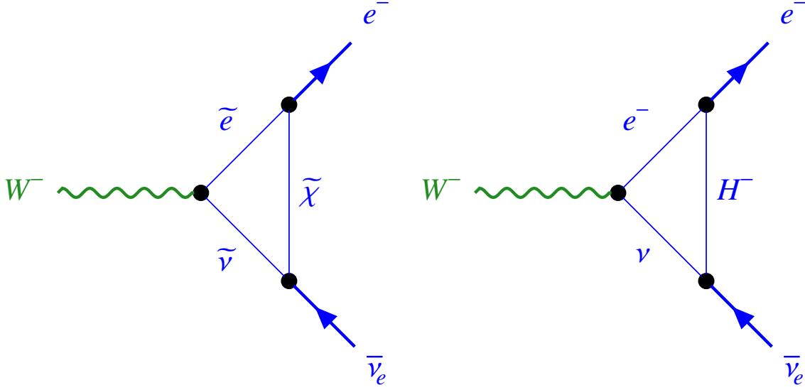
(a) W -boson decay via an intermediate loop containing super-symmetric particles. (b) W -boson decay via an intermediate loop containing a charged Higgs-boson.
