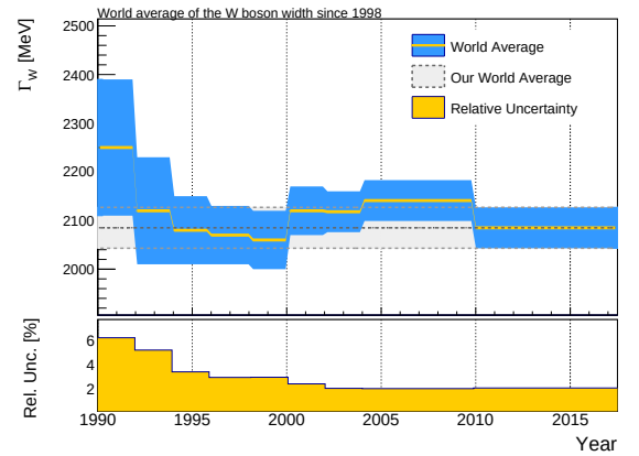
(b) Precision of the \Gamma_W measurement over the course of time.
