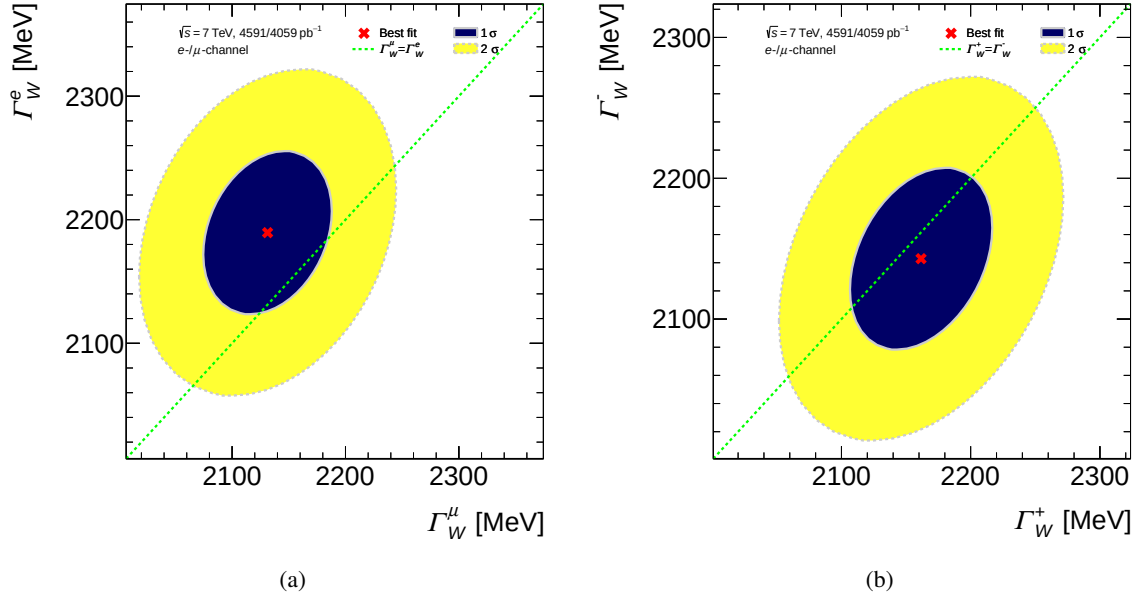
Figure 8.9: Consistency plots for different sub-fits of the W -boson width measurement performed in the m_T^W distribution. Shown are the central value and the 1 \sigma and 2 \sigma uncertainty contours for two POIs acting (a) on the different leptonic decay channels and (b) on the different charges of the final state lepton.
