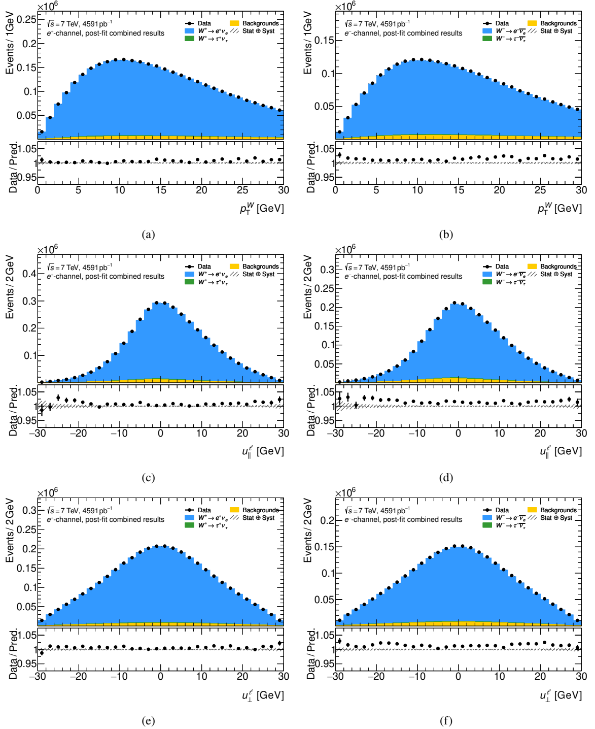
Figure F.17: Illustration of the post-fit recoil distribution in the electron channel for p_T^\ell fits of the W -boson width. Shown are the distributions of p_T^W (a,b), u_{\parallel}^\ell (c,d), and u_{\perp}^\ell (e,f) for positively (a,c,e) and negatively (b,d,f) charged electrons.
