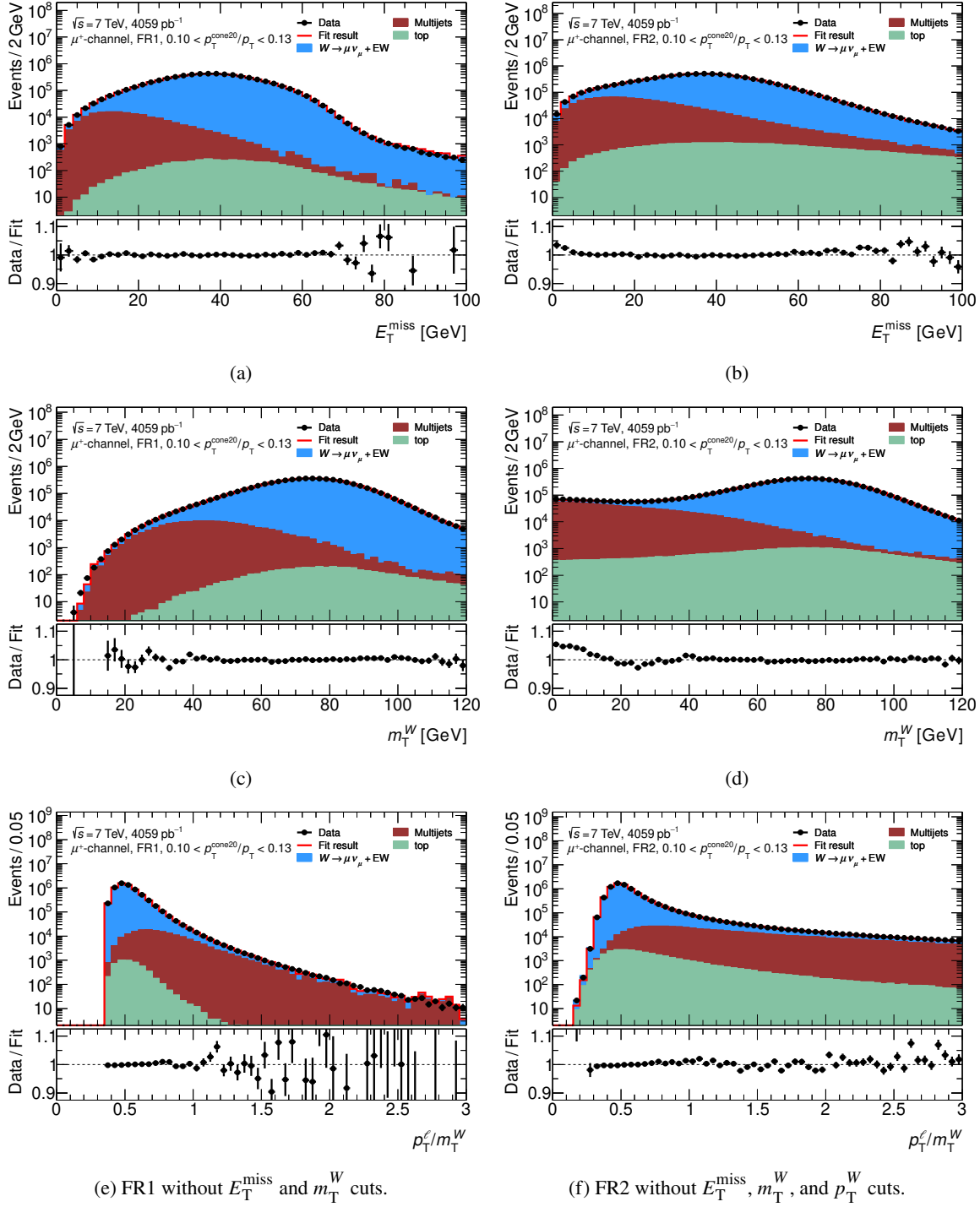
Figure 5.5: Example of multijet template fits of the observables E_T^{\text{miss}} , m_T^W , and p_T^{\ell}/m_T^W in FR1 (left) and FR2 (right) for the \mu^+ -channel. The multijet distribution is extracted from the first CR ( 0.10 < p_T^{\text{cone20}}/p_T < 0.13 ). The ratio shows the agreement between data and the template fits.
