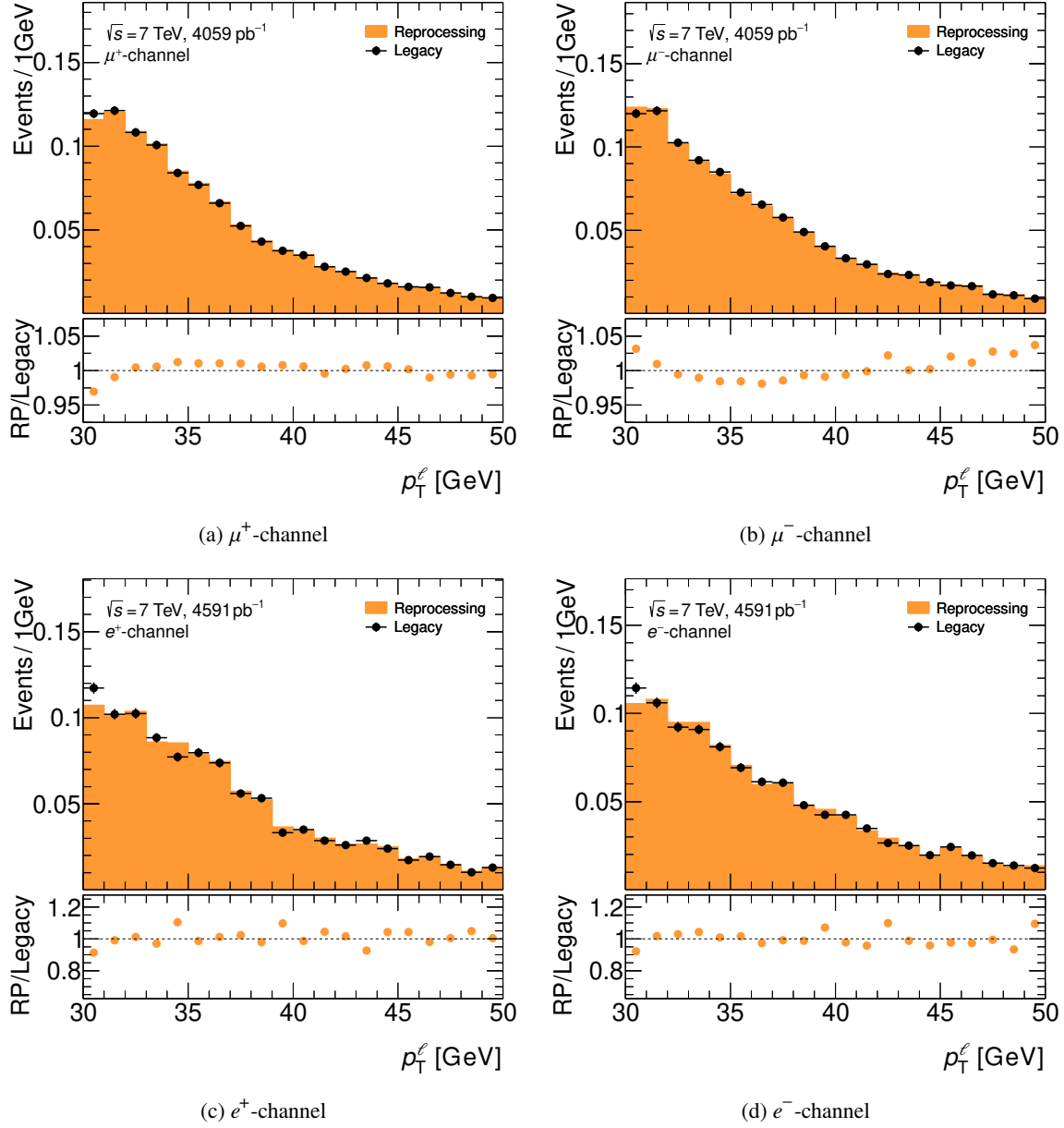
Figure 5.9: Comparison of the multijet background shape between the 2017 analysis and the reanalysis in the observable p_T^\ell . The agreement is shown for W^+ (a,c) and W^- (b,d) for the muon (a,b) and the electron channel (c,d).
