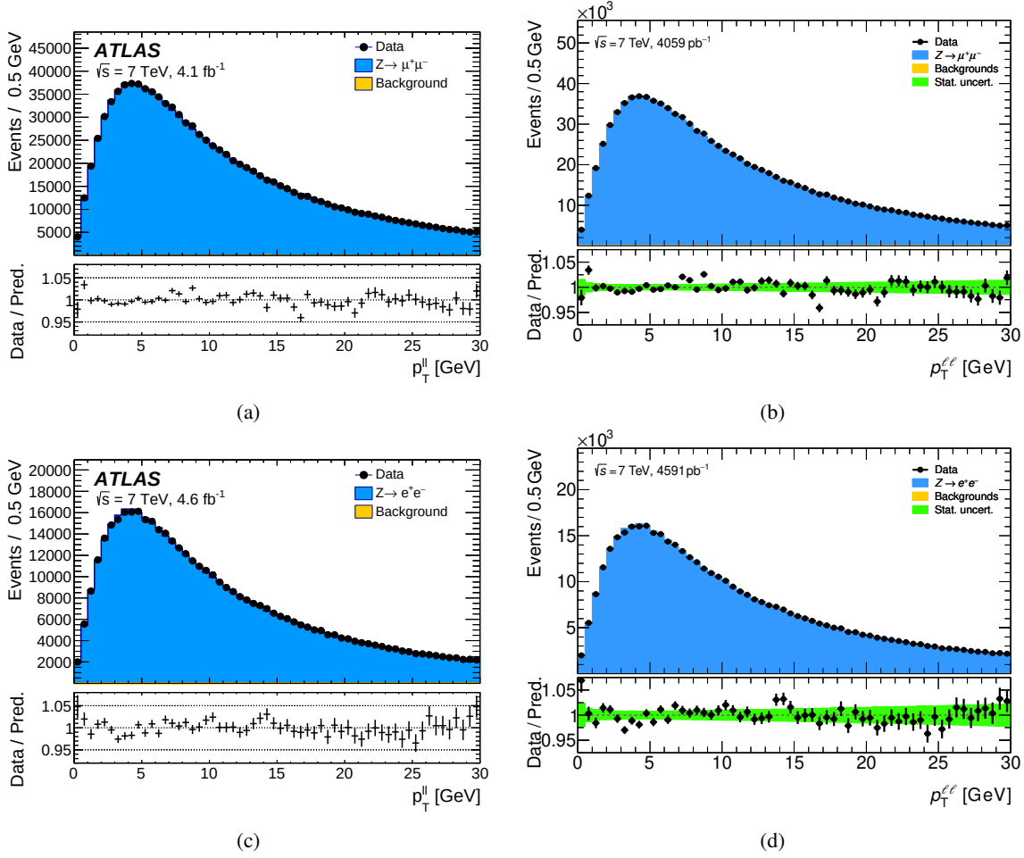
Figure 7.10: Comparison of the data to simulation agreement of the p_T^{\ell\ell} distributions from Z-boson events between the 2017 analysis (a,c) (taken from [86]) and the reanalysis (b,d). Shown are Z \rightarrow \mu\mu events (a,b) and Z \rightarrow ee events (c,d). The physics-modelling corrections and detector calibrations are applied to the simulation. The lower panel illustrates the data-to-prediction ratio with the error bars indicating the statistical uncertainties and the green band represents the uncertainty caused by the limited simulation sample size.
