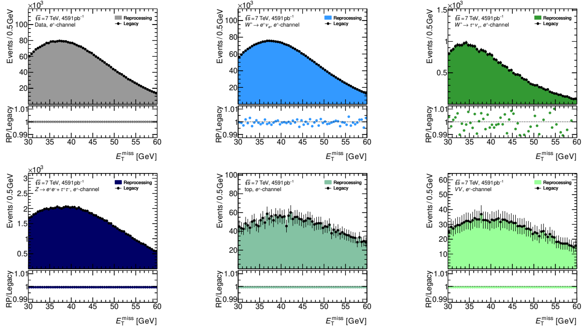
Figure C.15: Comparison between distributions published in the 2017 analysis (black dots) and the reprocessed samples (coloured filled areas) for electrons with charge q = +1 and the observable E_T^{\text{miss}} . Shown are the distributions of the data sample and the five MC samples.
