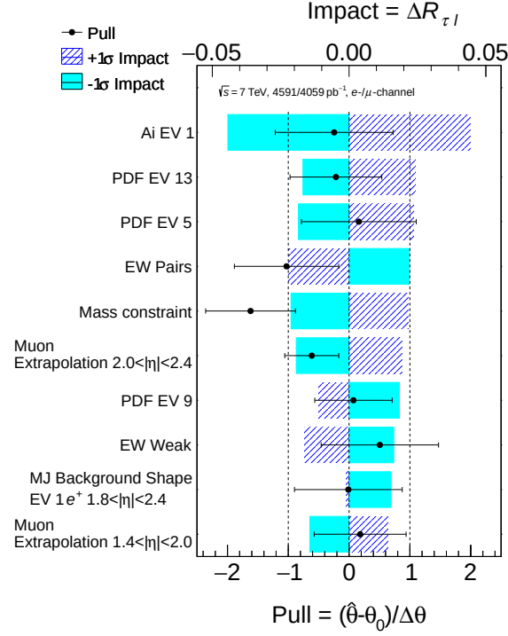
Figure 8.12: The ten NPs with the highest impact on the lepton universality measurement performed in the p_T^\ell distribution. Indicated are the +1\sigma and -1\sigma impacts, as well as the pull with its uncertainty.
