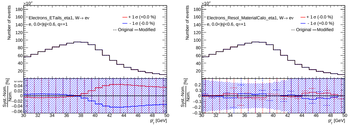
Figure F.4: Distributions of different systematic uncertainties of the electron channel comparing the original (dashed lines) and the modified (solid lines) envelopes. The lower panel illustrates the relative uncertainty compared to the nominal distribution given in per cent where the hatched area represents the statistical uncertainty of the nominal distribution.
