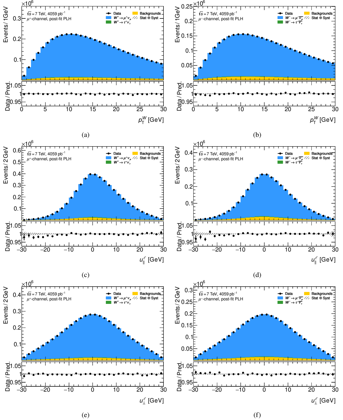
Figure F.10: Illustration of the post-fit recoil distribution in the muon channel for p_T^\ell fits of the W -boson mass. Shown are the distributions of p_T^W (a,b), u_{\parallel}^\ell (c,d), and u_{\perp}^\ell (e,f) for positively (a,c,e) and negatively (b,d,f) charged muons.
