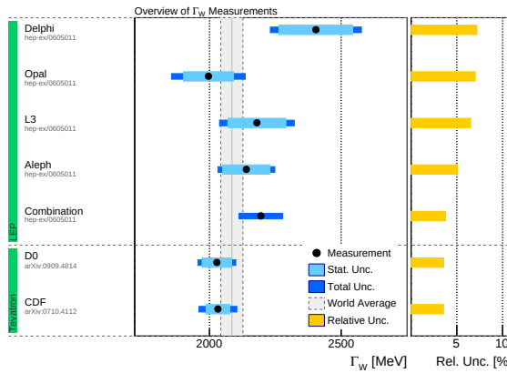
(a) Different \Gamma_W measurements.
