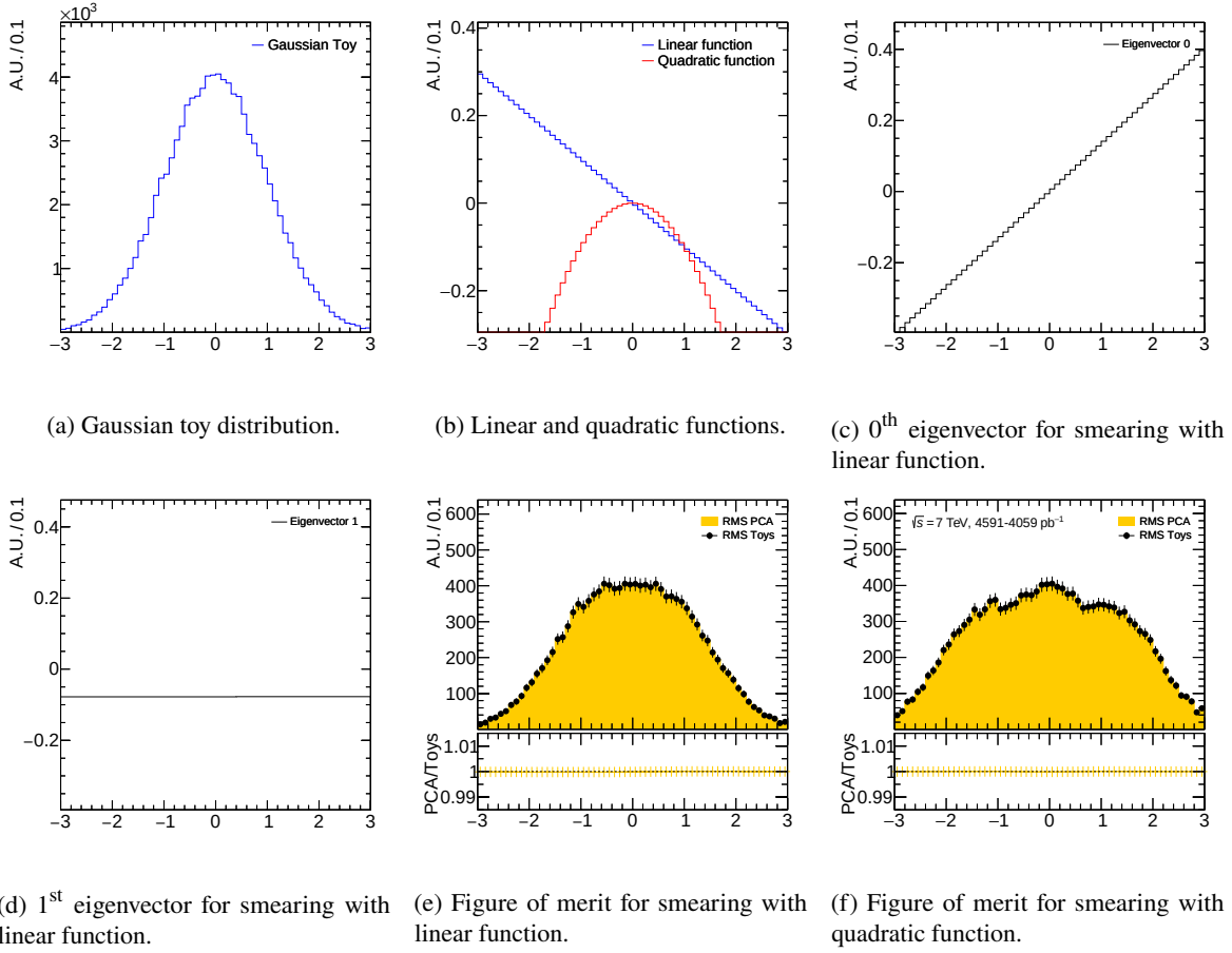
Figure E.8: Graphical illustration of the toy example for the PCA. (a) shows the gaussian toy distribution being the base and (b) the linear (blue) and the quadratic (red) function the base distribution is smeared with. The two eigenvectors originating from the smearing with the linear function are shown in (c) (0 th eigenvector) and (d) (1 st eigenvector). The figures of merit in (e) and (f) for the two different smearings compare the RMS of the toys (black points) to the RMS of the PCA eigenvectors (solid orange histogram) and their ratio indicates the closure between both quantities.
