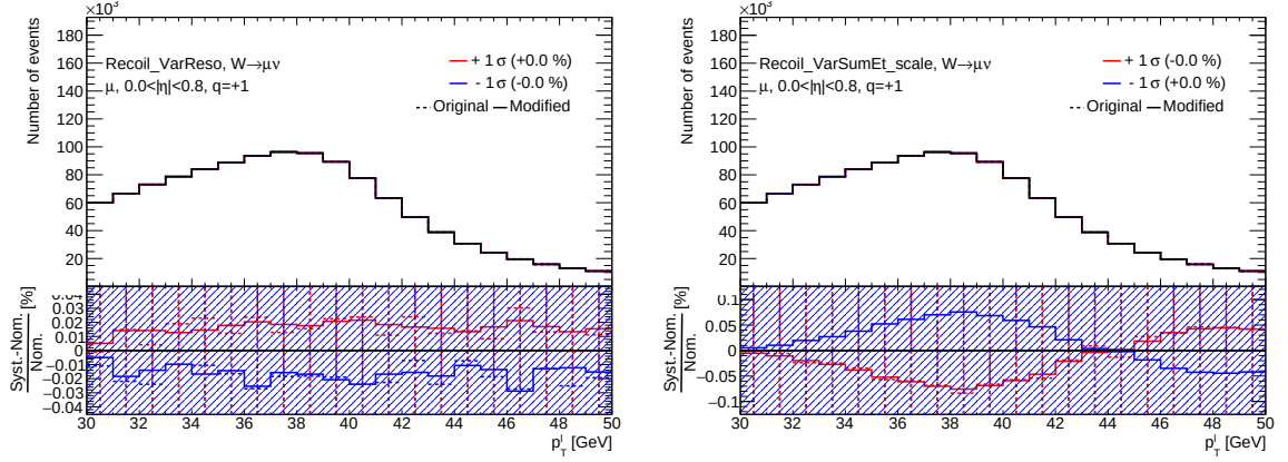
Figure F.3: Distributions of different systematic uncertainties of the muon channel comparing the original (dashed lines) and the modified (solid lines) envelopes. The lower panel illustrates the relative uncertainty compared to the nominal distribution given in per cent where the hatched area represents the statistical uncertainty of the nominal distribution.
