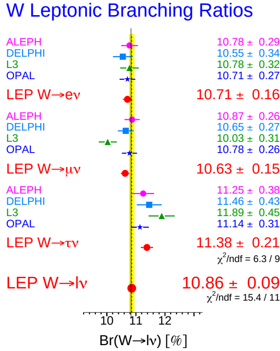
Figure 4.6: Leptonic branching ratios in the W decay. Shown are the results for the three lepton flavours for the individual experiments as well as their combination and the combination of all lepton families (taken from [120]).
