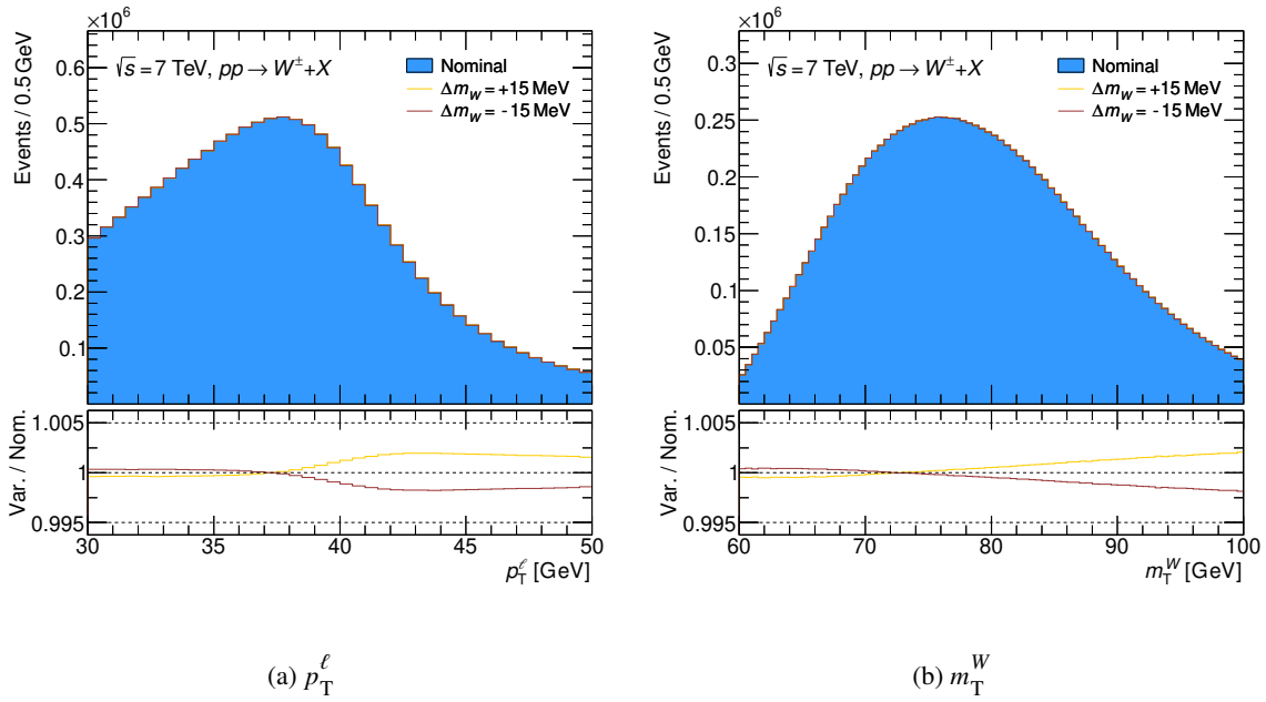
Figure B.1: Mass templates for the nominal hypothesis and two mass variations. Shown is the sum of all fitting categories of both processes initiated by a W -boson, W \rightarrow \ell \nu and W \rightarrow \tau \nu , for the kinematic distributions p_T^\ell (a) and m_T^W (b). The lower panel illustrates the ratio of the mass variations compared to the nominal mass template.
