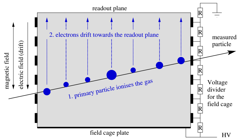
FIGURE 2.2: Schematic view of TPC principle [13].
