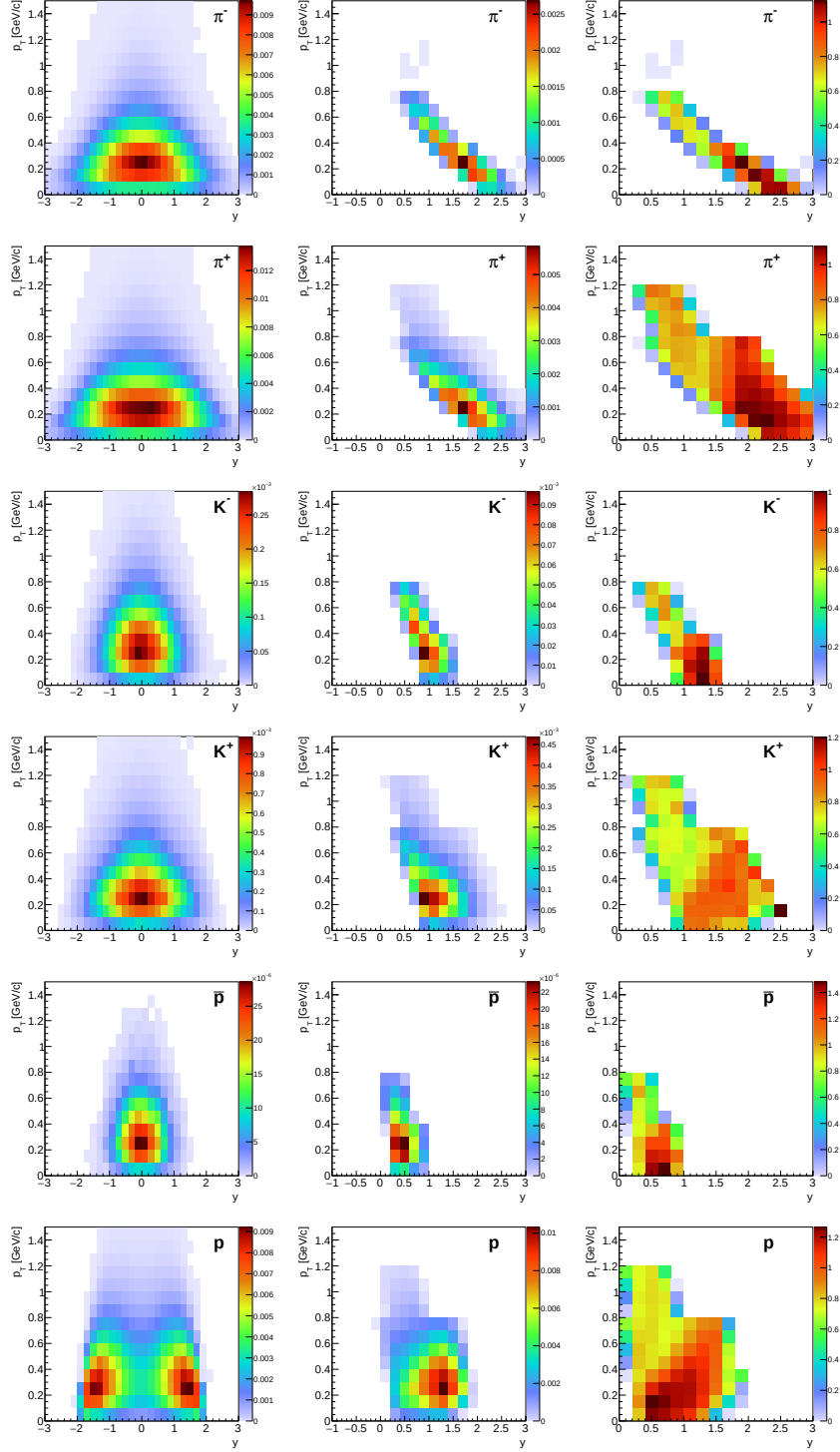
FIGURE 7.2: Example of generated Monte-Carlo particles spectra (left panels), spectra after selection criteria (middle panels) and correction factor (right panels) for p + p interactions at 30.9 GeV/c for positively and negatively charged pions, kaons and protons.
