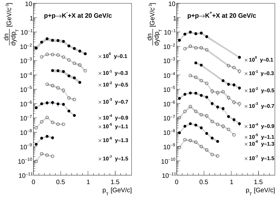
FIGURE 9.2: K^- and K^+ spectra produced in inelastic p + p collisions at 20 GeV/c beam momentum. Rapidity values on the figure correspond to the middle of the presented bin.
