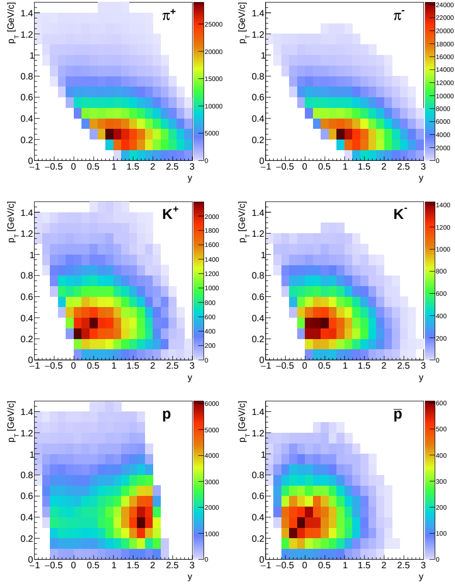
FIGURE 6.9: Yields of positively and negatively charged pions (top panel), kaons (middle panel) and protons (bottom panel) measured in p + p interaction at 158 GeV/c (not corrected).
