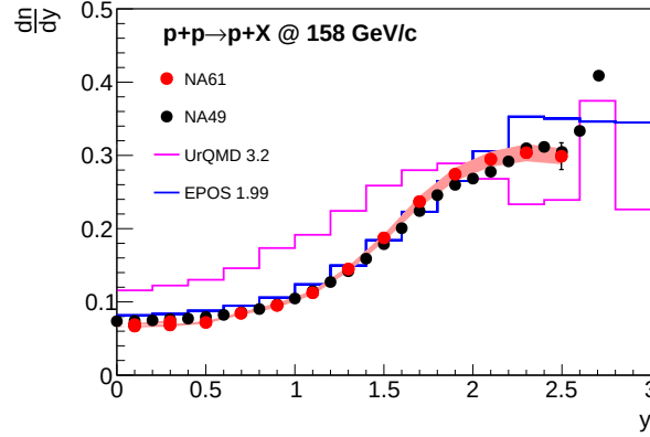
FIGURE 9.17: Proton rapidity distribution at 158 GeV/c compered with NA49 measurement and Monte-Carlo models.
