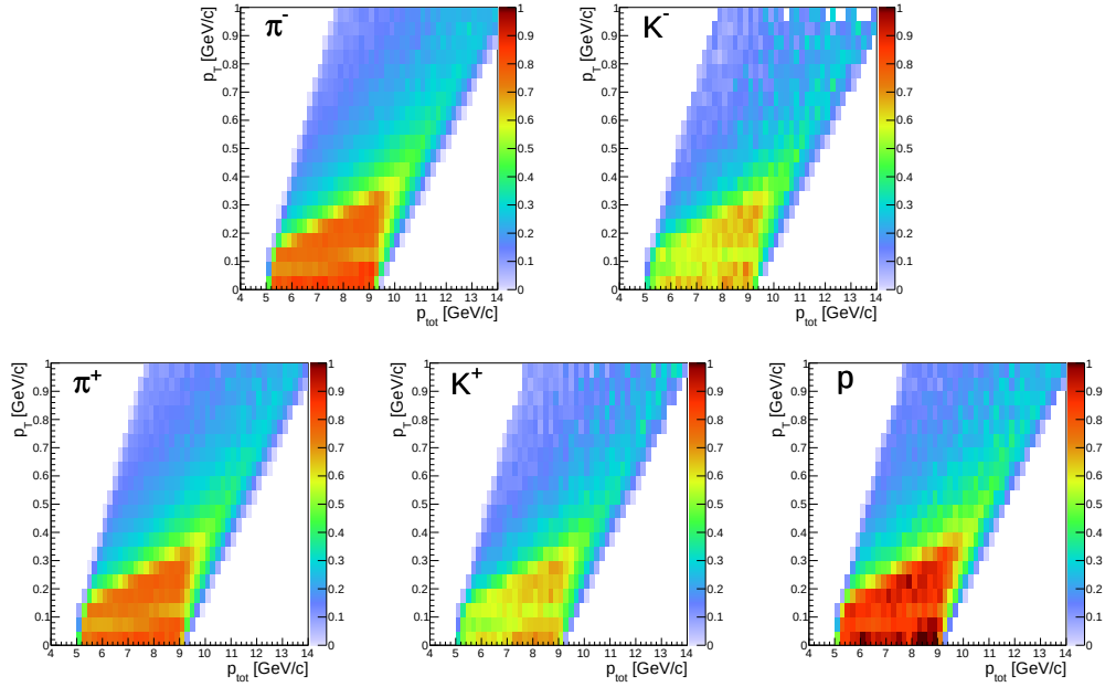
FIGURE 7.3: Correction for geometrical acceptance and decays before two last padrows of MTPC for p + p collisions at 158 \text{ GeV}/c .
