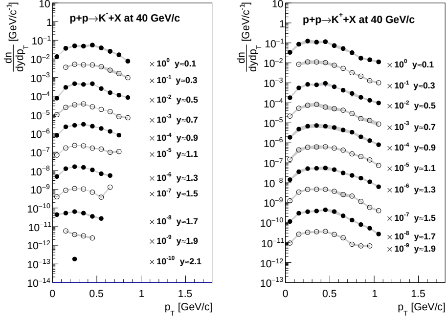
FIGURE 9.4: K^- and K^+ spectra produced in inelastic p + p collisions at 40 GeV/c beam momentum. Rapidity values on the figure correspond to the middle of the presented bin.
