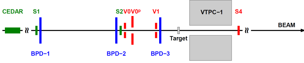
FIGURE 2.1: Schematic layout (horizontal cut in the beam plane, not to scale) of the beam detectors used in 2009 during p + p data taking periods.
