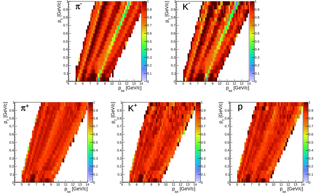
FIGURE 7.5: Monte-Carlo correction for not active pixels. Visible strips with lower value are due to groups of not working pixels.
