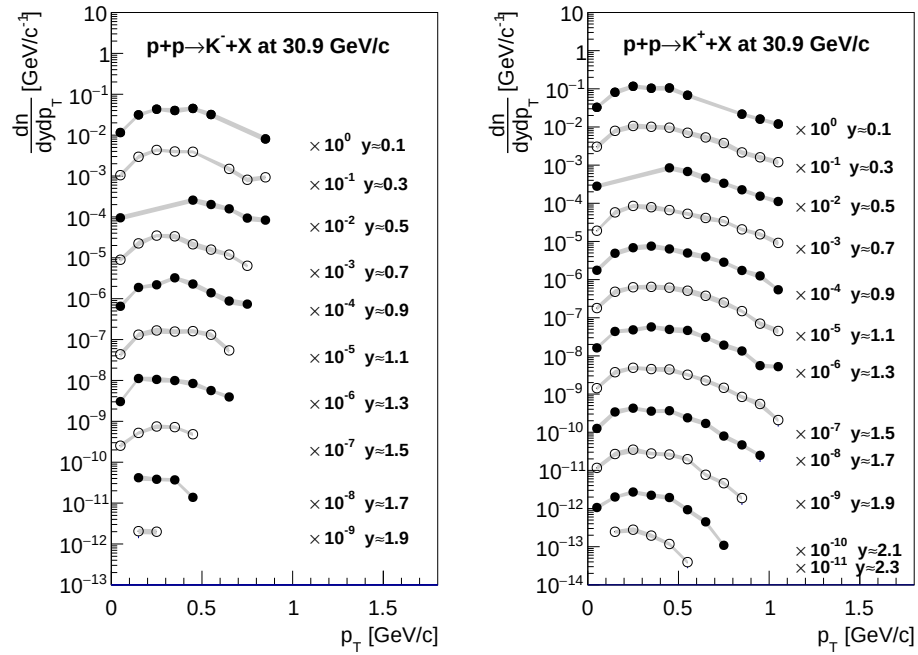
FIGURE 9.3: K^- and K^+ spectra produced in inelastic p + p collisions at 30.9 GeV/c beam momentum. Rapidity values on the figure correspond to the middle of the presented bin.
