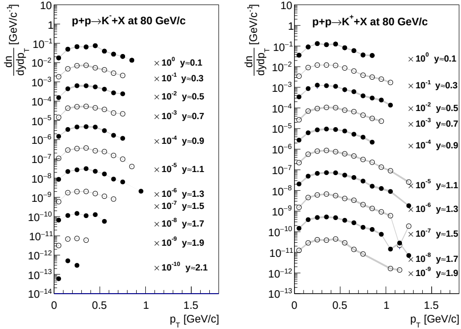
FIGURE 9.5: K^- and K^+ spectra produced in inelastic p + p collisions at 80 GeV/c beam momentum. Rapidity values on the figure correspond to the middle of the presented bin.
