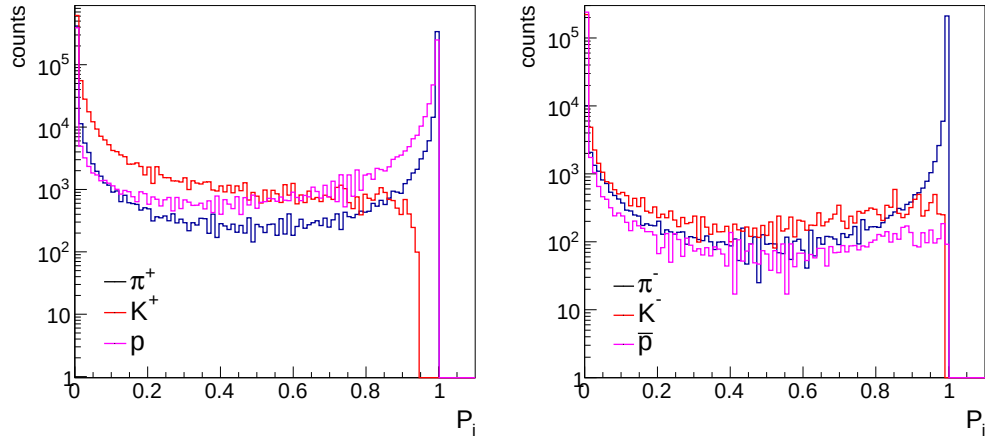
FIGURE 6.7: Probability of track identification as pion, kaon, proton for positively (left panel) and negatively (right panel) charged tracks from dE/dx measured in p + p interactions at 40 GeV/c .
