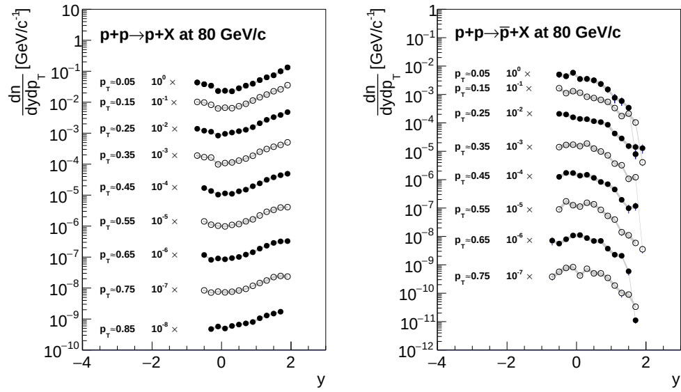
FIGURE 9.14: Double differential rapidity spectra of protons and anti-protons from p + p at 80 GeV/c for different transverse momentum intervals.
