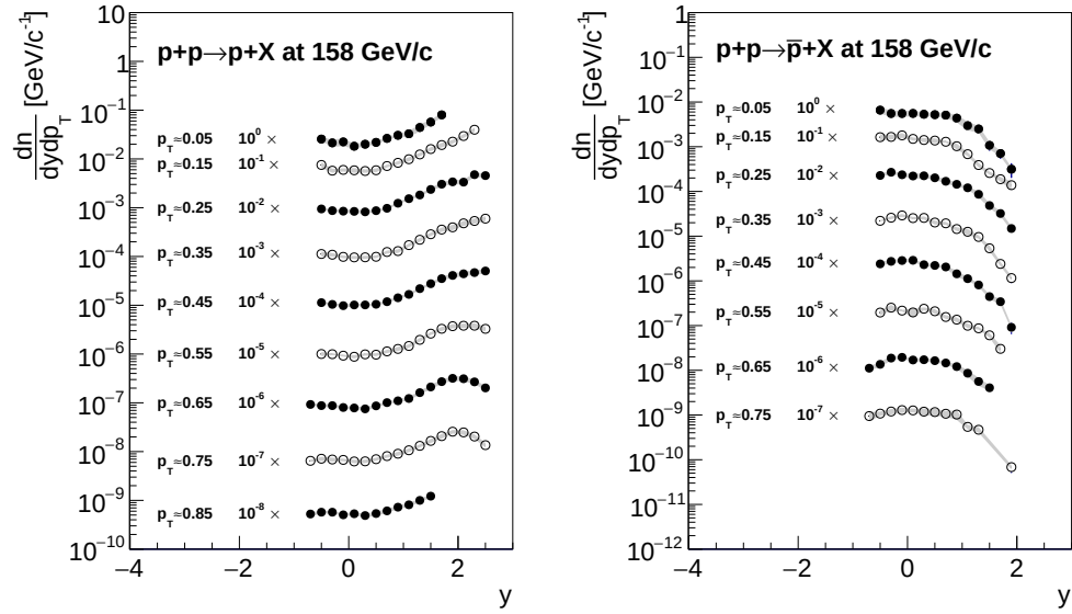
FIGURE 9.15: Double differential rapidity spectra of protons and anti-protons from p + p at 158 GeV/c for different transverse momentum intervals.
