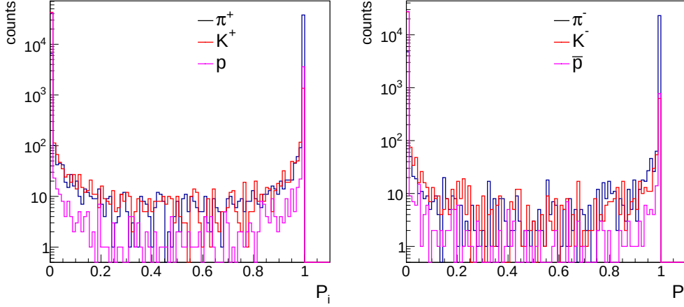
FIGURE 6.8: Probability of track identification as pion, kaon, proton for positively (left panel) and negatively (right panel) charged tracks from tof - dE/dx measured in p+p interactions at 158 GeV/c .
