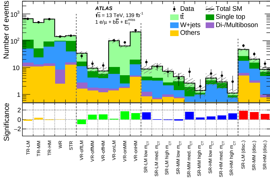
Figure 6.7: Plot showing the data/SM agreement in all CR/VR/SRs for the 139 \text{ fb}^{-1} SUSY Wh\ 1\ell + b\bar{b} + E_{\text{T}}^{\text{miss}} analysis. Good agreement is seen in all regions.
