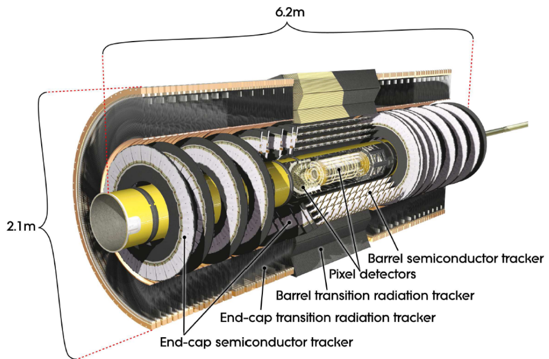
Figure 2.5: A cutaway diagram of the ATLAS inner detector showing its structure [6].
