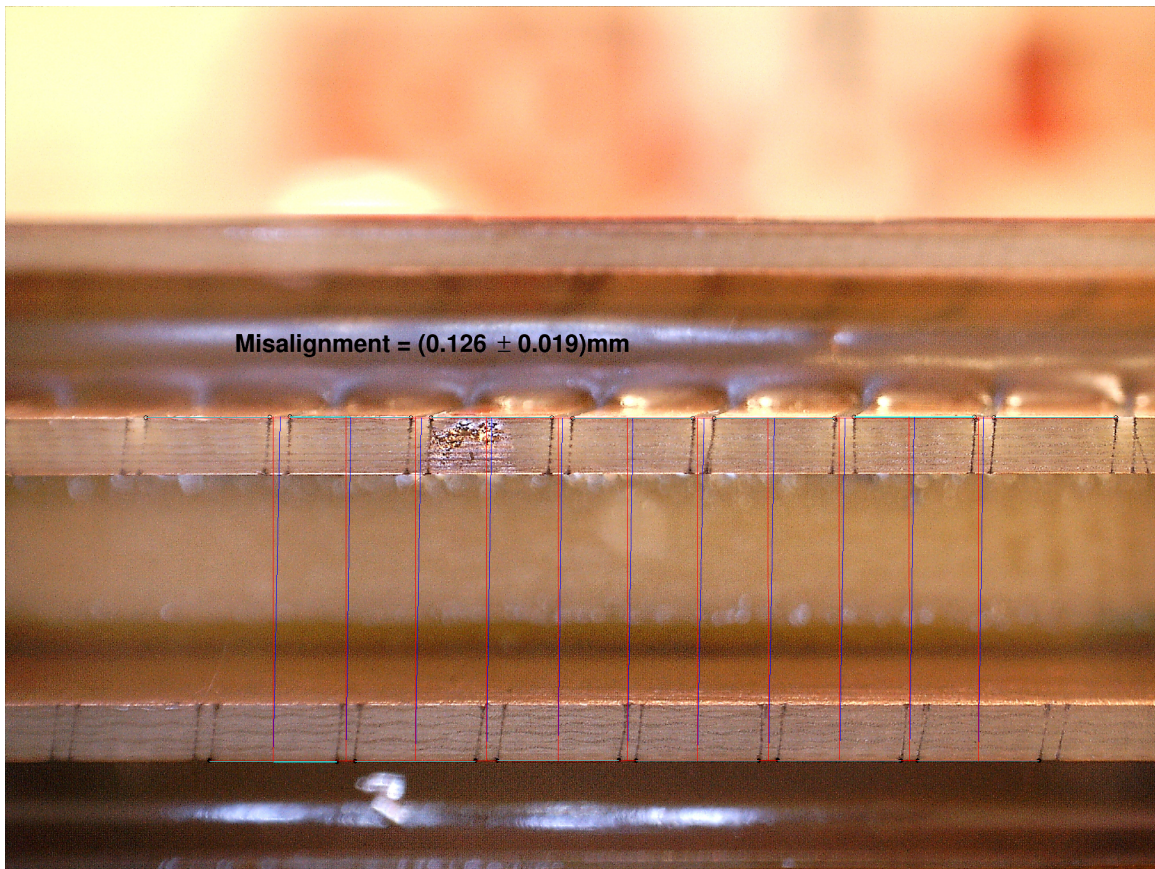
Figure 6.7: A sample microscope picture used to measure the misalignment on a QS3 doublet.
