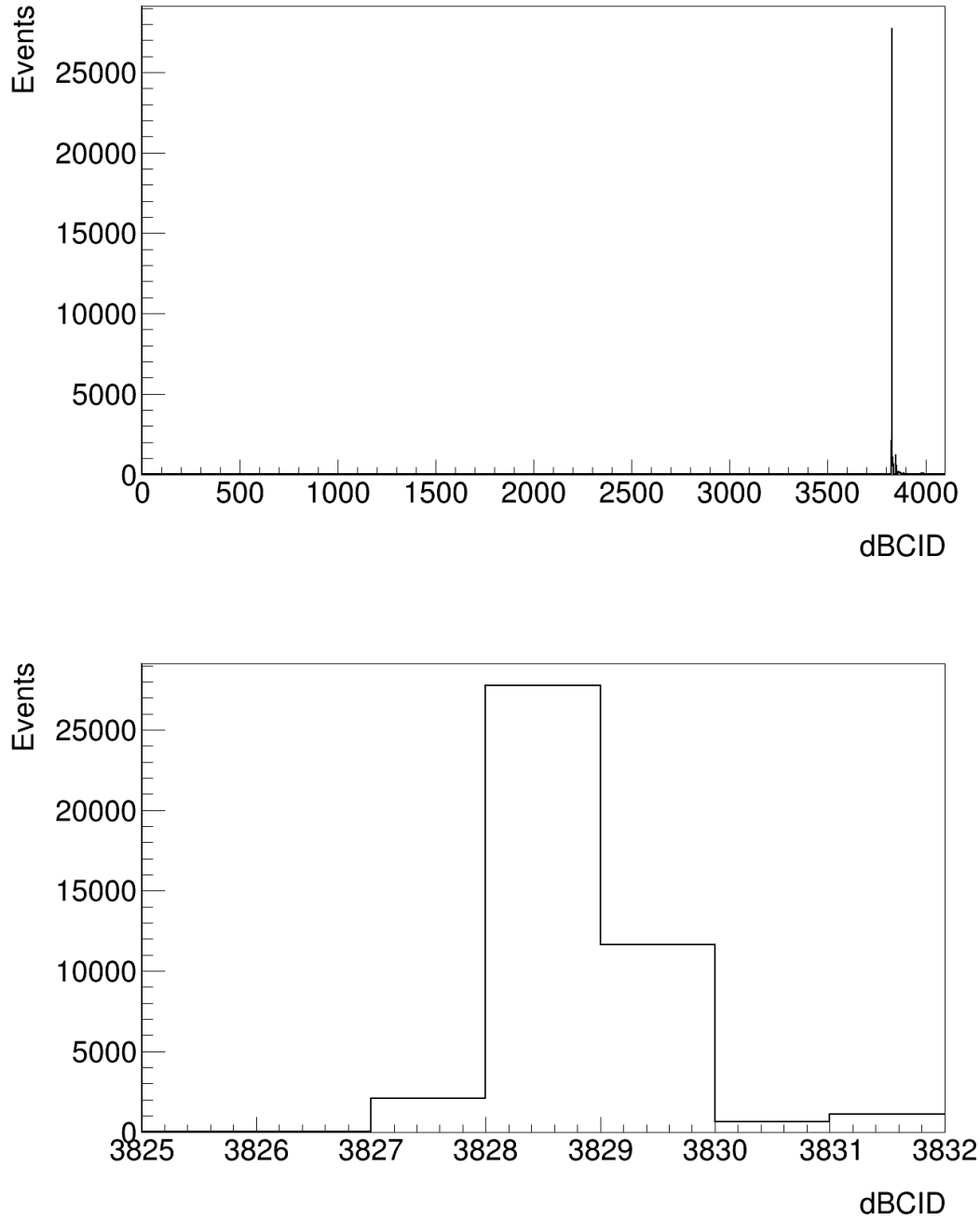
Figure 5.1: The top plot shows the distribution of the difference of the BCID of the pad signal and the BCID of the trigger time injection. The bottom plot shows a zoomed in view of the peak of the distribution.
