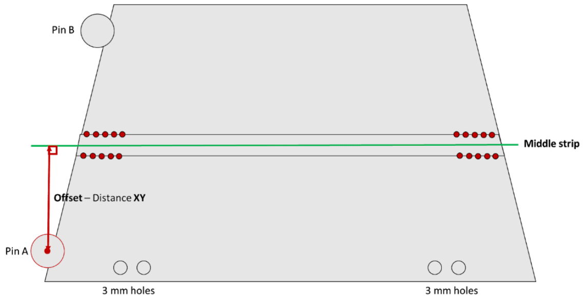
Figure 6.1: A diagram showing how the offset measurement was taken at Triangle Labs. A 24 board is depicted in this diagram, as the alignment features are on the left 3 .
