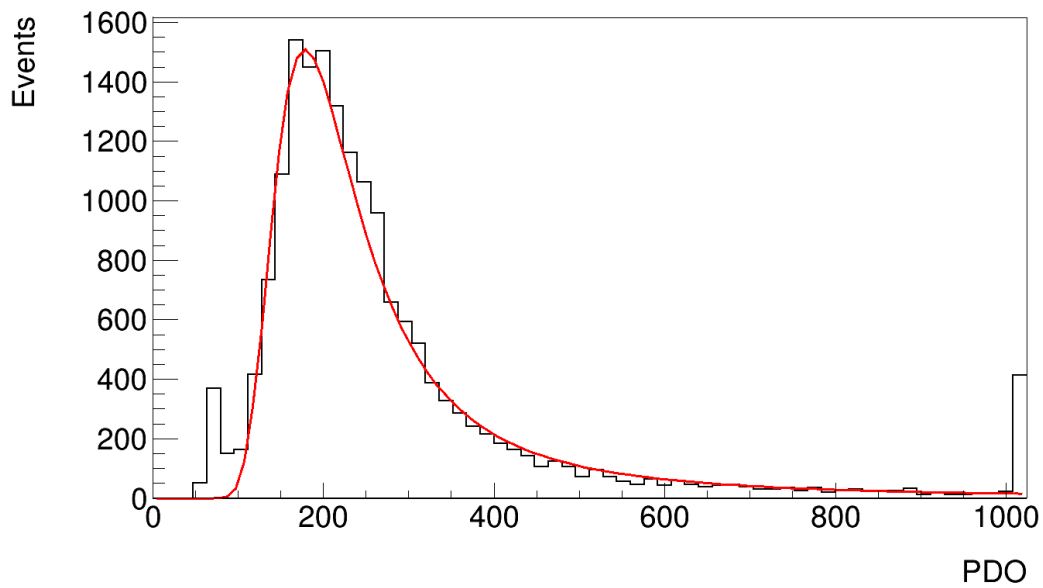
Figure 5.7: A plot demonstrating the two separate distributions of the beam constituents. The small peak on the left side of the distribution is a result of the beam impurities, where the secondary particles produce a secondary energy distribution.
