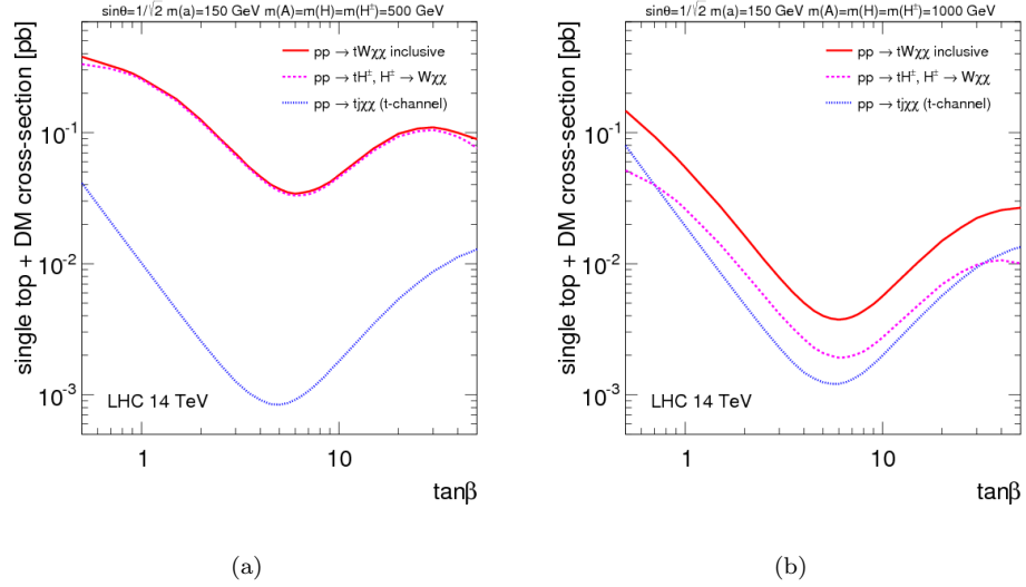
Figure 4.4: Cross-sections of the tW +DM and tj +DM signatures in the 2HDM+a model as a function of \tan\beta for \sin\theta = 1/\sqrt{2} , m_a = 150 GeV and (a) m_A = m_H = m_{H^\pm} = 500 GeV and (b) m_A = m_H = m_{H^\pm} = 1000 GeV [179]. The total tW +DM signature cross-section is indicated by the red solid line, the cross-section of the resonant diagram in Figure 4.1e is shown by the pink dashed line and the total cross-section of the tj +DM signature is shown by the blue dotted line. The cross-section calculation assumes a proton-proton collider with a centre-of-mass energy of 14 TeV.
