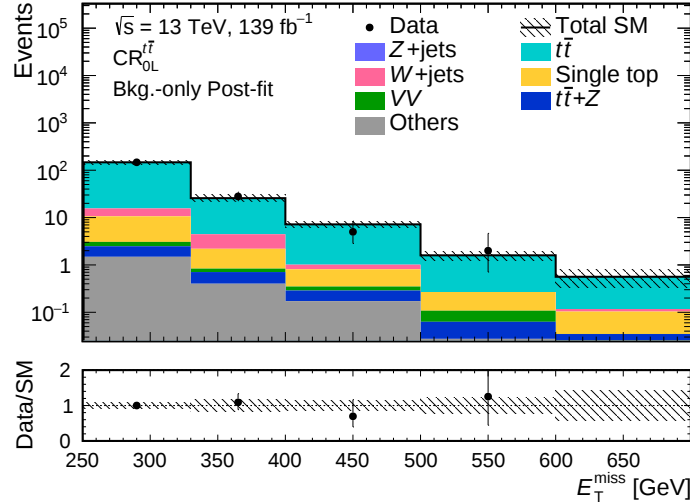
Figure 10.3: Distribution of the data and the SM background processes as a function of the E_T^{\text{miss}} in the \text{CR}_{0\text{L}}^{t\bar{t}} . The hashed uncertainty band includes all systematic uncertainty sources described in Section 10.3. The normalisation and nuisance parameters obtained from the background-only fit described in Section 8.4 are used for the SM predictions in the figure. Events beyond the range of the x -axis are added to the rightmost bin. The bottom panel shows the ratio of the data and the sum of all SM predictions in each bin. “Others” contains contributions from the triboson, tWZ , tZ , t\bar{t} + W , t\bar{t} + h , t\bar{t}t and t\bar{t}t\bar{t} processes.
