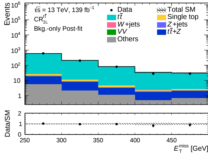
Figure 10.2: Distribution of the data and the SM background processes as a function of the E_T^{\text{miss}} in the \text{CR}_{1\text{L}}^{t\bar{t}} . The hashed uncertainty band includes all systematic uncertainty sources described in Section 10.3. The post-fit normalisation parameters of the SM processes and the post-fit systematic uncertainties obtained from the background-only fit described in Section 8.4 are used in the figure. Events beyond the range of the x -axis are added to the rightmost bin. The bottom panel shows the ratio of the data and the sum of all SM predictions in each bin. “Others” contains contributions from the triboson, tWZ , tZ , t\bar{t} + W , t\bar{t} + h , t\bar{t}t and t\bar{t}t\bar{t} processes.
