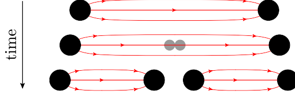
Figure 2.3: As the distance between two coloured particles increases, the force does, too and eventually leads to the production of additional coloured particles. Figure modified from Reference [25].
