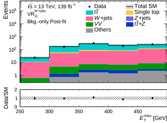
Figure 10.11: Distribution of the data and the SM background processes as a function of the E_T^{miss} in the VR_{1L}^{W+jets} . The hashed uncertainty band includes all systematic uncertainty sources described in Section 10.3. The post-fit normalisation of the SM processes and the post-fit systematic uncertainties obtained from the background-only fit described in Section 8.4 are used in the figure. Events beyond the range of the x -axis are added to the rightmost bin. The bottom panel shows the ratio of the data and the sum of all SM predictions in each bin. “Others” contains contributions from the triboson, tWZ , tZ , t\bar{t} + W , t\bar{t} + h , t\bar{t}t and t\bar{t}t\bar{t} processes.
