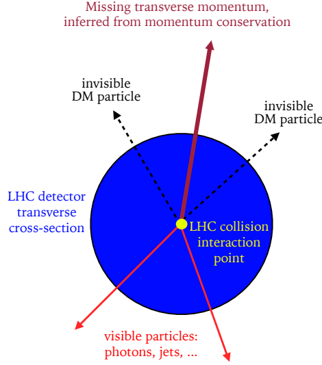
Figure 3.10: The DM particles do not produce a visible signature in the detector, leading to a non-zero sum of measured momenta in the plane transverse to the beam axis [142].
