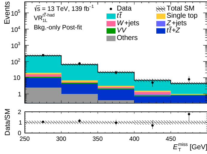
Figure 10.10: Distribution of the data and the SM background processes as a function of the E_T^{miss} in the VR_{1L}^{t\bar{t}-had} . The hashed uncertainty band includes all systematic uncertainty sources described in Section 10.3. The post-fit normalisation of the SM processes and the post-fit systematic uncertainties obtained from the background-only fit described in Section 8.4 are used in the figure. Events beyond the range of the x -axis are added to the rightmost bin. The bottom panel shows the ratio of the data and the sum of all SM predictions in each bin. “Others” contains contributions from the triboson, tWZ , tZ , t\bar{t} + W , t\bar{t} + h , t\bar{t}t and t\bar{t}t\bar{t} processes.
