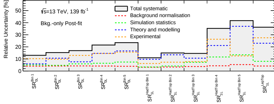
Figure 10.16: The total systematic uncertainty relative to the total SM prediction (solid black) in all SRs and their bins. The dashed lines indicate the size of the normalisation, simulation statistical, modelling and experimental uncertainties. As these systematic uncertainty components may be correlated, their quadratic sum may not agree with the square of the total systematic uncertainty. The systematic uncertainties shown are obtained from the background-only fit using the likelihood combining the 1L and 0L channels.
