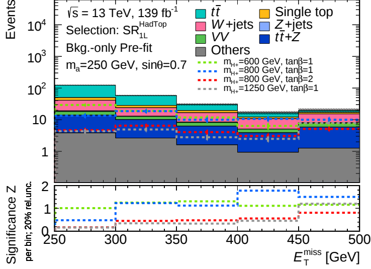
Figure 9.9: E_T^{\text{miss}} distribution in the \text{SR}_{1\text{L}}^{\text{HadTop}} . Background events are indicated by filled bars, which are stacked, while signal events for different 2HDM+ a model parameters are indicated by coloured, dashed lines. The significance is calculated per bin with Equation (9.1) using the yields in that bin. Only statistical uncertainties are shown. The normalisation of the simulated background samples has not been corrected by the background-only fit. “Others” contains contributions from the t\bar{t} + h , t\bar{t} + W , t\bar{t}Z and tWZ processes. Events beyond the range of the x -axis are added to the rightmost bin.
