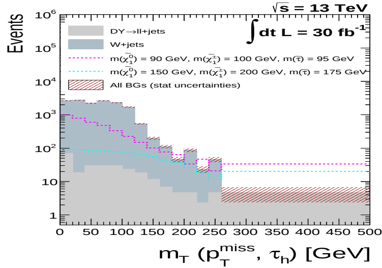
Figure 6.8: m_T(\tau_h, p_T^{\text{miss}}) distribution for the main backgrounds and two chosen signal points. This distribution is presented after all selections.
