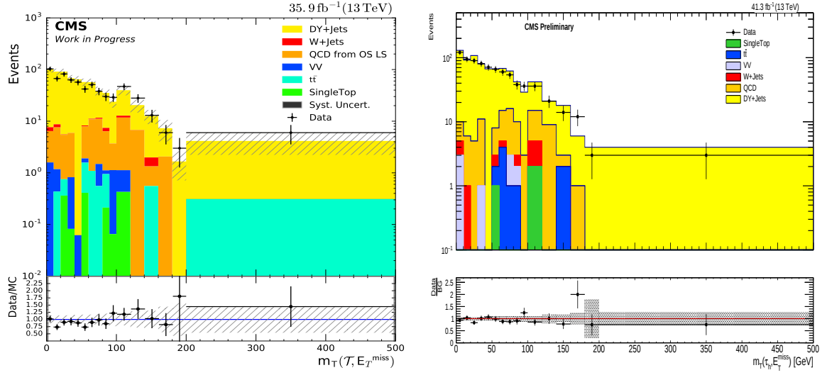
Figure 7.25: m_T(\tau_h, p_T^{\text{miss}}) distribution in the Z(\rightarrow \tau\tau)+\text{ISR} control region for 2016 (left) and 2017 (right) datasets.
