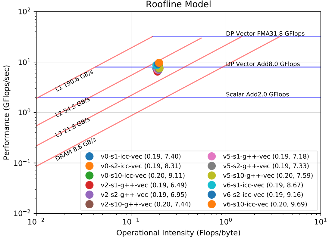
FIGURE 4.13: Roofline model applied in the kick() benchmark. The best performing variation (v6-s10-icc-vec) is bounded by L2 cache bandwidth. To break through this ceiling, we need to fit the entire data-set in the L1 cache.
