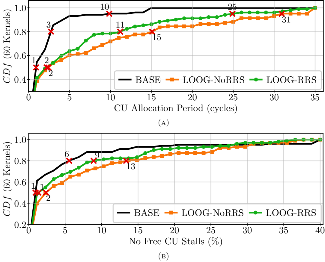
FIGURE 10.2: Cumulative Distribution Function of 60 GPU kernels of the CU allocation period (top), and pipeline stalls due to no available CU (bottom). The lines correspond to the baseline, LOOG without RRS, and LOOG with RRS architectures.
