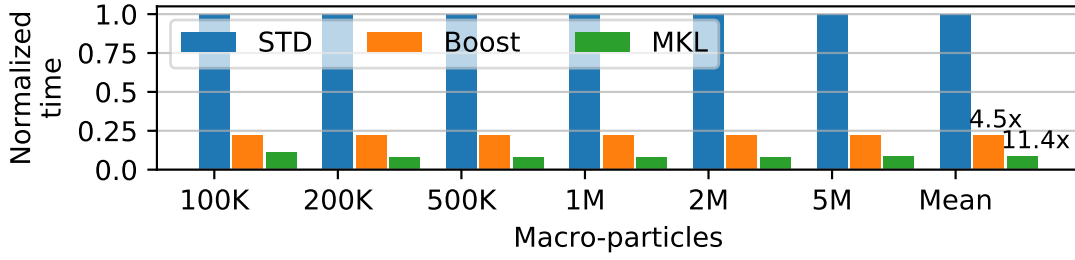
FIGURE 4.11: Benchmarking the STD, Boost and MKL libraries for the PRNG methods in the SR() function. The MKL PRNG method is on average 11.4× faster than the STD counterpart.
