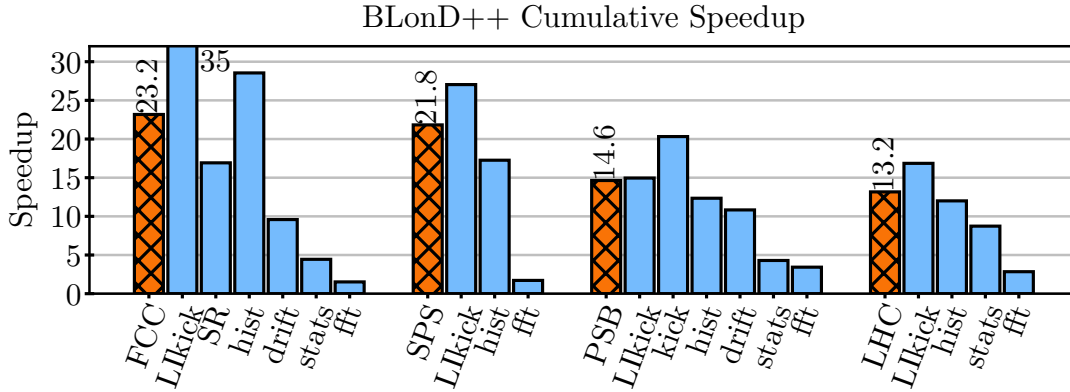
FIGURE 4.15: Single-core cumulative speedup of BLonD++ over the initial BLonD version. BLonD++ demonstrates a 18× speedup on average.
