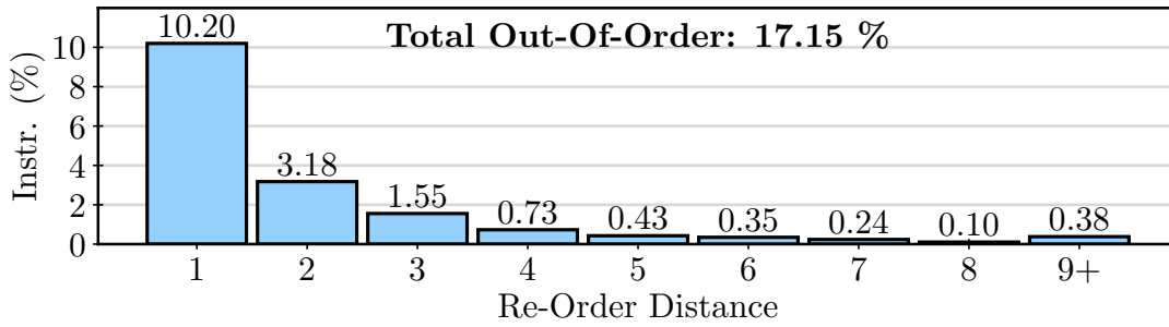
FIGURE 11.10: Percentage of instructions that dispatched OOO and their distance from the instruction in program order.
