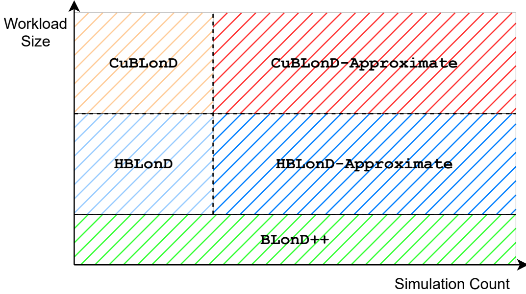
FIGURE 1.4: The three versions of BLongD developed in the scope of this thesis, and their recommended usage region.
