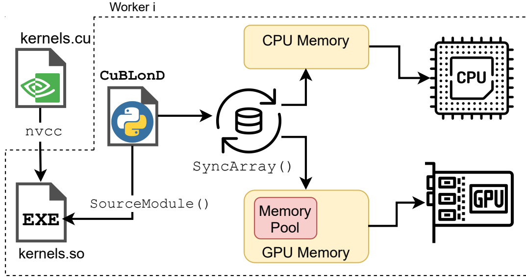
FIGURE 6.1: High-level software architecture of the GPU-accelerated BLongD code, CuBLonD .
