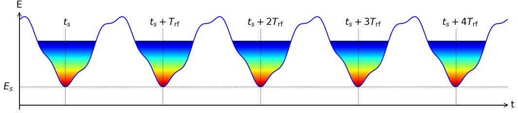
FIGURE 3.1: Example of a periodic potential well in a synchrotron, for several RF systems. In the absence of intensity effects, the synchronous point (t_s, E_s) is periodic with T_{\text{rf}} along the ring. The beam particles fill part of the potential well.
