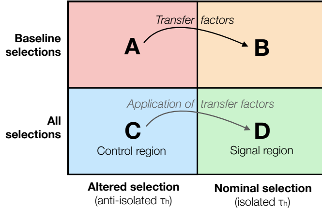
Figure 12.5: Illustration of the ABCD method: Transfer factors derived using events in regions A and B are used to normalize the background shape obtained from the control region C to the signal region D.
