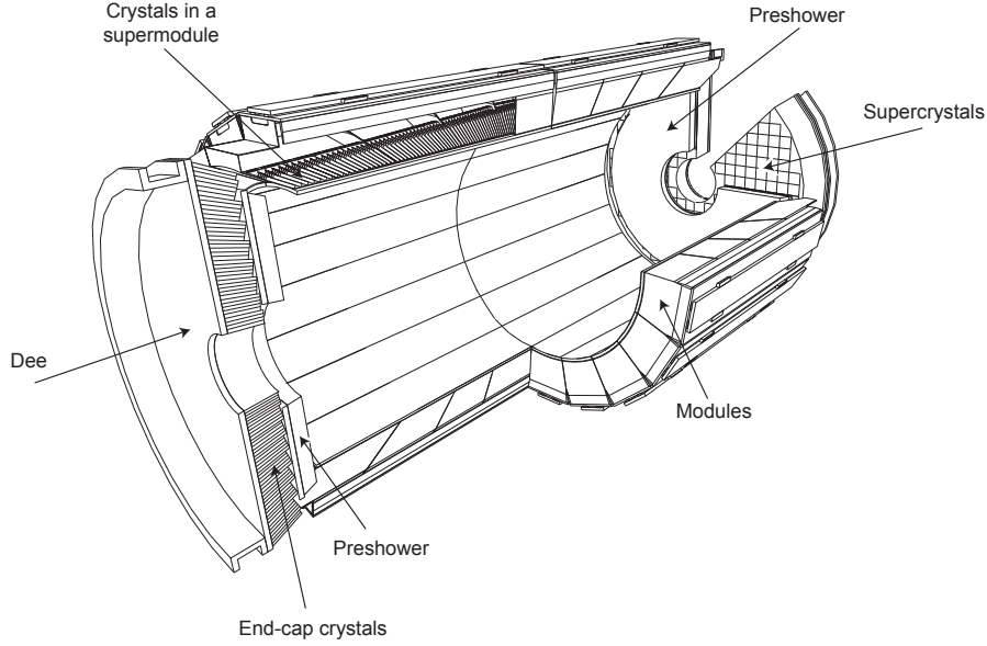
Figure 5.5: Illustration of the structure of the ECAL. The \text{PbWO}_4 crystals are grouped into modules and supermodules in the barrel, and into supercrystals in the endcaps. The preshower detectors provide additional sensitivity in the endcaps. [111]
