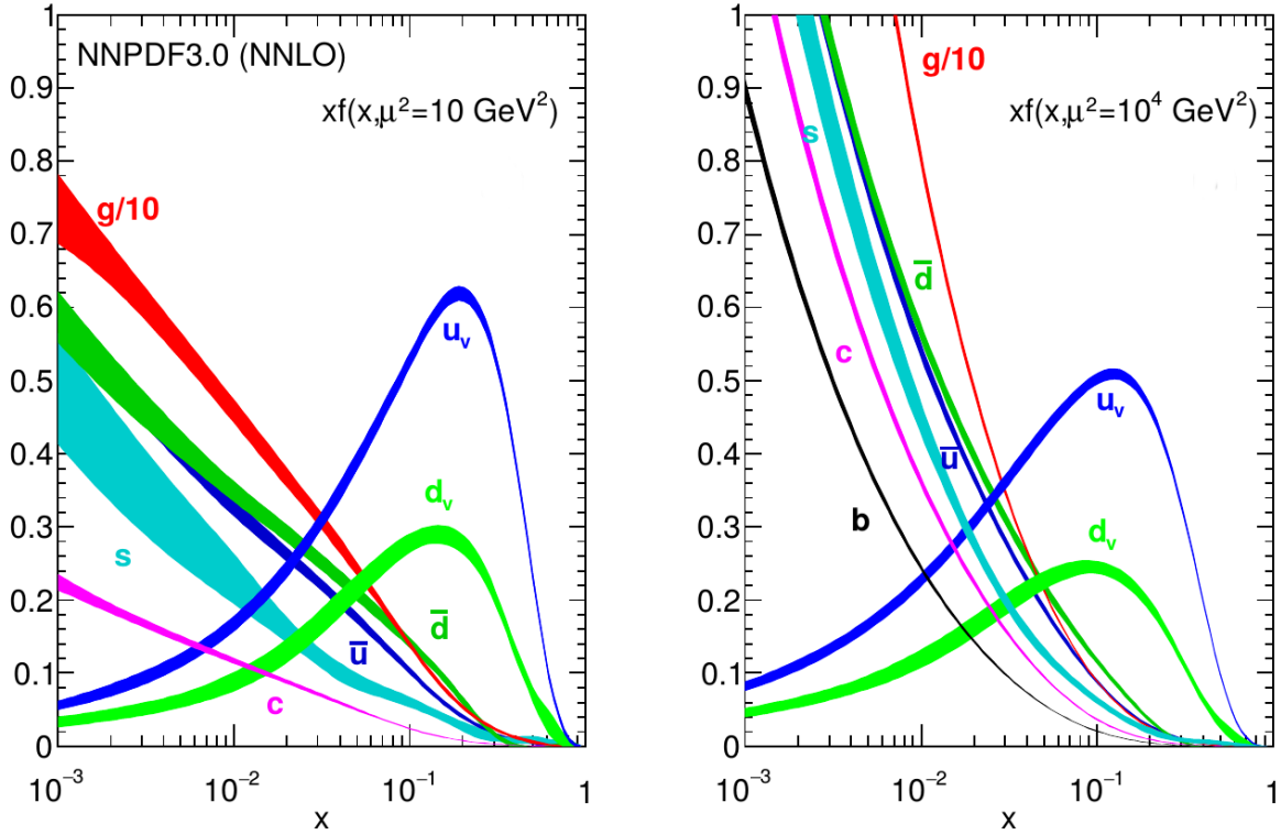
Figure 7.2: Examples of NNPDF3.0 parton distribution functions, shown as a function of x at low momentum transfer of 10 \text{ GeV}^2 (left) and at high momentum transfer of 10^4 \text{ GeV}^2 (right), with \alpha_s(M_Z^2) set to 0.118. [149]
