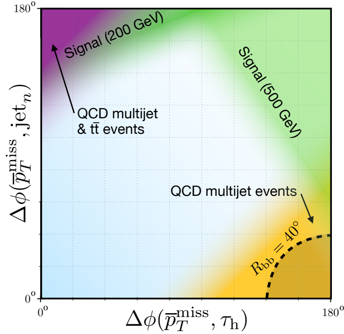
Figure 11.3: A schematic picture of the (\Delta\phi(\tau_h, \vec{p}_T^{\text{miss}}), \Delta\phi(\text{jet}, \vec{p}_T^{\text{miss}})) plane used in the R_{\text{bb}}^{\text{min}} selection. The selection affects the bottom-right corner of the plane, containing mostly QCD multijet events. Also the regions populated with signal events (using m_{H^\pm} = 200 \text{ GeV} and 500 \text{ GeV} as examples) and with the irreducible t\bar{t} background are shown for illustration.
