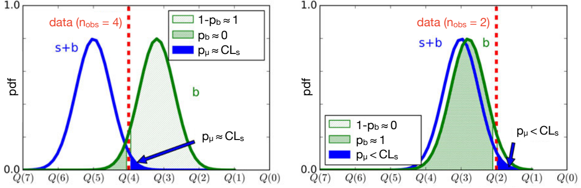
Figure 9.1: Illustration of \text{CL}_s and the probabilities p_\mu and p_b in a case of a simple cut-and-count experiment, with signal hypotheses predicting a large signal yield (left) and a small yield (right). The probability density functions f(\tilde{q}_\mu|\mu = \mu_{\text{hyp}}) ("s+b") and f(\tilde{q}_\mu|\mu = 0) ("b") are shown as a function of the test statistic value. Q(n_{\text{obs}}) denotes the value of the test statistic \tilde{q}_\mu when n_{\text{obs}} events are observed in data. The dashed vertical line represents the event yield observed in data. [180]
