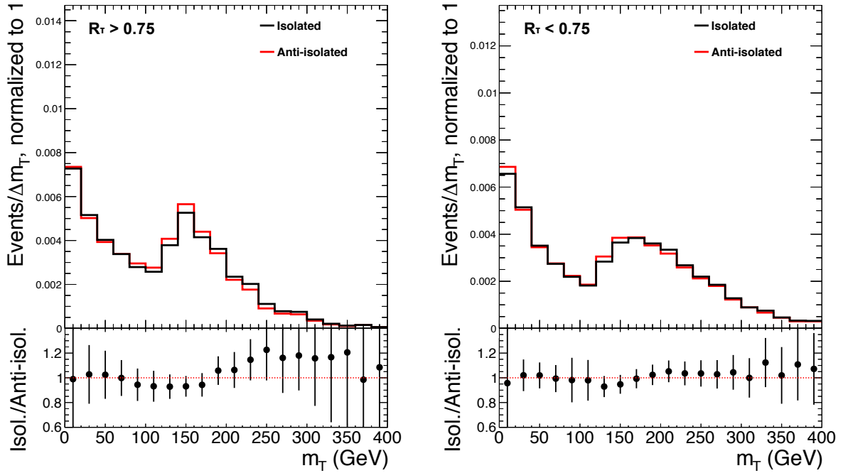
Figure 12.7: Comparison of \text{jet} \rightarrow \tau_h transverse mass distributions between events with \tau_h candidates that pass the isolation requirements ("Isolated"), and events with \tau_h candidates that fail them ("Anti-isolated"), in the R_\tau > 0.75 category (left) and R_\tau < 0.75 category (right). To suppress possible signal contamination, a veto on b-tagged jets is applied, contrary to the signal selection. The ratio of the two normalized shapes is also shown, together with statistical uncertainties propagated to the ratio. In both categories, the shapes agree within their statistical uncertainties.
