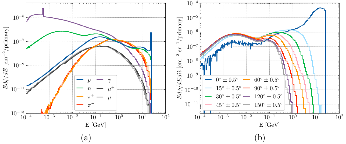
Figure 2.8: Monte Carlo simulation with the FLUKA code of the fluence energy spectra of particles emitted from a 50 cm copper target hit by 24 GeV/c proton beam: (a) fluences integrated over the whole solid angle; (b) double differential neutron fluence at selected angles with respect to the beam direction.
