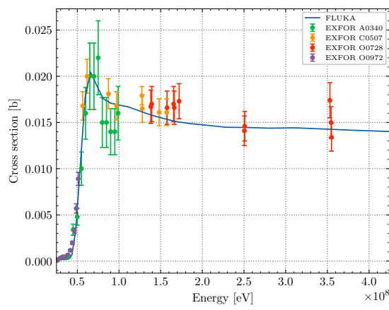
(c) ^{\text{nat}}\text{Si}(p, x)^{22}\text{Na}
