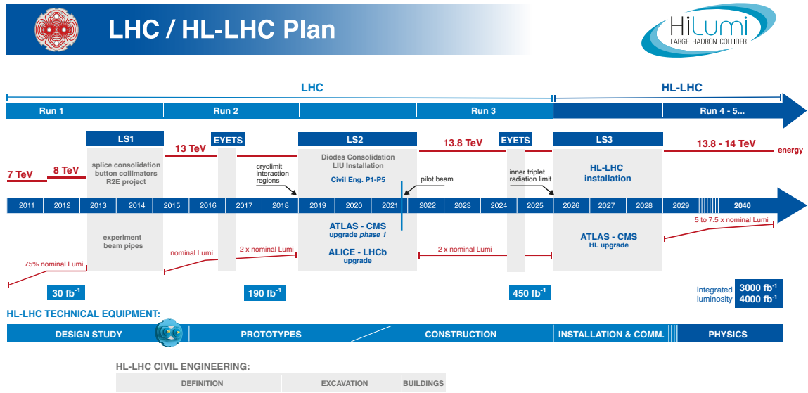
Figure 1.2: Current LHC baseline plan for the next decade and beyond, showing the collision energy (upper line) and luminosity (lower line) [5].
