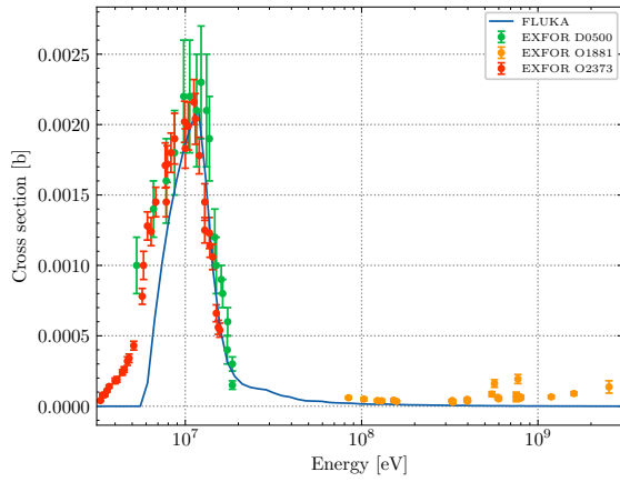
(e) ^{\text{nat}}\text{Fe}(p, x)^{58}\text{Co}
