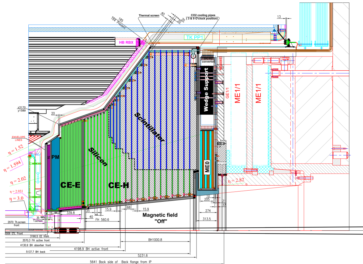
Figure 1.8: Longitudinal cross section of the upper half of the CMS High Granularity Calorimeter [27].
