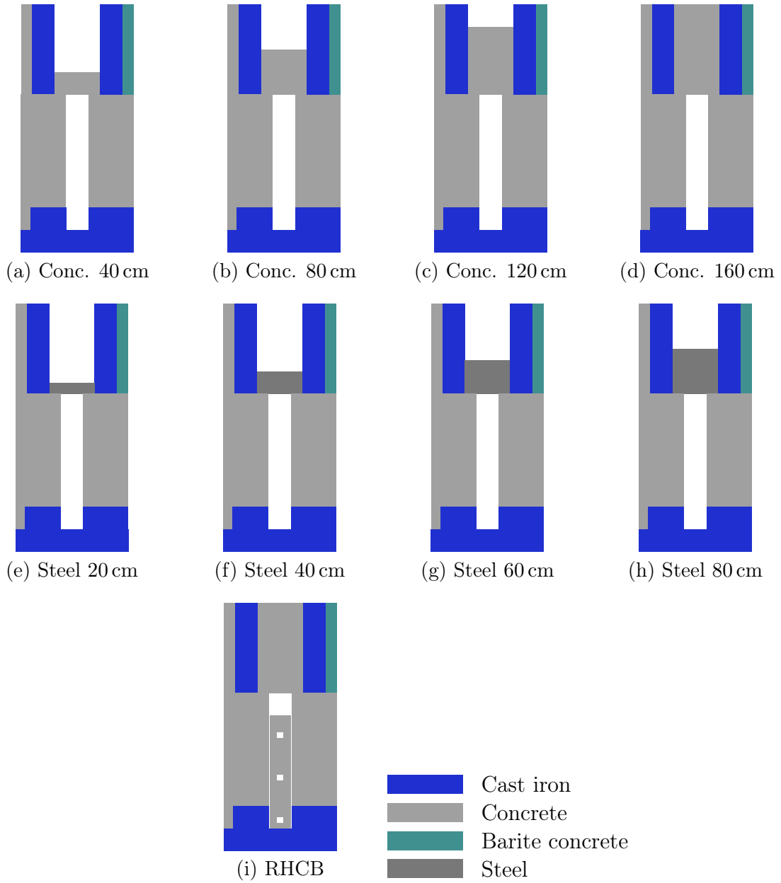
Figure 5.5: Summary of the various CSBF shielding configurations for the activation experiments with C, Al, In, and Bi samples: for the configurations (a) to (h) the samples are installed at the bottom and on top of the shielding block in the material test location; for the configuration (i) the samples are installed in the holes of the concrete bar and on top of it.
