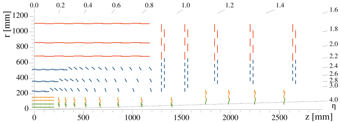
Figure 1.7: Schematic drawing of one quarter of the Phase II CMS Tracker. Each coloured line corresponds to a sensor layer: green and yellow lines correspond to Inner Tracker modules with respectively two and four readout chips, double blue and double red lines represent PS and 2S Outer Tracker modules [26].
