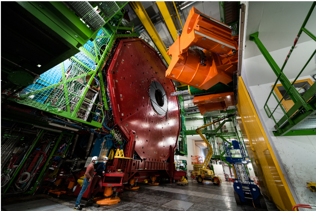
(b) CMS forward shield installed at present (in orange) during the full opening procedure [113].
