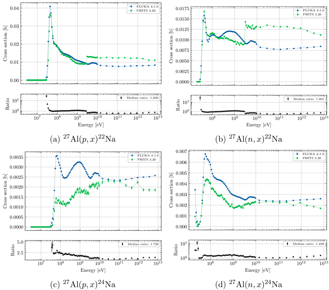
Figure A.2: Comparison of radionuclide production data computed with FLUKA and PHITS for selected elements and relevant radionuclides.
