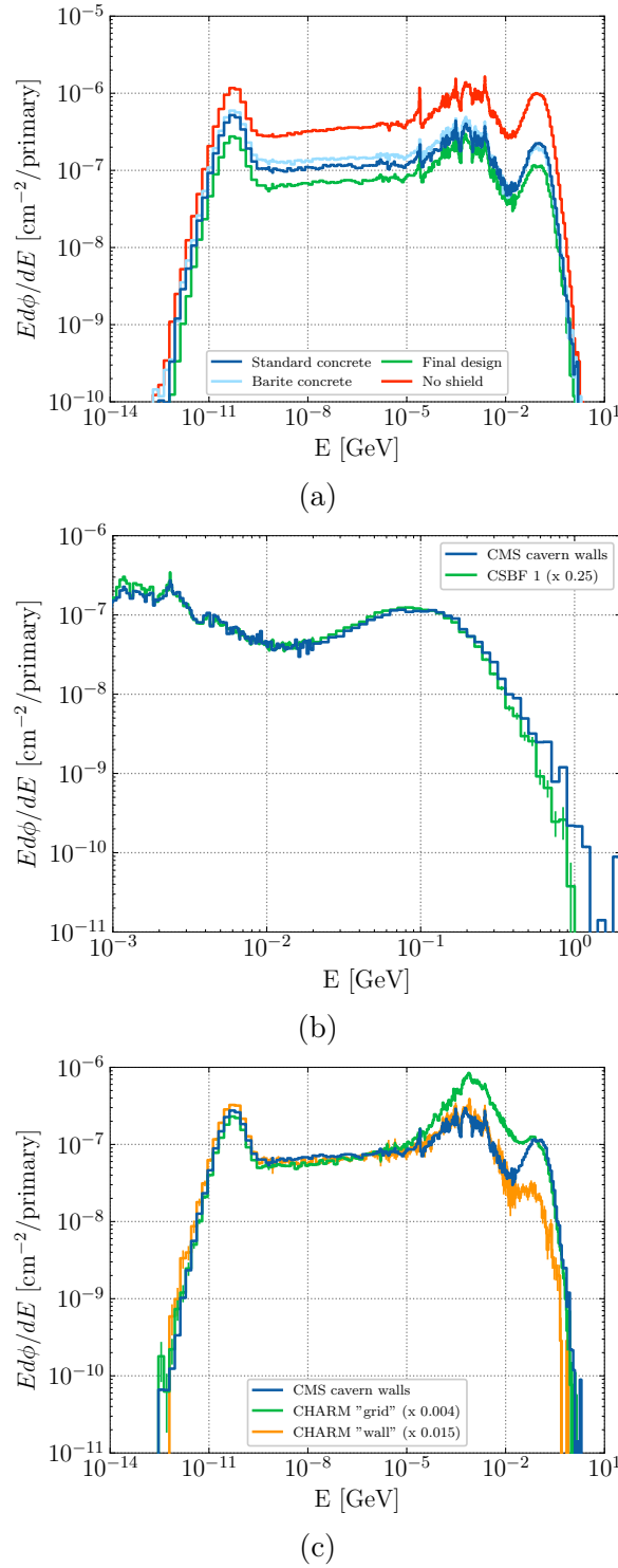
Figure 6.11: FLUKA simulation of the neutron fluence energy spectra at the CMS cavern walls and their comparison with those at the CERN Shielding Benchmark Facility (CSBF) and in the CERN High energy Accelerator Mixed field (CHARM) facility: (a) neutron fluence spectra at the CMS cavern walls for various shield designs; (b) neutron fluence spectra above 1 MeV at the CMS cavern walls (final shield installed) compared with those at the first CSBF location; (c) neutron fluence spectra at the CMS cavern walls (final shield installed) compared with those at CHARM.
