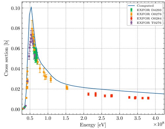
(h) ^{59}\text{Co}(p, x)^{56}\text{Co}
