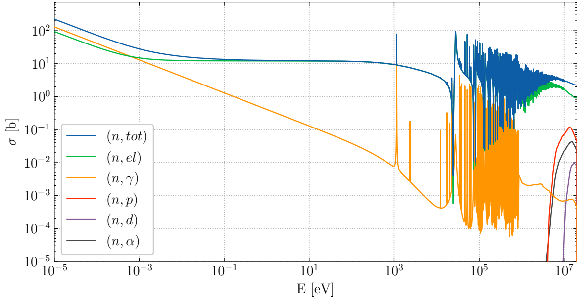
Figure 2.7: Cross sections of neutron interactions in ^{56}\text{Fe} below 20 MeV: (n, tot) , (n, el) and (n, \gamma) indicate respectively the total, elastic and capture cross sections. The data shown are extracted from the JEFF-3.3 nuclear data library [46].
