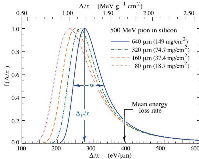
Figure 2.2: Straggling function of 500 MeV pions for various silicon thicknesses: the distributions have been normalized to unity at the most probable value [33].
