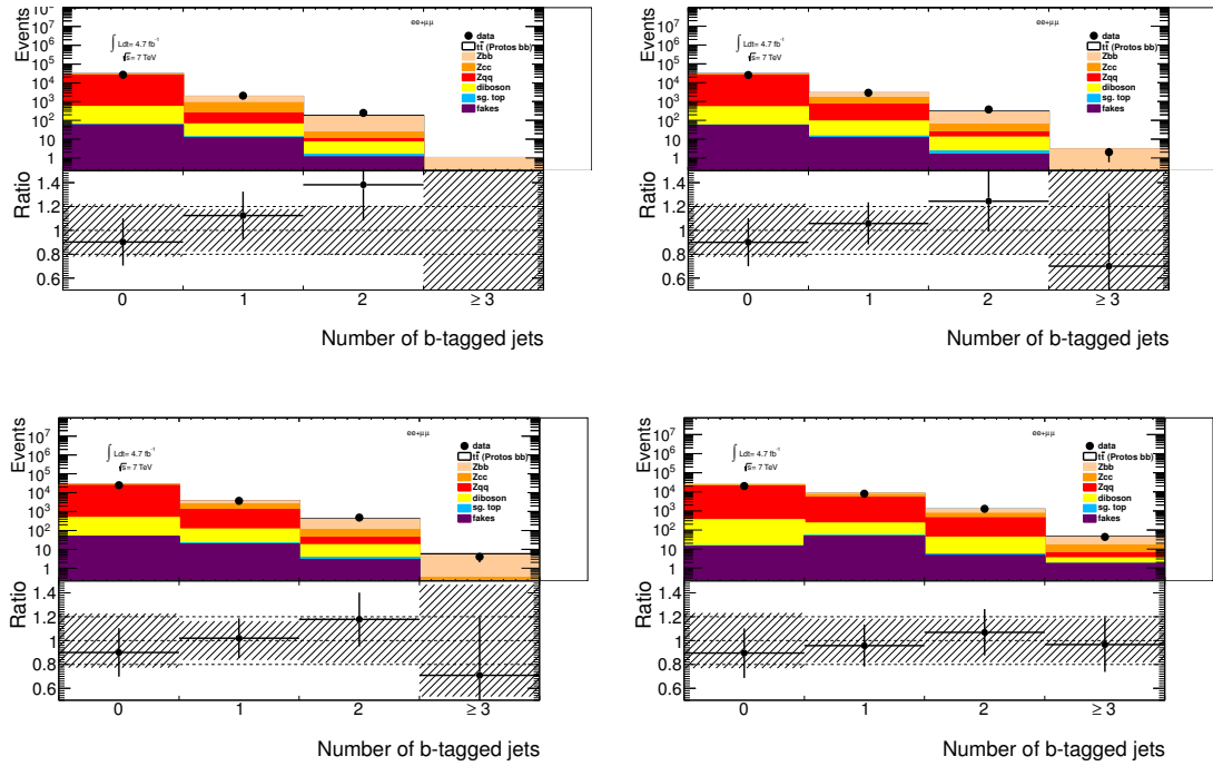
Figure D.1: Comparison of templates of physics processes simulation and data in Z+jets control region ( ee+\mu\mu channels combined). pTrel+system8 b -tagging scale factors had been applied to simulation. Distributions show number of tagged jets with MV1 algorithm at the (a) 60%, (b) 70%, (c) 75%, (d) 85% average tagging efficiency working point. The bottom panel shows data to simulation ratio, the shaded area shows the uncertainty associated with the b -tagging scale factors and the flavour composition of jets in the Z+jets events.
