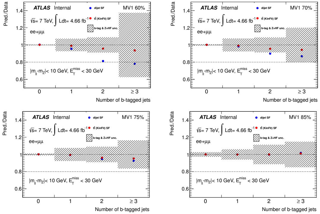
Figure D.4: Ratio of templates with p_{T\text{rel}}+\text{system8} scale factors and t\bar{t} scale factors with respect to results with no b -tagging scale factors applied ( ee+\mu\mu channels combined). The shaded area represents the uncertainty associated with the p_{T\text{rel}}+\text{system8} b -tagging scale factors and the flavour composition of jets in the Z +jets events. Distributions show ratios for the number of tagged jets with MV1 algorithm at the (a) 60%, (b) 70%, (c) 75%, (d) 85% average tagging efficiency working point. The bottom panel shows data to simulation ratio.
