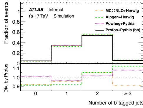
Figure 5.3: Number of b -tagged jets with MV1 at the 85% average efficiency working point for various t\bar{t} samples: MC@NLO+HERWIG, ALPGEN+HERWIG, POWHEG+PYTHIA and PROTOS ( t\bar{t} \rightarrow WWbb events only), which are described in section 3.4.1. All distributions are normalised to unity. The lower panel shows a comparison with PROTOS ( t\bar{t} \rightarrow WWbb ), which is used as the baseline.
