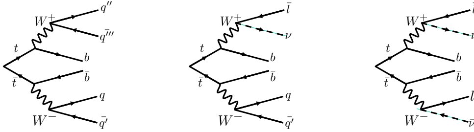
Figure 1.8: Top quark pair decay channels: All-jets (left), lepton+jets (middle) and dilepton (right) final states.
