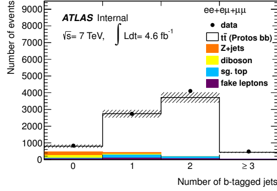
Figure 5.2: Number of b -tagged jets with MV1 at the 85% average efficiency working point. Data is compared to expectation from Monte Carlo simulation and a data-driven estimation of the contribution from fake leptons described in section 3.3.2. In case of Protos, only t\bar{t} \rightarrow WWbb events are considered here.
