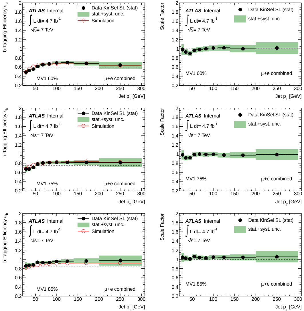
Figure C.2: b -tagging efficiency estimated from data compared with true efficiency (left) and resulting scale factors (right) together with statistical (bars) and systematic (band) uncertainties for the MV1 tagger at the working points corresponding to 60%, 75% and 85% b -tagging efficiency measured with the kinematic selection method in the single lepton channel [85]. The 70% working point is presented in figure 4.7.
