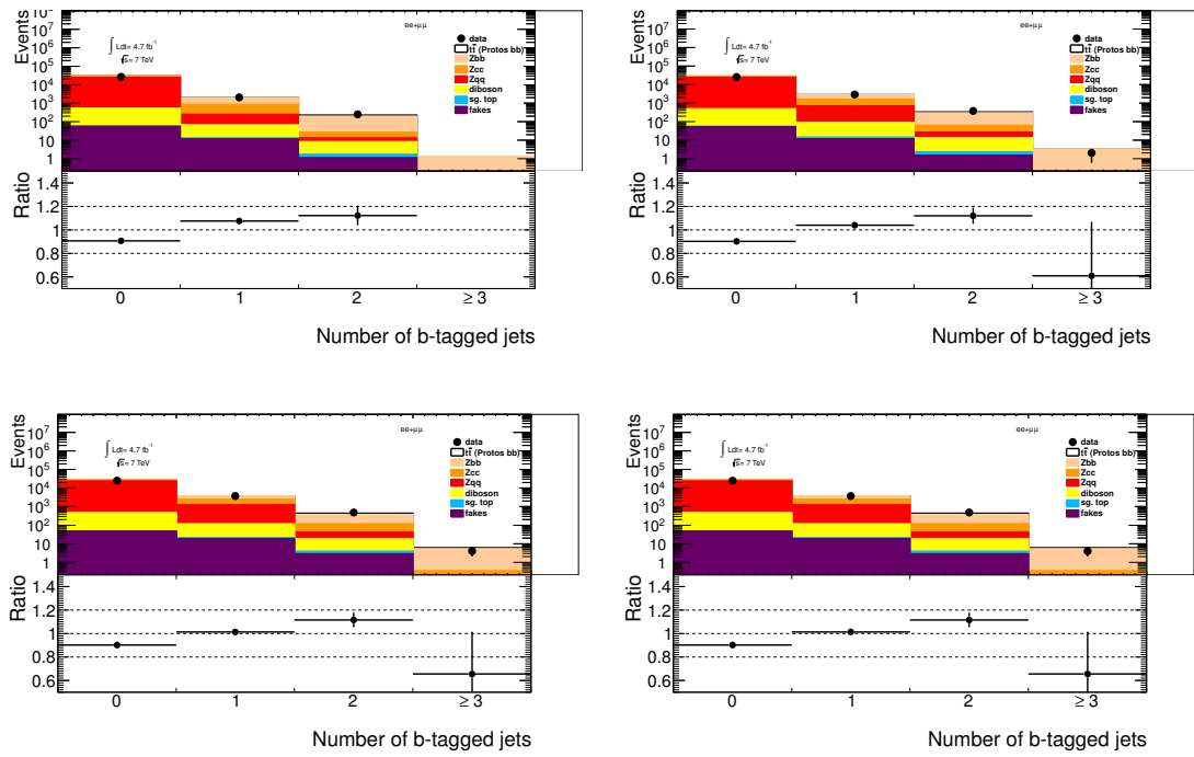
Figure D.3: Comparison of templates of physics processes simulation and data in Z+jets control region ( ee+\mu\mu channels combined). No scale factors had been applied to simulation. Distributions show number of tagged jets with MV1 algorithm at the (a) 60%, (b) 70%, (c) 75%, (d) 85% average tagging efficiency working point. The bottom panel shows data to simulation ratio.
