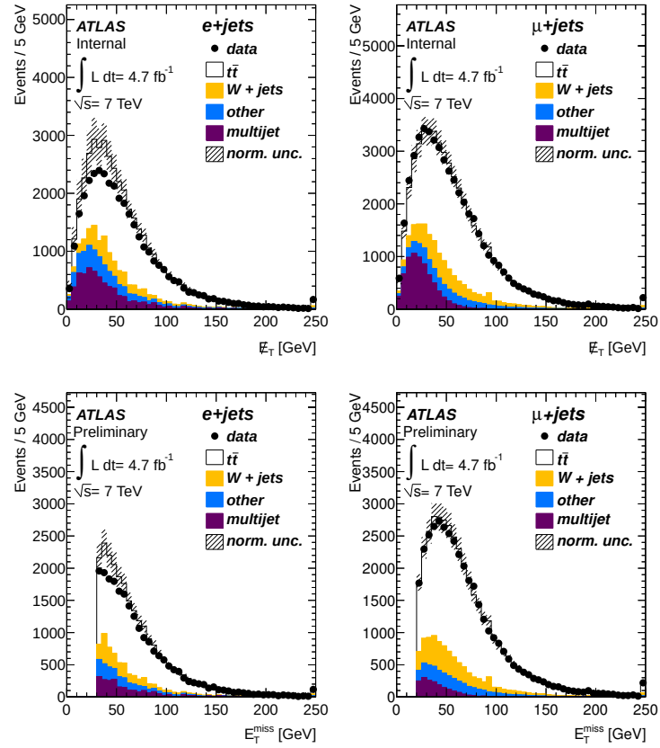
Figure 3.3: Missing transverse energy E_T^{\text{miss}} without [85] (upper row) and with [83] (lower row) the E_T^{\text{miss}} and m_T(l\nu) requirements for the e +jets channel (left) and \mu +jets channel (right). All other event selection criteria, including the requirement of at least one b -tagged jet, are applied. “Other” is a sum of contributions from Z +jets, single top and diboson production. The error band represents the sum of theoretical uncertainties on the cross sections ( t\bar{t} , single top, diboson and Z +jets) and uncertainties on the estimation directly from data ( W +jets and multijet). The last bin is inclusive.
