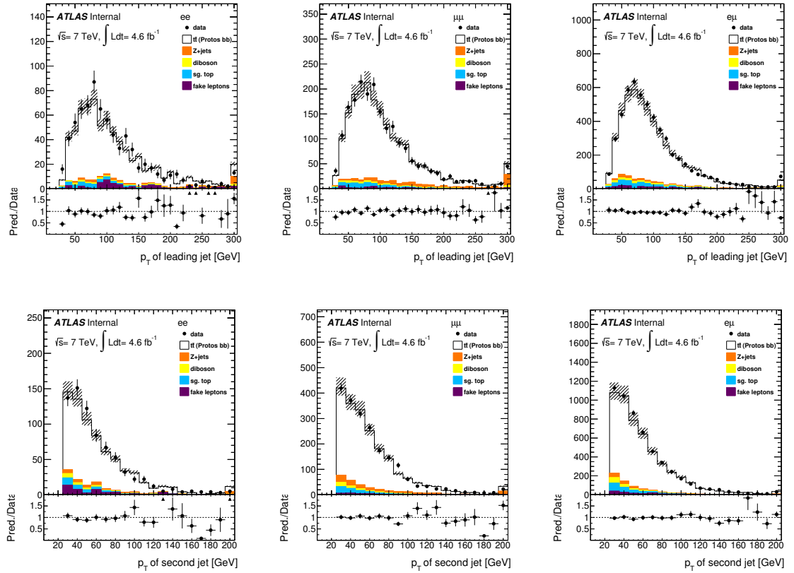
Figure 3.9: Distribution of the p_T of the leading (upper row) and second (lower row) jet in the ee (left), \mu\mu (middle) and e\mu channel (right). All event selection criteria are applied. The error band represents the sum of theoretical uncertainties on the cross sections ( t\bar{t} , single top, diboson and Z+jets production in e\mu channel) and uncertainties on the estimation directly from data (fakes, Z \rightarrow ee and Z \rightarrow \mu\mu ). The last bin is inclusive.
