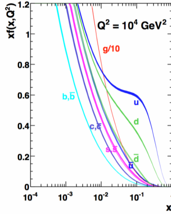
Figure 1.2: MSTW 2008 NLO PDFs at Q^2 = 10^4 \text{ GeV}^2 [13] which corresponds to the order of magnitude of m_t^2 .
