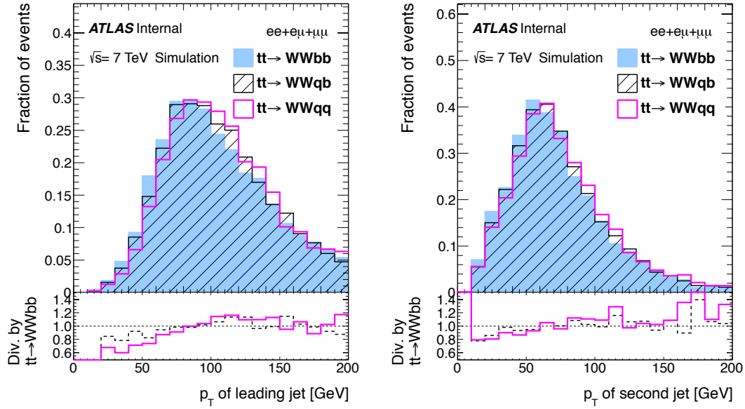
Figure 5.4: Distributions of p_T for the leading (left) and second (right) jet for tt \rightarrow WWbb , tt \rightarrow WWqb and tt \rightarrow WWqq events in the PROPOS + PYTHIA sample. The lower panel shows a comparison of the tt \rightarrow WWqb and tt \rightarrow WWqq distributions with tt \rightarrow WWbb , which is used as the baseline.
