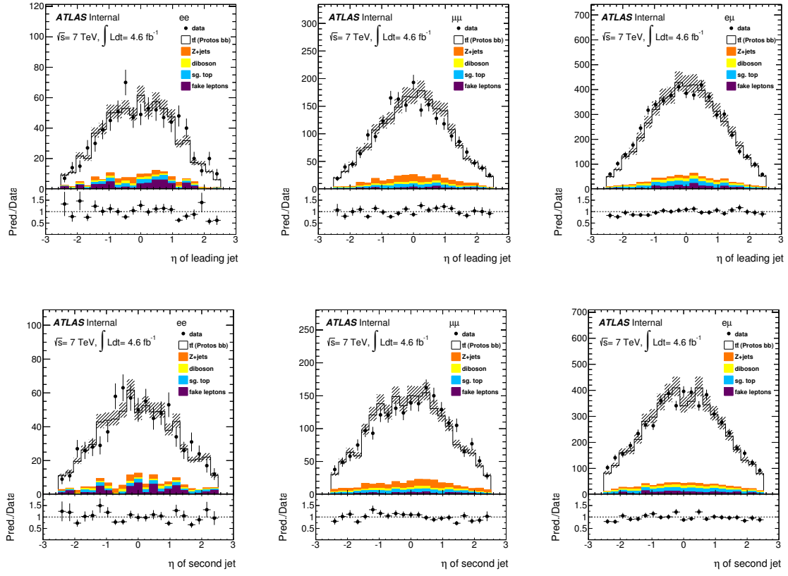
Figure A.1: Distribution of the \eta of the leading (upper row) and second (lower row) jet in ee (left), \mu\mu (middle) and e\mu channel (right). All event selection criteria are applied. The error band represents the sum of theoretical uncertainties on the cross sections ( t\bar{t} , single top, diboson and Z+jets production in e\mu channel) and uncertainties on the estimation directly from data (fakes, Z \rightarrow ee and Z \rightarrow \mu\mu ).
