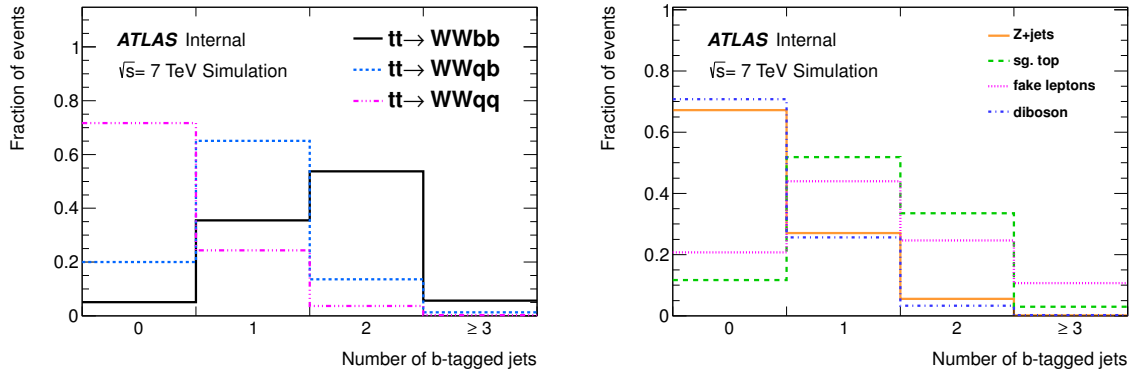
Figure 5.1: Number of b -tagged jets with MV1 at the 85% average efficiency working point for three signal categories: t\bar{t} \rightarrow WWbb , t\bar{t} \rightarrow WWqb and t\bar{t} \rightarrow WWqq (left) and for the background processes (right). All distributions are normalised to unity.
