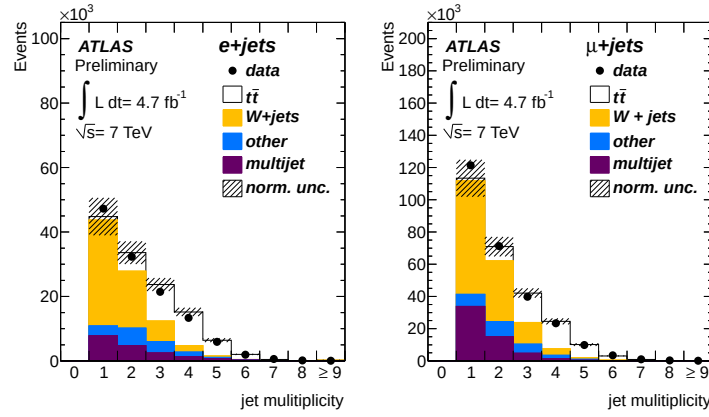
Figure 3.4: Jet multiplicity in the e+jets channel (left) and in the \mu+jets channel (right) [83]. At least one jet is required in these distributions. All other event selection criteria, including the requirement of at least one b -tagged jet, are applied. “Other” is a sum of contributions from Z+jets , single top and diboson production. The error band represents the sum of theoretical uncertainties on the cross sections ( t\bar{t} , single top, diboson and Z+jets ) and uncertainties on the estimation directly from data ( W+jets and multijet). The last bin is inclusive.
