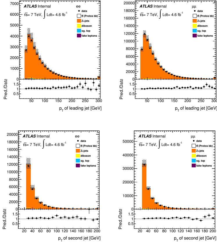
Figure 3.11: Distribution of the p_T of the leading (upper row) and second (lower row) jet for the ee (left) and \mu\mu channel (right) in the control region with E_T^{\text{miss}} < 60 GeV or |m_{ll} - 91 \text{ GeV}| < 10 GeV. All other standard event selection criteria are applied. The error band represents the sum of theoretical uncertainties on the cross sections ( Z +jets, t\bar{t} , single top, diboson) and uncertainties on the estimation directly from data (fake leptons). The last bin is inclusive.
