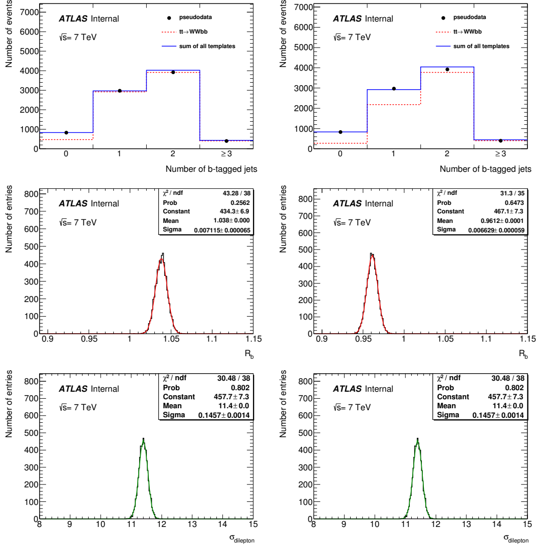
Figure H.1: Results for pseudo-experiments using templates with b -tagging 9 th eigenvalue variation – B_{\text{tag}} \text{ EV } 9 – down (left) and up (right). B_{\text{tag}} \text{ EV } 9 introduced the largest uncertainty from all 9 b -tagging eigenvalues, see appendix G. The top row shows an example fit in one of the pseudo-experiments, middle row shows distribution of measured values of R_b in the series of pseudo-experiments and the bottom rows shows the distribution of measured values of \sigma_{\text{dilepton}} .
