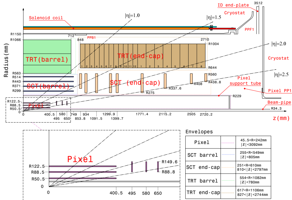
Figure 2.5: Alignment of the components of the inner detector [67].
