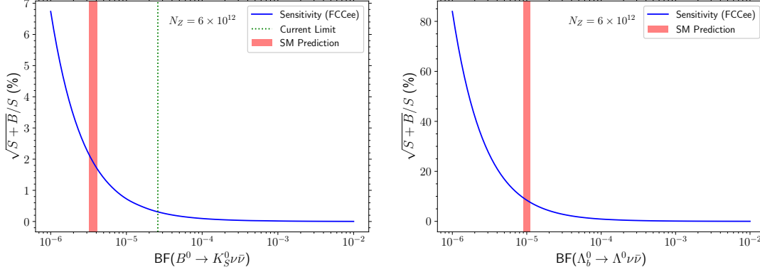
Figure 9: The expected sensitivity of the Tera-Z run at FCC-ee to the branching fraction of B^0 \rightarrow K_S^0\nu\bar{\nu} (left) and \Lambda_b^0 \rightarrow \Lambda^0\nu\bar{\nu} (right).
