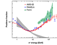
Figure 8: Positron fraction observed in terms of energy
