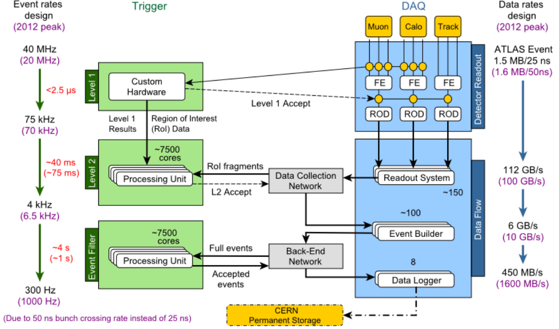
Figure 2.3: Overview of the TDAQ system
