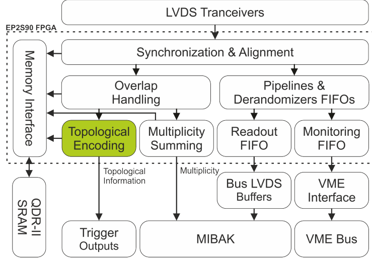
Figure 5.1: MIOCT block diagram
