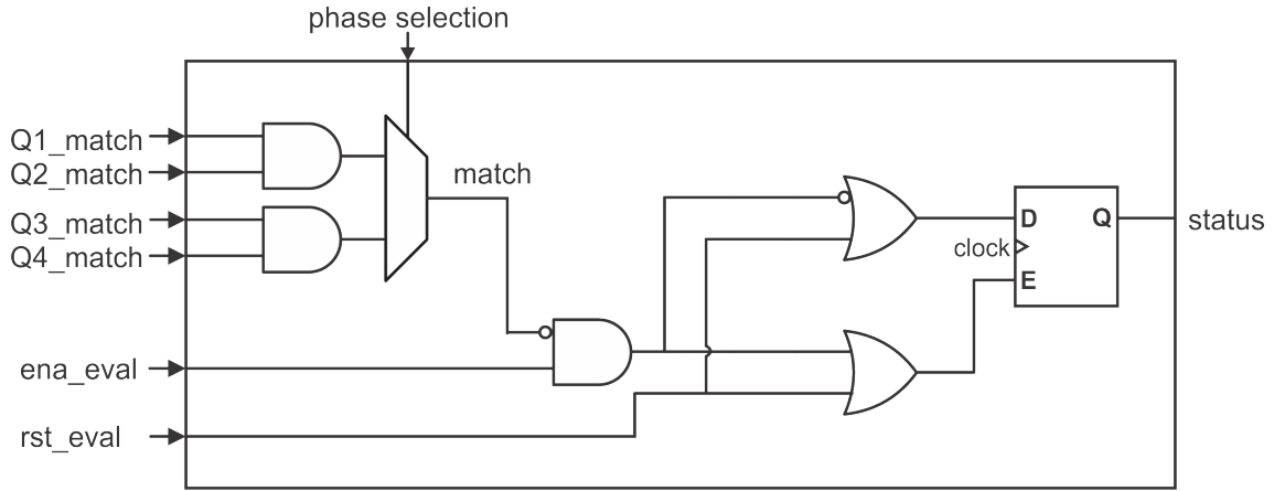
Figure 4.13: Transition detection circuit
