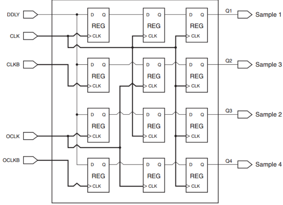
Figure 4.7: Xilinx ISERDES block diagram in Networking interface mode
