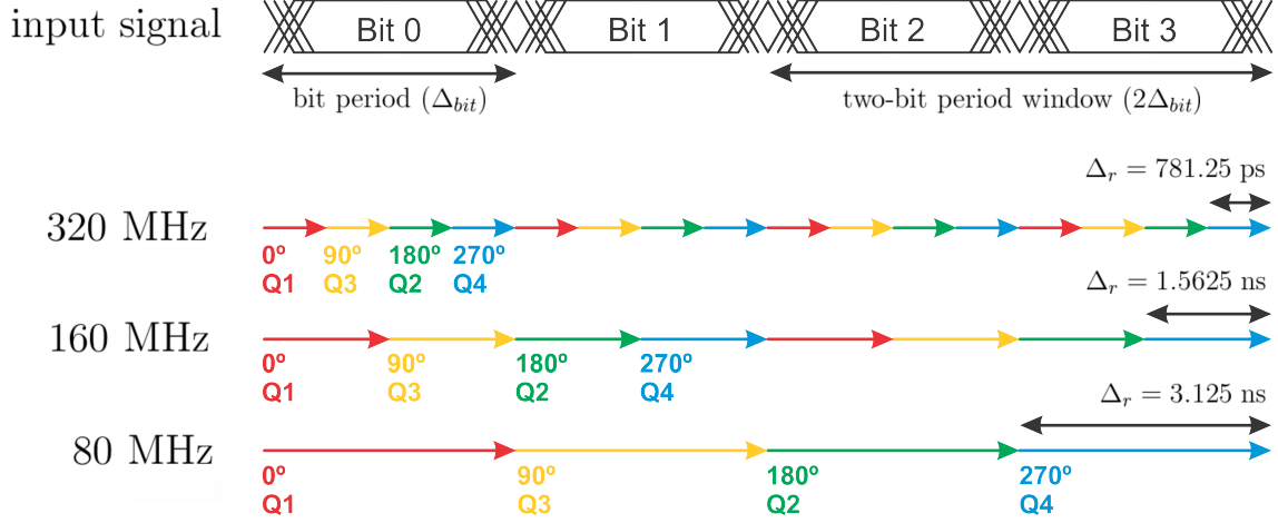
Figure 4.8: Timing diagram of the four different sampling points using four orthogonal clocks running at 320 MHz, 160 MHz, and 80 MHz
