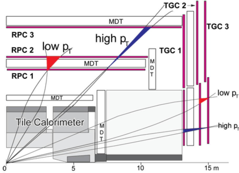
Figure 3.1: Schematic view of the muon detector
