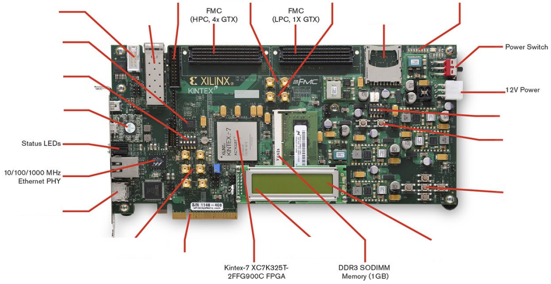
Figure 4.3: Xilinx Kintex-7 FPGA KC705 Evaluation Kit resources
