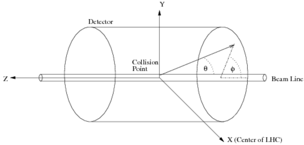
Figure A.1: ATLAS coordinate system
