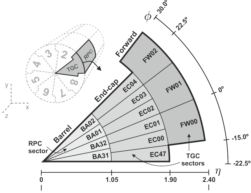
Figure 3.2: Muon trigger subsystems segmentation
