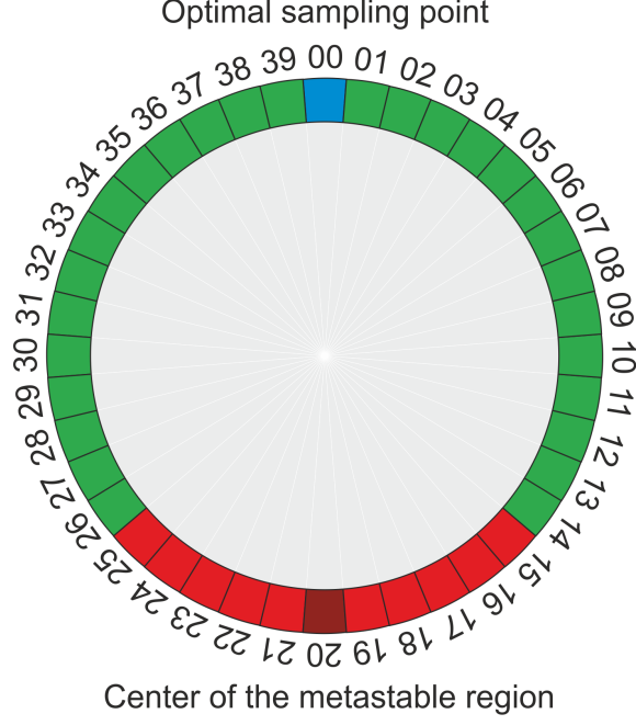
Figure 4.19: A cyclic description of the transition detector results for the channel 31
