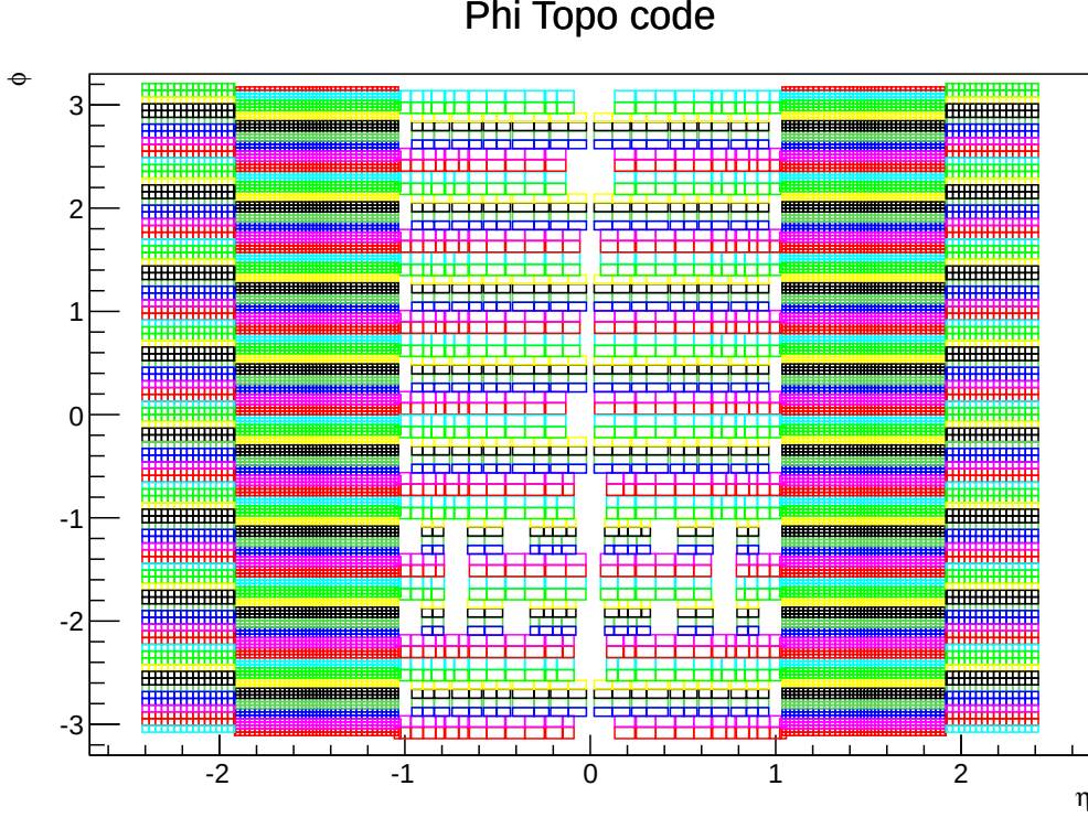
Figure 5.8: Sector and RoI Encoded in \phi
