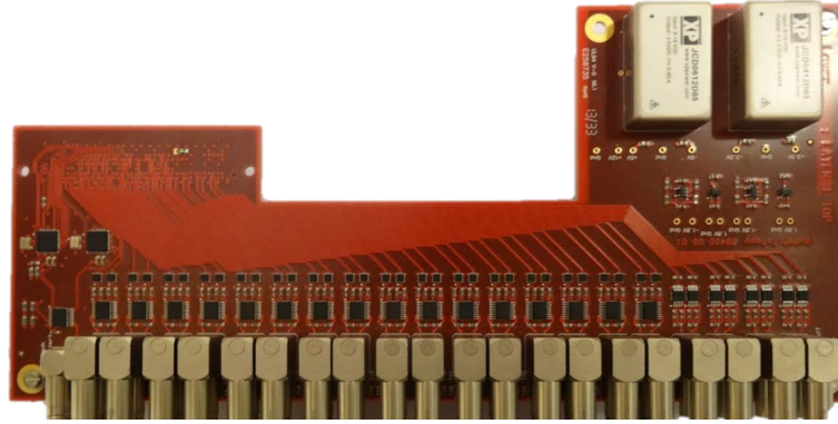
Figure 4.4: MUCTPI receiver mezzanine card
