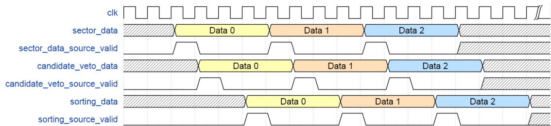
Figure 5.6: Timing diagram of the data flow control signals of the candidate veto and sorting units
