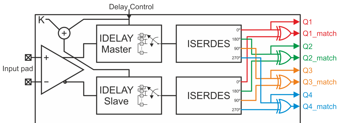
Figure 4.10: DDR input block diagram
