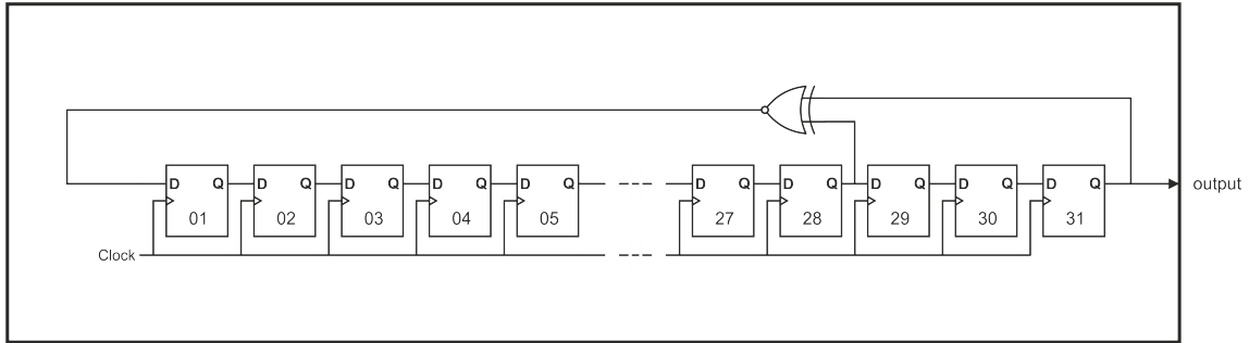
Figure 4.1: A PRBS generator of 2^{31} - 1 bits generated as the output of a 31-bit Fibonacci linear shift register
