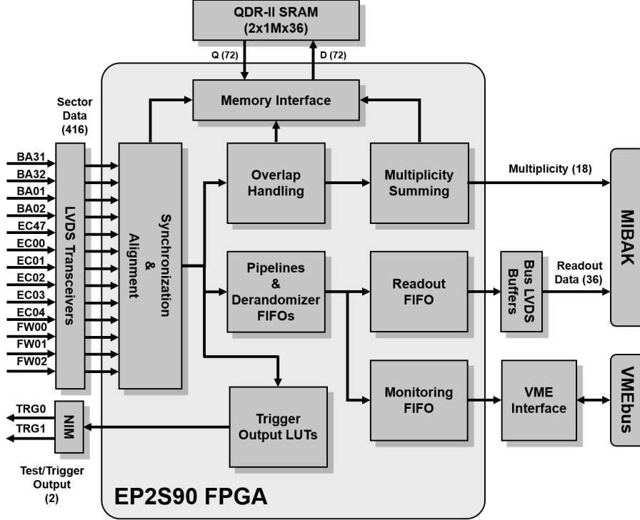
Figure 3.5: MIOCT block diagram
