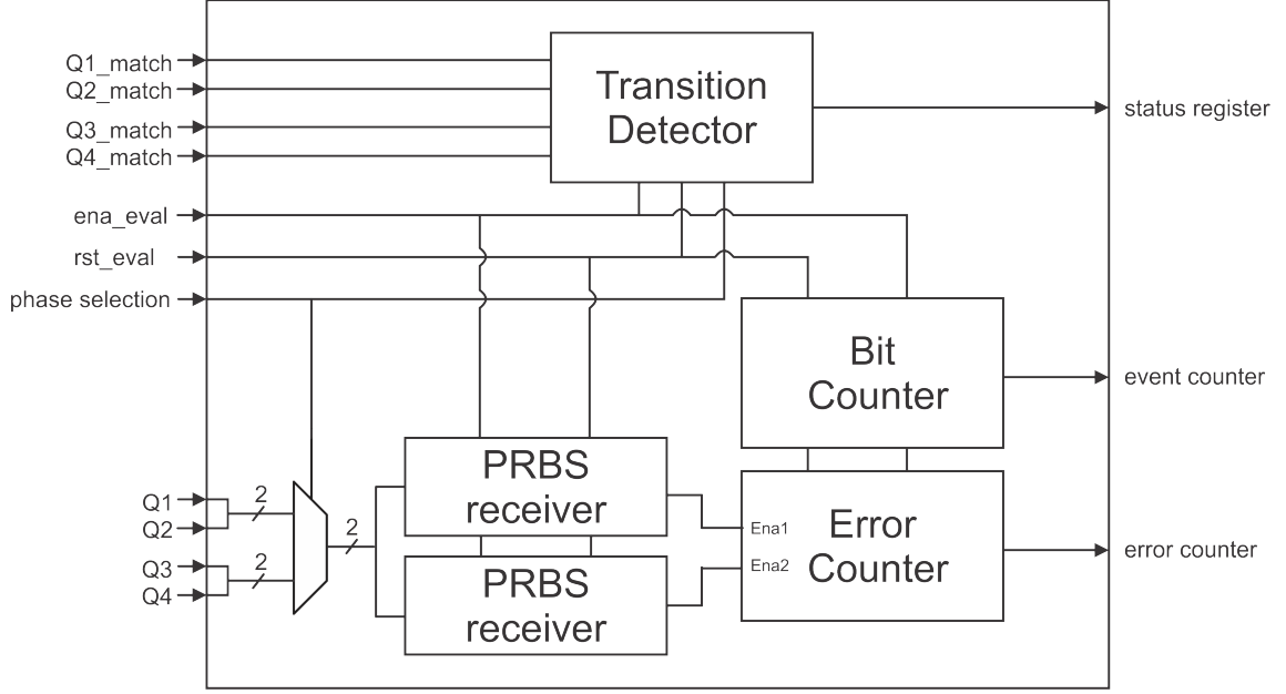
Figure 4.15: PRBS evaluation block diagram
