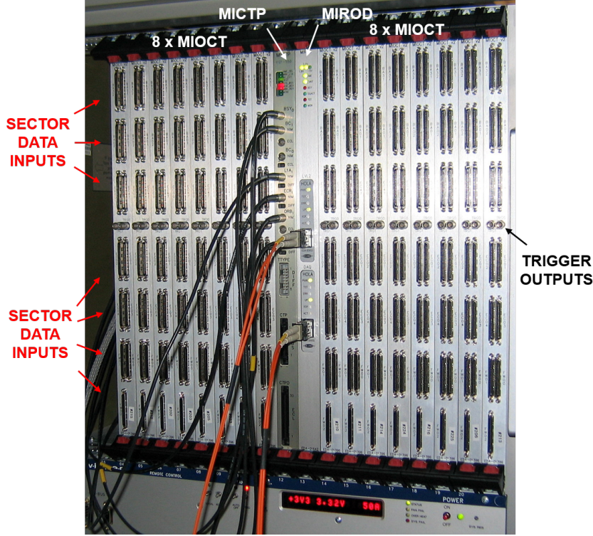
Figure 3.4: MUCTPI crate
