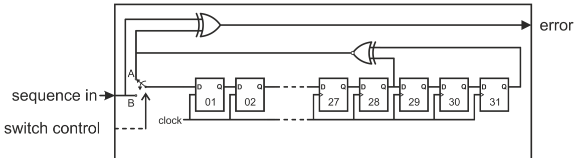
Figure 4.14: PRBS receiver circuit
