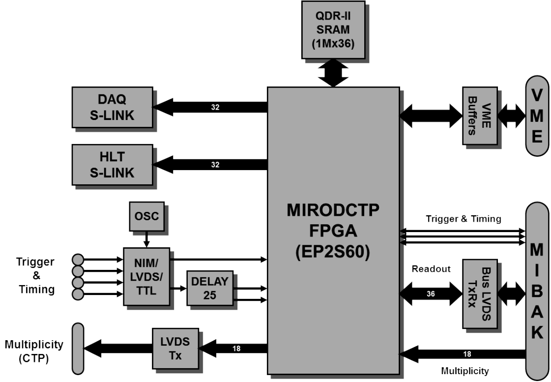
Figure 3.7: MIRODCTP module block diagram
