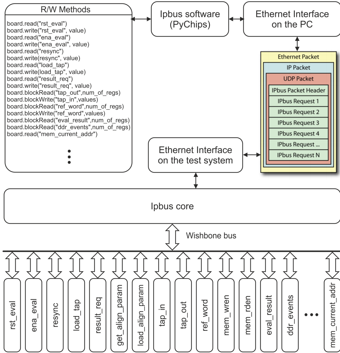
Figure 4.16: Principle of operation of the IPbus system
