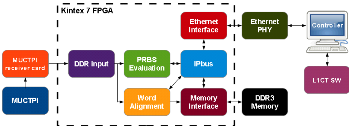
Figure 5.11: Block diagram of the upgraded error rate test system
