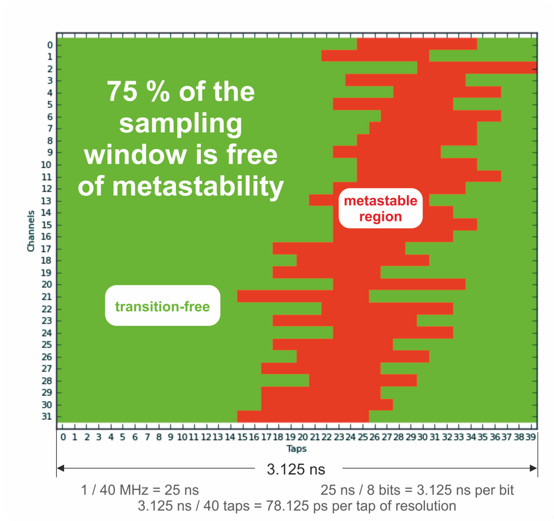
Figure 4.18: Phase scan of the received data from the MUCTPI system with the electrical trigger outputs operating at 320 Mbps
