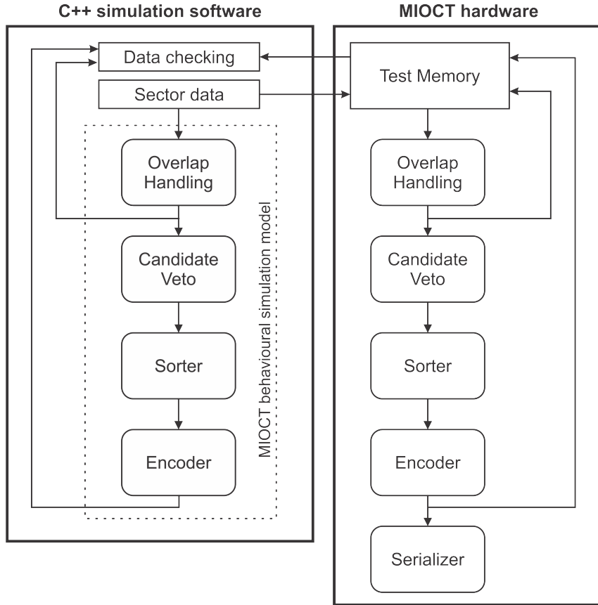
Figure 5.10: In-system Verification flow (only results from the overlap handling and the topology encoder are checked)
