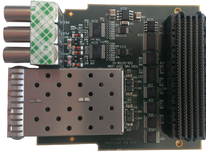
Figure 4.5: TCDS mezzanine card
