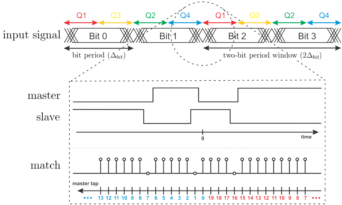
Figure 4.11: Timing diagram illustrating how transitions can be detected using the DDR input circuit
