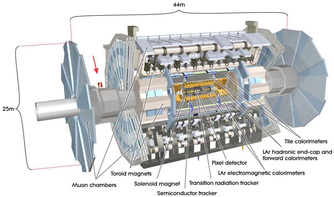
Figure 2.2: Overview of the ATLAS experiment
