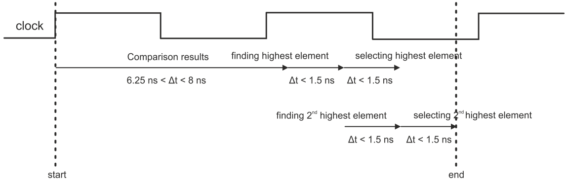
Figure 5.4: Simplified timing diagram of the sorting unit pipelined in four stages
