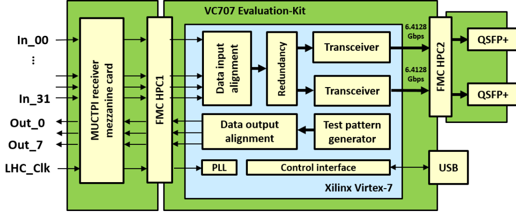
Figure 6.1: MuCTPiToTopo block diagram
