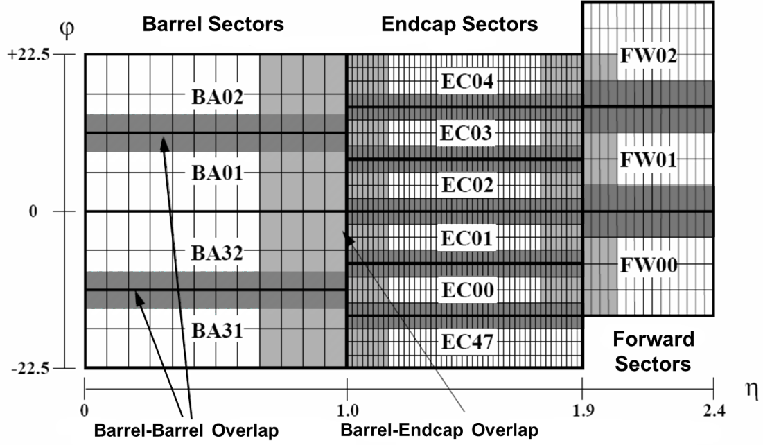
Figure 3.6: Overlap regions handled by the MIOCT module
