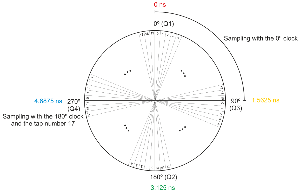
Figure 4.9: Phase coverage, when the tap delay selection is limited to 20 taps and four orthogonal phases are used to sample the input data
