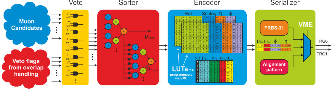
Figure 5.2: Topological encoding block diagram
