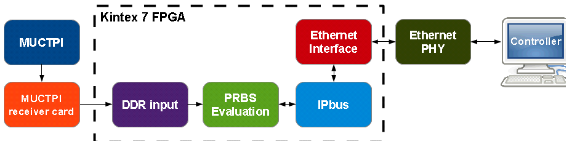
Figure 4.6: Error rate test system block diagram
