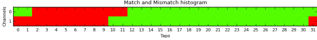
Figure 4.20: Phase scan color-coded histogram of the received data from the MUCTPI operating at 400 Mbps
