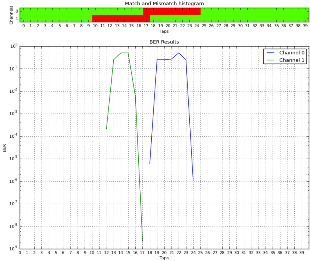
Figure 4.21: A plot of the BER of the data received from two MUCTPI electrical trigger outputs
