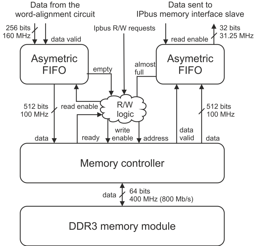
Figure 5.12: Memory interface block diagram
