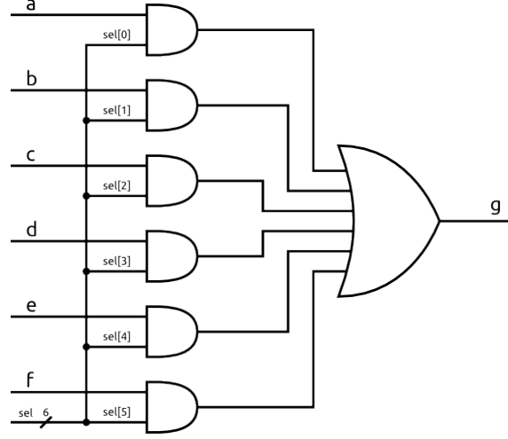
Figure 5.3: Logic diagram for a 6-input one-hot multiplexer
