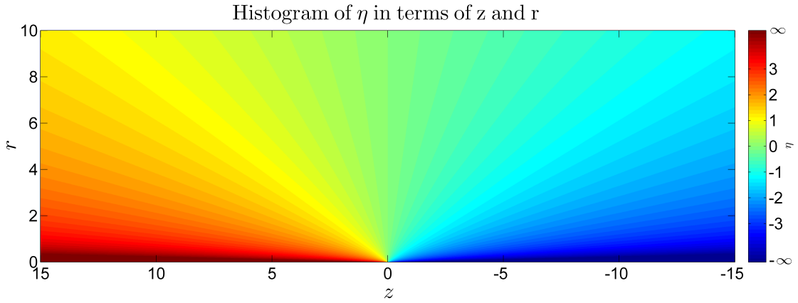
Figure A.2: Histogram of \eta in terms of z and r
