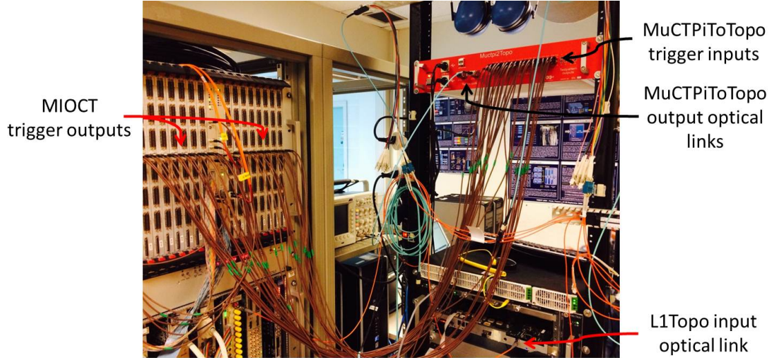
Figure 6.3: Photo of the MUCTPI integration tests with MuCTPiToTopo interface and L1Topo processor
