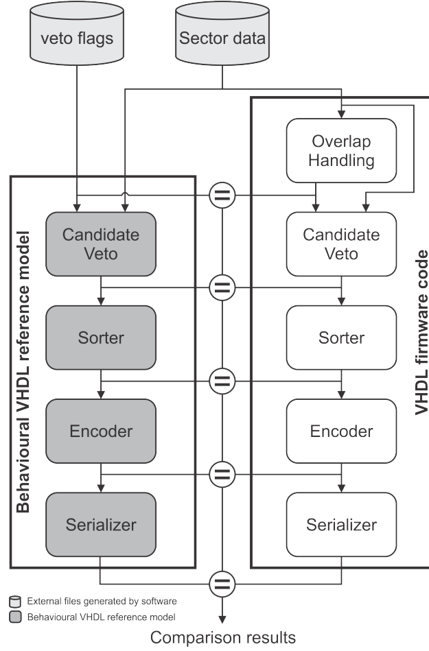
Figure 5.9: Functional simulation flow
