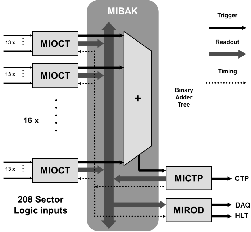
Figure 3.3: MUCTPI system block diagram
