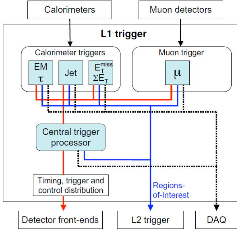
Figure 2.4: Overview of the Level-1 trigger system
