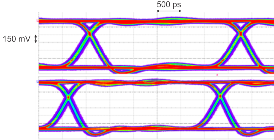
Figure 4.2: Eye-diagram of two MIOCT outputs operating at 320 Mbps
