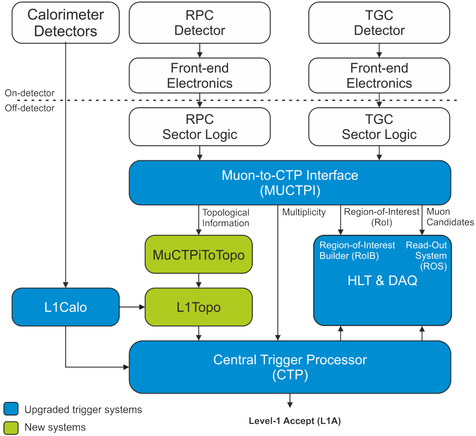
Figure 2.5: Overview of the Level-1 trigger for the Run 2 with emphasis on the muon trigger system
