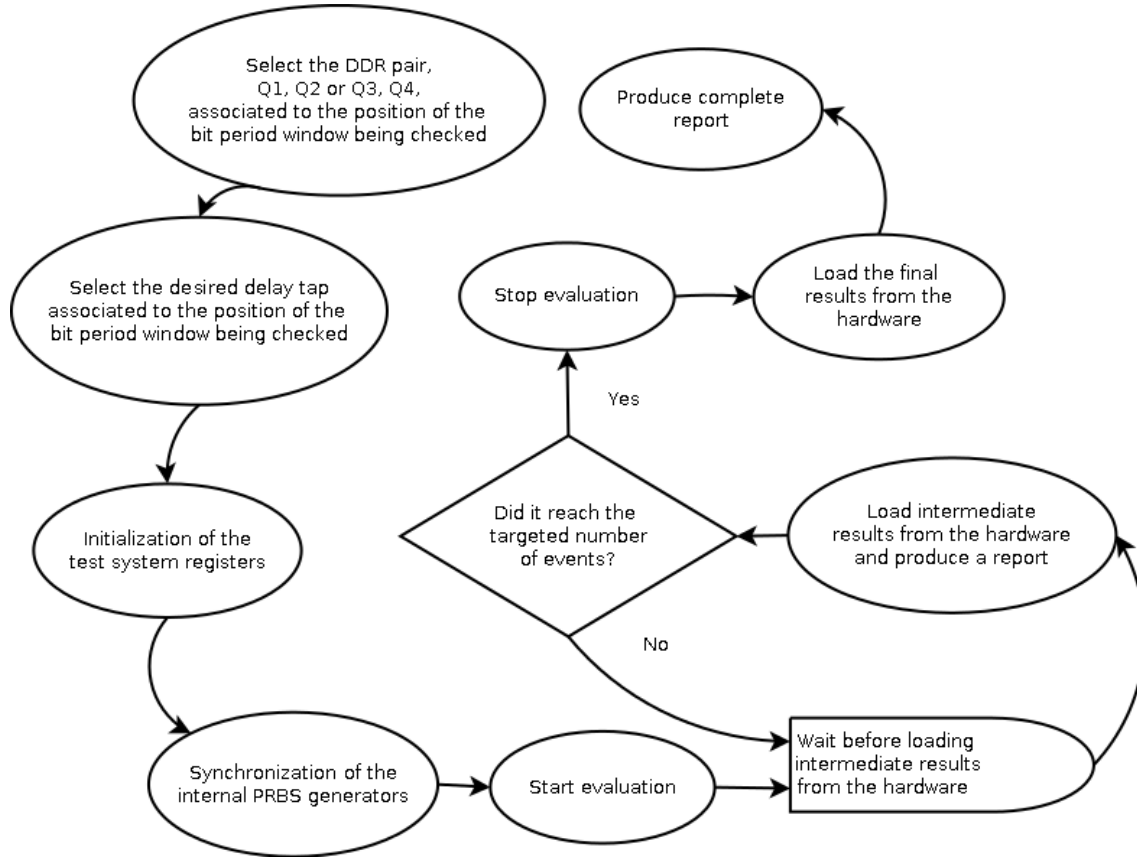
Figure 4.17: FSM diagram of the software operation of a test iteration (an iteration is executed for each position of the bit period window being checked)
