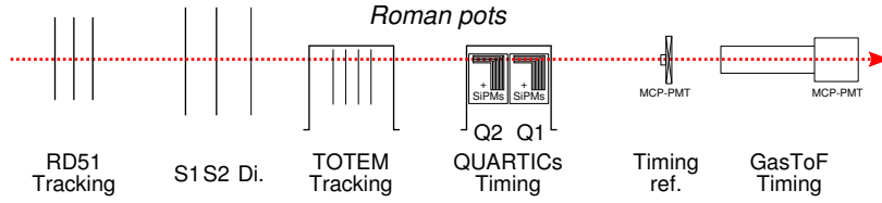
Figure 4.18: Detectors layout for the end of 2015 test beams at CERN's SPS.
