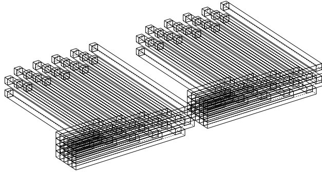
Figure 4.3: Schematic view of two Quartic stations containing an array of 4 \times 5 radiator bars each, as developed for the early CT-PPS timing operations. The SiPMs readout devices are pictured as the squared volumes at the end of the "L"-bars.
