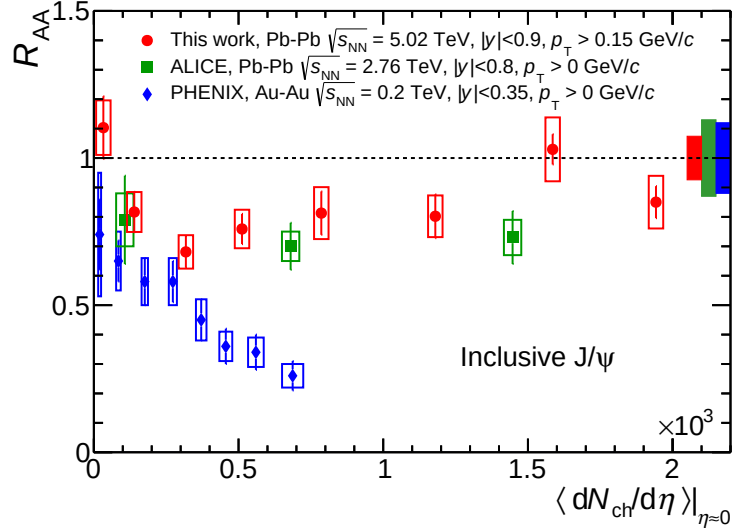
Figure 5.5: Inclusive J/\psi R_{AA} at midrapidity as a function of the midrapidity charged-particle density dN_{ch}/d\eta|_{\eta=0} measured in Pb–Pb collisions at \sqrt{s_{NN}} = 5.02 TeV and at \sqrt{s_{NN}} = 2.76 TeV [174] and in Au–Au collisions at \sqrt{s_{NN}} = 0.2 TeV [97]. Values of dN_{ch}/d\eta|_{\eta=0} are taken from [175] for \sqrt{s_{NN}} = 5.02 TeV, from [176] for \sqrt{s_{NN}} = 2.76 TeV and from [177] for \sqrt{s_{NN}} = 0.2 TeV.
