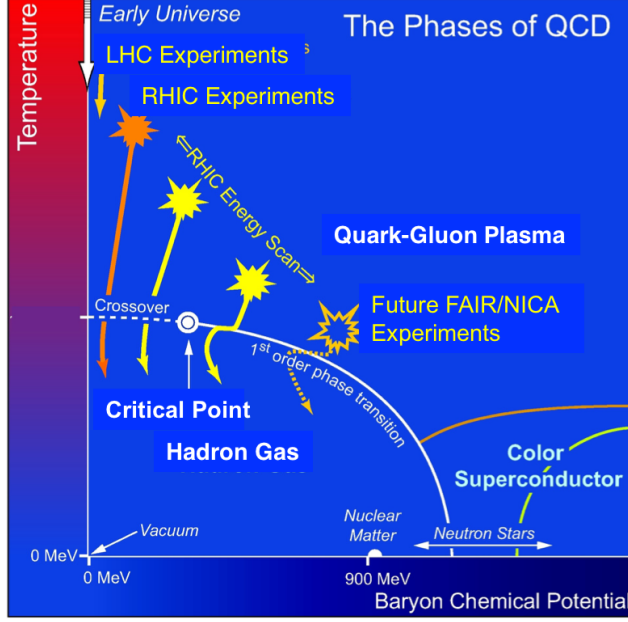
Figure 1.3: Possible QCD phase diagram in the temperature and baryon chemical potential plane. Regions probed by different hadron collider and fixed-target experiments are indicated. (Figure is taken from [13].)
