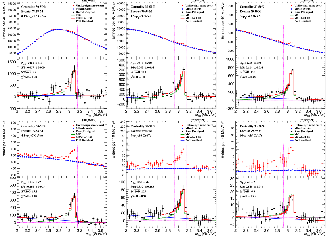
Figure 4.11: Invariant mass distribution of J/\psi candidates and background obtained by event mixing for centrality 30–50% and different p_T intervals are shown in the tops of the plots. The distribution of J/\psi candidates after subtraction of background modeled by event mixing is shown in the lower panels together with a fit function.
