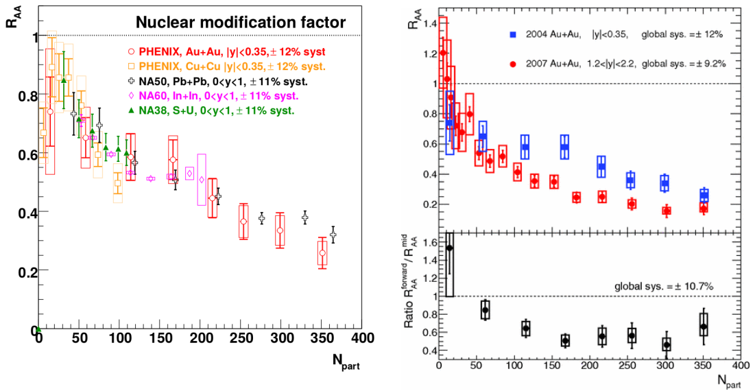
Figure 2.10: Left: Inclusive J/\psi nuclear modification factor R_{AA} measured by the SPS experiments NA38, NA50 and NA60 in In–In, S–U, and Pb–Pb collision and the RHIC experiment PHENIX in Au–Au and Cu–Cu collisions as a function of the participant number. (Figure is taken from [98].) Right: Inclusive J/\psi nuclear modification factor R_{AA} at forward rapidity [96] and at midrapidity [97] and their ratio measured by the PHENIX experiment in Au–Au collisions [96].
