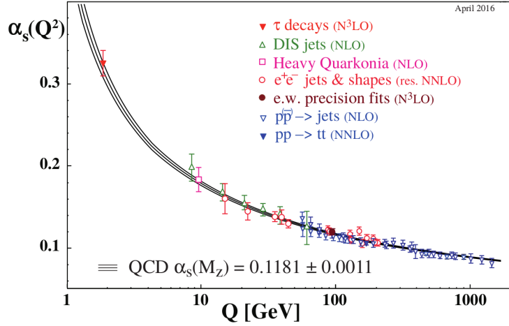
Figure 1.2: Measurements of the strong coupling constant \alpha_s as a function of the energy scale Q . (Figure is taken from [9].)
