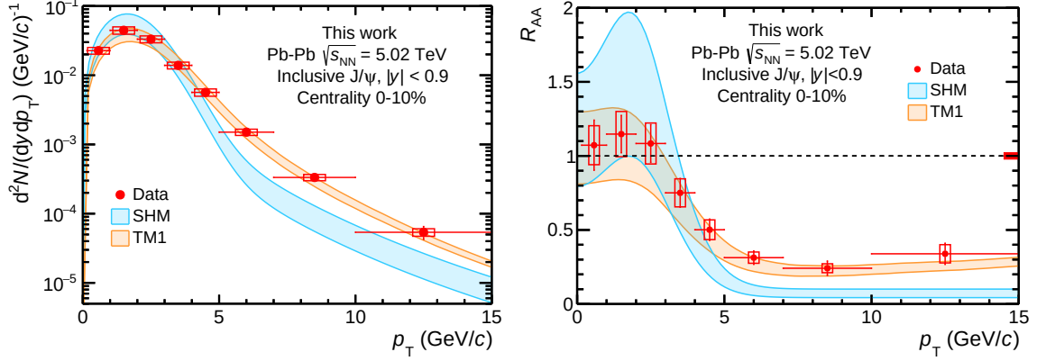
Figure 5.9: Inclusive J/\psi production yield (left) and R_{AA} (right) as a function of p_T in Pb-Pb collisions in the centrality class 0–10%. The measurement is compared to the model calculations of the SHM [101] and the TM1 [105].
