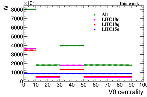
Figure 4.3: The centrality distribution for selected events.
