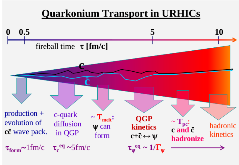
Figure 2.12: Schematic time evolution of a correlated charm-anti-charm quark pair in an expanding fireball in an ultra-relativistic heavy-ion collision. (Figure is taken from [102].)
