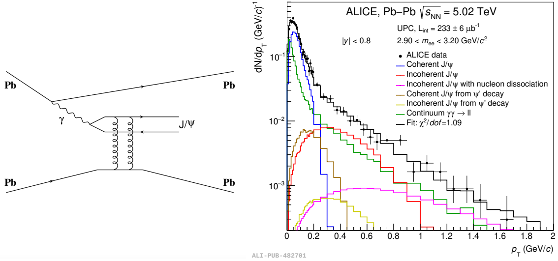
Figure 2.9: Left: J/\psi production mechanism in UPCs at the leading order. (Figure is taken from [90].) Right: Number of coherent photoproduction J/\psi candidates as a function of transverse momentum. The distribution is fitted with Monte Carlo templates corresponding to different production mechanisms. (Figure is taken from [89].)
