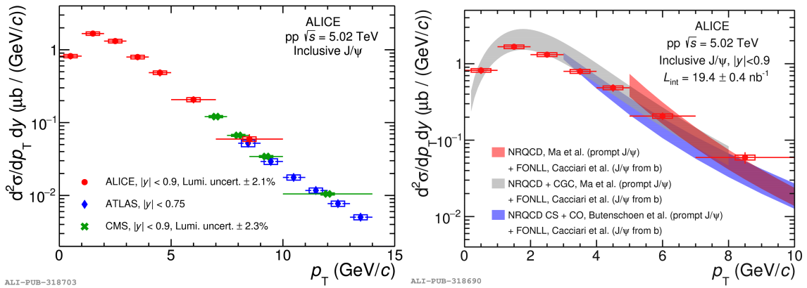
Figure 2.5: Left: p_T -differential inclusive J/\psi cross section in pp collisions at 5.02 TeV measured by ALICE [66] compared with ATLAS [67] and CMS [68] measurements at midrapidity. Right: p_T -differential inclusive J/\psi cross section [66] compared with NLO NRQCD [69, 70] and LO NRQCD+CGC [71] prompt J/\psi calculations summed with FONLL calculations for non-prompt J/\psi contribution [72].
