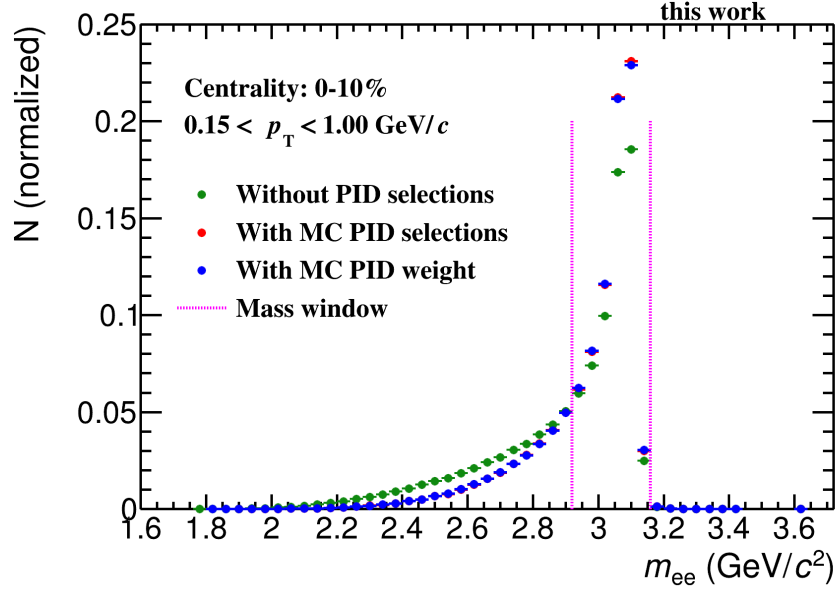
Figure 4.25: J/\psi invariant mass shape for 0.15 < p_T < 1 GeV/ c and centrality 0–10% for three cases: when not applying PID selections, when applying MC PID selections and when applying the efficiency weight using the MC leg PID efficiency.
