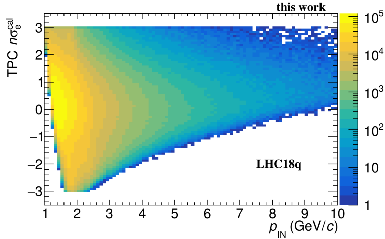
Figure 4.8: n\sigma_e^{\text{cal}} versus momentum in the inner wall of the TPC after applying selection criteria on post-calibrated n\sigma_e , n\sigma_p and n\sigma_\pi for LHC18q data set.
