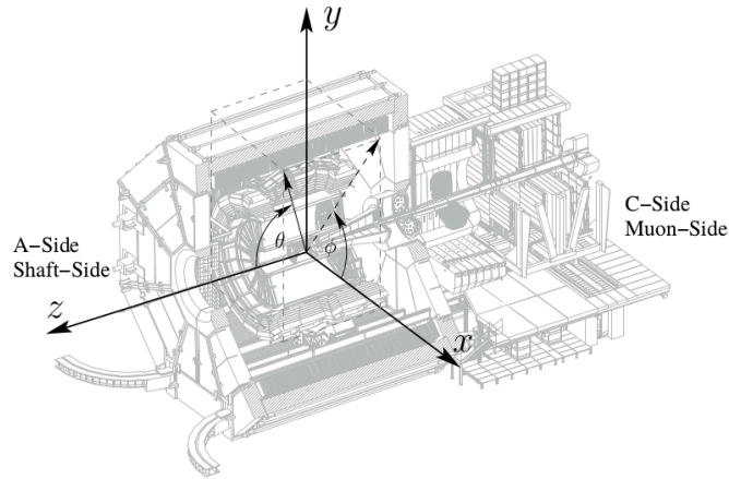
Figure 3.2: The ALICE detector and its coordinate system. (Figure is taken from [126].)
