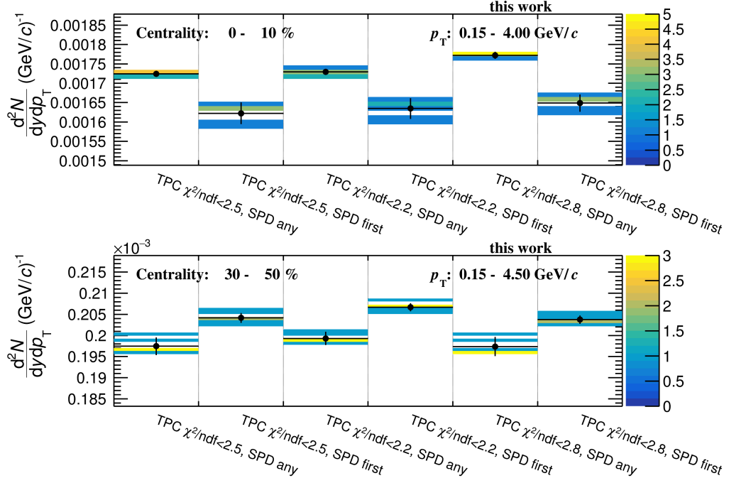
Figure 4.20: Examples of corrected J/\psi yield for simultaneous fit range and tracking selection variations. Means of cases with different fit ranges for one set of tracking selections shown in black. Color scale corresponds to the number of the variations falling into an interval of corrected J/\psi yield.
