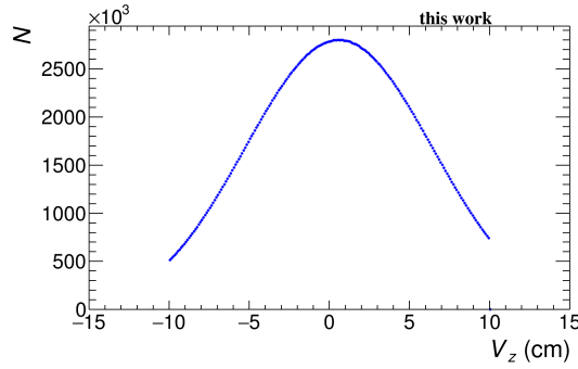
Figure 4.1: The distribution of vertex z position after applying the selection |V_z| < 10 cm.
