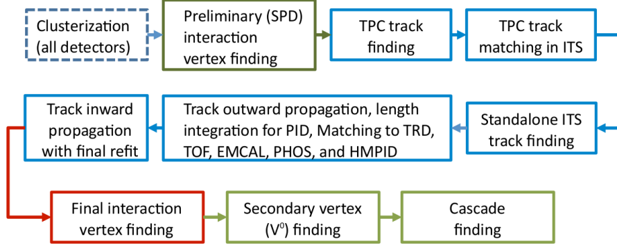
Figure 3.6: Flow of Central Barrel event reconstruction. (Figure is taken from [134].)
