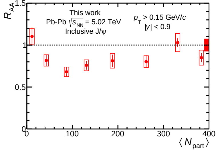
Figure 5.3: Inclusive J/\psi nuclear modification factor R_{AA} , integrated over p_T , as a function of \langle N_{\text{part}} \rangle . Vertical bars indicate statistical uncertainty, the boxes around the data points represent the systematic uncertainties on J/\psi yield in Pb–Pb collisions and the average nuclear overlap function \langle T_{AA} \rangle . The box around unity show global uncertainty originating from the uncertainty on the J/\psi cross section in pp collisions.
