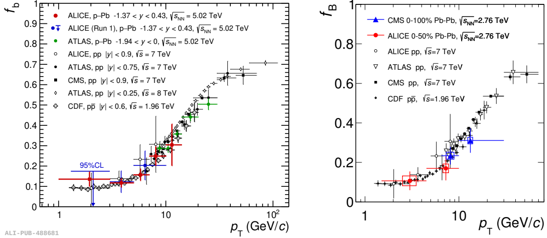
Figure 2.3: Fraction of J/\psi from b-hadron decays as function of J/\psi p_T in pp, p\bar{p} , p\bar{p} , and p–Pb collisions at TeV energies [56] (left) and in pp and Pb–Pb collisions [57] (right).
