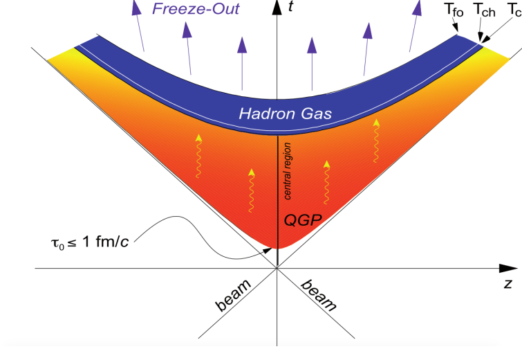
Figure 1.4: Illustration of the space-time evolution of a heavy-ion collision with sufficient energy density for the QGP formation. (Figure is taken from [17].)
