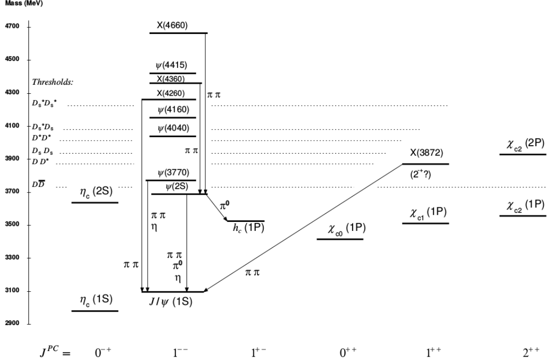
Figure 2.2: The level scheme of experimentally established charmonium states. Only observed hadronic transitions are shown. The single photon transitions \psi(nS) \rightarrow \gamma\eta_c(mS) , \psi(nS) \rightarrow \gamma\chi_{cJ}(mP) , \chi_{cJ}(1P) \rightarrow \gamma J/\psi are omitted for clarity. (Figure is taken from [9].)
