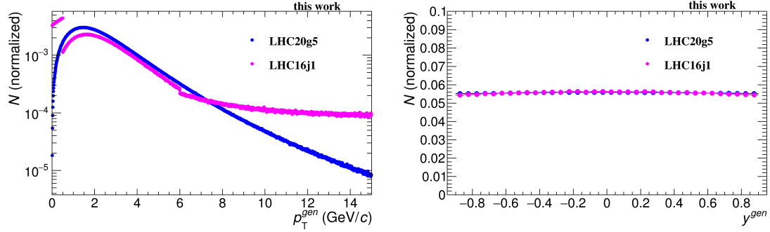
Figure 4.4: The transverse momentum and rapidity distributions of J/\psi generated by the MC simulations.
