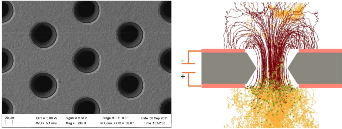
Figure 3.11: Left: An electron microscope photograph of a GEM foil. (Figure is taken from [150].) Right: Simulation of charge dynamics of two electrons passing through a GEM hole. Electron paths are shown as yellow lines, whereas ions as dark red lines. Places of ionization are marked with spots. (Figure is taken from [151].)
