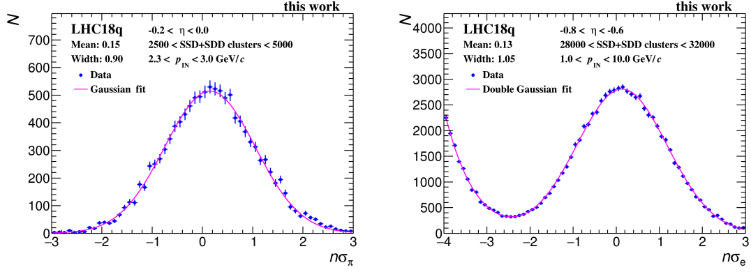
Figure 4.6: Left: Distribution of n\sigma_\pi of clean pion sample fitted by Gaussian function. Right: Distribution of n\sigma_e of relatively clean electron sample from photon conversions fitted by double Gaussian function to account for pion contamination.
