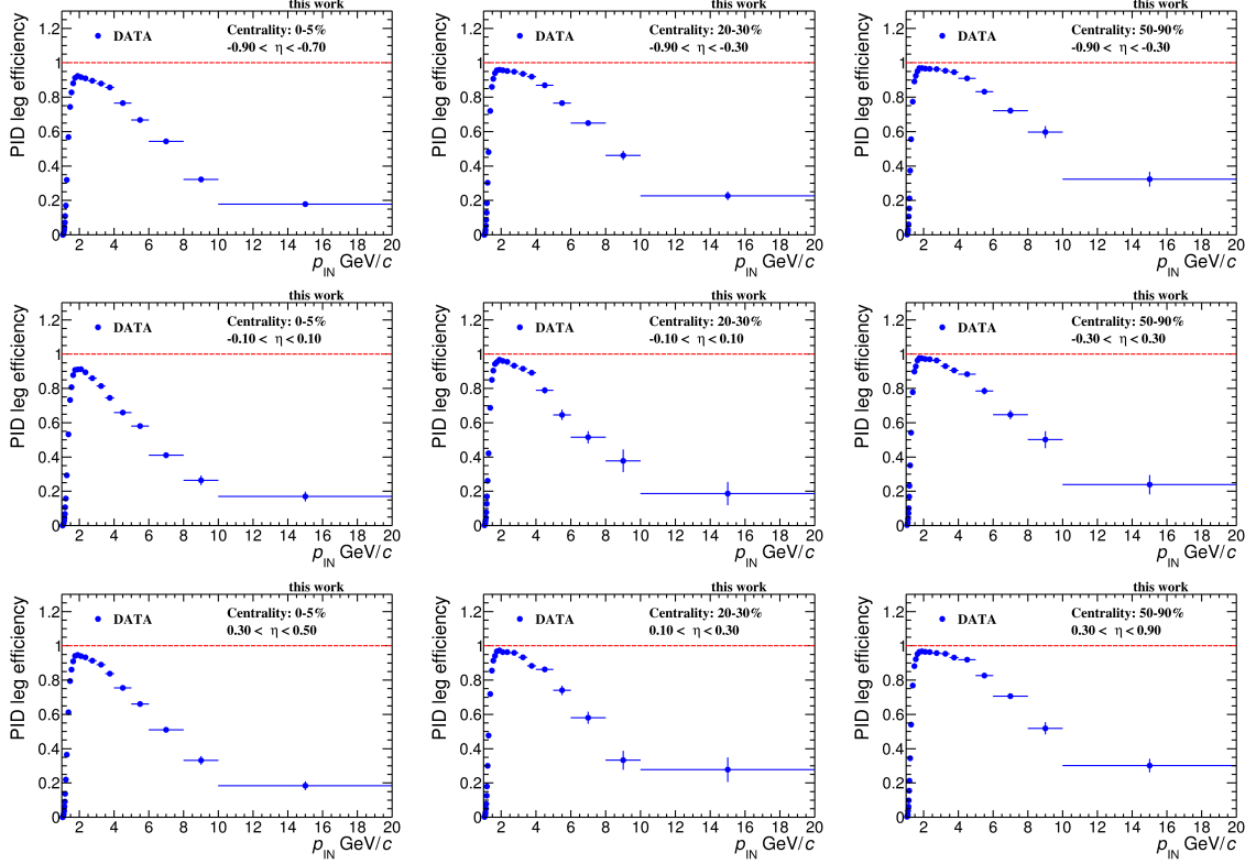
Figure 4.15: Examples of leg PID efficiency distribution as a function of p_{\text{IN}} for different \eta intervals and centralities 0–5% (left), 20–30% (middle) and 50–90% (right).
