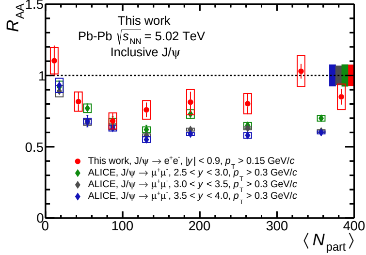
Figure 5.4: Inclusive J/\psi nuclear modification factor R_{AA} in Pb–Pb collisions at \sqrt{s_{NN}} = 5.02 TeV as a function of \langle N_{part} \rangle at midrapidity ( |y| < 0.9 ) and at forward rapidity for three rapidity intervals ( 2.5 < y < 3.0 , 3.0 < y < 3.5 and 3.5 < y < 4.0 ) [173].
