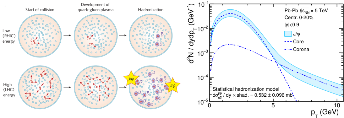
Figure 2.11: Left: Illustration of charm production in A–A collisions at low energies (RHIC) and high energies (LHC). The blue small circles represent light quarks and anti-quarks, red circles charm quarks and anti-quarks. The beginning of the collision is depicted on the left. It is followed by QGP and hadronization phases. (Figure is taken from [21].) Right: Transverse-momentum spectrum at midrapidity ( |y| < 0.9 ) of J/\psi in Pb–Pb collisions at \sqrt{s_{NN}} = 5 TeV with centrality 0–20% as predicted by [101]. Contributions for thermal core and corona parts are shown as dashed and dash-dotted lines. (Figure is taken from [101].)
