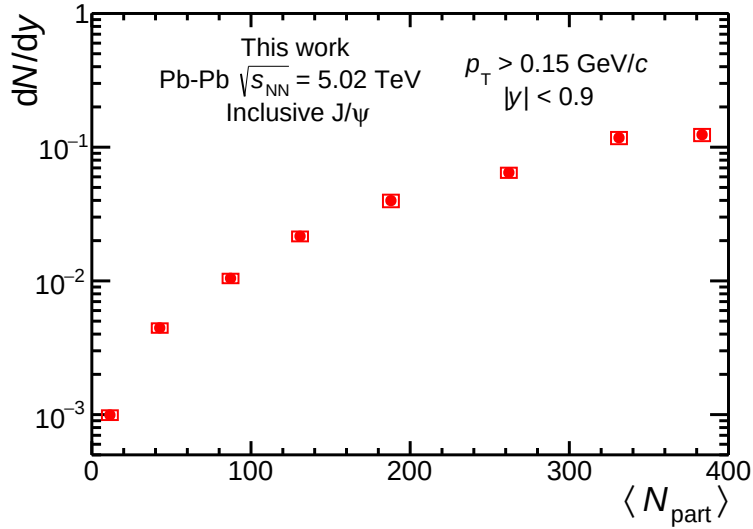
Figure 5.1: Inclusive J/\psi production yield in Pb–Pb collisions at \sqrt{s_{\text{NN}}} = 5.02 TeV as a function of the average number of participants \langle N_{\text{part}} \rangle . The values of \langle N_{\text{part}} \rangle are obtained for collisions in centrality classes (0–5%, 5–10%, 10–20%, 20–30%, 30–40%, 40–50%, 50–70%, 70–90%). The vertical error bars indicate statistical uncertainty and the boxes around the data points represent the systematic uncertainty.
