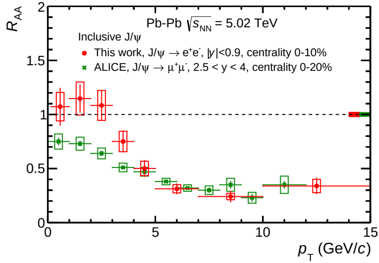
Figure 5.8: Inclusive J/\psi nuclear modification factor R_{AA} in the most central Pb–Pb collisions at \sqrt{s} = 5.02 TeV as a function of p_T at midrapidity ( |y| < 0.9 ) and forward rapidity ( 2.5 < y < 4.0 ) [173].
