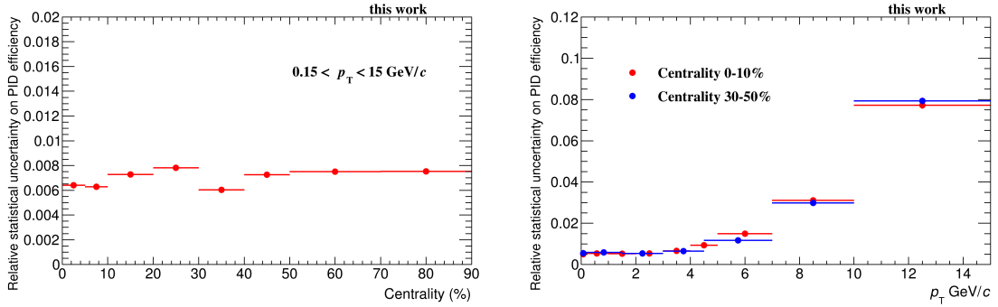
Figure 4.23: The systematic uncertainty from the statistical uncertainty on the leg PID efficiency as a function of centrality (left) and p_{\text{T}} for centralities 0–10% and 30–50% (right).
