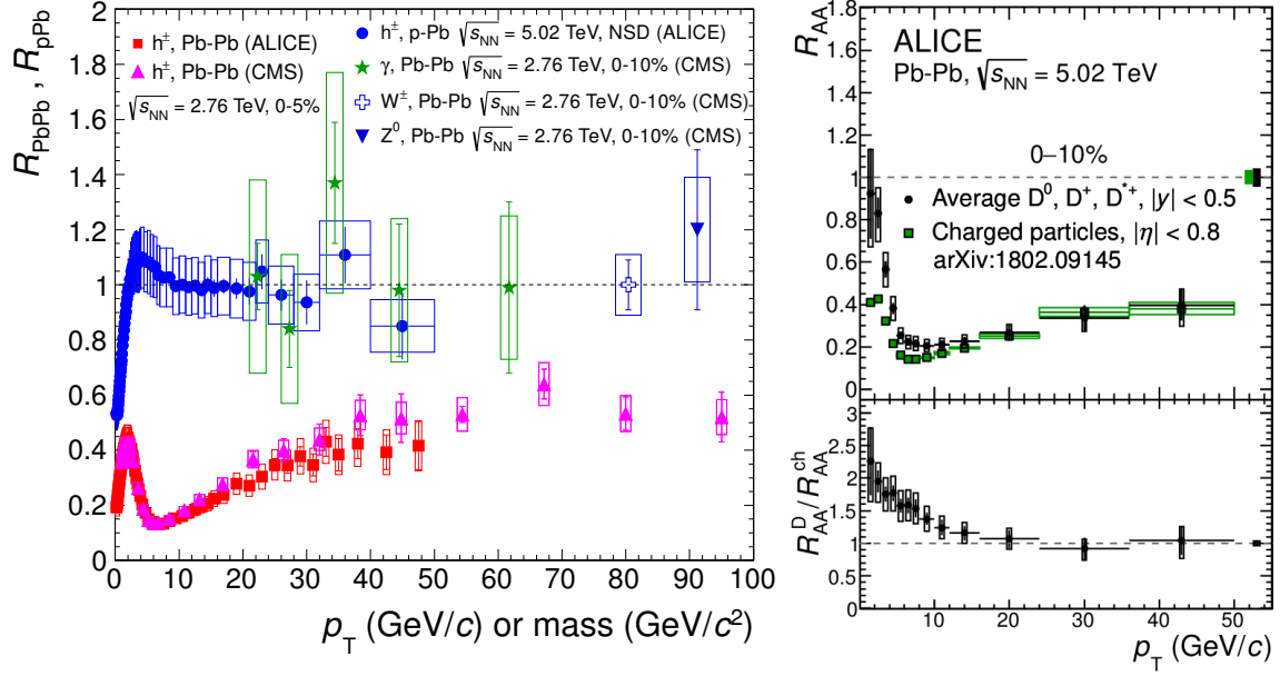
Figure 1.9: Left: Nuclear modification factors R_{pPb} in p-Pb collisions and R_{PbPb} in the most central Pb-Pb collisions as a function of transverse momentum p_T . The R_{PbPb} of charged particles [32, 33], direct photons [35], Z^0 bosons [37] and W^\pm bosons [36] is measured in Pb-Pb collisions at \sqrt{s_{NN}} = 2.76 TeV. The R_{pPb} of charged particles ( h^\pm ) in p-Pb collisions at 5.02 TeV [34] is compared to the R_{PbPb} . (Figure is taken from [34].) Right: Nuclear modification factors R_{PbPb} of prompt D^0 , D^+ and D^{*+} mesons and R_{PbPb} of charged particles [38] as a function of p_T measured in Pb-Pb collisions at \sqrt{s_{NN}} = 5.02 TeV. R_{PbPb} is shown in three centrality classes: 0–10% (left), 30–50% (middle) and 60–80% (right). (Figure is taken from [39].)
