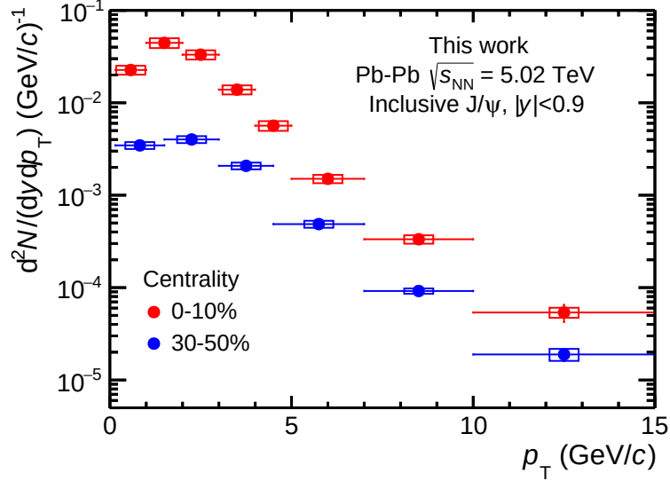
Figure 5.2: Transverse momentum dependence of the inclusive J/\psi production yields for the centrality classes 0–10% and 30–50%. The vertical error bars indicate statistical uncertainty and the boxes around the data points represent the systematic uncertainty.
