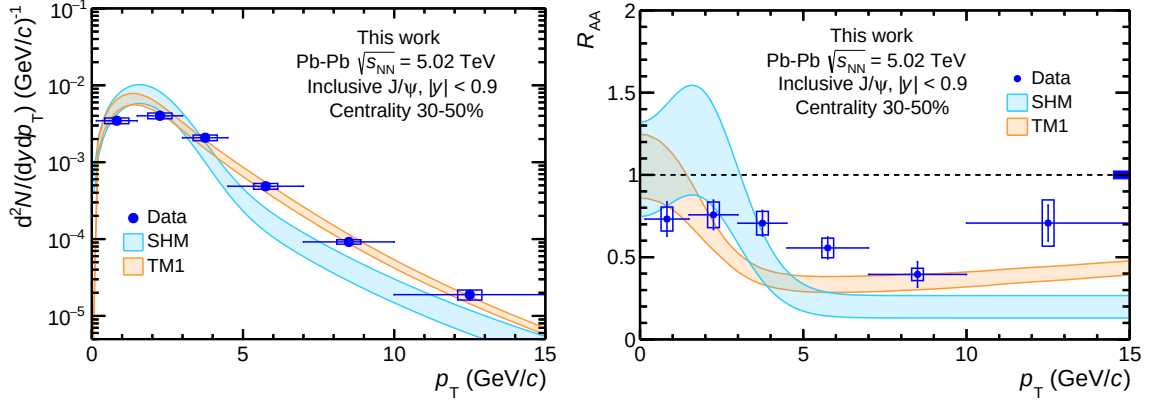
Figure 5.10: Inclusive J/\psi production yield (left) and R_{AA} (right) as a function of p_T in Pb-Pb collisions in the centrality class 30–50% compared to the model calculations of the SHM [101] and the TM1 [105].
