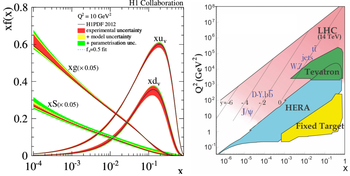
Figure 2.4: Left: Parton distribution functions for Q^2 = 10 \text{ GeV}^2 relevant for J/\psi -meson production at the LHC. (Figure is taken from [59].) Right: Regions of x and Q^2 studied by different collider and fixed-target experiments. (Figure is taken from [60].)
