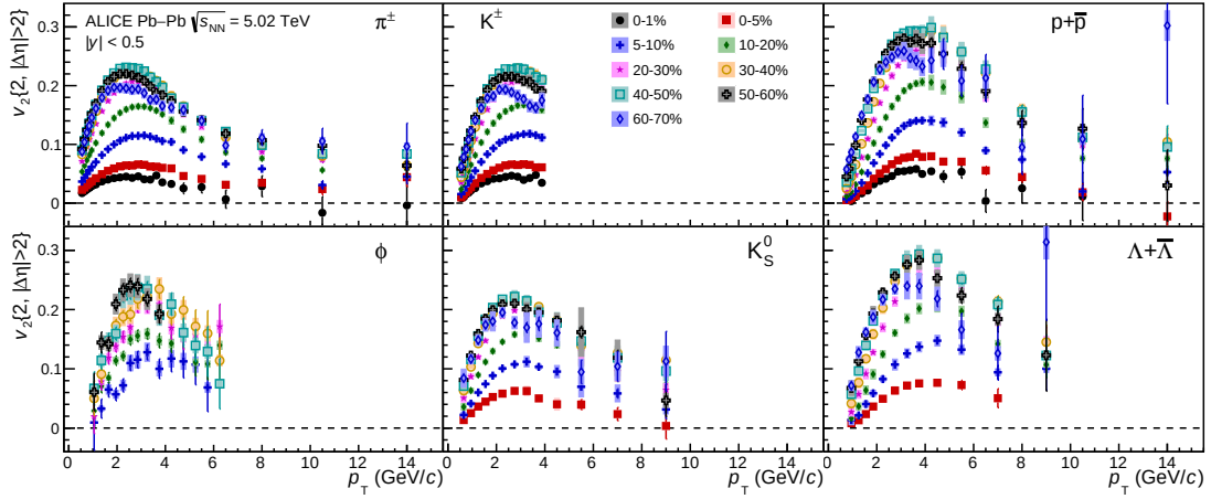
Figure 1.8: Elliptic flow coefficient v_2 as a function of transverse momentum p_T in different centrality classes for \pi^\pm , K^\pm , p + \bar{p} , \Lambda + \bar{\Lambda} , K_s^0 and the \phi meson. (Figure is taken from [27].)
