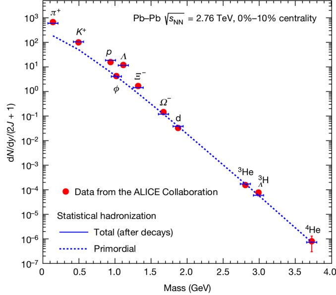
Figure 1.6: Yields of different hadron species measured by ALICE in the 10% most central Pb–Pb collisions at \sqrt{s_{NN}} = 2.76 TeV divided by the spin degeneracy factor. The yields are fitted by the Statistical Hadronization Model [23]. The result of the fit is shown as the dashed blue line. The total yields marked by the solid blue lines are obtained by adding contributions from the resonance decays. (Figure is taken from [24].)
