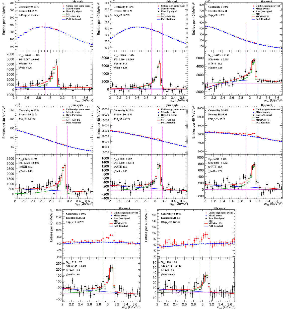
Figure 4.10: Invariant mass distribution of J/\psi candidates and background obtained by event mixing for centrality 0–10% and different p_T intervals are shown in the tops of the plots. The distribution of J/\psi candidates after subtraction of background modeled by event mixing is shown in the lower panels together with a fit function.
