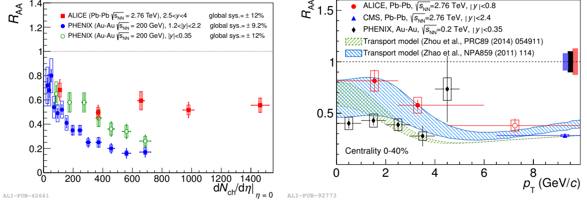
Figure 2.13: Left: Inclusive J/\psi R_{AA} at forward rapidity as a function of midrapidity charged-particle density measured by ALICE in Pb–Pb collisions at \sqrt{s_{NN}} = 2.76 TeV [109] compared to the PHENIX results in Au–Au collisions at 0.2 GeV at forward rapidity and midrapidity [96]. (Figure is taken from [109].) Right: Inclusive J/\psi R_{AA} at midrapidity in Pb–Pb collisions at \sqrt{s_{NN}} = 2.76 TeV as a function of transverse momentum p_T measured by ALICE [110] compared to PHENIX results for Au–Au collisions at 0.2 TeV [111], CMS results for Pb–Pb collisions at \sqrt{s_{NN}} = 2.76 TeV [112], and model predictions of Zhou et al. [106] and Rapp et al. [104, 113] (referred to as Zhao et al. in the figure). (Figure is taken from [110].)
