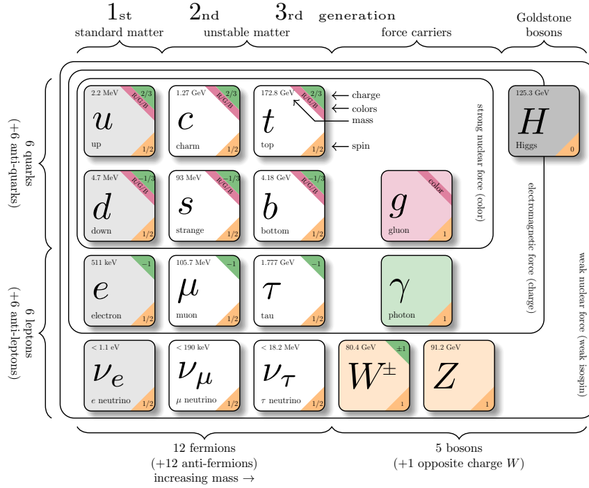
Figure 1.1: Elementary particles of the Standard Model. (The figure is taken from [2] and modified with values from [3].)
