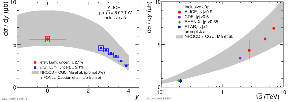
Figure 2.6: Left: Inclusive J/\psi cross section in pp collisions at 5.02 TeV as a function of rapidity measured by ALICE [55, 66]. Right: Inclusive J/\psi cross sections measured by ALICE [66, 76, 77], CDF [78], PHENIX [79] and prompt J/\psi cross section measured by STAR [80] at midrapidity as a function of collision energy. The measurements are compared to the LO NRQCD+CGC [71] prompt J/\psi calculations summed with FONLL predictions [72] for non-prompt J/\psi contribution. The figures are taken from [66].
