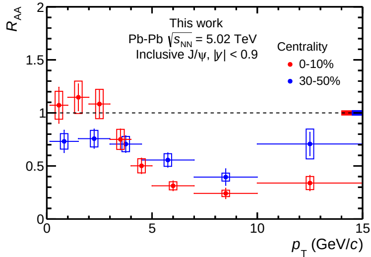
Figure 5.7: Inclusive J/\psi nuclear modification factor R_{AA} in Pb–Pb collisions at \sqrt{s_{NN}} = 5.02 TeV as a function of p_T in the centrality classes 0–10% and 30–50%. The vertical bars indicate the statistical uncertainty, whereas the boxes around the data points indicate the systematic uncertainty. In both cases, the uncertainties on the J/\psi production yield in Pb–Pb collisions and the pp reference are added. The box around unity represents the global uncertainty originating from the integrated luminosity of the pp data sample and the mean nuclear overlap function \langle T_{AA} \rangle .
