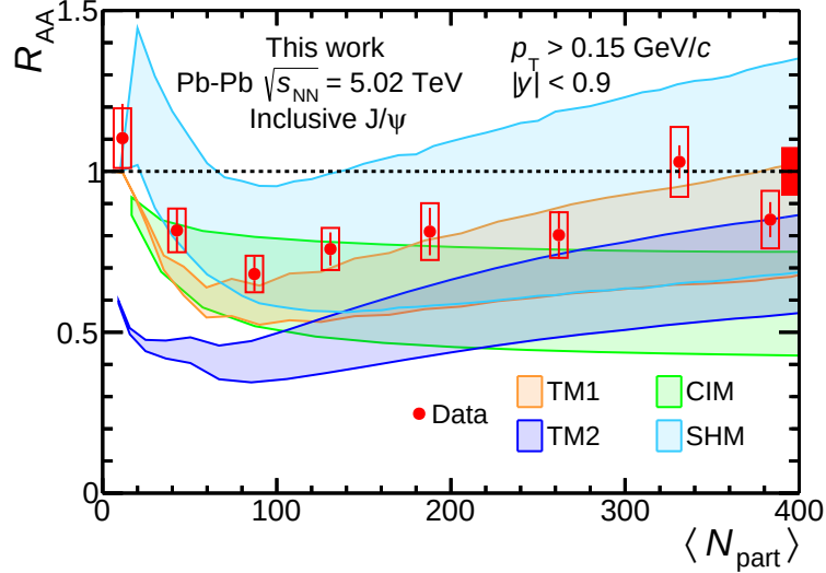
Figure 5.6: Inclusive J/\psi nuclear modification factor R_{AA} in Pb–Pb collisions at \sqrt{s_{NN}} = 5.02 TeV compared to the model calculations of the comover interaction model (CIM) [108], the statistical hadronization model (SHM) [101] and two transport models TM1 [105] and TM2 [106].
