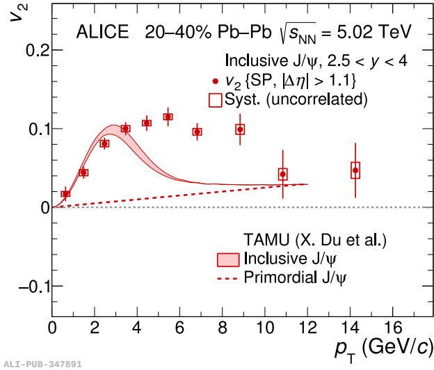
Figure 2.14: Inclusive J/ψ elliptic flow coefficient v_2 as a function of transverse momentum at forward rapidity measured by ALICE in Pb–Pb collisions at \sqrt{s_{NN}} = 5.02 TeV with centrality 20–40% [114] compared to the predictions from the transport model of Rapp et al. [105] (referred to as X. Du et al. in the figure). (Figure is taken from [114].)
