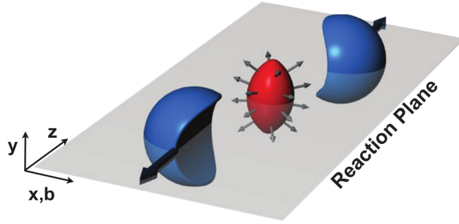
Figure 1.7: An illustration of a semi-central heavy-ion collision. The almond-shaped participant zone is shown in red color, while spectator zones in blue color. Pressure gradients are represented by arrows. The reaction plane corresponds to the xz -plane. (Figure is taken from [25].)
