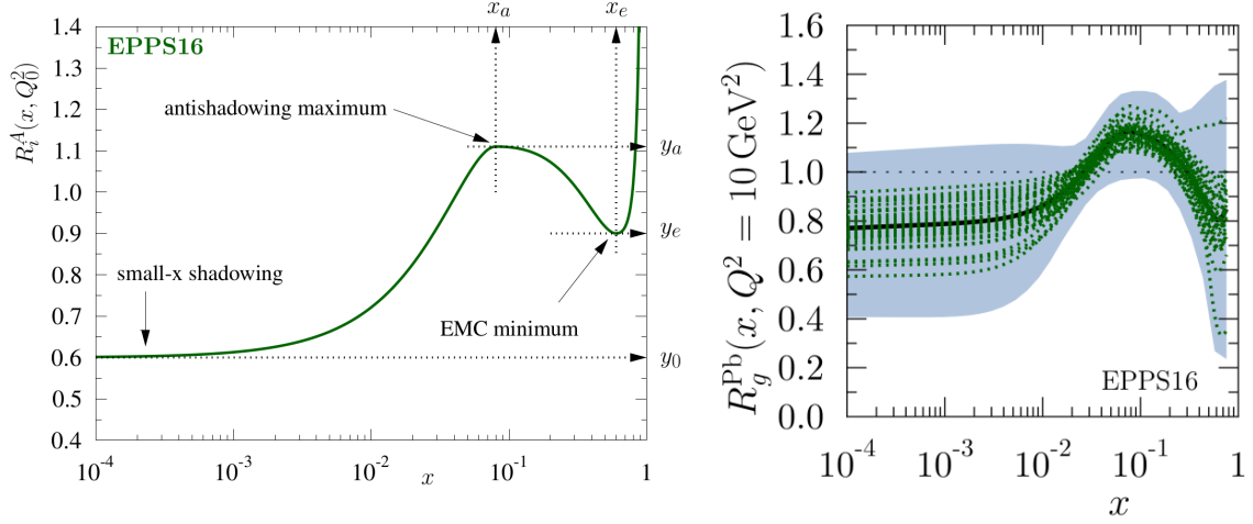
Figure 2.7: Left: Illustration of the fit function of R_i^A(x, Q^2) used in the extraction of nPDFs. Right: Gluon nuclear modification function R_g^{Pb}(x, Q^2 = 10 \text{ GeV}^2) for lead nuclei. The figures are taken from [81].
