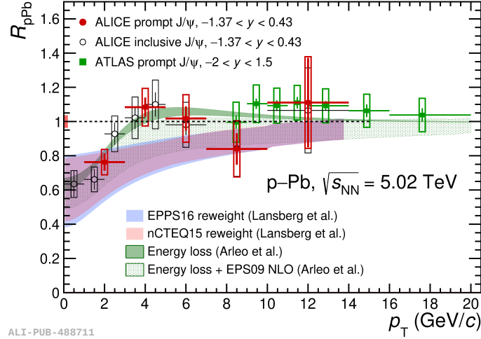
Figure 2.8: R_{pPb} of prompt and inclusive J/\psi as a function of transverse momentum measured by ALICE compared to the ATLAS measurement of prompt J/\psi [86]. The experimental results are compared to theoretical predictions [84, 87] which are shown as shaded areas. The figure is taken from [56].
