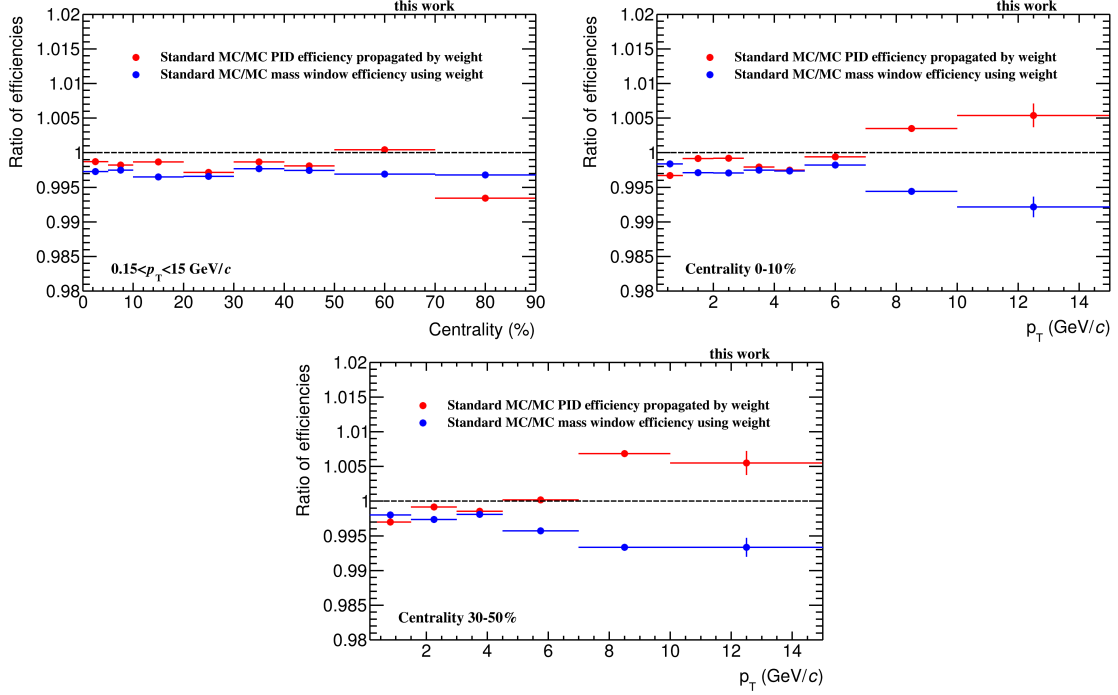
Figure 4.24: Ratios of MC PID and mass window efficiencies: the ratio of the standard MC J/\psi PID efficiency to the J/\psi PID efficiency propagated via the efficiency weight using the MC leg PID efficiency and the ratio of mass window efficiency after applying PID selections in the MC simulation to the efficiency weight. The ratios are shown as a function of centrality (top left) and p_T for centrality 0–10% (top right) and centrality 30–50% (bottom).
