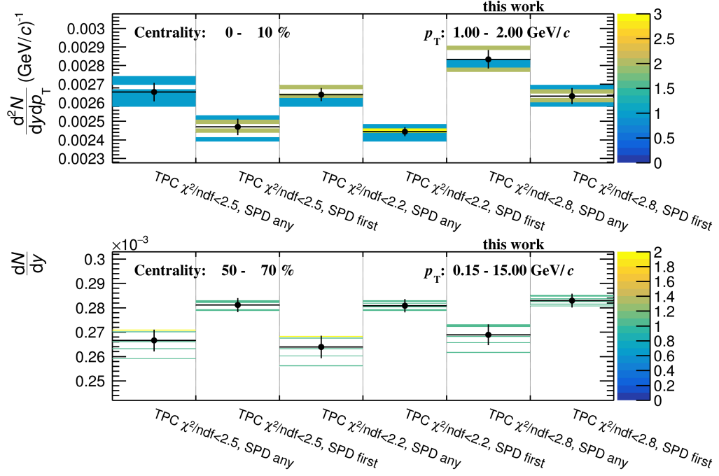
Figure 4.29: Examples of corrected J/\psi yield for simultaneous fit range and tracking cut variations and means of cases with different fit ranges for one set of tracking selections shown in black. Error bar on means is calculated as RMS with respect to the case of standard fit range. Color scale corresponds to the number of the variations falling into a bin of corrected J/\psi yield.
