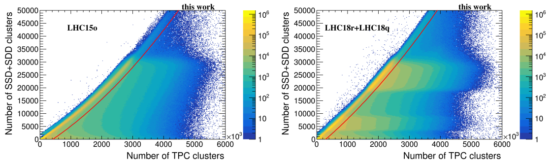
Figure 4.2: The sum of the numbers of SSD and SDD clusters versus the number of TPC clusters. The red line corresponds to the boarder between events that are accepted and rejected events affected by the pile-up. Left: 2015 data set LHC15o. Right: 2018 data sets LHC18q and LHC18r.
