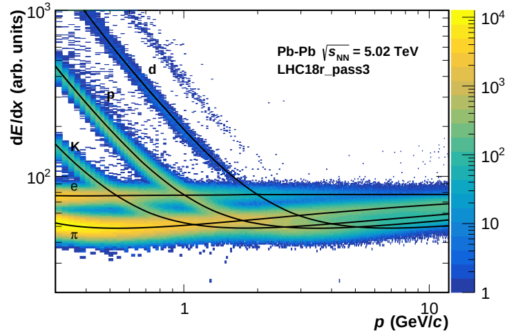
Figure 3.8: Specific energy loss of charged particles, dE/dx , in the TPC as a function of the particle momentum. Expected values for different particle species are shown as black lines. (Figure by Michael Ciupek.)
