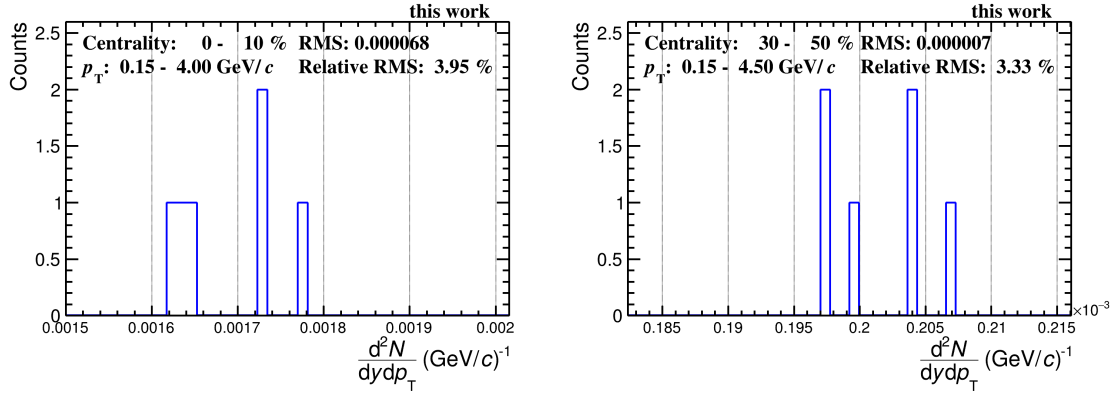
Figure 4.22: Distribution of means over signal extraction variations for a given tracking selection used for the estimation of systematic uncertainty originating from imperfect MC description of tracking selection criteria. Each entry corresponds to one tracking selection criterion.
