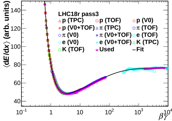
Figure 3.9: Bethe-Bloch fit to the means of the TPC dE/dx distributions of clean samples. The samples of different particle species are obtained using various detector PID signals or decay products of clean V^0 samples. (Figure by Michael Ciupek.)
