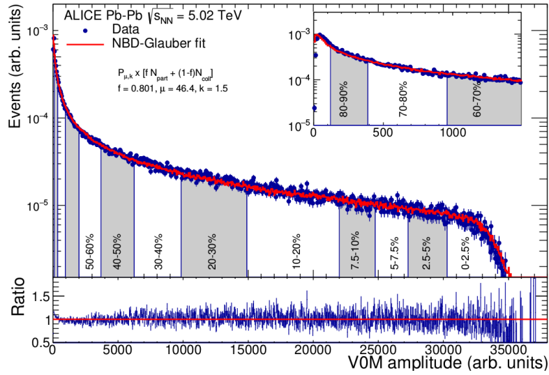
Figure 3.10: The distribution of amplitudes from the V0 detector for Pb–Pb collisions at \sqrt{s_{\text{NN}}} = 5.02 TeV. The red line represents the fit of data points by the Glauber model. The ratio of the data to the fit is shown in the lower panel of the figure. A zoom into the interval corresponding to the peripheral events is shown in the right top corner.
