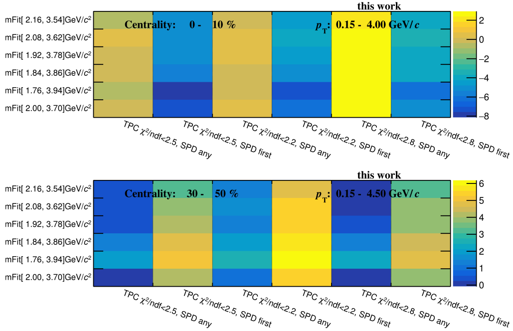
Figure 4.21: Examples of deviations in percent shown in color from the standard case for the simultaneous variations of the tracking selection criteria and fit range.
