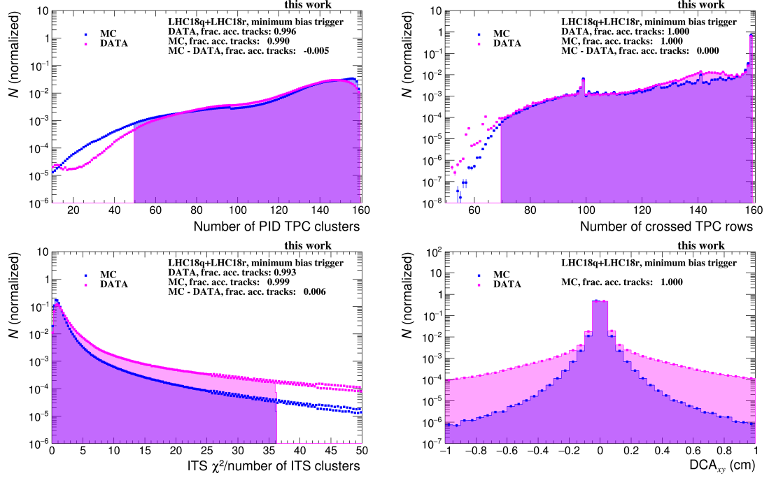
Figure 4.5: Distributions of different tracking variables in MB collisions with centrality 0–90% and fractions of accepted tracks in the data, MC and their difference. The shaded areas correspond to accepted tracks.
