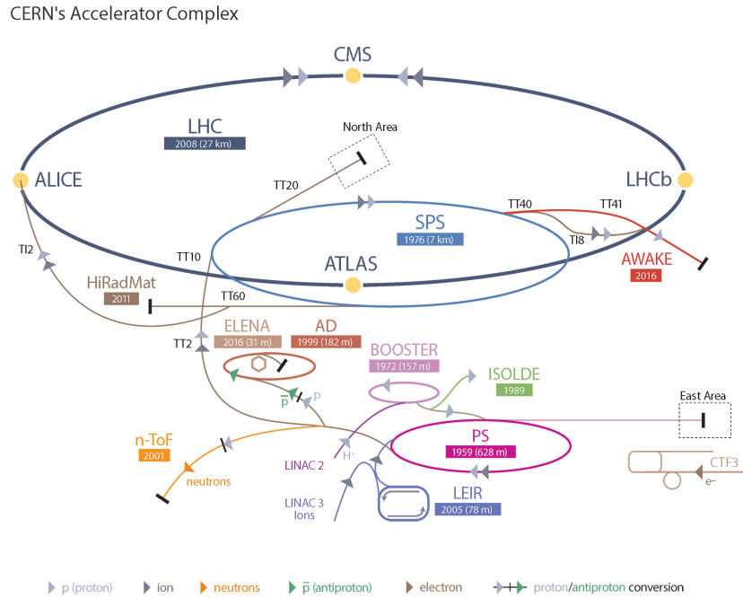
Figure 3.1: CERN's accelerator complex. The path of protons starting in LINAC 2 is marked by light gray arrows and the path of ions starting in LINAC 3 by dark gray arrows. Protons and ions travel on same trajectories since they get to the PS. (Figure is taken from [115].)
