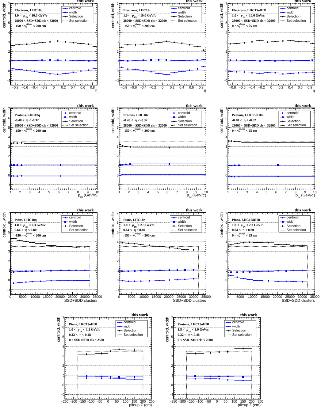
Figure 4.7: Examples of centroids and widths as functions of \eta , p_{\text{IN}} , the number of SSD+SDD clusters and v_z^{\text{pileup}} are shown in the blue color. Black dashed lines correspond to the set selections listed in Table 4.2. The black markers represent estimates of the effective selections that would be applied if no additional calibration of n\sigma_i were applied.
