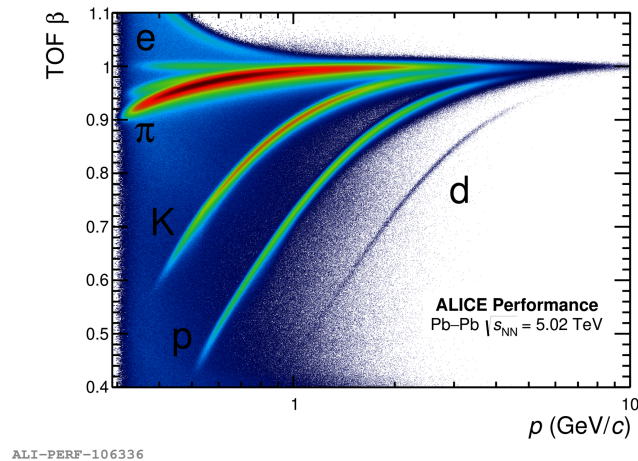
Figure 3.5: Distribution of particle velocity \beta as a function of momentum. (Figure is taken from [135].)
