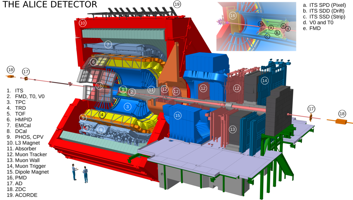
Figure 3.3: Sketch of the ALICE setup and its detector subsystems. Different detectors are indicated by numbers. (Figure is taken from [127].)
