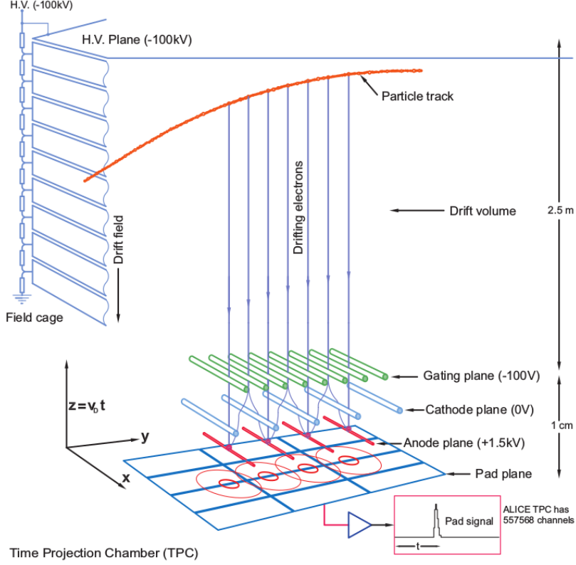
Figure 3.4: Illustration of the TPC working principle. (Figure is taken from [130].)
