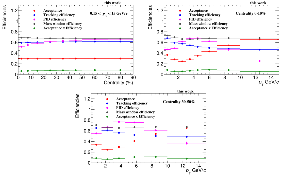
Figure 4.12: J/\psi acceptance and efficiencies as a function of centrality (top left) and p_T for centrality 0–10% (top right) and 30–50% (bottom).
