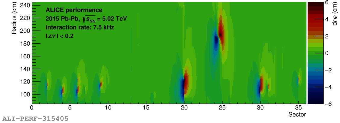
Figure 3.7: The radial space-charge distortions dr\varphi in 2015 Pb–Pb data as a function of the radius and the TPC sector coordinate for the largest drift distances ( |z/r| < 0.2 ). (Figure is taken from [140].)
