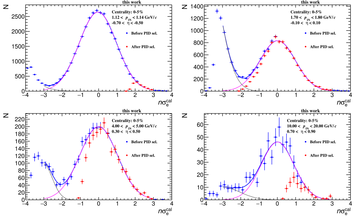
Figure 4.14: Examples of n\sigma_e^{\text{cal}} distributions before (blue) and after (red) applying the PID selection criteria. Function consisting of two Gaussian functions used to describe n\sigma_e^{\text{cal}} distribution is shown in blue color, the component describing the pion contamination in gray color and the electron component in magenta color.
