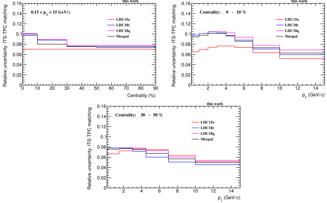
Figure 4.18: Systematic uncertainty originating from the uncertainty on the ITS-TPC matching efficiency as a function of the centrality (top left) and p_T for centrality 0–10% (top right) and 30–50% (bottom).
