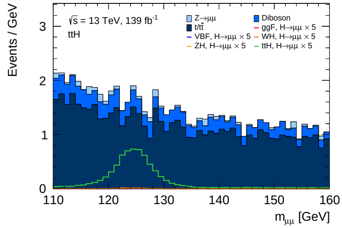
Figure 4.41 The dimuon invariant mass distribution for the \text{ttH} category.
