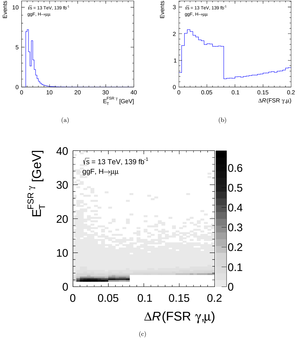
Figure 4.31 The distributions of E_T and \Delta R_{\gamma, \mu} for fake FSR photon candidates.
