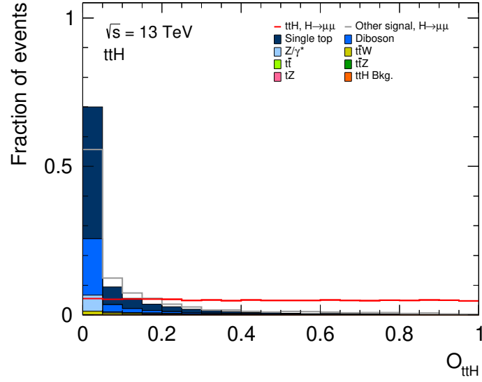
Figure 4.40 The BDT output score of \text{ttH} classifier O_{\text{ttH}} for MC samples.
