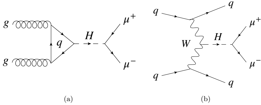
Figure 4.1 Feynman diagrams of the H \rightarrow \mu\mu decay in the ggF (a) and VBF (b) processes. In the VBF process, there are two jets in addition to the opposite-charge muon pair in the final state.
