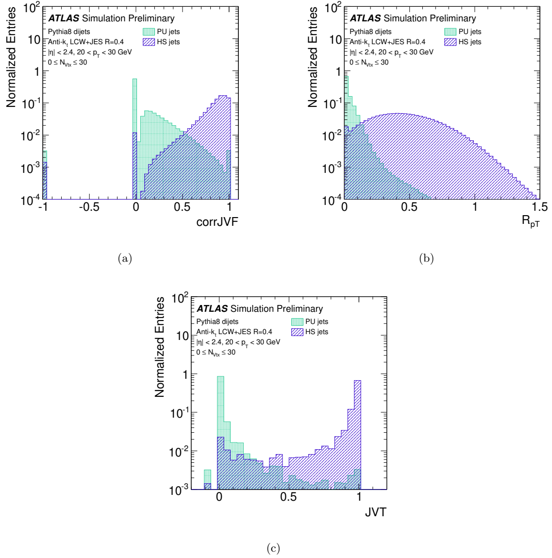
Figure 4.20 The distributions of corrJVF (a), R_{pT} (b), and JVT score (c) for the jets from the primary vertex (blue) and pile-up jets (green). The entries with corrJVF = -1 correspond to jets with no associated tracks.
