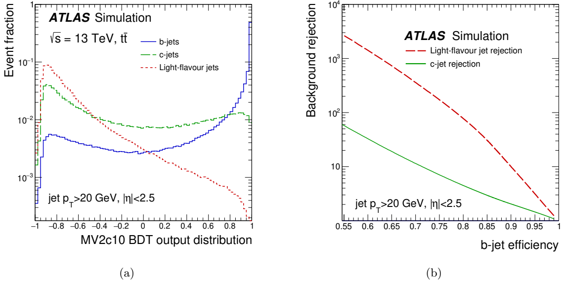
Figure 4.21 The b -tagging performance by the MV2c10 algorithm [78]. The MV2c10 output scores for b -jets (blue), c -jets (green) and light-flavor jets (red) are shown in (a). The rejections of c -jet (green) and light-flavor jet (red) as a function of the b -jet efficiency of the MV2c10 algorithm are shown in (b). These are evaluated using t\bar{t} simulation events.
