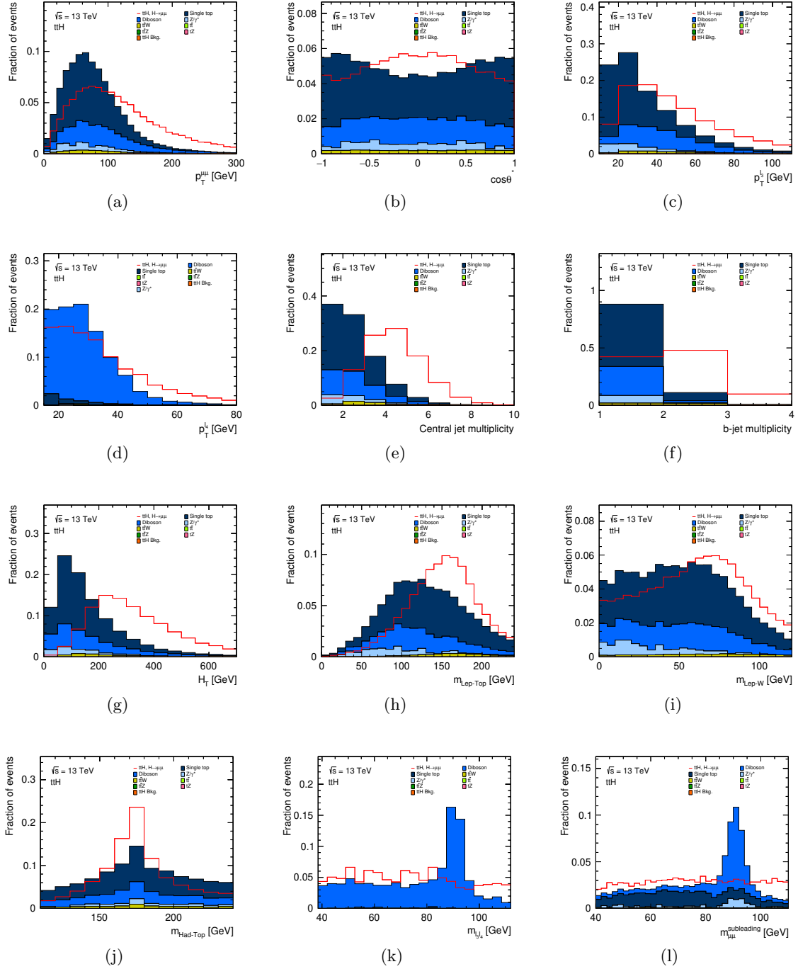
Figure 4.39 The BDT input variables for ttH classifier. The distributions are shown for MC samples.
