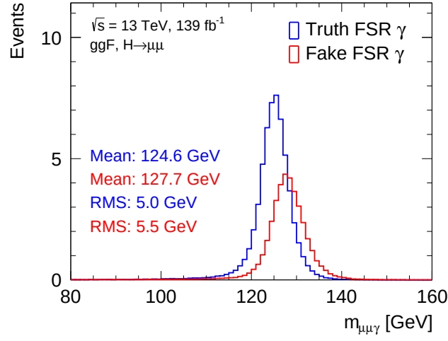
Figure 4.32 Invariant mass distributions after the FSR recovery for the events with the FSR candidate matched to the truth-level FSR (blue) and for the events with the fake FSR candidate (red).
