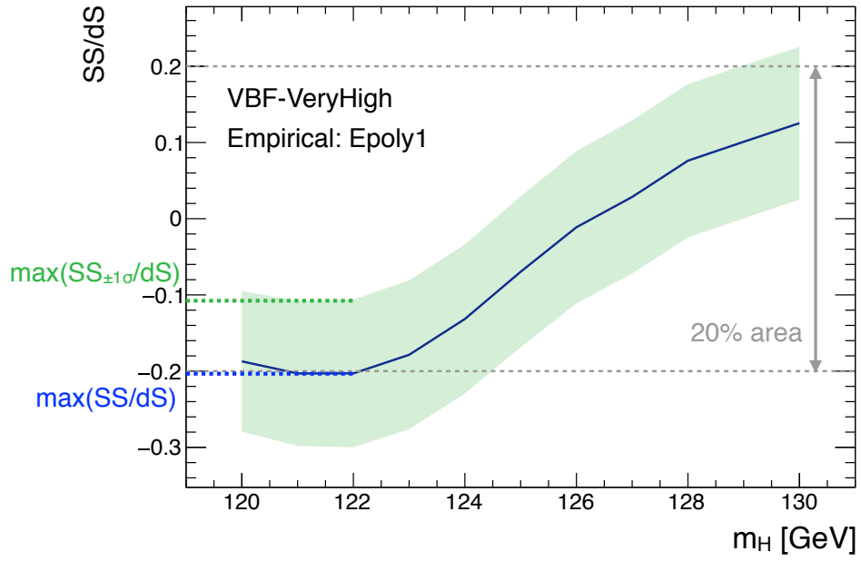
Figure 4.54 The spurious signal relative to its uncertainty SS/\delta S as a function of the dimuon invariant mass. The figure is shown for the VBF-VeryHigh category. The value of |\max(SS_{\pm 1\sigma}/\delta S)| is required to be smaller than 20%.
