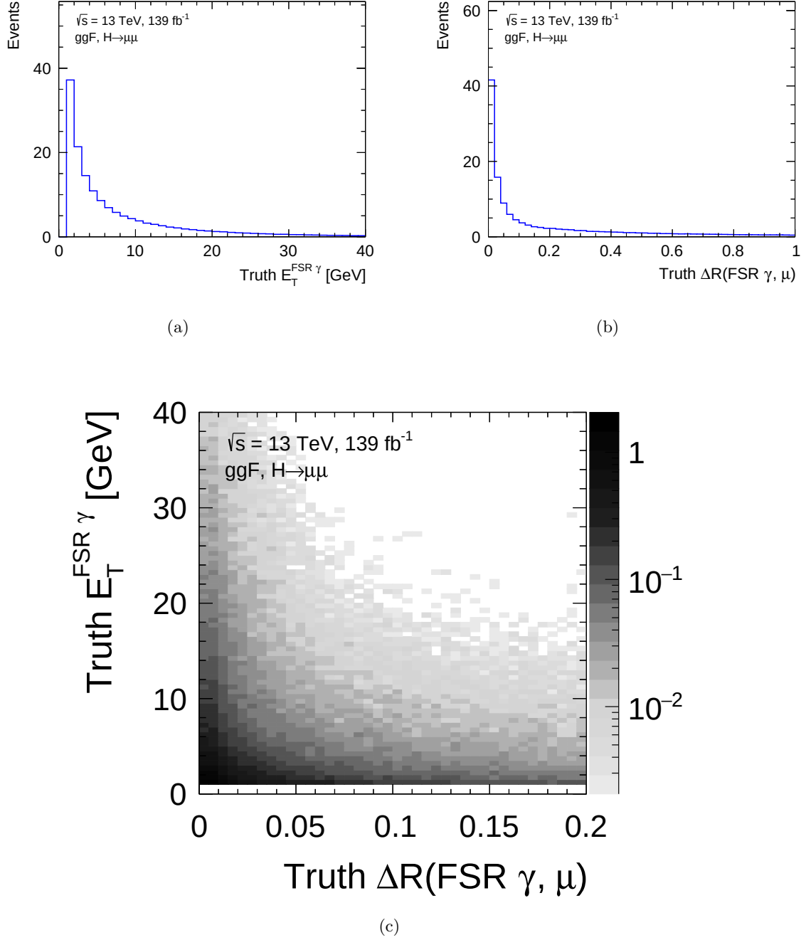
Figure 4.25 The distributions of E_T and \Delta R_{\gamma,\mu} for truth-level FSR photons.
