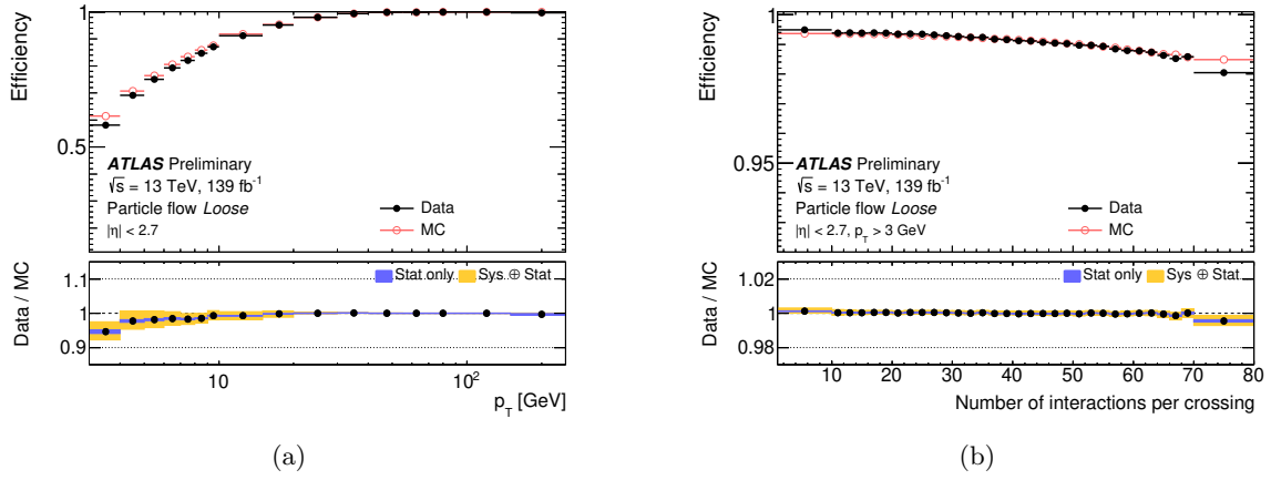
Figure 4.10 The muon isolation efficiencies for the WP used in this analysis. These are measured in Z \rightarrow \mu\mu events for muons with p_T > 3 GeV as a function of p_T (a) and the number of interactions per bunch crossing (b).
