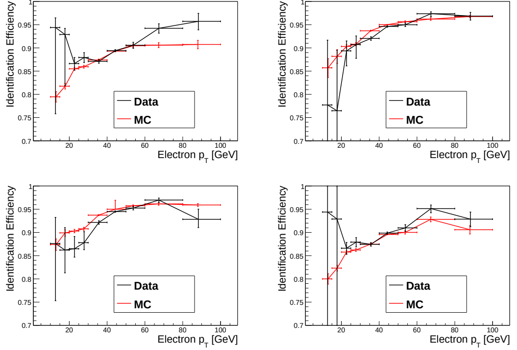
Figure 7.8: Identification efficiency \epsilon_{ID}^e for electrons from the tag & probe method for different \eta -regions compared to MC simulation. The bin edges of the \eta -ranges are top left to right: -2.5, -1.2, 0 and bottom left to right: 0, 1.2, 2.5.
