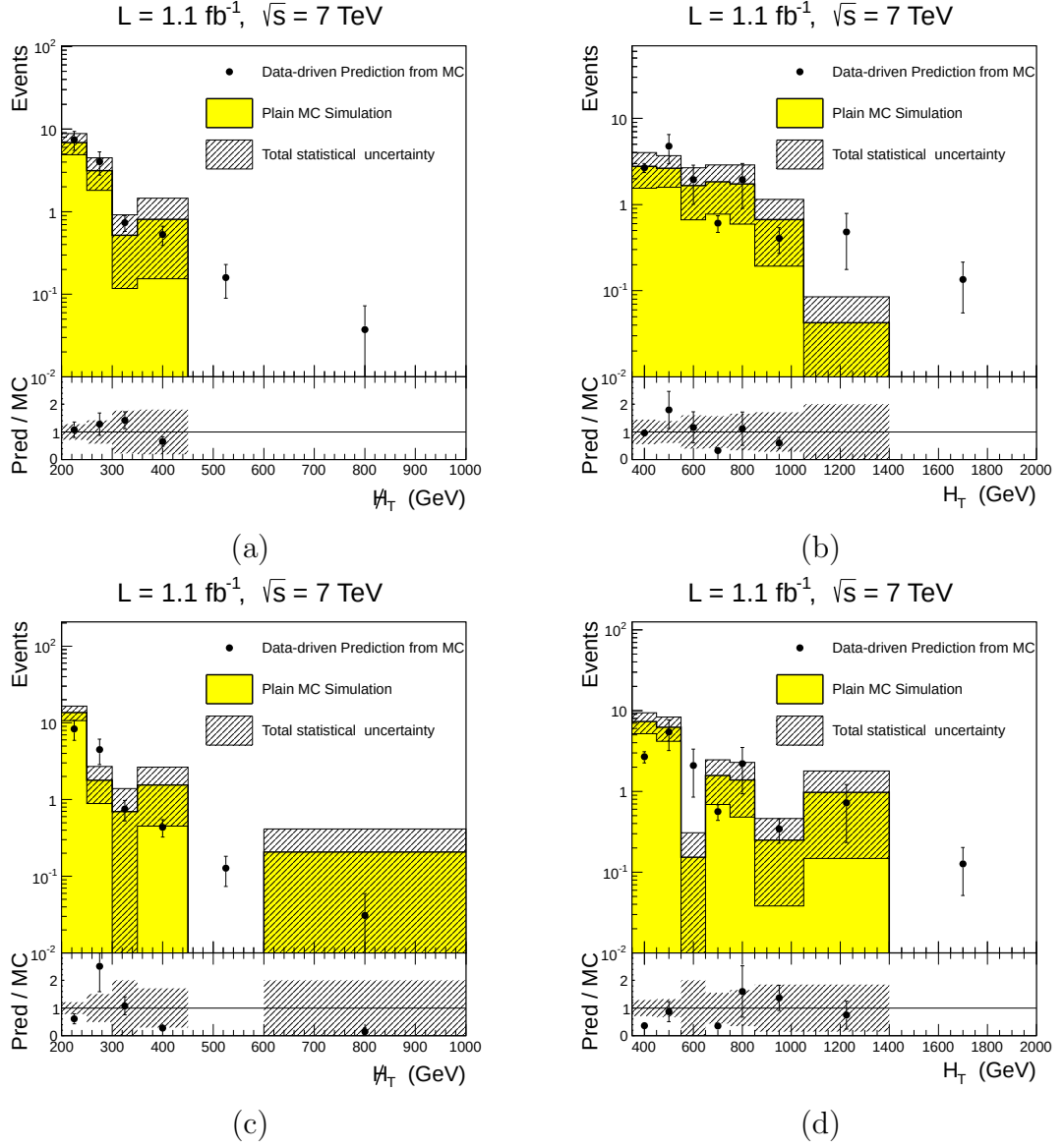
Figure A.3: Comparison of the kinematic properties of the plain W + \text{jet} MC simulation and the prediction on the same sample of identified but non-isolated leptons, for electrons (upper two plots) and muons (lower two plots). The shown variables are M_{HT} (left) and H_T (right)
