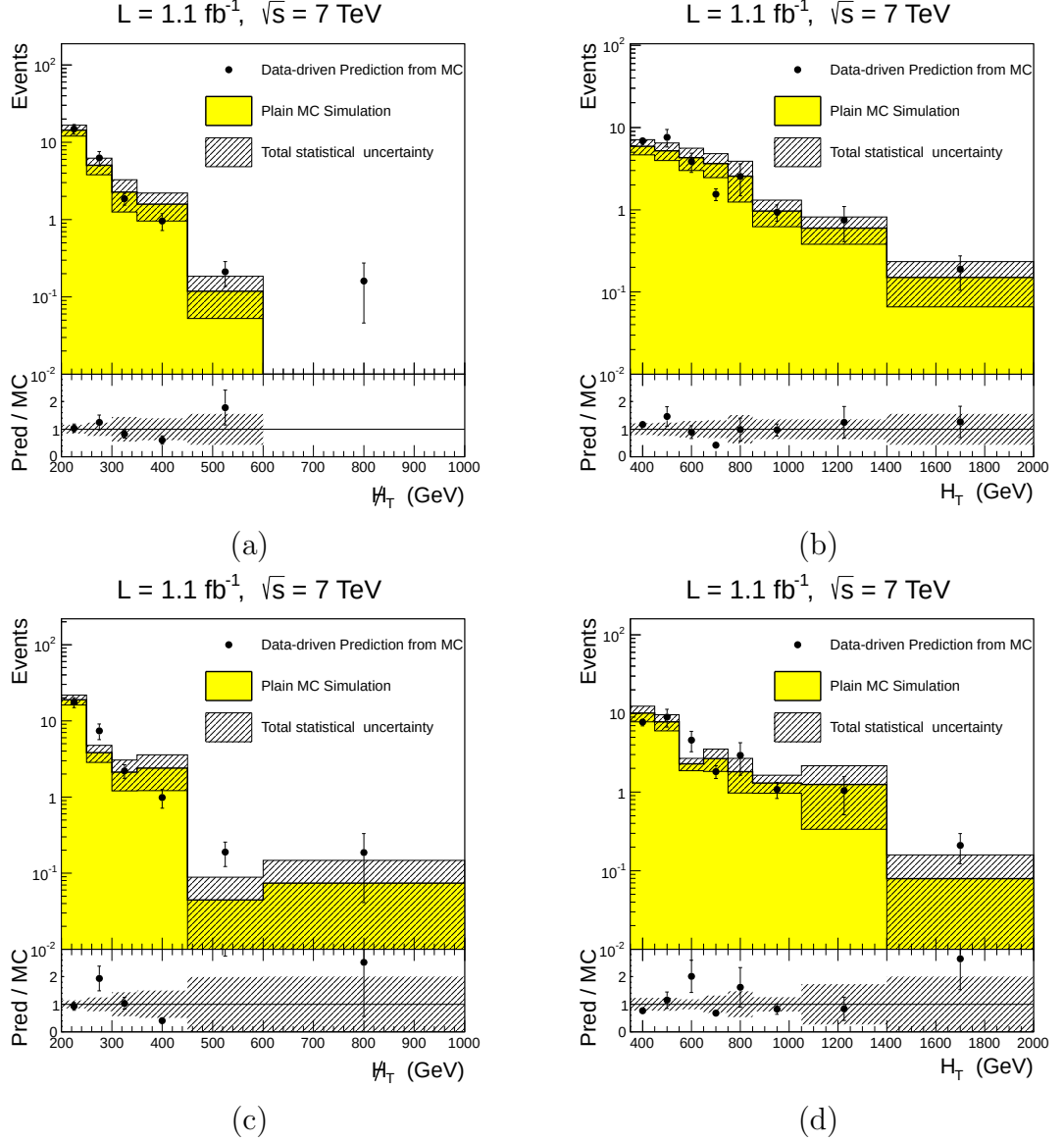
Figure 7.12: Comparison of the kinematic properties of the plain MC simulation and the prediction on the same sample of identified but non-isolated leptons from t\bar{t} and W + \text{jet} channel combined on MC, for electrons (upper two plots) and muons (lower two plots). The shown variables are M_{HT} (left) and H_T (right)
