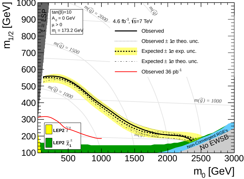
Figure 8.7: Limits on the cMSSM with the combination of several exclusive search regions on 4.65\text{fb}^{-1} .
