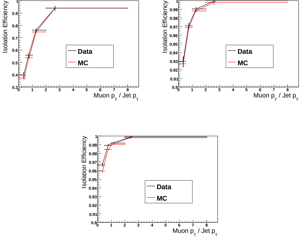
Figure 7.9: Isolation efficiency \epsilon_{Iso}^\mu for muons from the tag & probe method for different \Delta R -regions as function of p_T^\mu/p_T^{\text{closest jet}} compared to MC simulation. The bin edges of the \Delta R -ranges are for the top left to right: 0, 0.5, 1.0 and on the bottom 1.0 and 5.0.
