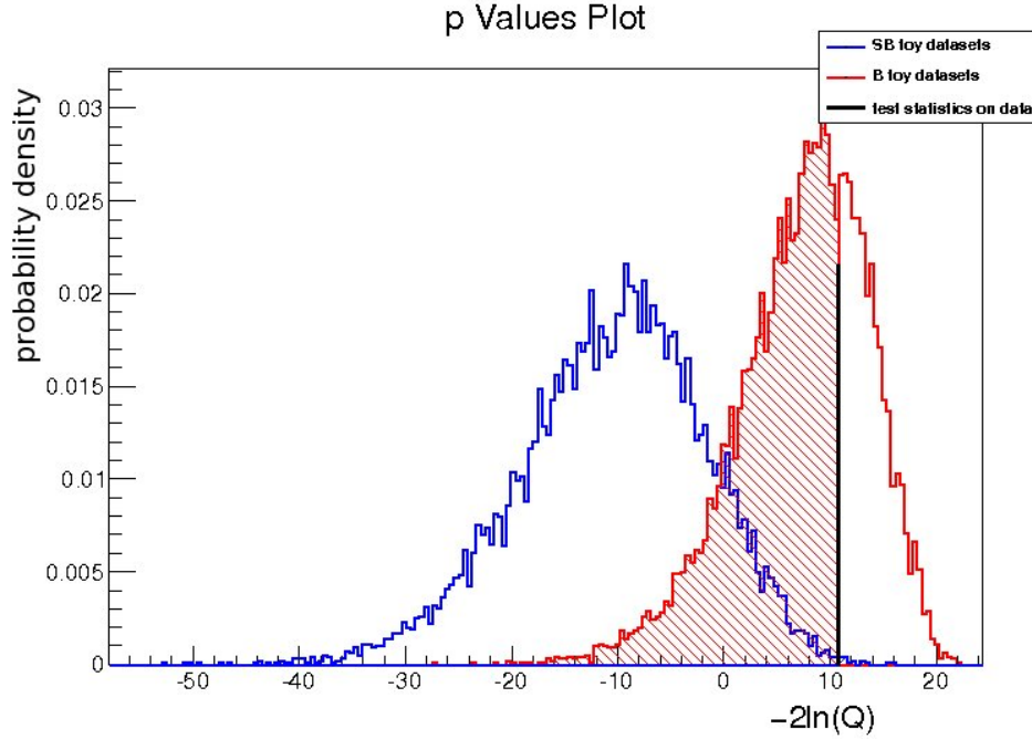
Figure 8.1: Test statistics shown as -2 \ln(Q) for an example susy point ( m_0 = 300 , m_{1/2} = 500 ). The red plot shows the distribution with data from a background-only toy dataset and the blue plots shows the distribution with data from a signal-plus-background toy dataset. The curves are normalised to the integral of one. The shaded area of the red plot corresponds to 1 - CL_b , the small shaded area under the blue graph on the right of the Q value found in data corresponds to CL_{s+b}
