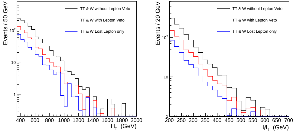
Figure 7.2: The plots show the H_T (left) and H_{TT} (right) distribution of the t\bar{t} and W + \text{jet} background before and after the lepton veto and the contribution of the "lost lepton" background for the baseline selection.
