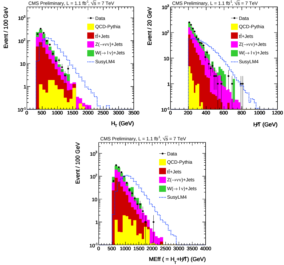
Figure 6.2: Comparison between data and MC after baseline selection. The plots show the H_T (left) and H_T (right) and effective mass defined as sum of H_T and H_T distribution (bottom). These plots are taken from [47].
