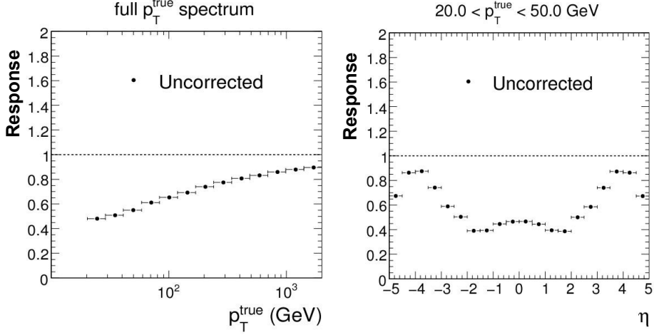
Figure 5.1: Jet response as a function of p_T^{\text{truth}} (left) and \eta^{\text{truth}} (right) for uncorrected jets.
