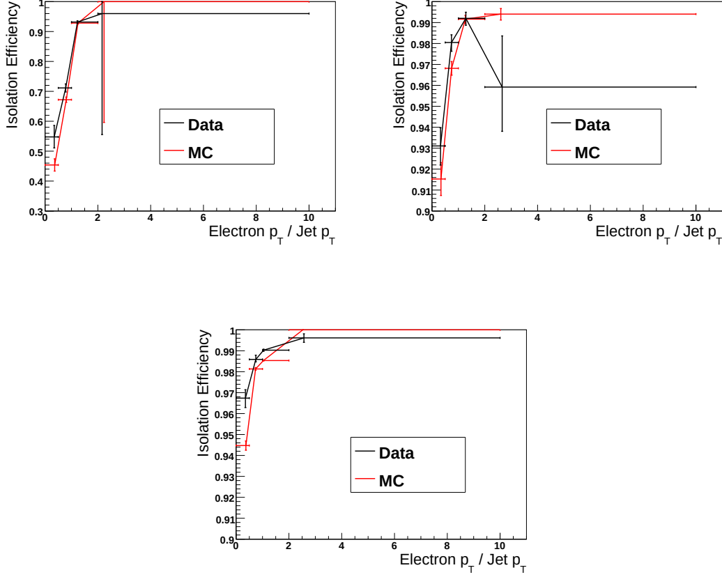
Figure 7.10: Isolation efficiency \epsilon_{Iso}^e for electrons from the tag & probe method for different \Delta R -regions as function of p_T^e / p_T^{\text{closest jet}} compared to MC simulation. The bin edges of the \Delta R -ranges are for the top left to right: 0, 0.5, 1.0 and for the bottom 1.0 and 5.0.
