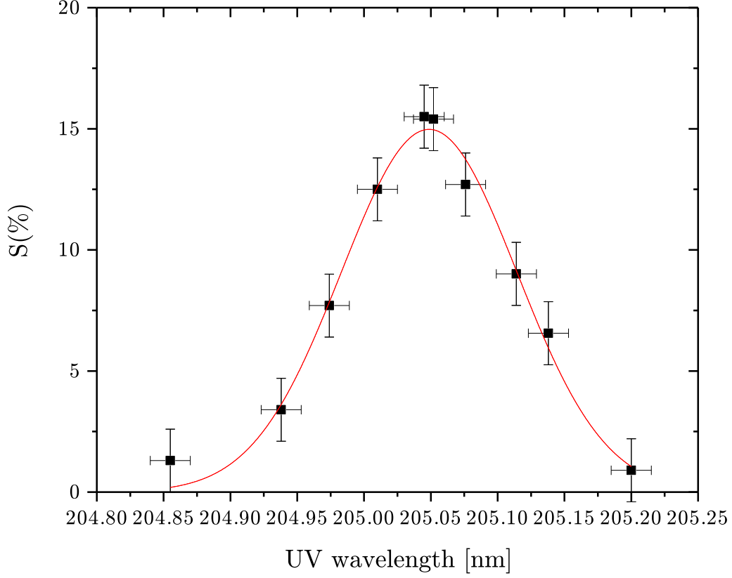
Figure 4.15: The S(\%) parameter as a function of the UV wavelength, giving the linewidth of the 1^3\text{S}-3^3\text{P} transition. All these measurements were done with a UV laser energy of 60\ \mu\text{J} and an IR laser energy of 55\ \text{mJ} . The excited fraction reaches a maximum close to the predicted resonant wavelength of 205.0474\ \text{nm} , and decreases when the wavelength deviates from this wavelength. The solid curve is a Gaussian distribution fitted to the data. Each data point is an average of 15 lifetime measurements, where the error bars of the S(\%) parameter is calculated from the standard deviation of these measurements. The error bars of the UV wavelength result from a variation in the laser output.
