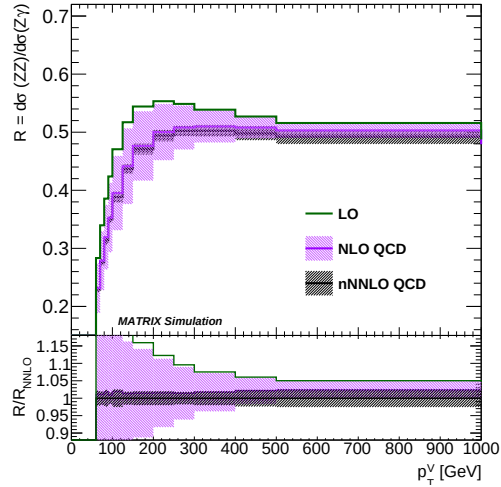
Figure 36: Ratio at the three different orders LO (green), NLO (purple), nNNLO (gray). The bands shown correspond to the QCD uncertainties ( \delta^{scale}, \delta^{shape}, \delta^{HO} ) added in quadrature. For the LO case only \delta^{scale}, \delta^{shape} are considered. The bottom frame shows the ratios normalised to the nNNLO prediction.
