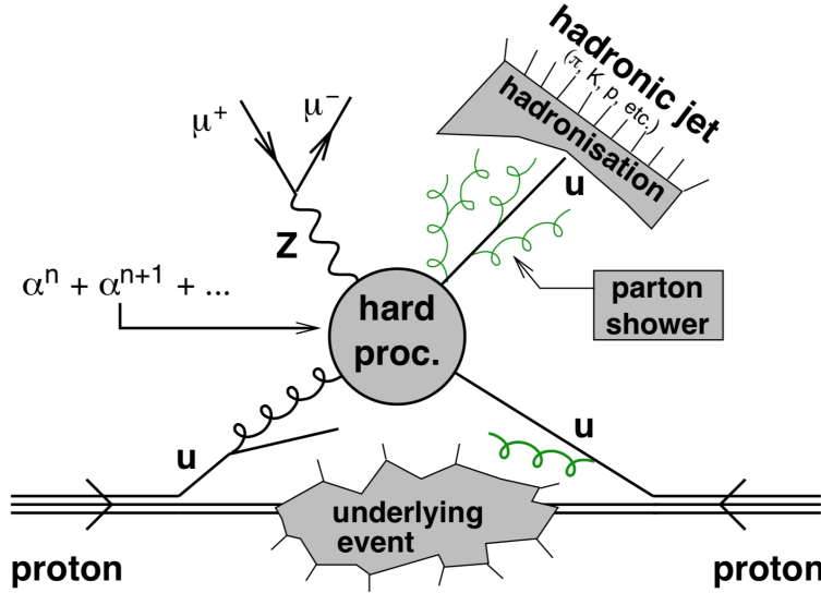
Figure 5: Sketch of a proton-proton collision. Figure taken from [41].
