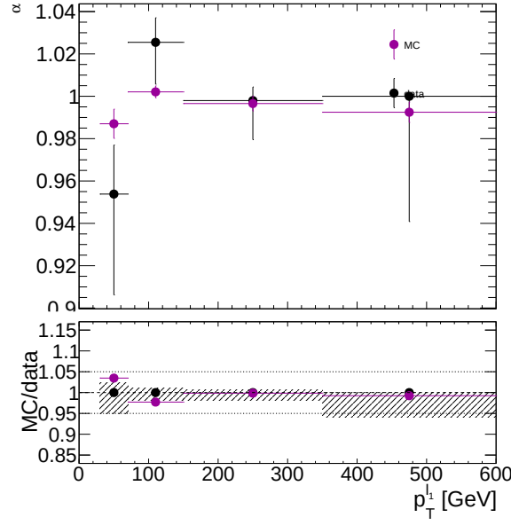
Figure 56: Trigger efficiency correction \alpha calculated for data (black) and MC (purple). MC includes: t\bar{t}, Wt, Z(\rightarrow \tau\tau) + \text{jets}, VV, VVV . The bottom frame shows the \alpha values normalised to data. The uncertainties are statistical only.
