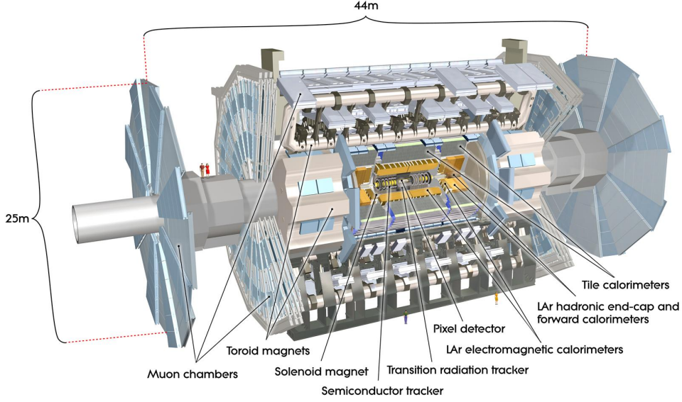
Figure 12: View of the ATLAS detector and subdetectors. Figure taken from [58].
