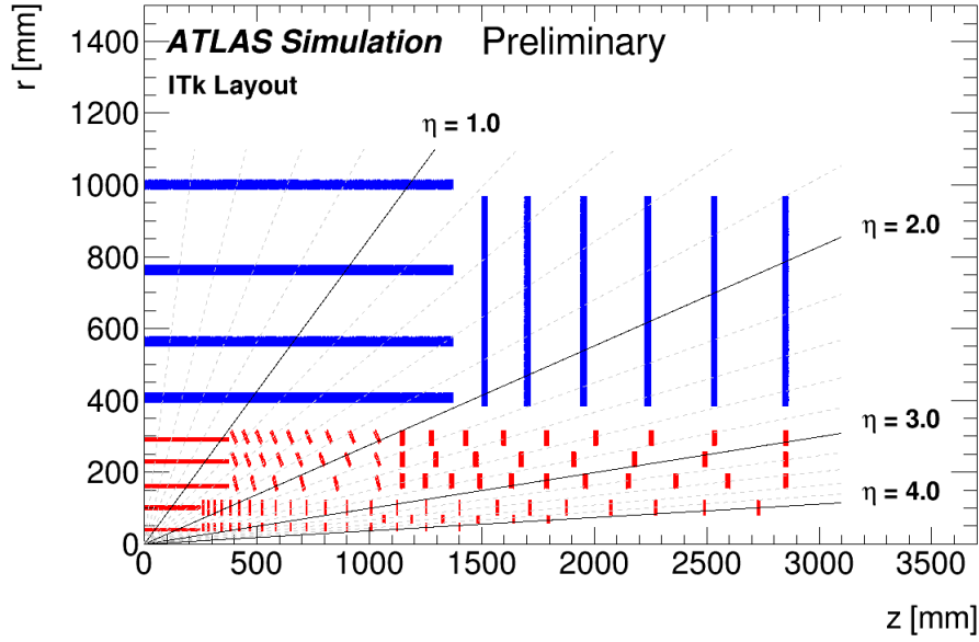
Figure 17: ATLAS ITk layout from [61].
