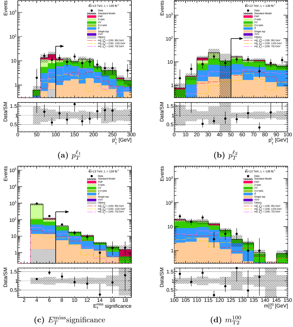
Figure 47: Plots of the most sensitive variables used in the analysis for the main background and for three benchmark signal points ( m(\tilde{\ell}, \tilde{\chi}_1^0) = (100, 70), (150, 110), (150, 90) GeV), after all the cuts described in Table 12 (SR 1-jet), except the cut on the variable shown in the plot. The uncertainties shown are statistical only. In the bottom frame of each plot the data to MC ratio is shown.
