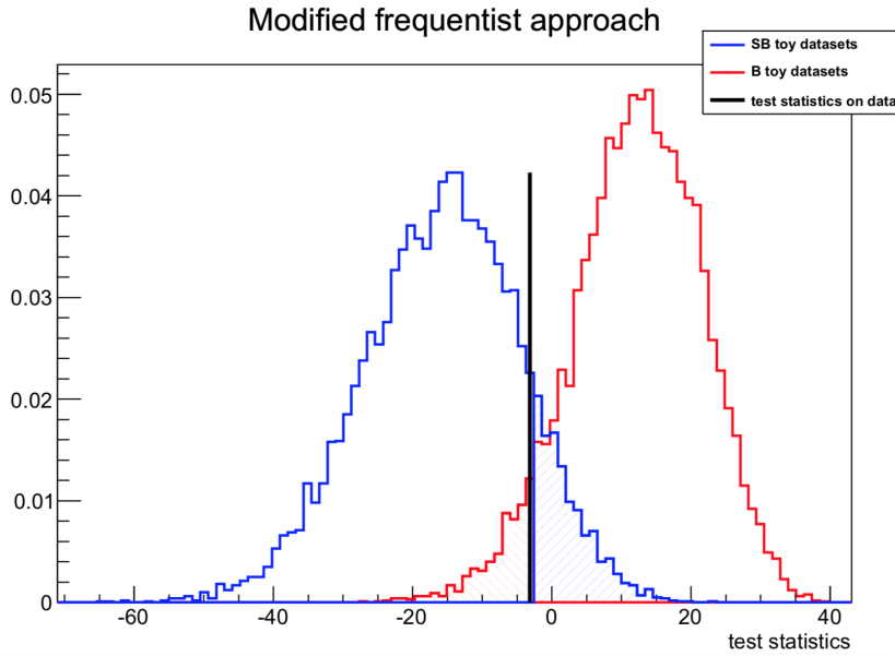
Figure 86: Example distribution of the test statistic t_\mu = -2 \ln \lambda for the background-only hypothesis (red) and signal+background hypothesis (blue). The black line corresponds to the test statistic measured in data. The hatched areas correspond to 1 - \text{CL}_b (red) and \text{CL}_{s+b} (blue). Figure taken from [160, 161].
