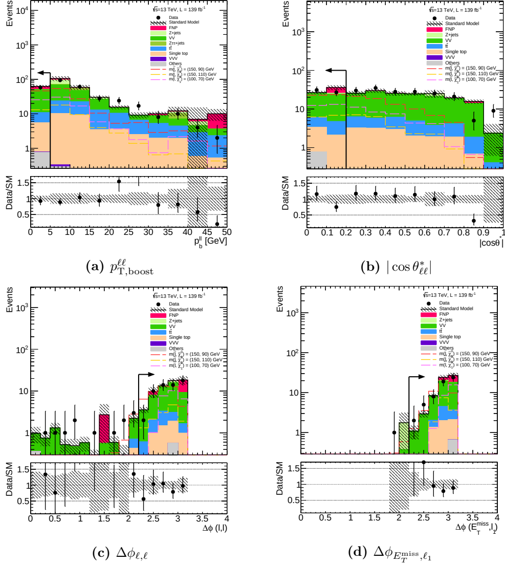
Figure 45: Plots of the most sensitive variables used in the analysis, the main background and for three benchmark signal points (m(\tilde{\ell}, \tilde{\chi}_1^0) = (100, 70), (150, 110), (150, 90) \text{ GeV}) , after all the cuts described in Table 10 (SR 0-jet), except the cut on the variable shown in the plot. The uncertainties shown are statistical only. In the bottom frame of each plot the data to MC ratio is shown.
