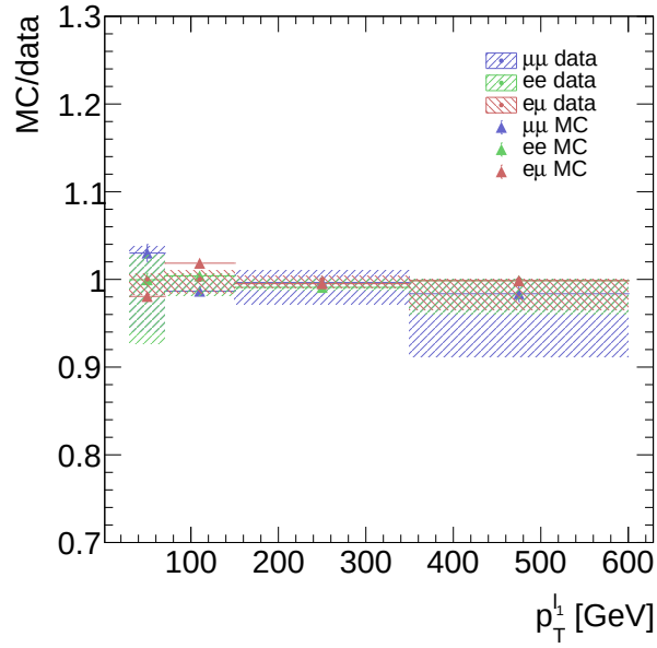
Figure 55: MC trigger efficiencies normalised to the data trigger efficiencies for \mu\mu (blue), ee (green), e\mu (red). MC includes: t\bar{t}, Wt, Z(\rightarrow \tau\tau) + \text{jets}, VV, VVV . The uncertainties are statistical only.
