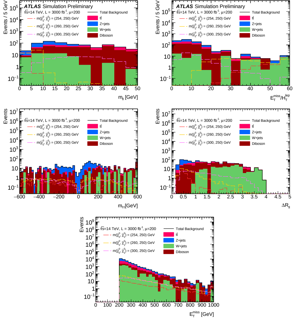
Figure 64: Background distributions of m_{\ell\ell} (top left), E_T^{\text{miss}}/H_T^{\text{lep}} (top right), m_{\tau\tau} (middle left), \Delta R(\ell, \ell) (middle right) and E_T^{\text{miss}} (bottom) used for the SR optimisation. The variables are presented with the full SR selections implemented aside from the selection on the variable shown. Three signal models with m(\chi_1^0) = 250 GeV and different mass splittings ( \Delta m(\tilde{\chi}_2^0, \tilde{\chi}_1^0) = 4, 10, \text{ and } 50 GeV) are overlaid. The m_{\ell\ell} and E_T^{\text{miss}}/H_T^{\text{lep}} figures are taken from [147].
