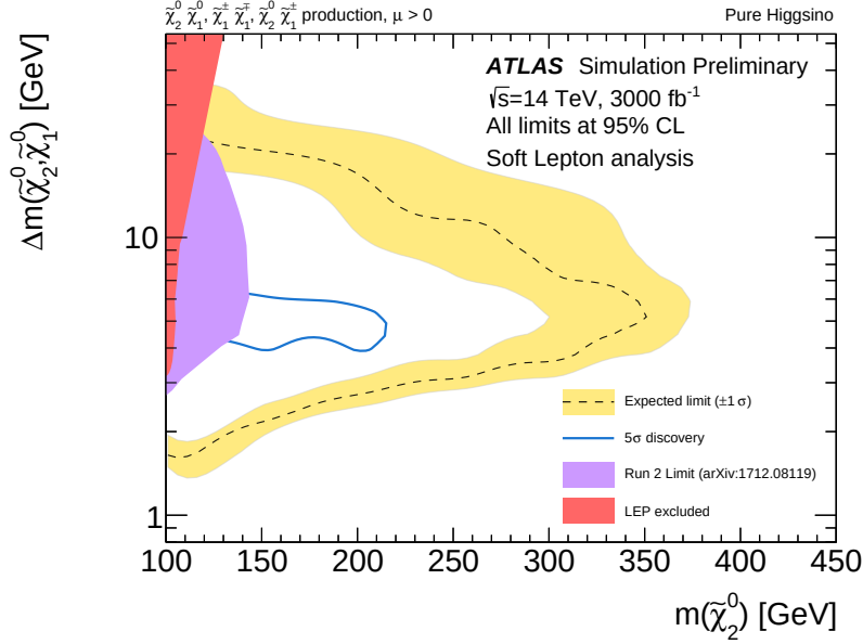
Figure 65: Expected exclusion limit (dashed line) in the \Delta m(\tilde{\chi}_2^0, \tilde{\chi}_1^0) - m(\tilde{\chi}_2^0) mass plane, at 95% CL with 3000 fb -1 of 14 TeV proton-proton collision data in the context of a pure Higgsino LSP with \pm 1\sigma (yellow band) from the associated systematic uncertainties. The blue curve presents the 5 \sigma discovery potential of the search. The purple contour is the observed exclusion limit from the Run 2 analysis [151], corresponding to a luminosity of 36.1fb -1 . The figure also presents the limits on chargino production from LEP [23]. The relationship between the masses of the chargino and the two lightest neutralinos in this scenario is m(\tilde{\chi}_1^\pm) = \frac{1}{2}(m(\tilde{\chi}_1^0) + m(\tilde{\chi}_2^0)) . Figure from [147].
