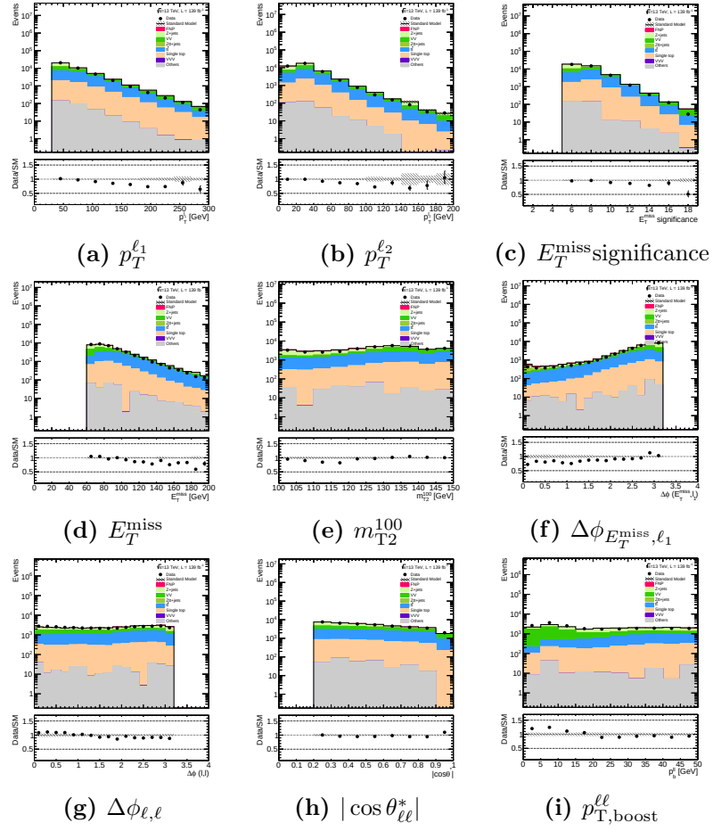
Figure 79: Data and MC distributions of the relevant variables in this analysis, for the \mu\mu channel and after the \text{CR}^{\text{eff}} cuts in Table 17 are applied. The uncertainties shown are statistical only.
