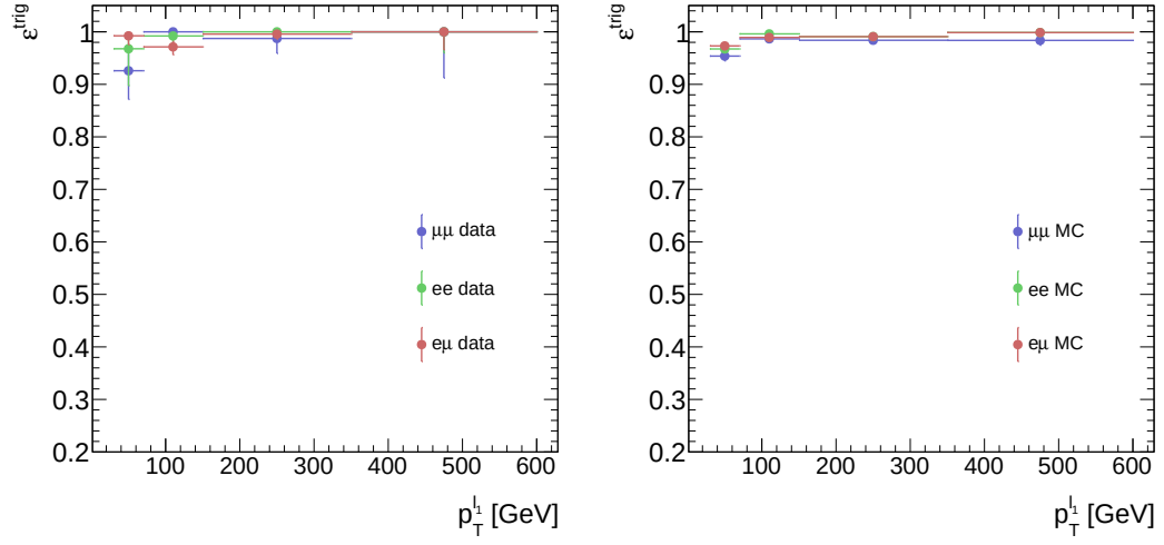
Figure 54: Trigger efficiencies for data (left) and MC (right) as a function of p_T^{\ell_1} in the three different channels: \mu\mu (blue), ee (green), e\mu (red). MC includes: t\bar{t}, Wt, Z(\rightarrow \tau\tau) + \text{jets}, VV, VVV .
