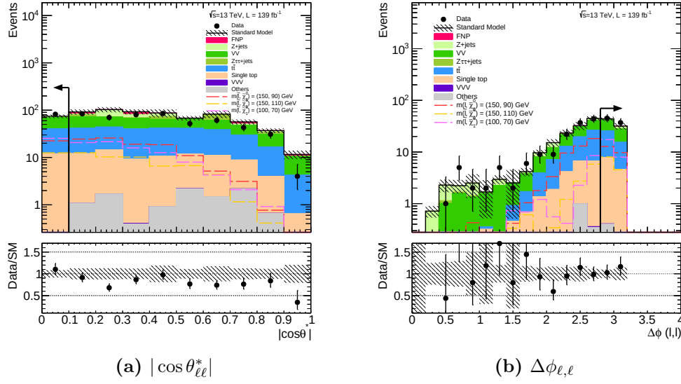
Figure 48: Plots of the most sensitive variables used in the analysis for, the main background and for three benchmark signal points (m(\tilde{\ell}, \tilde{\chi}_1^0) = (100, 70), (150, 110), (150, 90) \text{ GeV}) , after all the cuts described in Table 12 (SR 1-jet), except the cut on the variable shown in the plot. The uncertainties shown are statistical only. In the bottom frame of each plot the data to MC ratio is shown.
