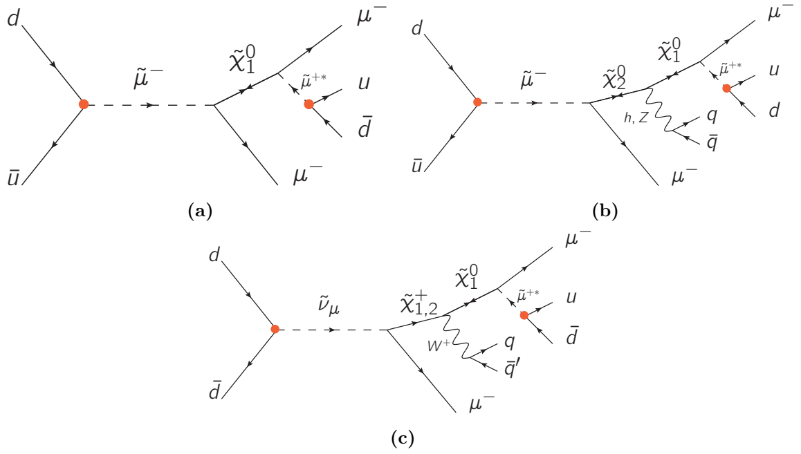
Figure 3.5.: Feynman graphs of the three dominant processes that lead to the signal signature. Each of the cascades leads to the neutralino LSP, which then decays through the \lambda'_{211} coupling, adding two jets and one muon to the final state.
