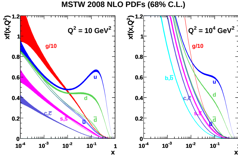
Figure 8.1.: Parton distribution functions of the MSTW2008 set at two different energy scales Q^2 . The width of the bands represent the \pm 1\sigma -confidence intervals. The graphs are taken from the "Parton distribution functions for the LHC" publication [80].
