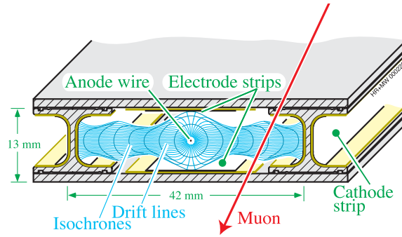
Figure 2.5.: Schematic drift cell of the drift tubes in the muon system of the CMS detector [32]. Both the driftlines and isochrones are shown.
