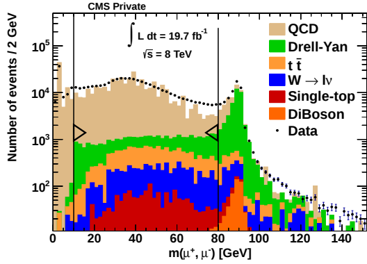
(e) Invariant dimuon mass closest to Z-mass
