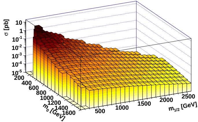
Figure 4.3.: NLO cross section map for the production of second generation sleptons used in the analysis. The production branching fractions of both the smuon and sneutrino have been taking into account for the calculation.
