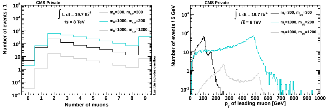
(a) Number of reconstructed muons. p_{T,1st\mu} > 10 GeV, p_{T,st\mu} > 5 GeV. No further requirements applied. (b) Transverse momentum of leading muon, p_{T,1st\mu} > 10 GeV. Structures are caused by the smuon and sneutrino 3 .
