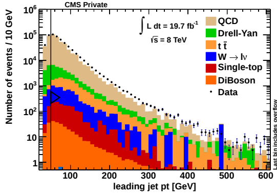
(c) Transverse momentum of jets
