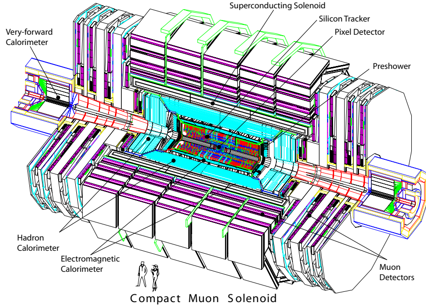
Figure 2.2.: Overview of the CMS experiment at the LHC [27]. For a size comparison, two experimentalists are shown.
