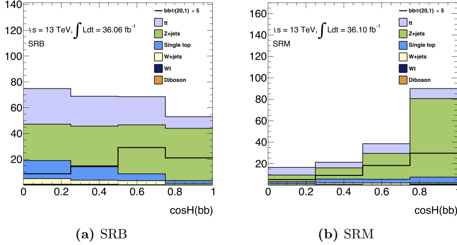
Figure 5.12: \cos\theta^* distributions for SRB (a) and SRM (b). Signal model with m_\chi = 1\text{ GeV} and M_{med} = 20\text{ GeV} has been considered with a cross section increased by a factor 5.
