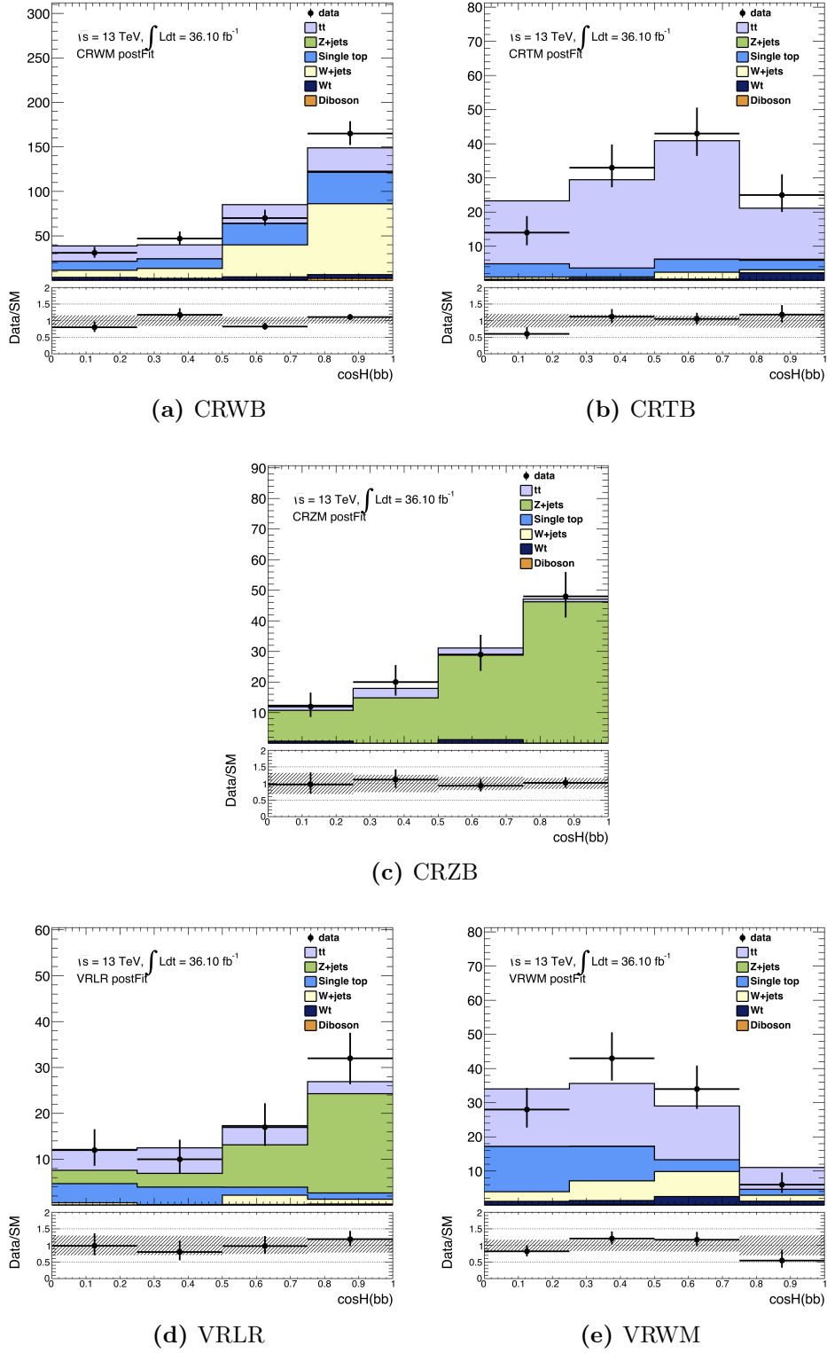
Figure 5.14: \cos \theta^* distributions after background only fits.
