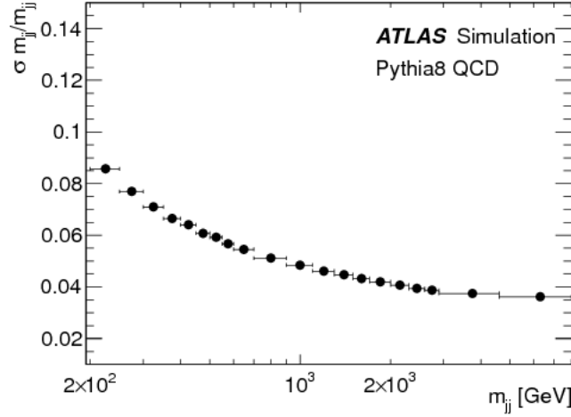
Figure 6.13: Dijet mass resolution obtained from fully simulated PYTHIA QCD Monte Carlo [77].
