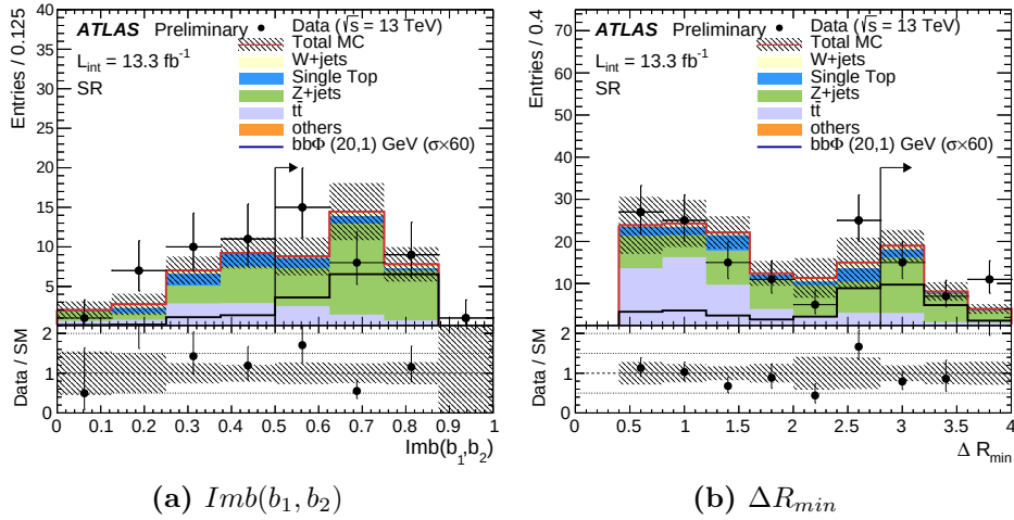
Figure B.2: Transverse momentum imbalance (a) and \Delta R_{\min} (b) in SR with all selection criteria applied except the one on the distribution shown. The requirement in each case is indicated by the arrow. The SM backgrounds are normalised to the fit results. The shaded band includes statistical uncertainties, as well as detector-related and theoretical systematic uncertainties [67].
