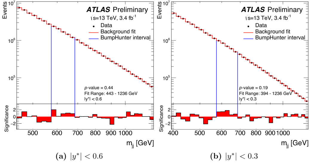
Figure 6.8: The reconstructed di-jet invariant mass in the |y^*| < 0.6 (a) and |y^*| < 0.3 (b) selections, for the TLA Analysis [78]. The vertical lines indicate the most discrepant intervals identified by the BUMP Hunter algorithm. The lower panels show the bin-by-bin significances of the data–fit differences, considering only statistical uncertainties.
