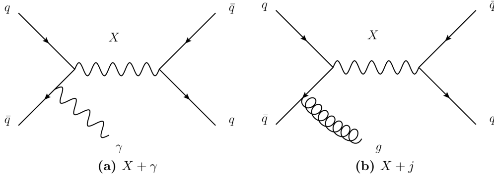
Figure 6.10: Feynman diagrams for the production of a new resonance X recoiling against an ISR (a) photon or (b) jet [79].
