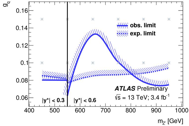
Figure 6.9: The 95% CL upper limit on the coupling g_q as function of the resonance mass m_{Z'} . The solid (dotted) lines indicates the observed (expected) limits [78].
