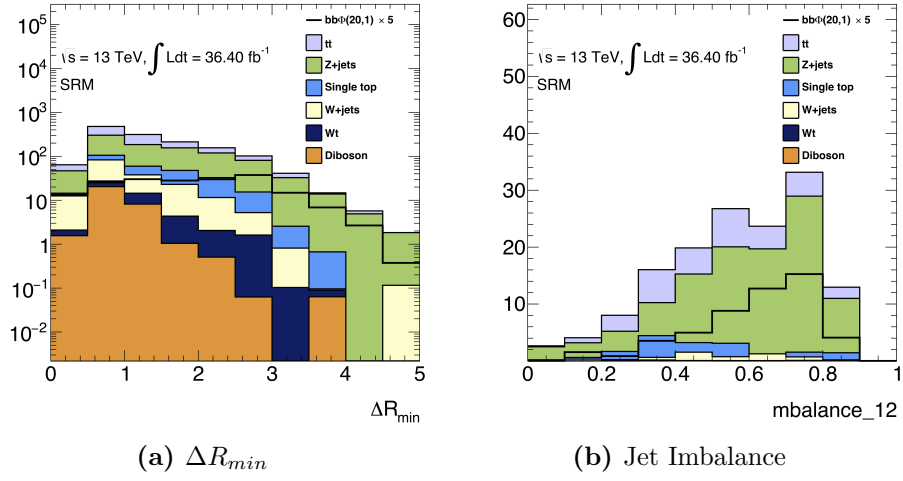
Figure 5.9: Discriminating variables for SRM. For each distribution all cuts except the one showed in the plot are applied. Signal models with m_\chi = 1 GeV and M_{med} = 20 GeV have been considered with a cross section increased by a factor 5.
