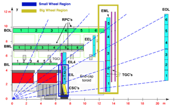
Figure 2.4: Cross-section of the ATLAS on the plane z - y [25].
