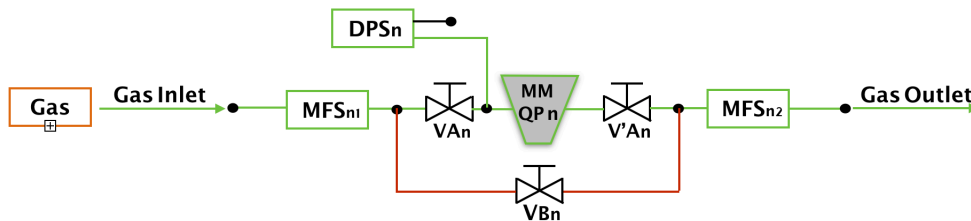
Figure 4.24: Valve adjustment to measure gas leakage of MM QP.
