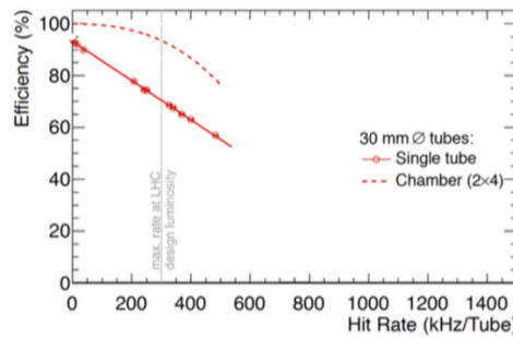
Figure 2.6: The efficiency of a single MDT tube and a MDT chamber, 2X4 tube levels, as a function of events from beam experiment data to luminosity \mathcal{L} = 3 \times 10^{34} \text{ cm}^{-2}\text{s}^{-1} [25].
