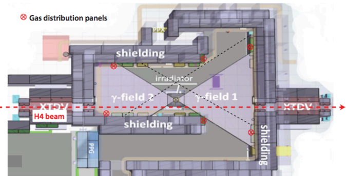
Figure 5.5: The Micromegas high voltage validation experimental setup at GIF++ irradiation setup.
