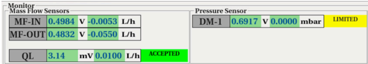
Figure 4.30: Checking the values of the sensors and the MM QP of each node with 1-Node Mode in the FRL method.
