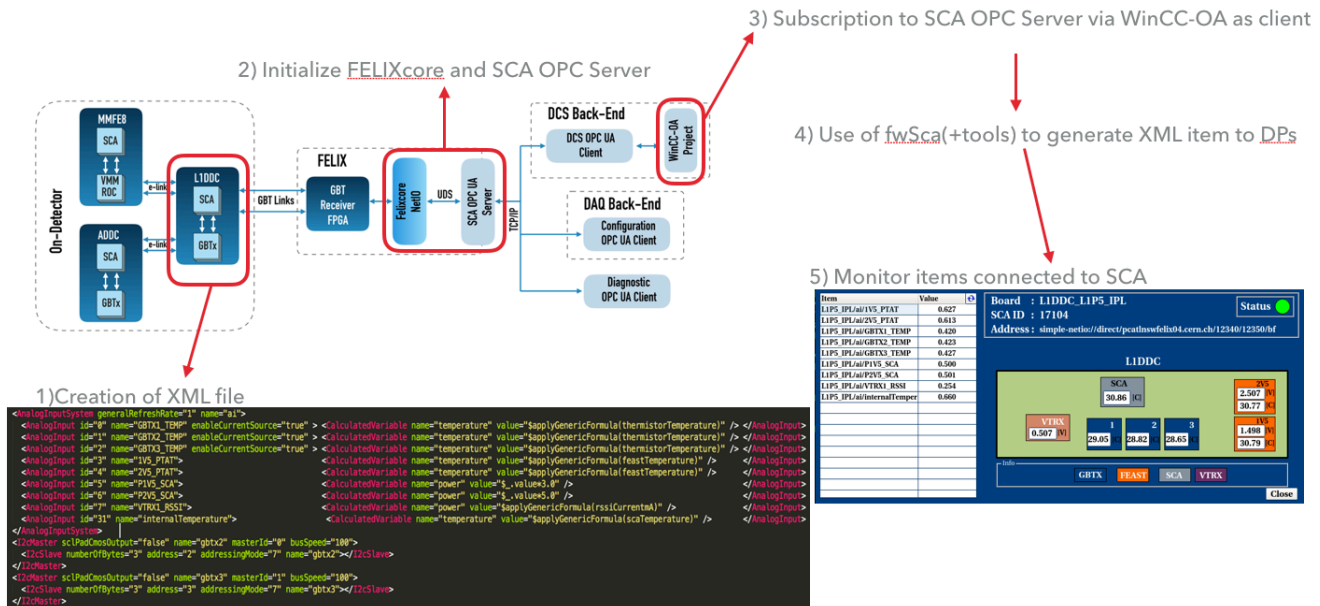
Figure 7.11: The readout concept of the SCA DCS.
