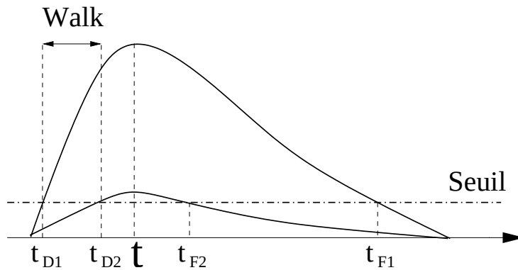
FIG. 4.8: Correction du walk. On a t = 0.6 \times t_{D1} + 0.4 \times t_{F1} = 0.6 \times t_{D2} + 0.4 \times t_{F2} .
