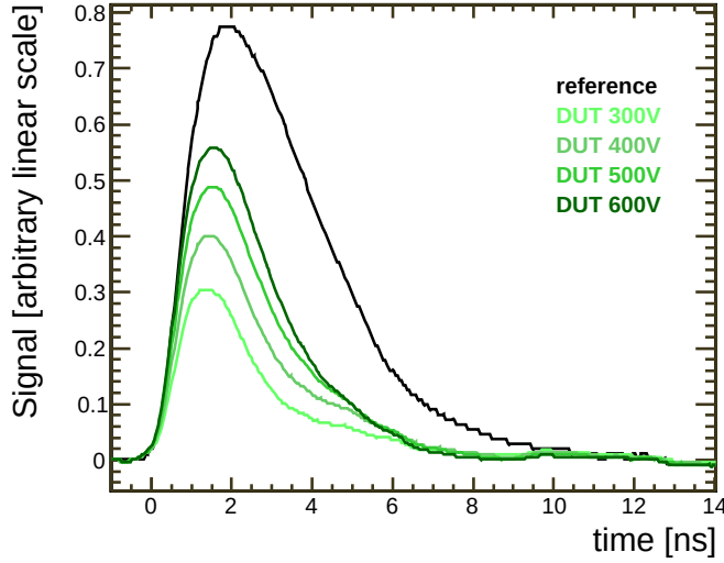
Figure 3.1: Signal response to an infrared laser pulse of a reference diode and an irradiated silicon test diode (being underdepleted) at various bias voltages measured using a TCT setup [46]. Typical pulses will be longer at the output of the shaper of the readout chip.
