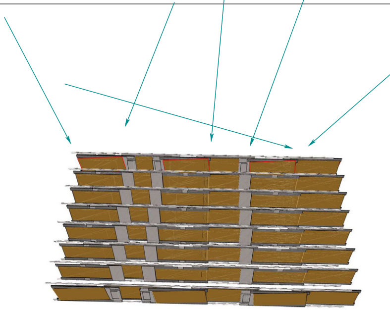
Figure 2.4: In a cosmic setup, the particles arrive from all directions. This figure illustrates the positioning of the FinnCRack detectors. In FinnCRack, the detectors and associated electronics are located in so-called rods. The rods used at FinnCRack are prototype rods of the outer barrel part of the CMS tracker discussed in, e.g., [39].
