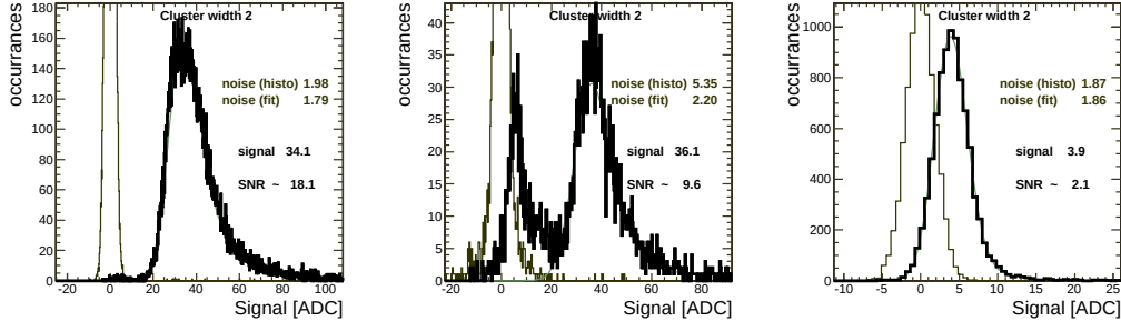
Figure 4.4: Signal histograms acquired using track-induced clustering. The control measurement is also shown. Noise data attached to the plots are calculated as RMS and function fit sigma of the control measurement. The data of Detectors 0, 3 and 11 (see p. 33) are shown.
