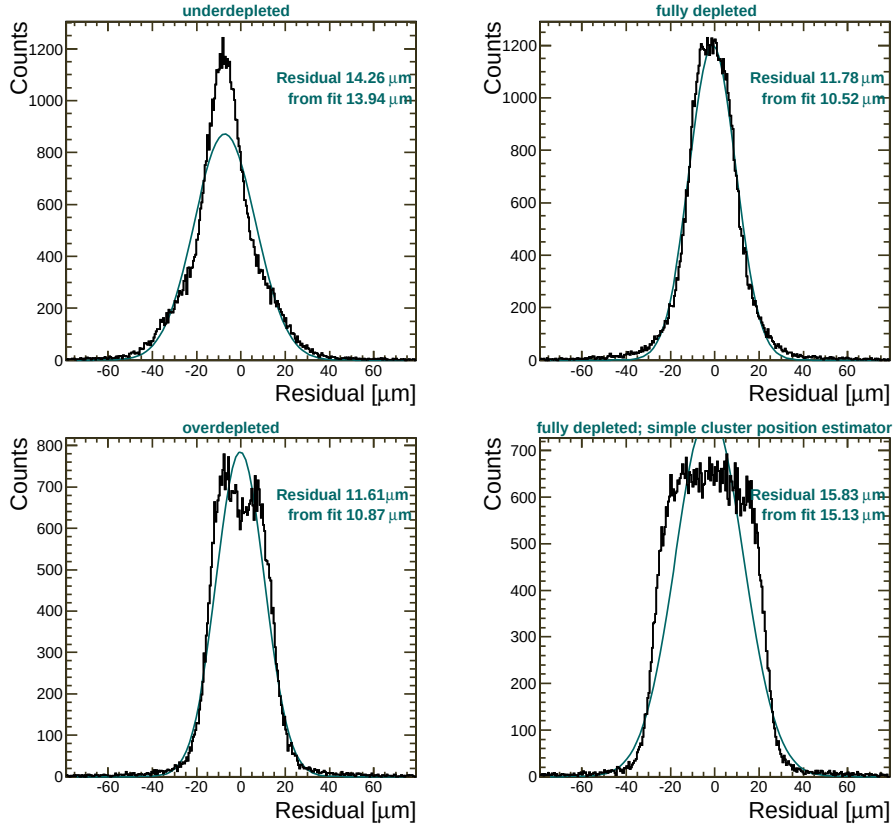
Figure 4.11: Residual distributions. In these plots a residual cut of 50 μm was used to select the clusters included in the calculation. All the plots show the response of detector 1 (p. 33); the detector bias voltage and the choice of the cluster position estimator algorithm varies.
