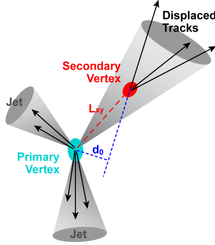
Figure 3.5.: Characteristics of collision events comprising b quarks, taken from [130]. The b quark fragments into a B meson, which typically has a lifetime on the order of \tau = 1.6 ps. The retarded decay is visible via displaced tracks possessing a large impact parameter d_0 with respect to the PV. In many cases out of several displaced tracks a secondary vertex with a distinctive distance to the PV ( L_{xy} ) can be reconstructed.
