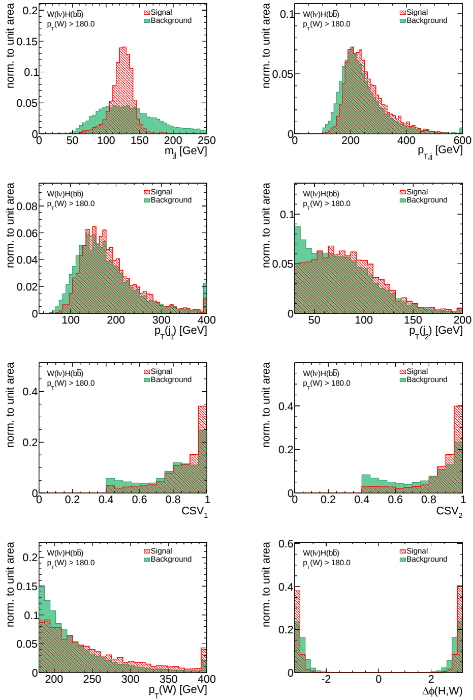
Figure 5.16.: Expected separation of BDT input variables in the DJ analysis. The signal and background distributions are normalized to unity. It should be noted that throughout this thesis the signal distributions are plotted in red.
