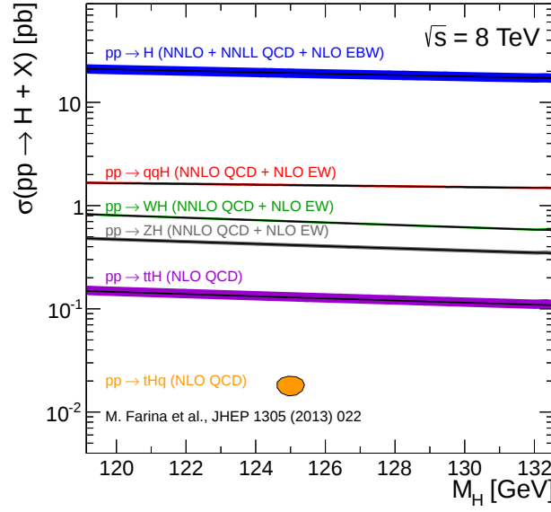
Figure 1.4.: Standard model Higgs boson production cross sections for different modes adopted from [45]. These cross section are many orders of magnitude smaller with respect to other well-known processes at the LHC, like the production of W bosons or top quark pairs.
