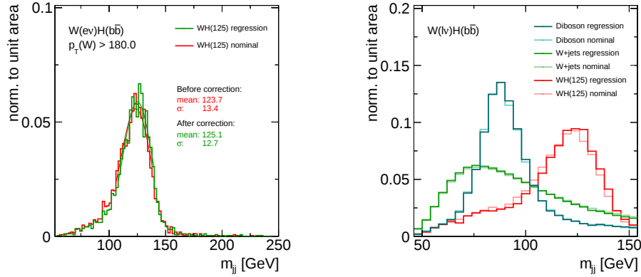
Figure 5.6.: Mass resolution improvement in signal MC (left) and mass distribution for signal, diboson and W+jets processes (right). In the left diagram the mass improvement for the 125 GeV signal template in the high p_T electron channel is found to be 6%. In the other regions the behavior is comparable. The right graph shows that the mass distribution of background processes are not visibly affected.
