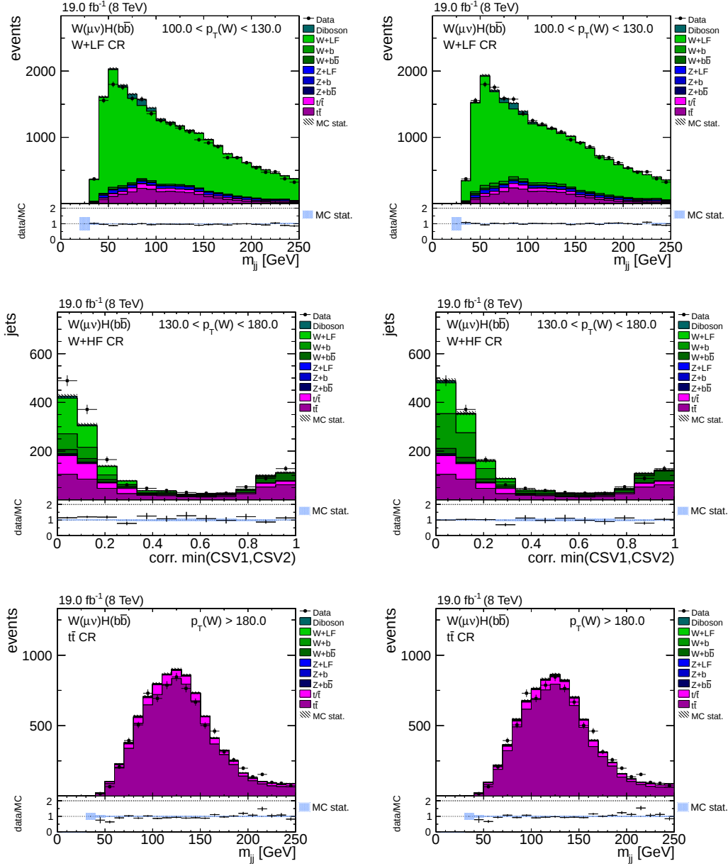
Figure 5.13.: Fitted distributions in the W(\mu\nu)H channel before (left column) and after applying the resulting scale factors (right column). Data/MC comparisons are shown for the low p_T region (top row), intermediate p_T region (middle row) and the high p_T region (bottom row) in all three control regions as indicated in the figures. The number of events in simulation is normalized to luminosity.
