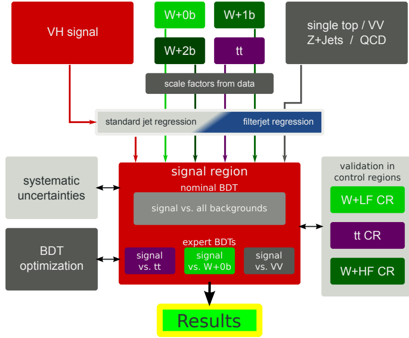
Figure 5.2.: Overview of the search strategy. Scale factors are computed in a data-driven way for t\bar{t} , W + 0b , W + 1b and W + 2b production. The estimates on the other processes are taken from simulation. Regression techniques are applied to correct the energies of standard and filter jets. After various validation steps and the evaluation of systematic uncertainties, four BDTs are evaluated and their combination is optimized. The exclusion limits are extracted on a template fit to the final discriminator.
