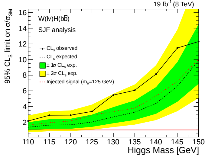
Figure 5.29.: Expected (dashed black line) and observed (solid black line) exclusion limits for the SJF analysis at all mass points. The green and yellow bands indicate \pm 1\sigma and \pm 2\sigma uncertainties on the expected limit. Additionally, the dashed red line shows the predicted values, when a Higgs boson with m_H = 125 GeV is present in the dataset.
