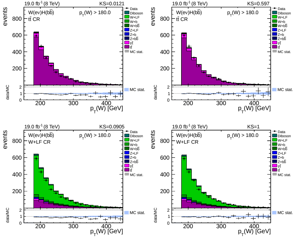
Figure 5.5.: Effect of vector boson p_T reweighting illustrated in the high p_T W(\text{ev})H channel. Simulation is scaled to luminosity and all scale factors are applied. In the left column the data/MC agreement is displayed for the t\bar{t} (top row) and the W+LF control region (bottom row). The control regions will be explained in Section 5.6. For both regions the KS-tests yield much better probabilities after applying the calculated p_T(W) -dependent weights, as shown in the right column.
