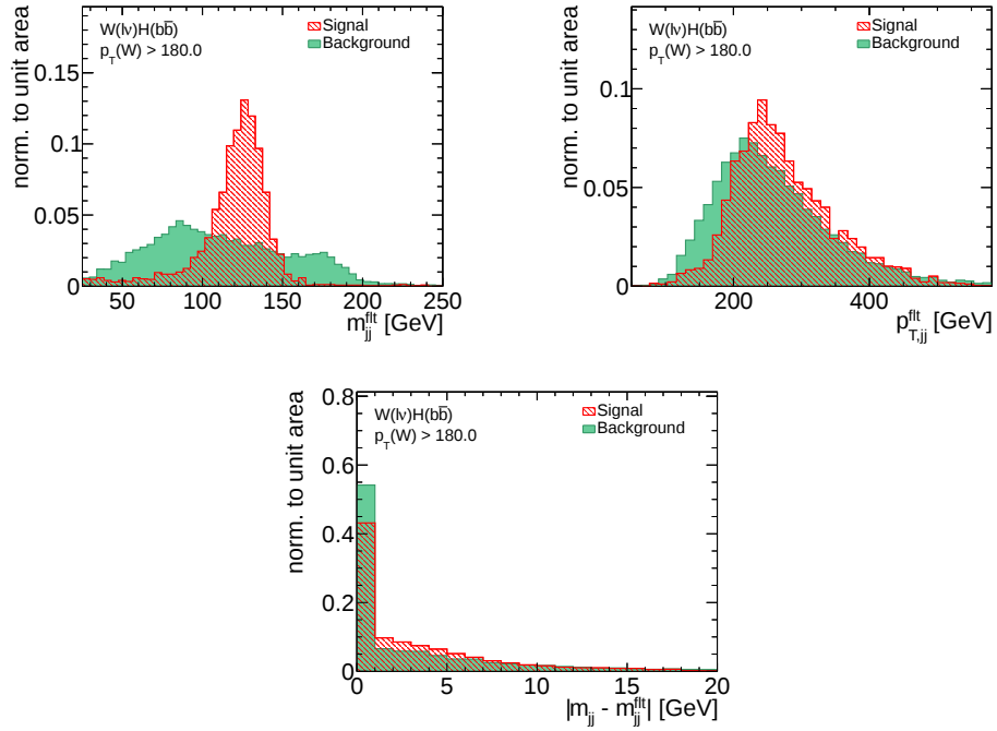
Figure 5.22.: Expected separation of added substructure variables in the SJF analysis. The signal and background distributions are normalized to unity.
