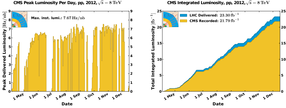
Figure 2.2.: Luminosity profile at the LHC in 2012 for proton-proton collisions at a center-of-mass energy of \sqrt{s} = 8 TeV, taken from [66]. The peak luminosity per day delivered from the LHC is depicted (left). Furthermore, the integrated luminosity over time (right) is given. The blue histogram shows the integrated luminosity provided by the LHC, and the yellow histogram indicates L_{\text{int}} recorded by CMS. The recorded integrated luminosity is corrected for downtime of the CMS trigger system, which is introduced in Section 2.2.4.
