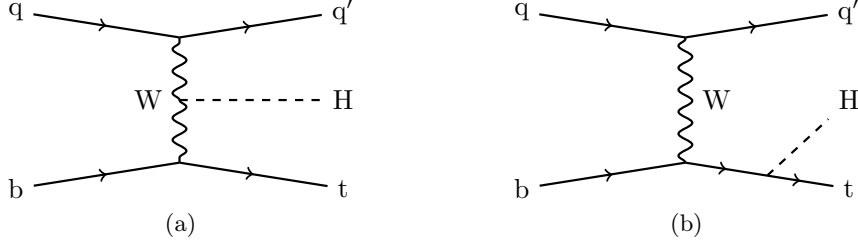
Figure 1.8.: Representative Feynman diagrams for Higgs boson production in association with single top quarks.
