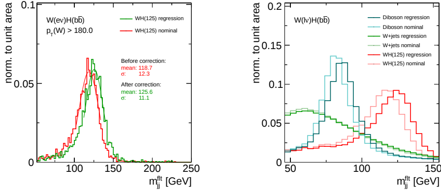
Figure 5.10.: Performance diagrams for filter jet regression. The mass resolution for signal MC (left) and mass distributions for signal, diboson and W+jets processes (right) are depicted. In the left figure the mass improvement for the 125 GeV signal template in the high p_T electron channel is found to be 15%. The performance is comparable in other regions. The right diagram shows that the mass bias is not only resolved for the signal process, but also for diboson production.
