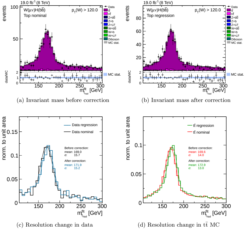
Figure 5.11.: Different validation checks for filter jet regression in t\bar{t} events as described in the text. The invariant mass of the reconstructed hadronically decaying top quark is shown before (a) and after applying the correction (b). It is visible that the regression does not introduce a bias. Furthermore, the mass resolution is compared before and after the correction for data in (c) and t\bar{t} MC in (d). In both cases, the resolution is improved and the mean values are shifted more towards the nominal top quark mass.
