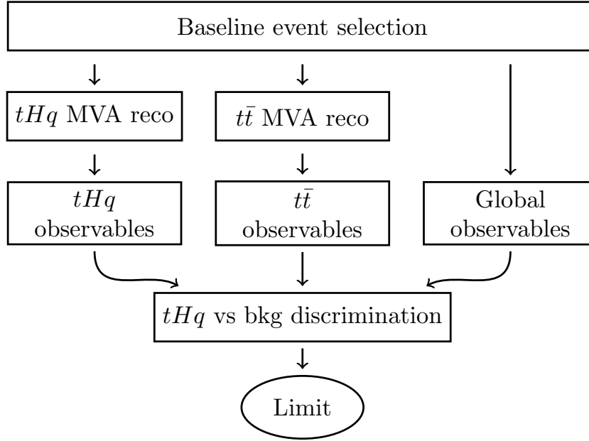
Figure 6.1.: Analysis scheme of the tHq search. After a tight event selection, every event is reconstructed under the assumption that it was a signal event and that it stems from t\bar{t} production. This information is input for the classification MVA, that is used for the limit extraction. The sketch is taken from [61].
