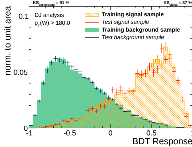
Figure 5.18.: BDT response for the DJ analysis in the high p_T region. The distributions are separated for signal and background events, and for training and testing samples. Adequate agreement is found by comparing the performance of the classification between the training and testing sample.
