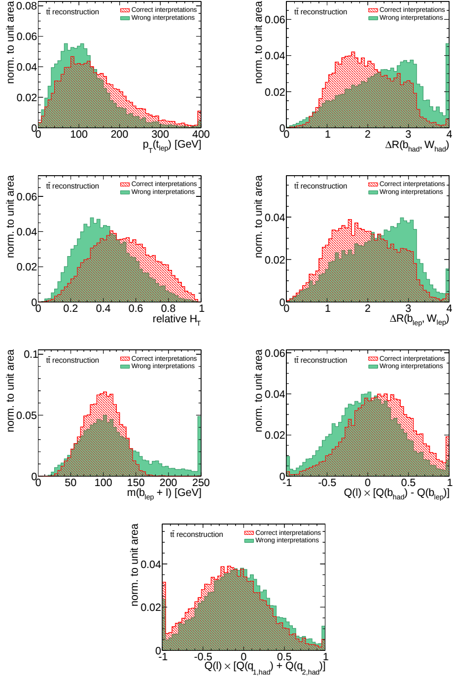
Figure B.5.: Remaining input variables for reconstruction under the t\bar{t} hypothesis.
