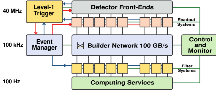
Figure 2.7.: Architecture of the CMS trigger and data acquisition system, taken from [71].
