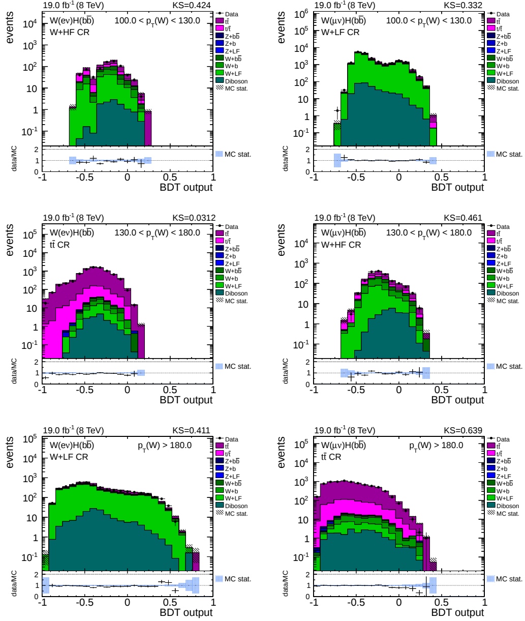
Figure 5.21.: Validation of classification BDT for the DJ analysis in control regions for the W(\text{ev})H (left column) and the W(\mu\nu)H channel (right column). Data/MC comparisons are shown for the low p_T region (top row), intermediate p_T region (middle row) and the high p_T region (bottom row) in all three control regions as indicated in the figures. Scale factors and event weights are applied on simulation. Overall a very good agreement is found, justifying the use of the BDTs.
