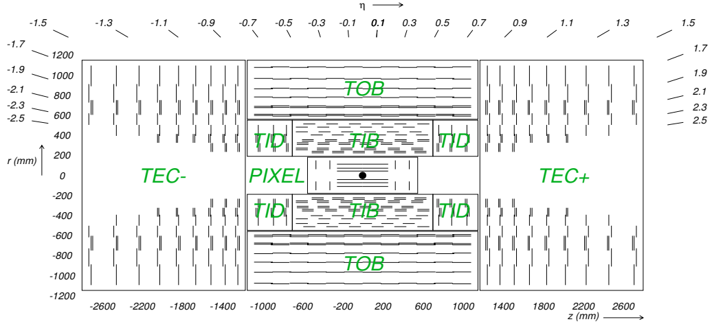
Figure 2.4.: Overview of the CMS tracking system, taken from [71]. The pixel detector environs the interaction point (black dot). The strip detector is partitioned into tracker inner barrel (TIB), tracker outer barrel (TOB), tracker inner disk (TID) and tracker endcaps (TEC). The detector modules (single line) and stereo modules (double lines) are shown.
