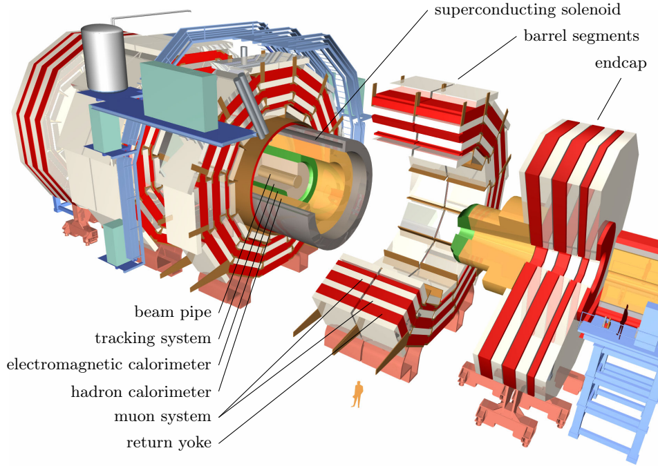
Figure 2.3.: Illustrative overview of CMS detector layout adapted from [65, 70]. The beam pipe is surrounded successively by the tracking system, the electromagnetic calorimeter and hadron calorimeter. These parts are located in the volume of the superconducting solenoid. The gas-ionizing muon chambers are found outside the solenoid embedded in the steel return yoke. The modular structure with several barrel segments and two endcaps facilitates maintenance and inspection of the detector parts.
