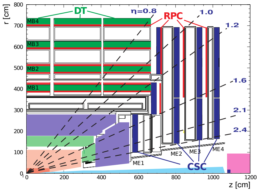
Figure 2.6.: Schematic overview of the muon system, taken from [78]. The sketch shows the longitudinal view of one quarter of the detector. Three different types of gas detectors are used. Drift tubes (DT) are installed in the four barrel muon stations, MB 1 to MB 4. The endcap muons stations, ME 1 to ME 4, are equipped with cathode strip chambers (CSC). In all stations additional resistive plate chambers (RPC) are embedded in the region |\eta| < 1.6 , where a high muon rate is expected.
