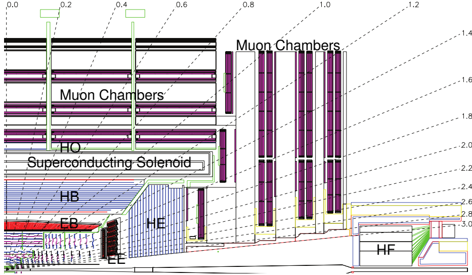
Figure 2.5.: CMS calorimetry and muon systems, adapted from [71] with modification. The sketch represents the longitudinal view in one quarter of the detector. The tracking system is encompassed by the calorimetry system, partitioned into electromagnetic barrel (EB), hadron barrel (HB) and hadron endcaps (HE). The electromagnetic endcaps (EE) are shown together with the electromagnetic preshower detector. Outside the superconduction solenoid the hadron outer calorimeter (HO) and the muon system embedded in the steel return yoke are located. The hadron forward calorimeter ensures energy measurements of particles with high pseudorapidities. For a detailed view of the muon system see Figure 2.6.
