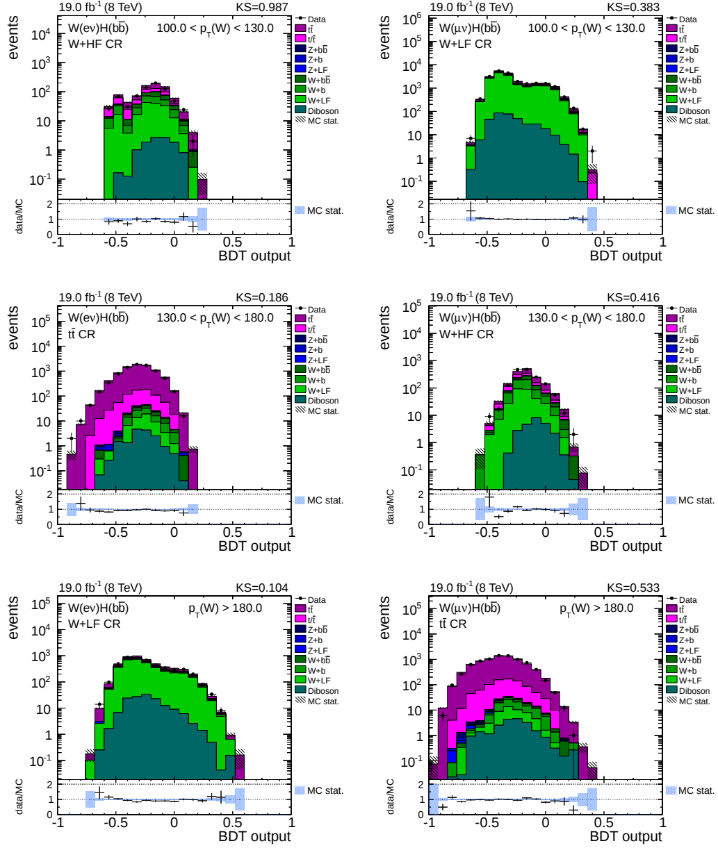
Figure 5.25.: Validation of classification BDT for the SJF analysis in control regions for the W(\text{ev})H (left column) and the W(\mu\nu)H channel (right column). Data/MC comparisons are shown for the low p_T region (top row), intermediate p_T region (middle row) and the high p_T region (bottom row) in all three control regions as indicated in the figures. Scale factors and event weights are applied on simulation. Overall very good agreement is found, justifying the use of the BDTs.
