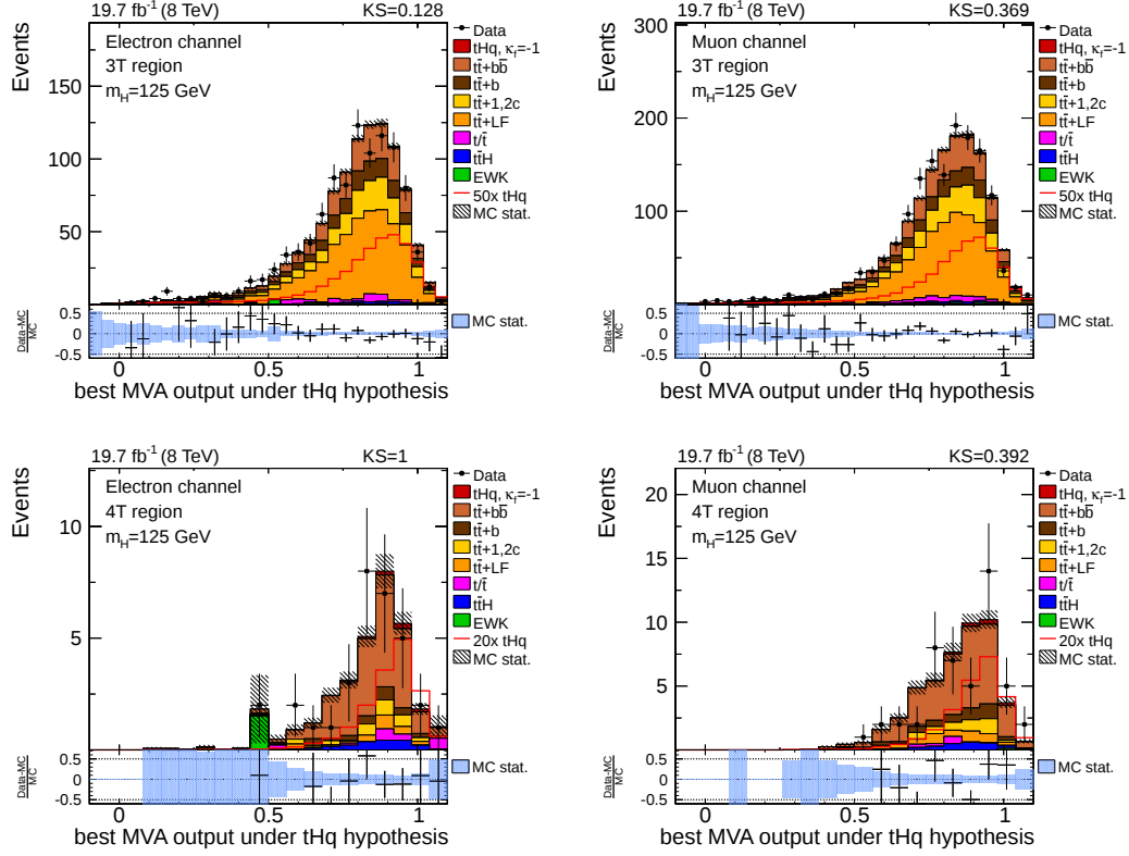
Figure B.4.: Data/MC comparisons for the tHq reconstruction when choosing the interpretation with the largest MVA output in each event. The distributions are shown for the 3T region (top row) and for the 4T region (bottom row) in both, the electron (left column) and muon channel (right column). The MC templates are normalized to data. KS-test probabilities are given and overall good agreement is found.
