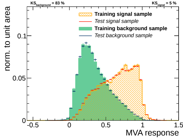
Figure 6.16.: Response of classification MVA for the signal and background processes. The shapes are shown separately for training and testing samples. A KS-test is performed and no hint for overtraining is found.
