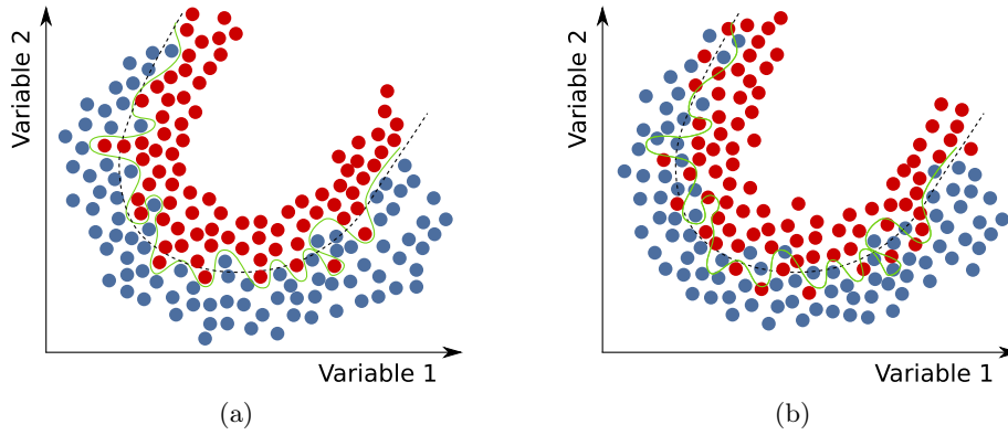
Figure 4.4.: Illustrative example for overtraining. Shown are two measurements for signal events (red) and background events (blue) in two arbitrary variables. On the left side, the training dataset is shown. The decision boundary from a well trained MVA (black dashed line) is depicted as well as from an overtrained MVA (green line) that learns from statistical fluctuations in the dataset. In a statistically independent dataset, illustrated on the right side, the fluctuations occur at different positions and the performance of the overtrained MVA is worse.
