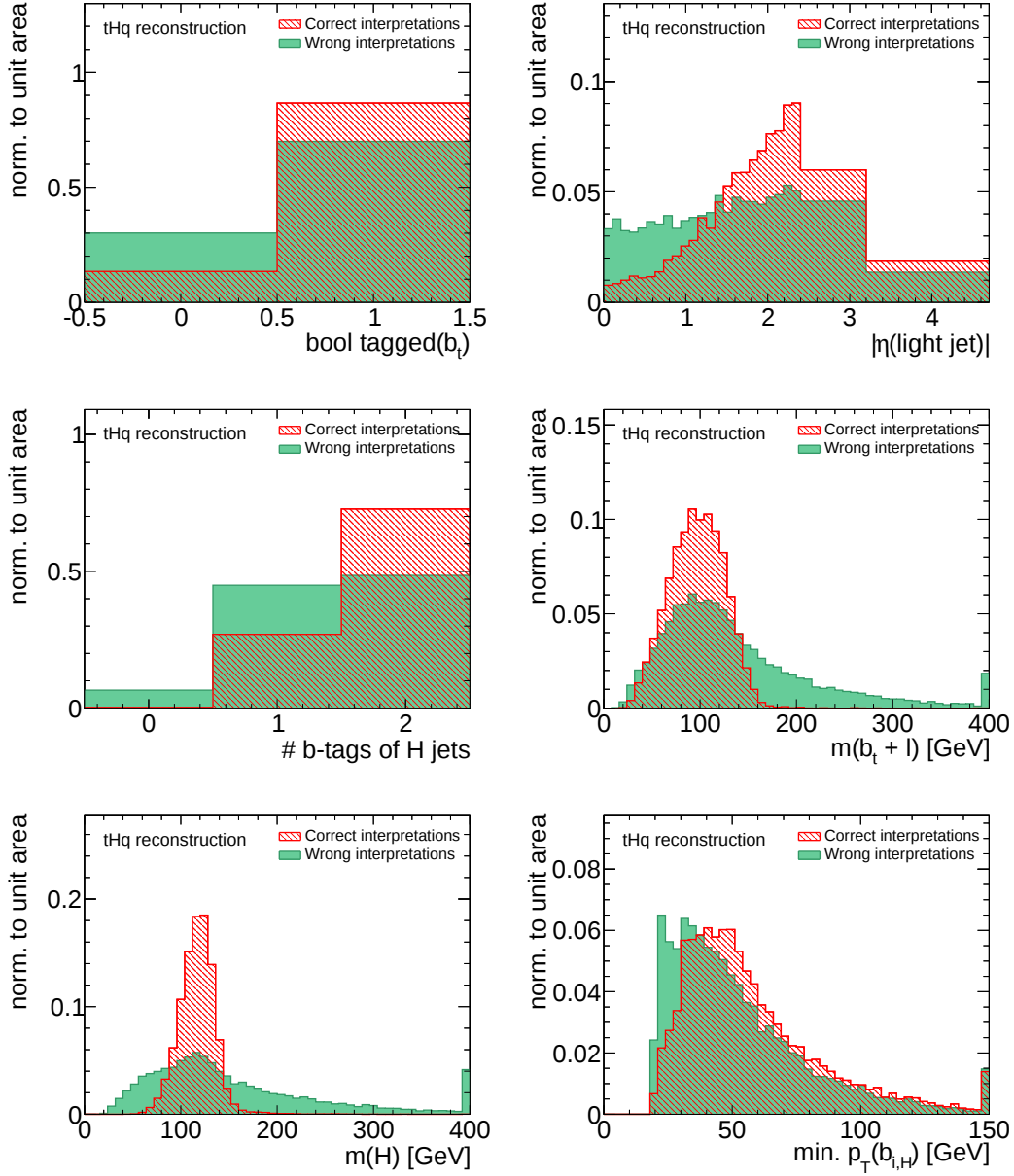
Figure 6.7.: Shapes of most important input variables for reconstruction under tHq hypothesis. The shapes are shown separately for correct and wrong interpretations. The corresponding diagrams for the remaining input variables can be found in Figure B.3. As the correct interpretations act as signal in the training, their distributions are consistently shown in red.
