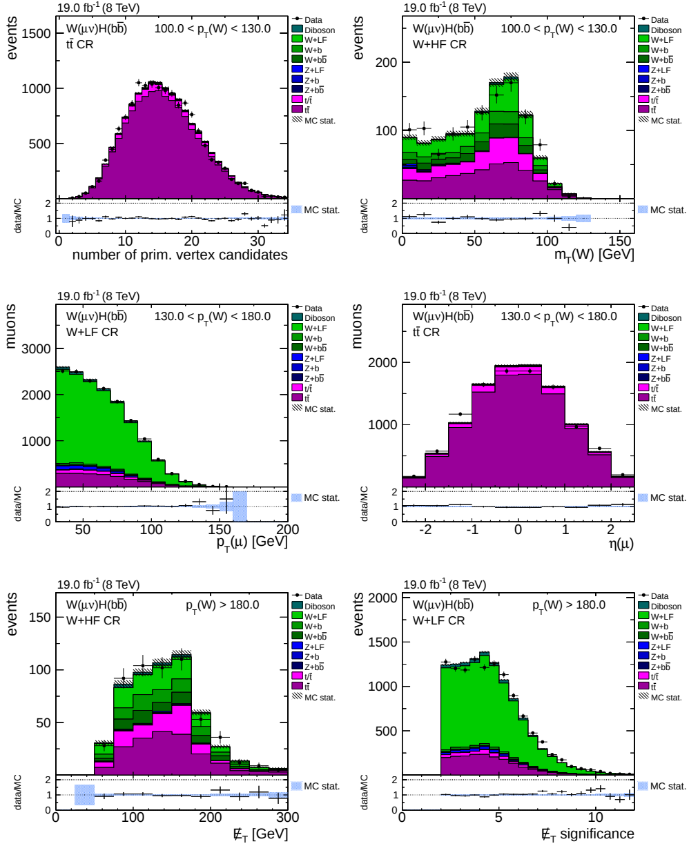
Figure A.1.: Different event distributions in control regions for the W(\mu\nu)H channel. Data/MC comparisons are shown for the low p_T region (top row), intermediate p_T region (middle row) and the high p_T region (bottom row) in all three control regions as indicated in the figures. The number of events in simulation is normalized to data.
