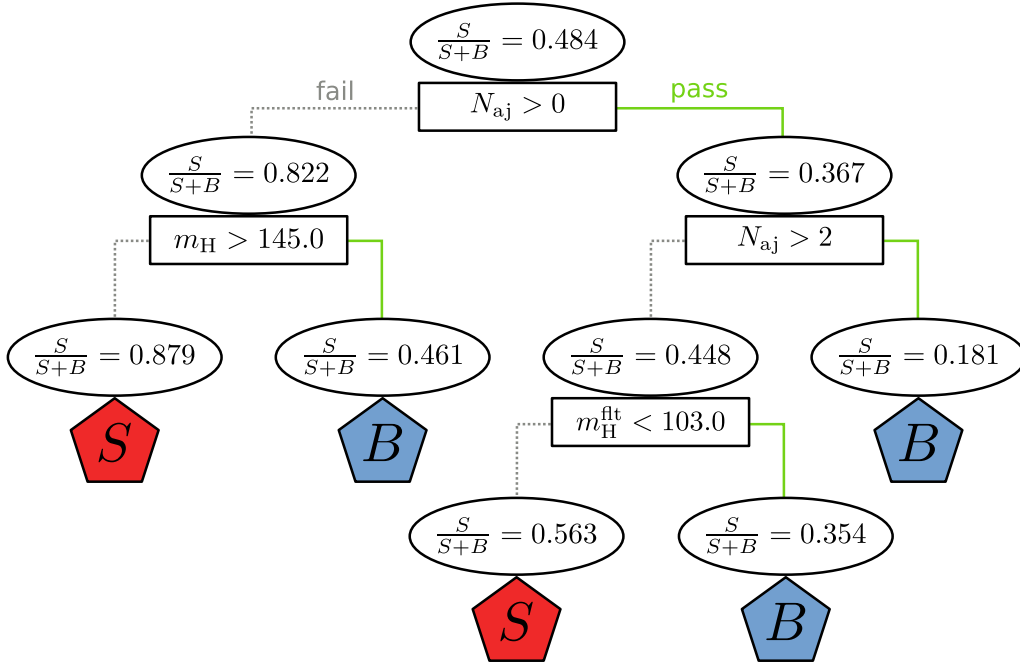
Figure 4.2.: Exemplary decision tree used in the analysis. The topmost node roughly has the same amount of signal and background events as input. Up to three subsequent requirements are applied depending on if an event passes or fails a cut. Each leaf classifies the event as signal (S) or background (B). On the order of hundreds of these trees are used simultaneously to make a majority decision.
