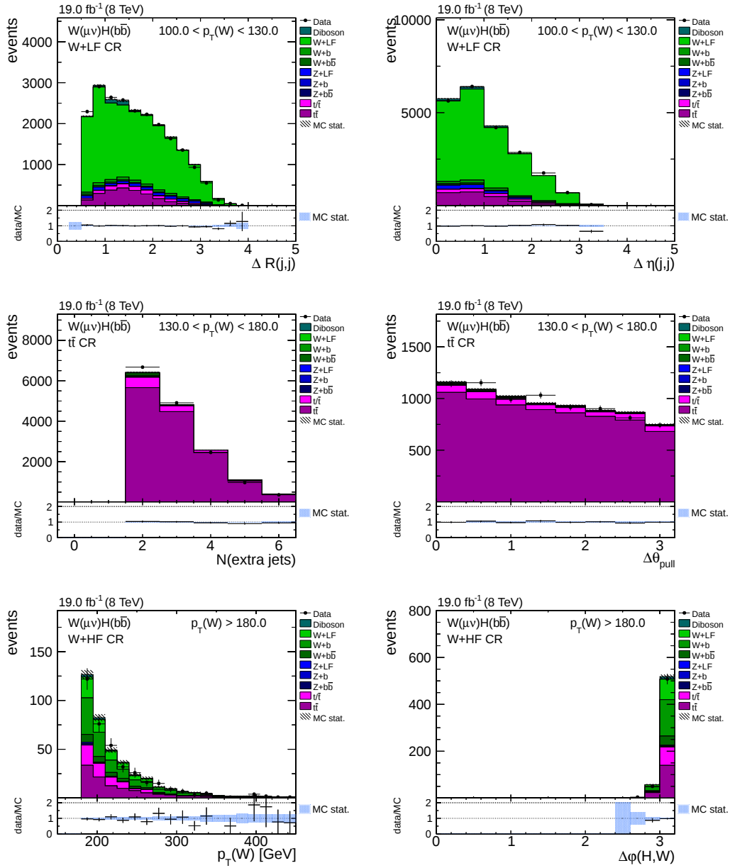
Figure 5.20.: DJ analysis input variables for the W(\mu\nu)H channel in different control regions as indicated within the diagrams (cont.). The simulation is scaled to luminosity and scale factors are applied. In all variables solid data/MC agreement is found. The corresponding distributions in the W(e\nu)H channel are presented in Figure A.3.
