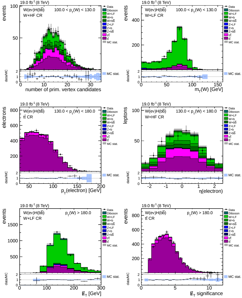
Figure 5.12.: Different event distributions in control regions for the W(e\nu)H channel. Data/MC comparisons are shown for the low p_T region (top row), intermediate p_T region (middle row) and the high p_T region (bottom row) in all three control regions as indicated in the figures. The number of events in simulation is normalized to data. The corresponding distributions for the W(\mu\nu)H channel are presented in Figure A.1 in the appendix.
