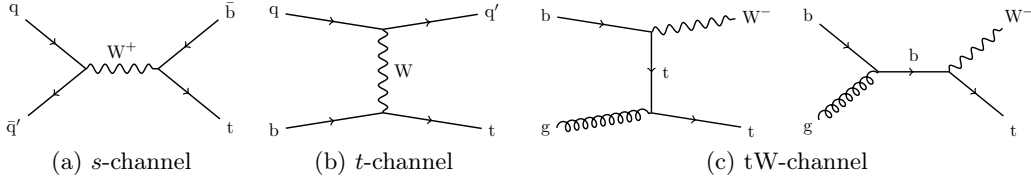
Figure 1.7.: Representative Feynman diagrams for single top quark production. The cross section for the t -channel is the highest of the three modes.
