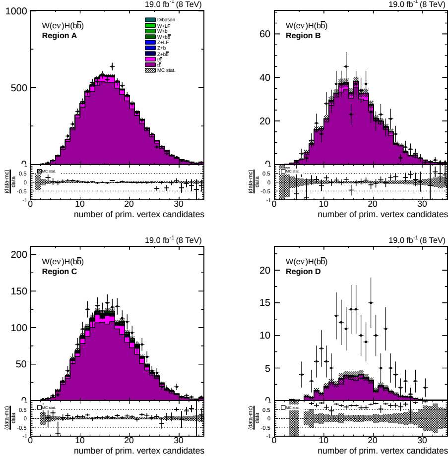
Figure 5.15.: Descriptive example of the ABCD method in the t\bar{t} control region. The number of primary vertices is shown in each QCD study region for the electron channel. Region A (upper-left) is the ordinarily-defined control region. For region B (upper right) the electron isolation requirements are reversed. Region C (lower left) is obtained by inverting the \cancel{E}_T cut and for region D (lower right) both cuts are reversed. Monte Carlo predictions are shown for all the major background processes with the exception of multi-jet QCD production. The difference between data and Monte Carlo prediction is attributed to this specific background process.
