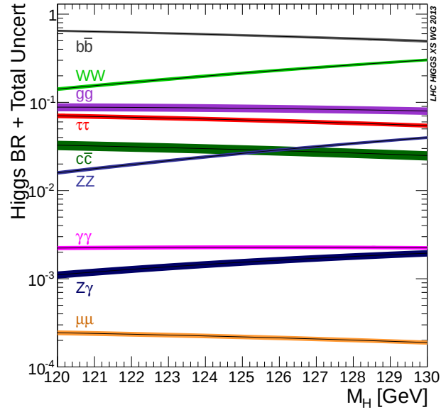
Figure 1.5.: Higgs boson branching ratios over its invariant mass, taken from [46]. The error bands account for theoretical and parametric uncertainties in the calculations. For a mass of m_H = 125 GeV the Higgs boson decays into a bottom quark pair in 58% of all cases.
