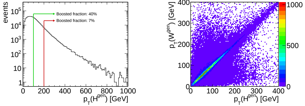
Figure 5.1.: Generated boost distributions in signal MC. The left diagram illustrates the signal efficiency for specific requirements on the transverse momenta of generated Higgs bosons. With the criterion p_T > 100 GeV 60% of the signal events are lost. In the right-hand figure the transverse momenta of W boson and H boson are compared at generator level. A clear correlation is visible.
