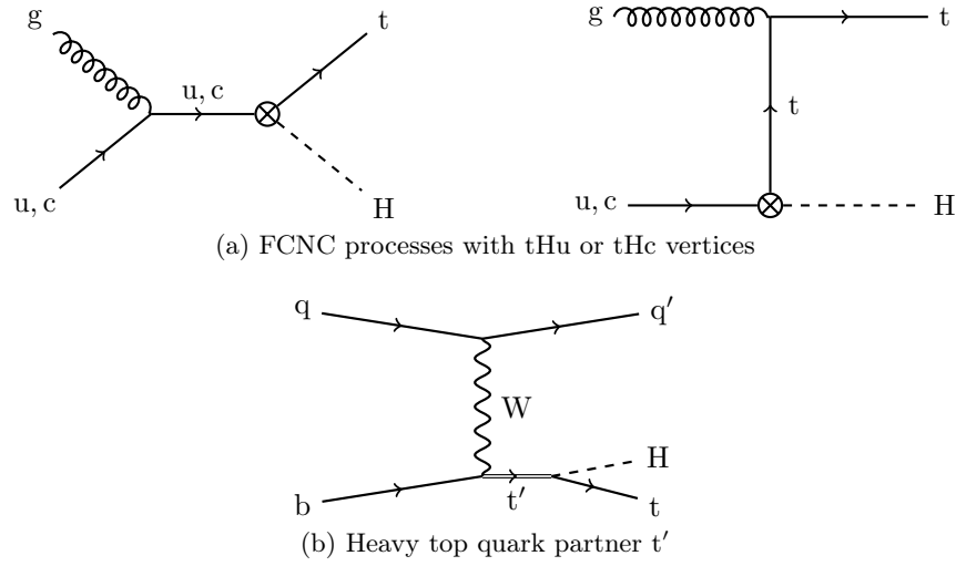
Figure 1.10.: Possible Feynman diagrams beyond the standard model contributing to tHq production. The crossed out vertices are in the two diagrams in (a) are suppressed in the standard model. The double line in (b) indicates a hypothetical top quark partner that is predicted in some new physics models.
