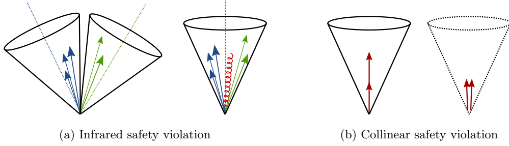
Figure 3.3.: Examples of violations of the two fundamental jet requirements. Additional soft emissions, e.g. by pile-up, are not supposed to change the jet definition (a). Furthermore, the number of reconstructed jets should not vary with collinear splitting (b).
