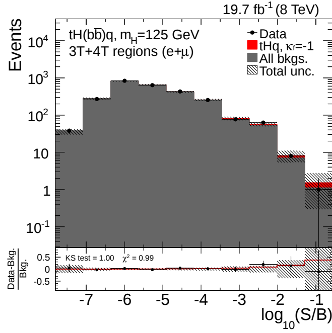
Figure 6.22.: Combination of all fitted distributions into one single diagram. Here, all events from all signal regions are sorted according to the expected signal-over-background ratios in their corresponding bins. Additionally, the ratio between data and background-only is given. The given uncertainties include all statistical and systematic effects. No excess in data with respect to the expected background is visible.
