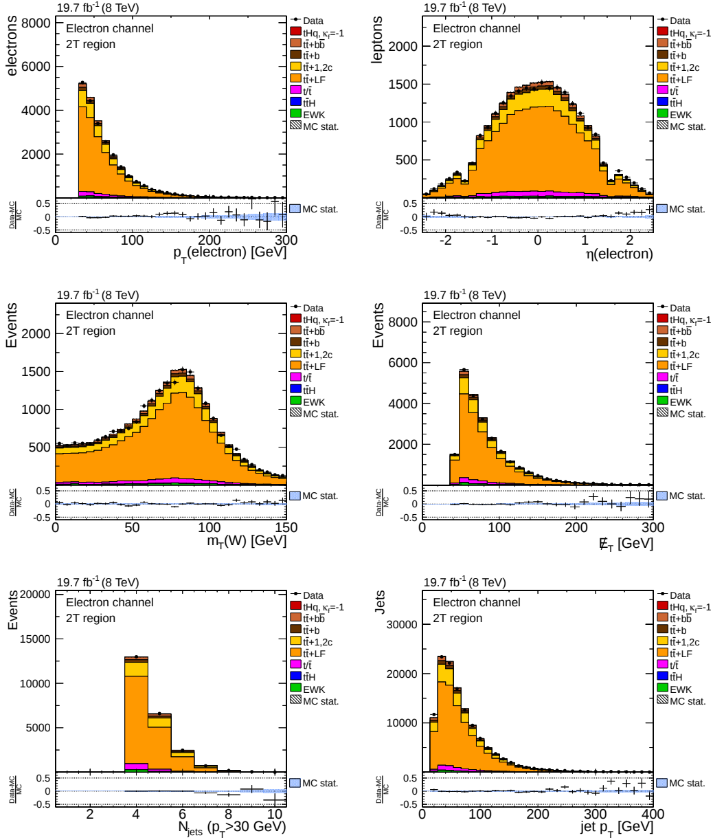
Figure 6.5.: Event information variables for the electron channel in the 2T region. The number of simulated events is normalized to data. Overall good agreement between data and simulation is found. The corresponding distributions for the muon channel are given in Figure B.1.
