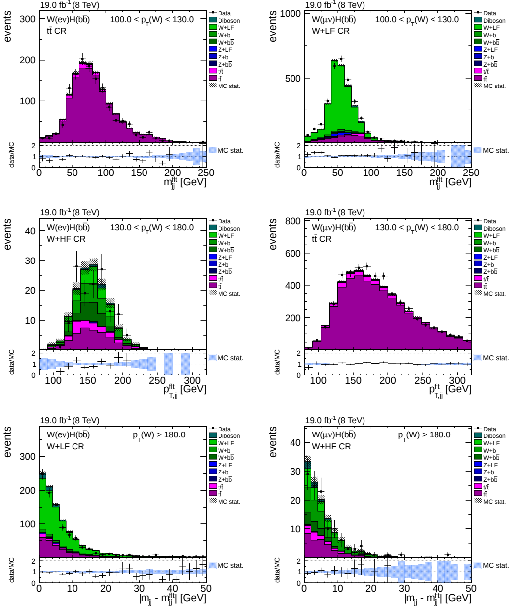
Figure 5.24.: Added filter jet variables in different control regions for the W(ev)H (left column) and the W( \mu\nu )H channel (right column). Data/MC comparisons are shown for the low p_T region (top row), intermediate p_T region (middle row) and the high p_T region (bottom row). Overall reasonable agreement is found. The agreement would improve, if additional requirements on p_{T,jj}^{\text{fit}} were applied.
