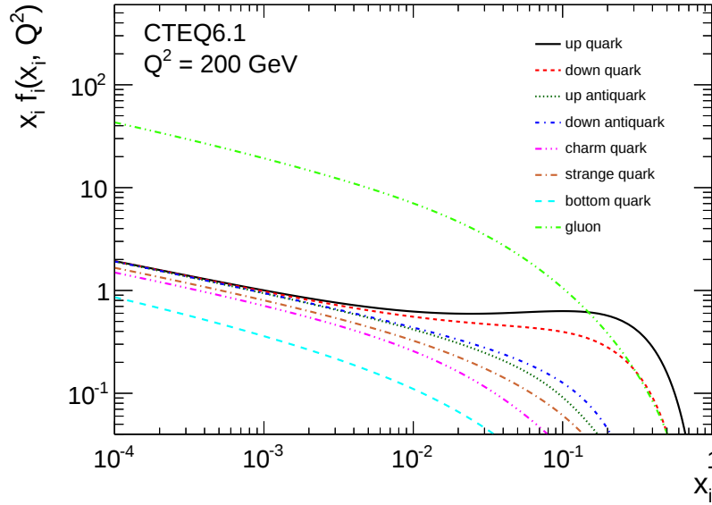
Figure 3.2.: Exemplary CTEQ61 proton PDF for gluons and quarks. This PDF is used for the majority of MC samples in thesis. The values shown at a scale of Q^2 = 200 GeV are provided by the Durham HepData Project [87].
