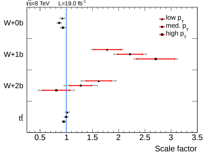
Figure 5.14.: Results of the scale factor estimation for all regions. The red and gray error bars denote the statistical and the total uncertainty on the fit, respectively. The discrepancy found in the values for W+1b arises due to generator mismodeling of the gluon splitting into a bottom quark pair.
