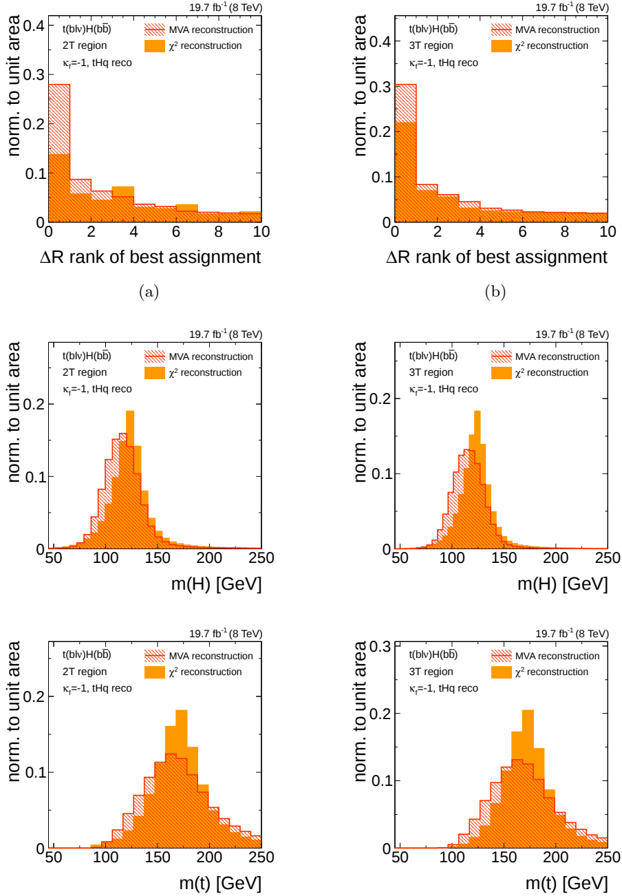
Figure 6.10.: Comparison for tHq reconstruction between MVA and \chi^2 reconstruction techniques. On the left side the \Delta R rank of the chosen hypothesis and the mass distributions of reconstructed Higgs boson and top quark candidates are shown in the 2T region. On the right side the same diagrams are given in the 3T region. Because the \chi^2 values depend on the difference between reconstructed and true mass, the mass distributions are narrower compared to the MVA reconstruction. However, with the MVA reconstruction the correct jet assignment is found more often, leading to a better description of the kinematics of the event.
