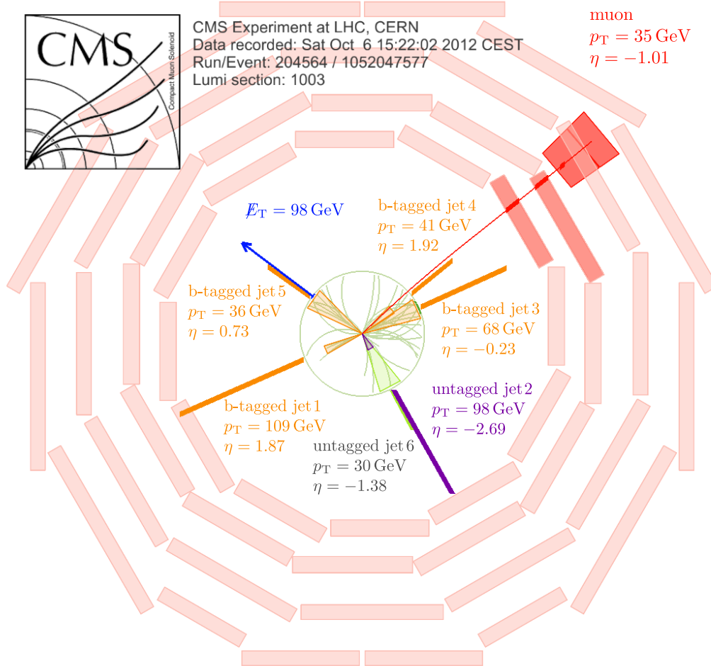
Figure 6.23.: Transverse detector view of the most signal-like event in data. The scheme shows the reconstructed objects comprising all corrections. There is exactly one isolated muon (red) and four b-tagged jets (orange bars) in the event. Furthermore, the characteristic forward jet (purple) and a large amount of missing energy is found. In this event jet 1 and jet 5 are assigned to the Higgs boson candidate. Jet 2 is the light quark candidate and jet 3 is assigned to the top quark. The reconstructed masses of the Higgs boson and top quark candidates are m_H = 100.3 \text{ GeV} and m_t = 173.3 \text{ GeV} , respectively.
