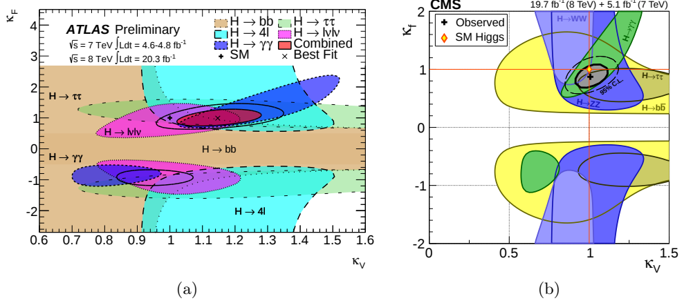
Figure 1.9.: Constraints on \kappa_f and \kappa_V from ATLAS [56] (a) and CMS measurements [48] (b). The allowed regions for the values are shown separately for the different Higgs boson decay modes.
