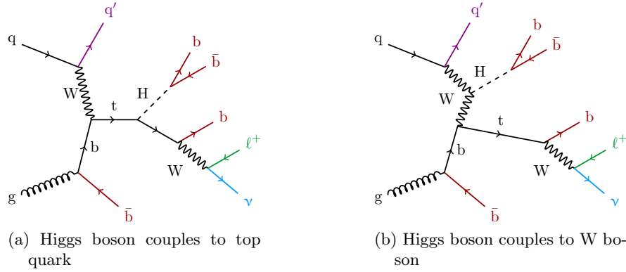
Figure 6.2.: Representative LO Feynman diagrams for tHq production. On the left side, the diagram where the Higgs boson arises from the top quark is shown. The right diagram depicts the case where the Higgs boson is radiated from the W boson.
