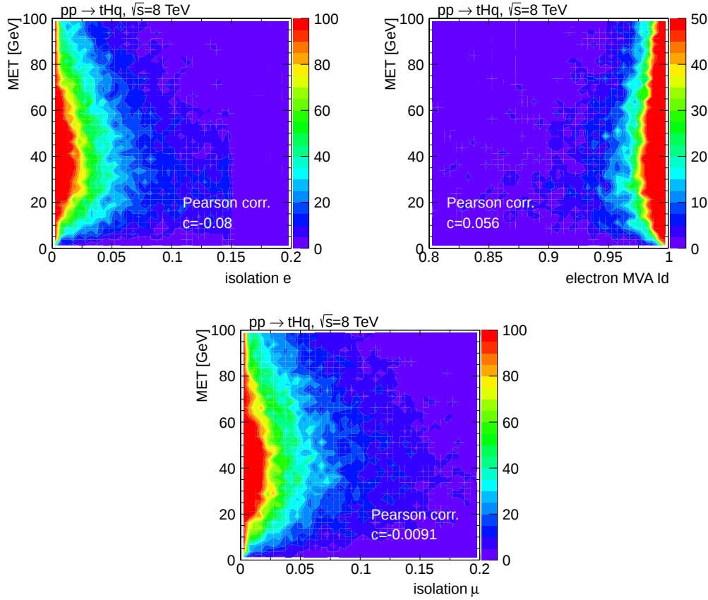
Figure 6.6.: Correlation between input variables for the ABCD method. The top row shows the correlation in data for the electron channel. Since in regions B and D both, the electron isolation and the MVA ID are inverted, two separate diagrams are shown. In the bottom row the correlation in data for the muon channel is depicted. For all three the correlation factors are given concurring in all cases with zero correlation.
