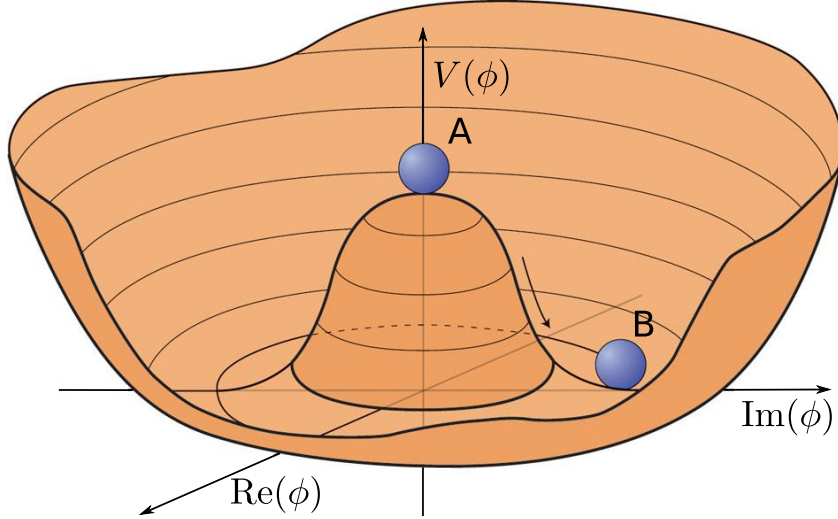
Figure 1.1.: Sketch of the effective potential of the Higgs field adopted from [34]. At high energies particles are located at \phi = 0 and do not interact with the Higgs field (A). The cylindrical symmetry of the system is conserved. At lower energies this symmetry is spontaneously broken, as the state of particle chooses one distinct minimum of the potential (B).
