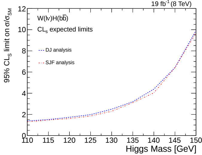
Figure 5.27.: Comparison between DJ (blue line) and SJF analyses (red line) in terms of expected limits. All analysis regions are combined. The diagram indicates that the SJF analysis yields better results in all cases.
