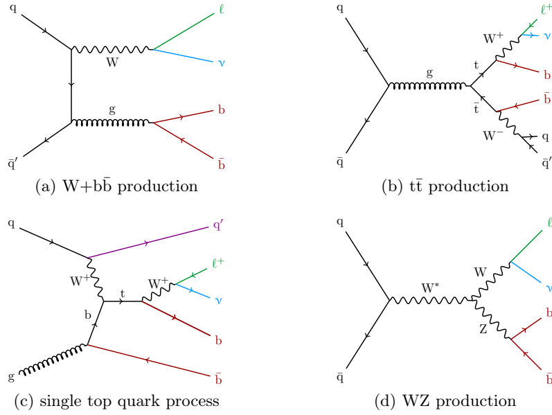
Figure 5.4.: Representative LO Feynman diagrams for important background processes to the WH search. To impart similarities in topology to the signal process, the same color code as in Figure 5.3 is introduced.
