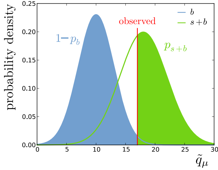
Figure 4.1.: Illustrative example of the \text{CL}_s value definition. The probability functions for the signal-plus-background s+b and the background-only b hypotheses are derived from simulation. Given a measurement with an observed value for the test statistic \tilde{q}_\mu , the \text{CL}_s value is defined as p_\mu/(1-p_b) , where p_\mu \equiv 1-p_{s+b} .
