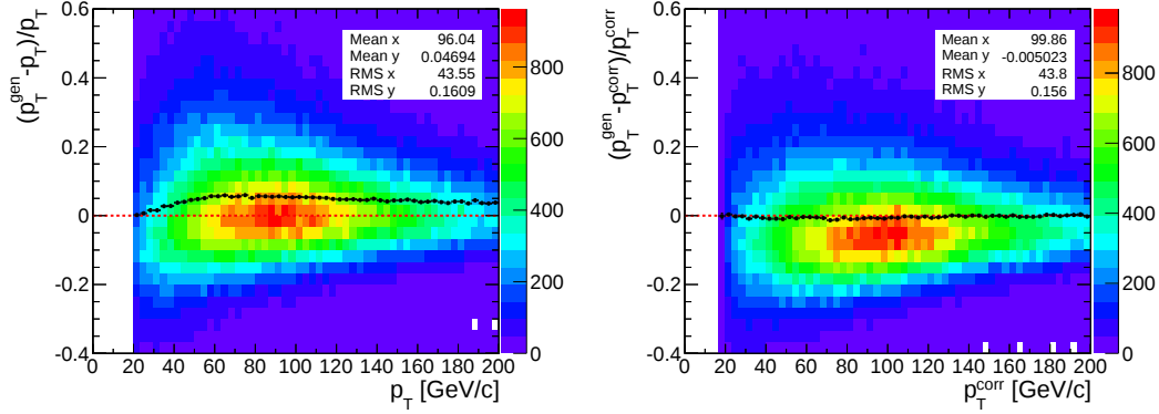
Figure 5.9.: Performance of filter jet regression on individual jet momenta. On the left side the relative difference between generated and reconstructed p_T over reconstructed p_T is shown before the correction. The black markers depict the mean values of each bin in p_T ( x -axis). A tendency towards values greater than zero is visible. The same diagram after applying the regression weights is shown on the right side. On the one hand, the mean values are now compatible with zero, and on the other hand the RMS value for the y -axis decreased. Interestingly, the relative difference between generated and reconstructed p_T peaks at zero before the correction. The improvements with respect to the mean and RMS values after applying the regression weight arise mainly from the corrections of the tails of these distributions.
