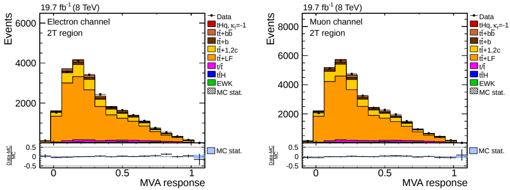
Figure 6.17.: Data/MC comparison of classification MVA response in the 2T region. The MC templates are normalized to data. The distributions agree well with each other.
