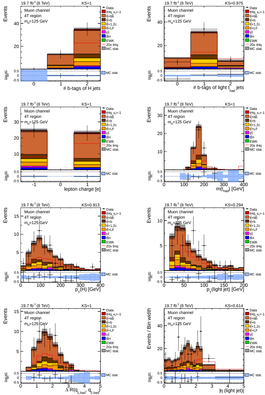
Figure 6.20.: MVA classification input variables for the muon channel in the 4T region. To facilitate shape comparisons the simulation is normalized to the number of events in data. In all variables good agreement between data and simulation is found. The corresponding distributions in the electron channel are provided in Figure B.9.
