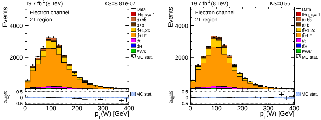
Figure 6.4.: Effect of top quark p_T reweighting in the 2T control region for the electron channel. The transverse momentum of the reconstructed W boson before (left) and after (right) applying the top quark p_T correction factors is shown. In both distributions the simulation is normalized to fit the observed events in data. The ratio in the left diagram indicates a clear slope that is cured in the right diagram. The KS-test probabilities are also vastly improved.
