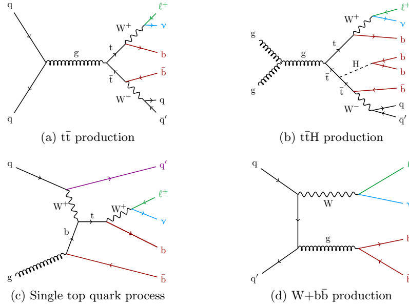
Figure 6.3.: Representative LO Feynman diagrams for the main background processes contributing to the tHq production. Similar to the WH search t\bar{t} (a), single-top quark (c) and W +jets production (d) needs to be taken into account. In this analysis also the production of a Higgs boson in association with t\bar{t} pairs (b) is considered.
