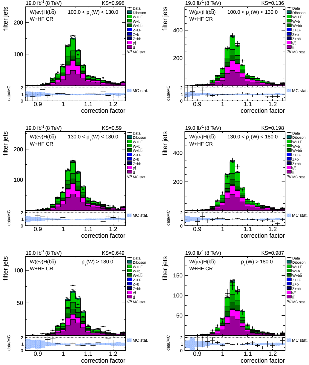
Figure 5.8.: Filter jet correction factors in the W+HF control region for the W(e\nu)H (left column) and the W(\mu\nu)H channel (right column). Data/MC comparisons are shown for the low p_T region (top row), intermediate p_T region (middle row) and the high p_T region (bottom row). Overall good agreement is found, indicated by the Kolmogorov-Smirnov-test probabilities printed on the upper right corner of each figure.
