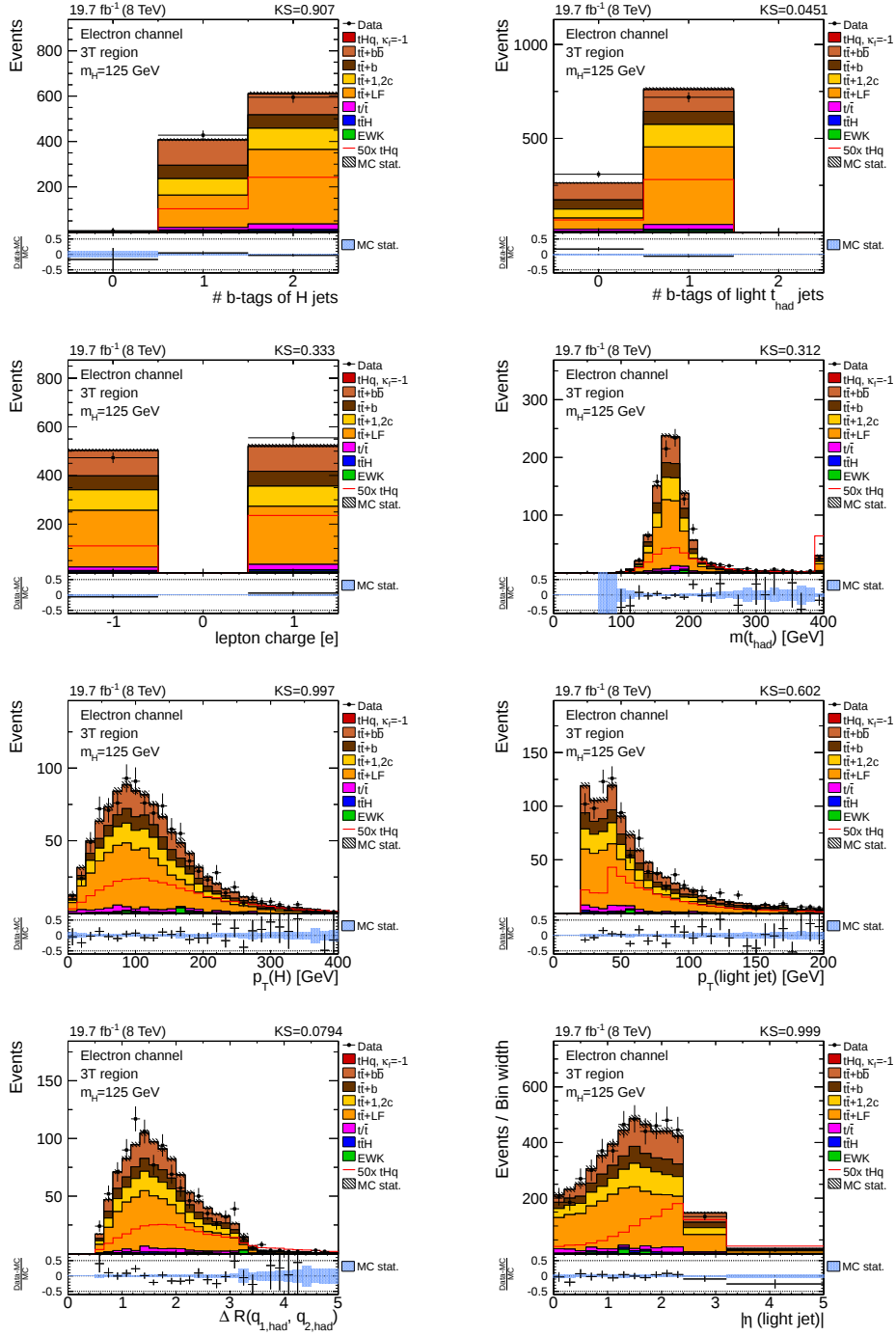
Figure B.8.: MVA classification input variables for the electron channel in the 3T region.
