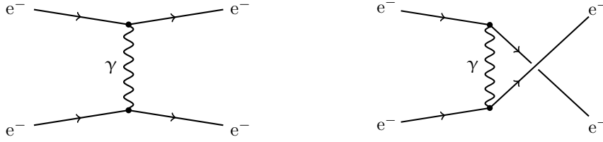
Figure 1.2.: Leading-order Feynman diagrams for Møller scattering. The lines and vertices represent mathematical terms for the calculation of the cross sections, in which all possible diagrams need to be summed. Throughout this thesis time is evolving from left to right.
