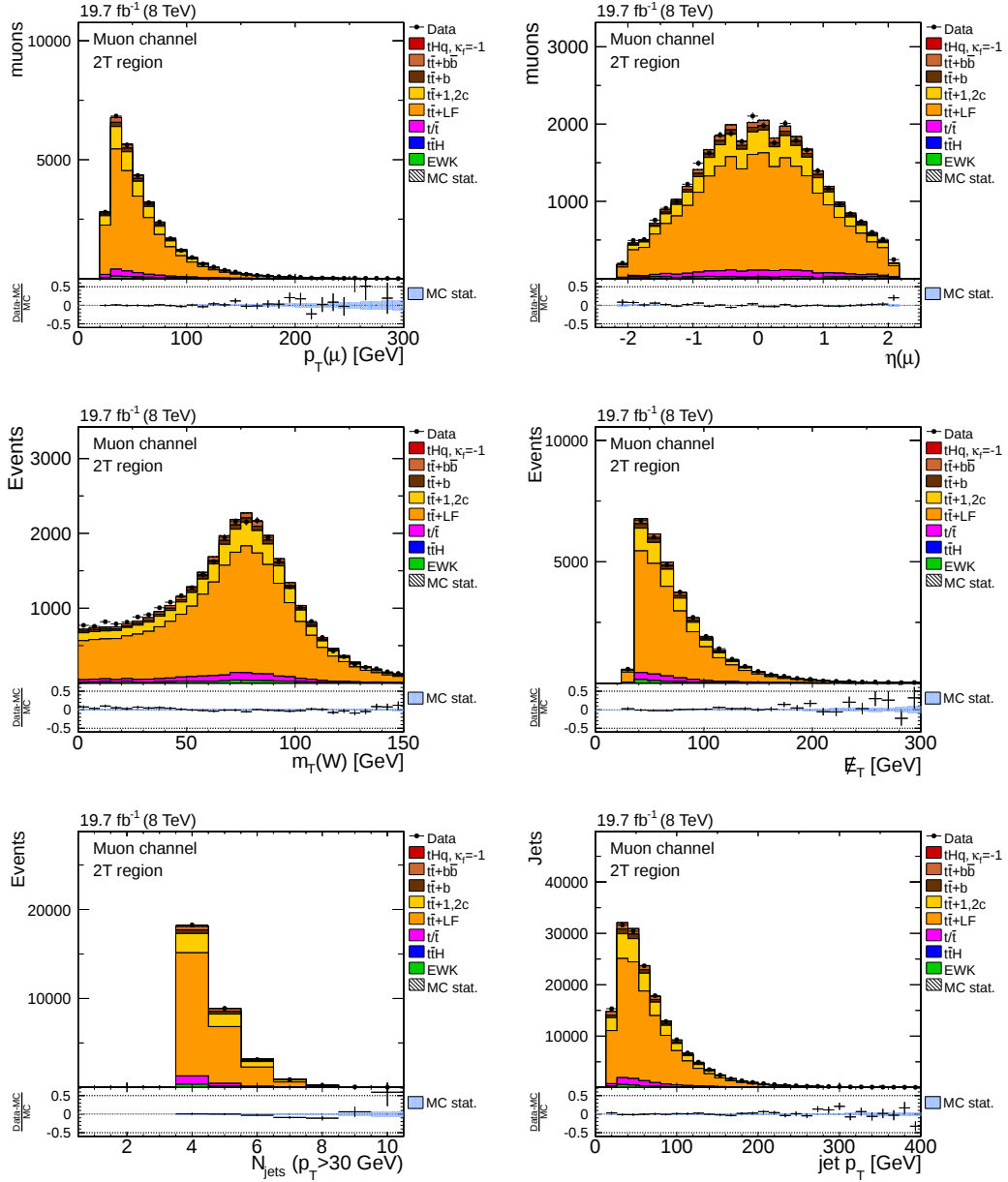
Figure B.1.: Event information variables for the muon channel in the 2T region. The number of simulated events is normalized to data. Overall good agreement between data and simulation is found.
