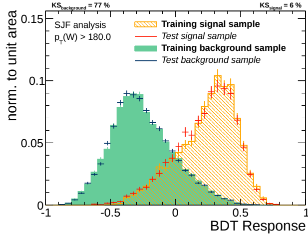
Figure 5.23.: BDT response for the SJF analysis in the high p_T region. The distributions are separated for signal and background events, and for training and testing samples. Good agreement is found by comparing the performance of the classification between training and testing samples.
