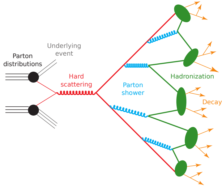
Figure 3.1.: Scheme of the Monte Carlo event generation process adopted from [86]. The proton characteristics are defined by parton distribution functions. The initial and final state partons participating in the hard scattering process are passed to the parton shower step, where soft radiations are generated. Colorless hadrons are formed in the hadronization step. Finally, the decay of unstable particles is simulated. Beyond, the remnants of the protons can interact further. The contributions from this process, known as underlying event, are simulated as well.
