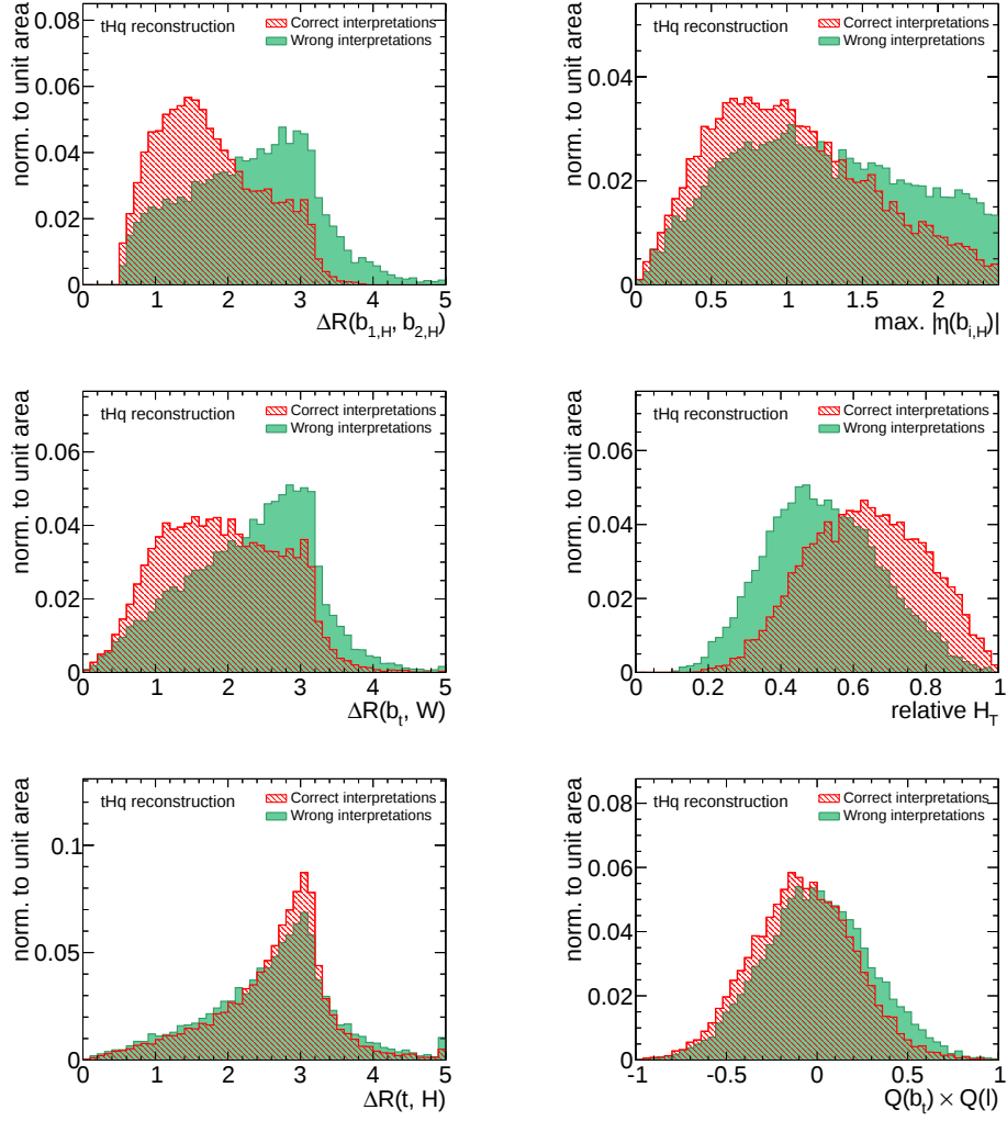
Figure B.3.: Remaining input variables for reconstruction under the tHq hypothesis.
