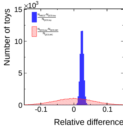
Figure B.2.: Closure test results for the ABCD method. In total 50,000 pseudo experiments are drawn with varied yields for each process. The blue histogram shows the relative difference between the QCD prediction calculated via the ABCD method ( N_{\text{ABCD}} ) and the drawn number of events in region A ( N_{\text{QCD,toy}} ). For the sake of completeness the relative difference of N_{\text{QCD,toy}} and the number of events predicted by simulation in A ( N_{\text{QCD,MC}} ) is depicted in hatched red.
