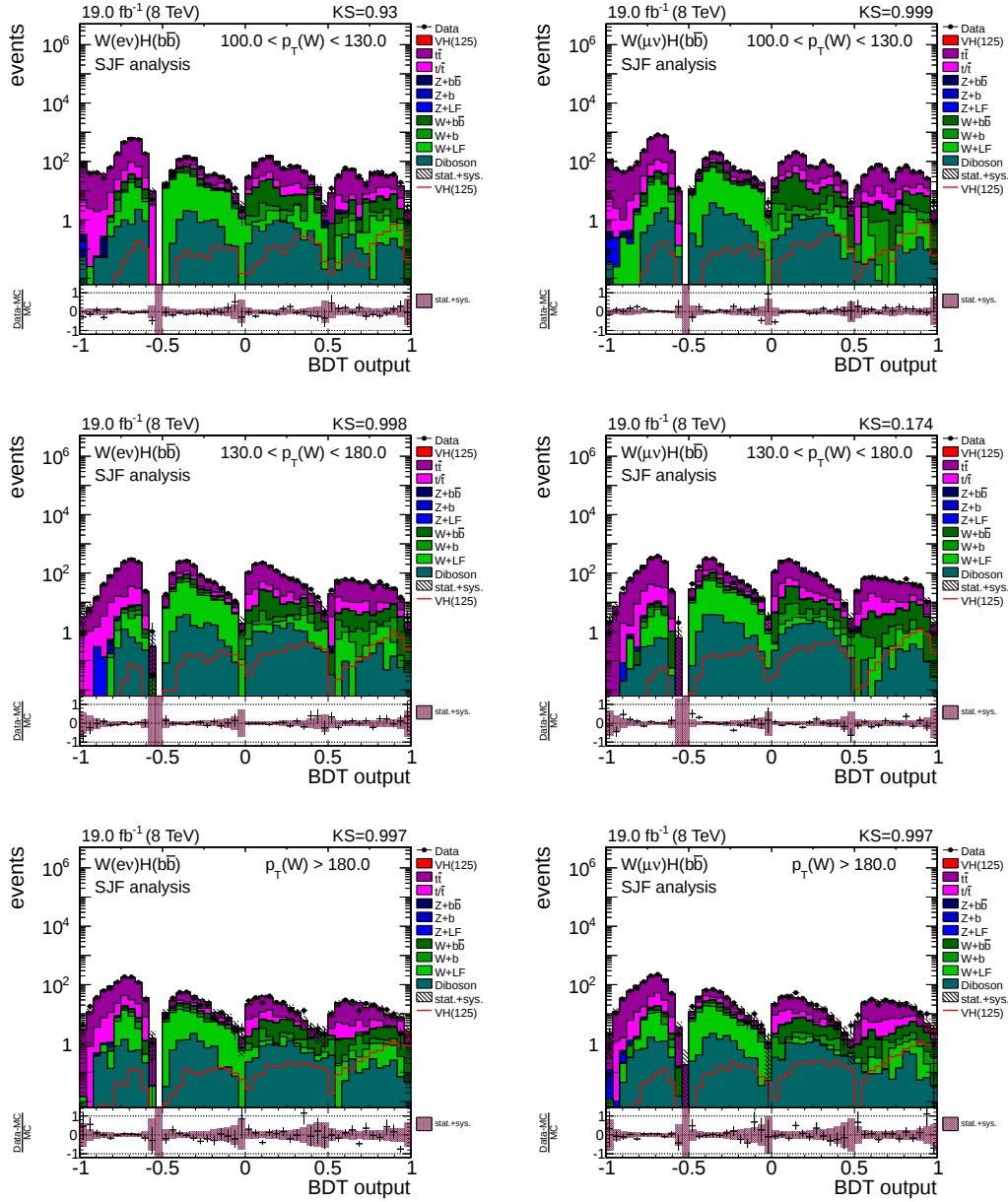
Figure 5.28.: Post-fit distributions for the m_H(125) training separately for all signal regions. The plotted uncertainties include both statistical and systematical effects.
