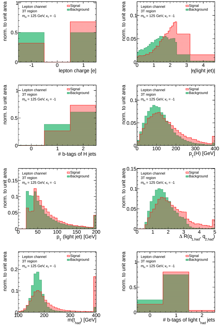
Figure 6.15.: Shapes of input variables for the final classification. The shapes are shown separately for signal and background processes and normalized to unit area.
