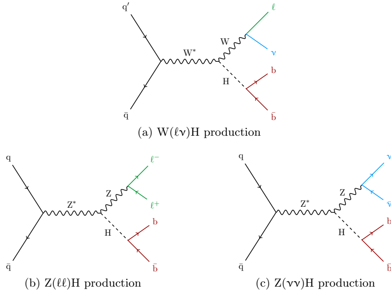
Figure 5.3.: Representative LO Feynman diagrams for VH production. The analysis is optimized for W(\ell\nu)H(b\bar{b}) production (a). Contributions from ZH processes shown in (b) and (c) are also taken into account. To facilitate the comparisons with diagrams of the background processes a color code is introduced. In the final state b quarks are indicated in red, charged leptons are green and neutrinos that give rise to missing transverse energy are blue.
