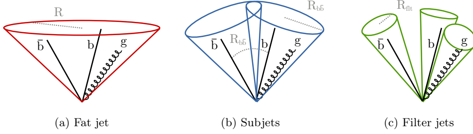
Figure 3.4.: Illustrative overview of the Subjet/Filter jet algorithm for reconstructing the decay H \rightarrow b\bar{b} , based on [124]. In a first step fat jets are clustered with the CA algorithm using R = 1.2 as size parameter (a). The clustering is then withdrawn until a certain mass drop criterion is reached (b). Finally, filter jets are obtained by re-clustering inside the subjets with a size parameter of R_{\text{flt}} = \min[0.3, R_{b\bar{b}}/2] (c). Therefore, filter jets have a smaller radius compared to the standard AK5 jets and are supposed to be more resilient against distortions from pile-up and underlying event.
