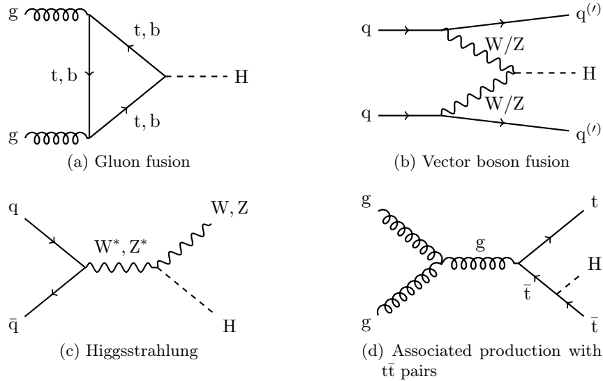
Figure 1.3.: Representative LO Feynman diagrams for the four main Higgs boson production.
