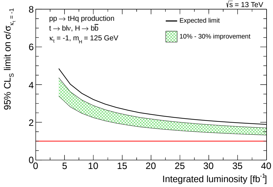
Figure 6.24.: Assumed sensitivity on tHq production with \kappa_t = -1 at 13 TeV. The results from Chapter 6 are extrapolated by scaling all processes according to the predicted cross sections in [210, 211]. The systematic uncertainties are simply scaled according to the higher luminosity for this study. In addition, the effect of possible 10% to 30% analysis improvement in terms of expected limits is shown.
