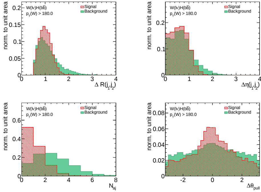
Figure 5.17.: Expected separation of BDT input variables in the DJ analysis (cont.). The signal and background distributions are normalized to unity.
