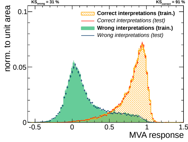
Figure 6.12.: MVA response in t\bar{t} reconstruction for correct and wrong interpretations. The shapes are shown separately for the training and test samples. The KS-test yields probabilities above 30% (wrong interpretations) and above 90% (correct interpretations), so no hint for overtraining is found.
