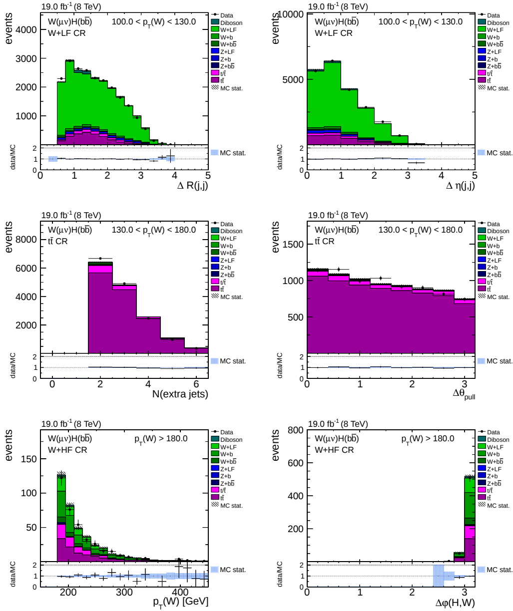
Figure 5.20.: DJ analysis input variables for the W(\mu\nu)H channel in different control regions as indicated within the diagrams (cont.). The simulation is scaled to luminosity and scale factors are applied. In all variables solid data/MC agreement is found. The corresponding distributions in the W(e\nu)H channel are presented in Figure A.3.
