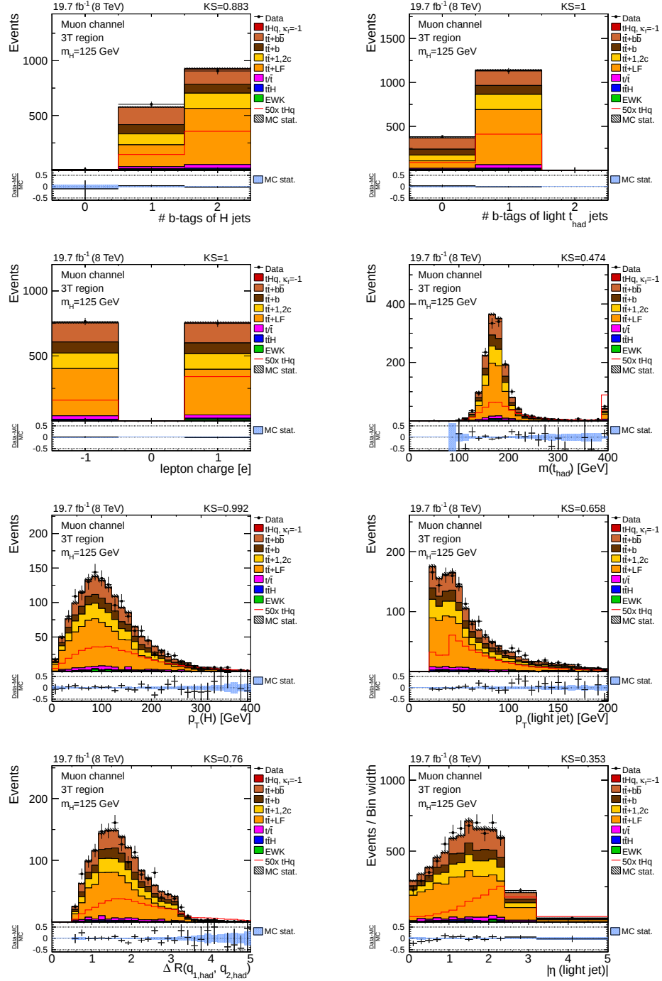
Figure 6.19.: MVA classification input variables for the muon channel in the 3T region. To facilitate shape comparisons the simulation is normalized to the number of events in data. In all variables good agreement between data and simulation is found. The corresponding distributions in the electron channel are provided in Figure B.8.
