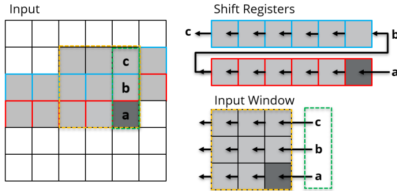
Figure 10. Color coded diagram demonstrating the buffer update process when a new pixel is read. We allocate two shift registers (red and blue) and an input window buffer (yellow). Reading pixel “a” causes pixel “b” and “c” to be popped from the shift register chain. Pixels “a”, “b”, and “c” are then used to update the input window.
