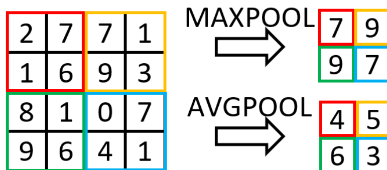
Figure 3. Comparison of MaxPooling and AveragePooling in two-dimensions with a (2, 2) pooling window. The different pooling windows are indicated by color.
