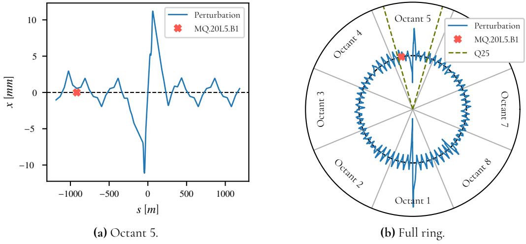
Figure 3.2: Closed orbit perturbation from a horizontal misalignment of the quadrupole \text{MQ.20L5.B1} plotted for Beam 1 in the horizontal plane. Plotted as an unfolded line from Q25 to Q25 in octant 5 (a) , and for the full ring (b) .
