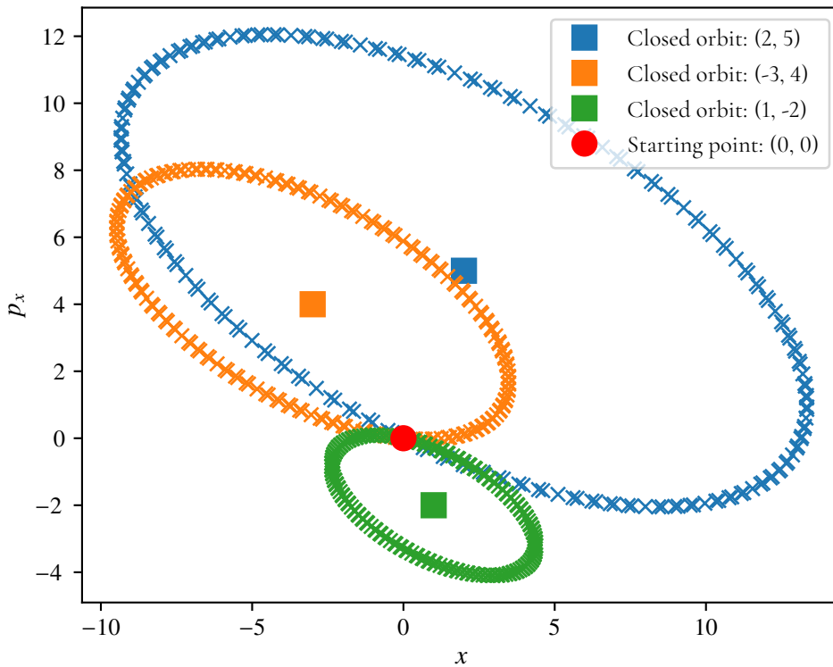
Figure 2.6: Phase-plots for a FODO lattice where L = 1 , f = \sqrt{2} and different closed orbits. Each cross in the graph corresponds to an iterate derived from the starting point (0, 0) with a closed orbit coded with the same color.
