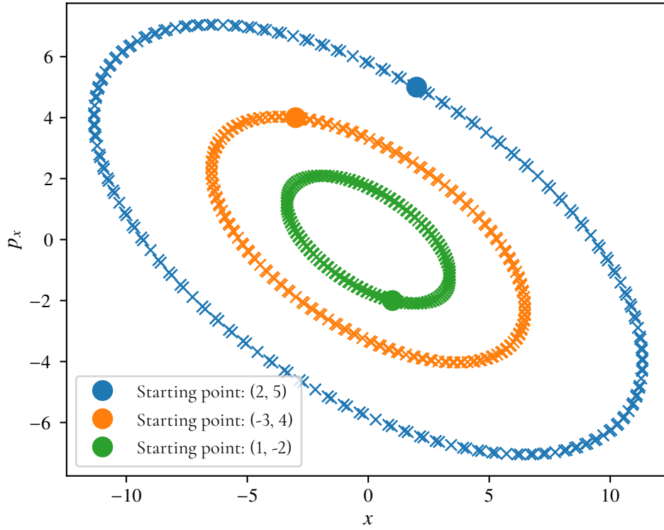
Figure 2.2: Phase plots for different initial phase space vectors in a FODO lattice where L = 1 , f = \sqrt{2} . Each cross corresponds to the horizontal phase space vector measured after having passed through the defocusing quadrupole in such a periodic FODO lattice.
