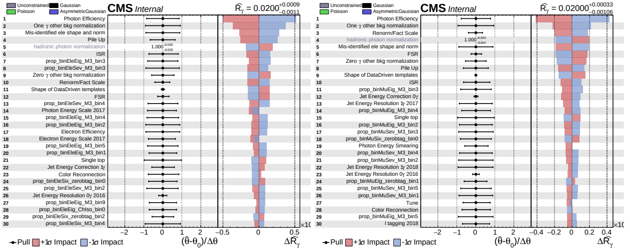
Figure 84: The impact plot that shows postfit pulls and constraints on nuisance parameters for R_\gamma fit in e + \text{jets} (left) and \mu + \text{jets} (right) separately to Asimov data for full Run 2.
