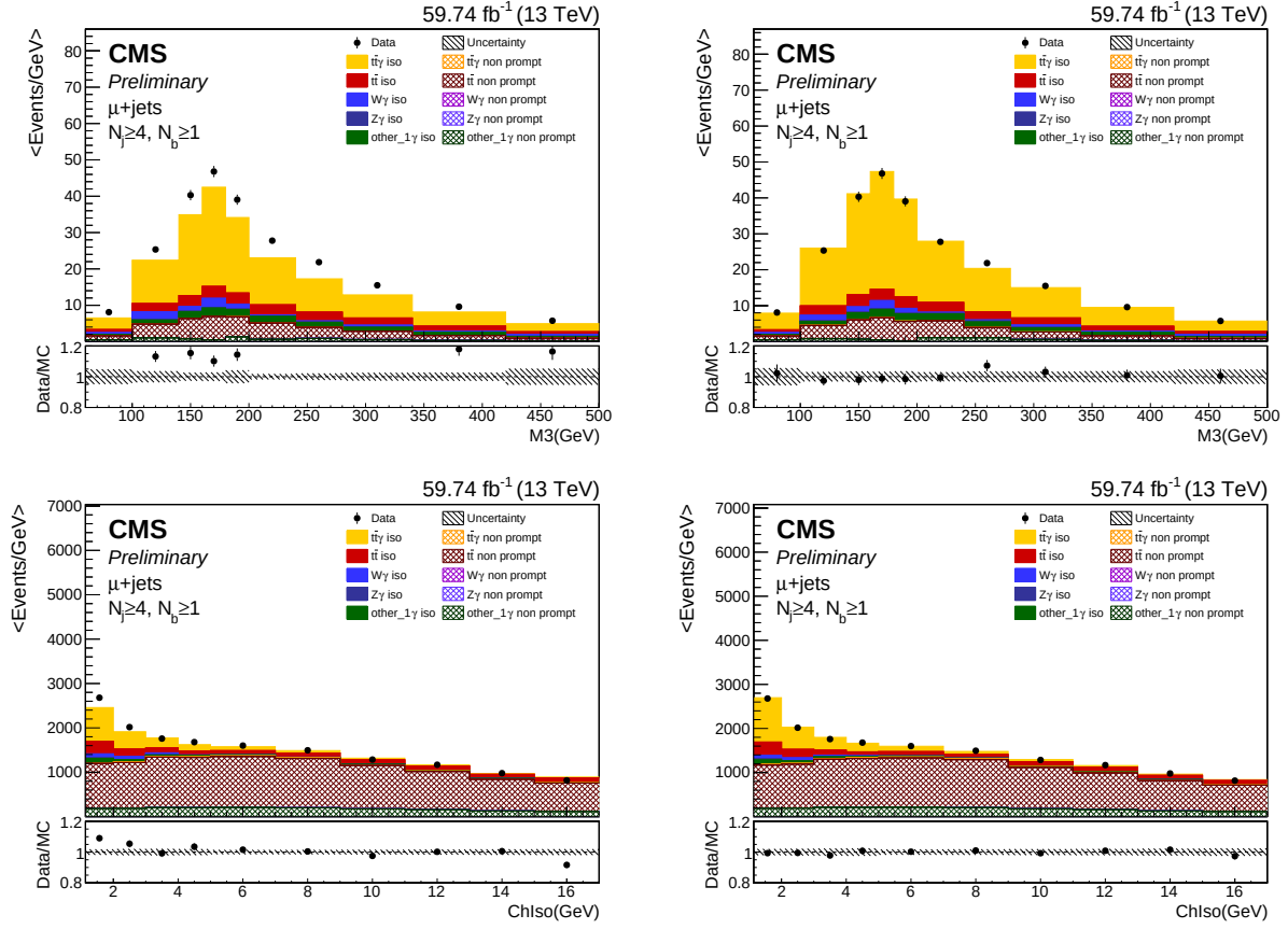
Figure 165: Pre-fit (left) and post-fit (right) plots for Data MC agreement for \sigma_{t\bar{t}\gamma} fitting in the signal region for M_3 (top) and ChIso (bottom) for \mu channel in 2018 data.
