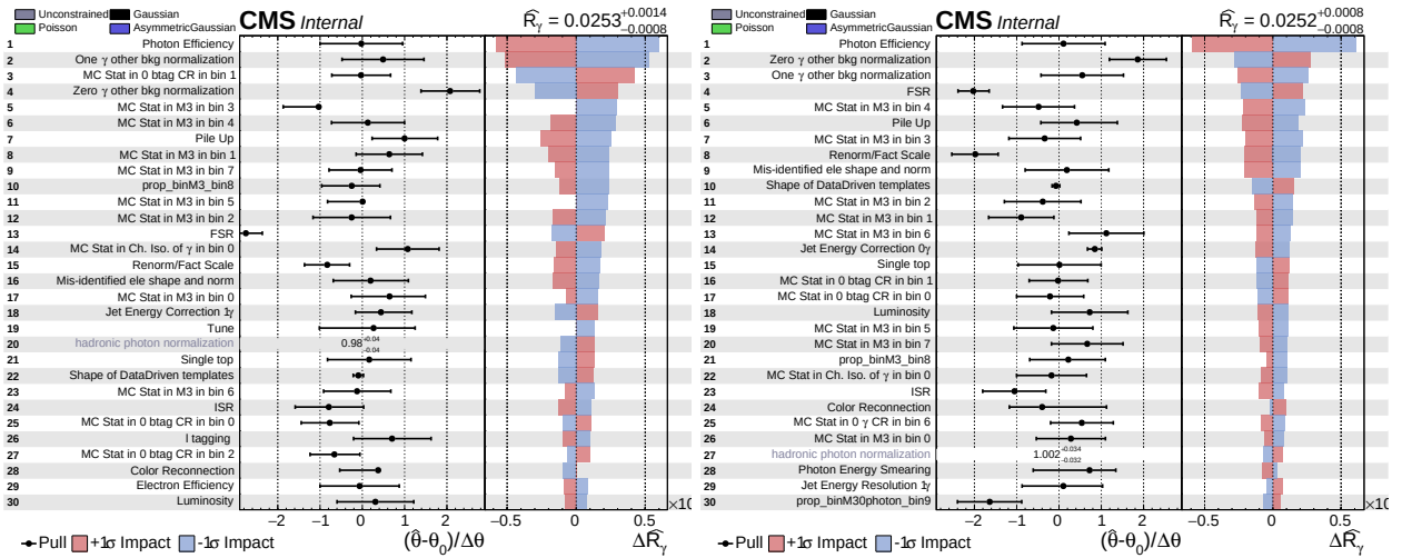
Figure 107: The impact plot that shows postfit pulls and constraints on nuisance parameters for R_\gamma fit in e + \text{jets} (left) and \mu + \text{jets} (right) separately to 2018 data.
