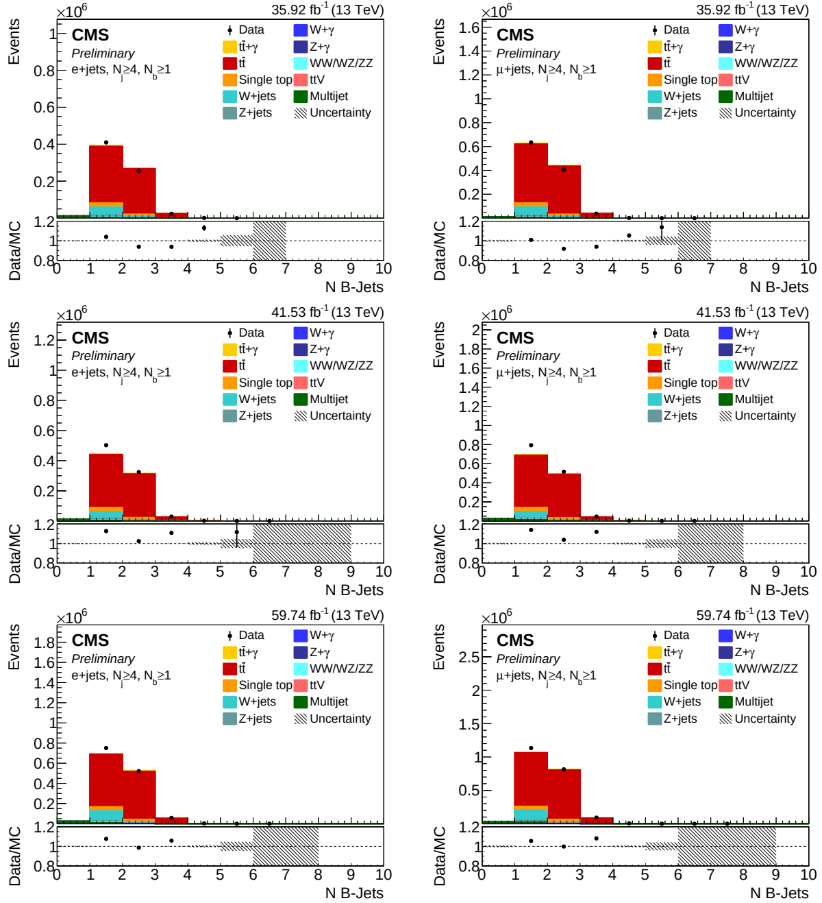
Figure 122: The number of b tagged jets distribution in 0 \gamma control region with N_j \geq 4, N_b \geq 1 in e + \text{jets} and \mu + \text{jets} for 2016(top), 2017(middle), and 2018(bottom).
