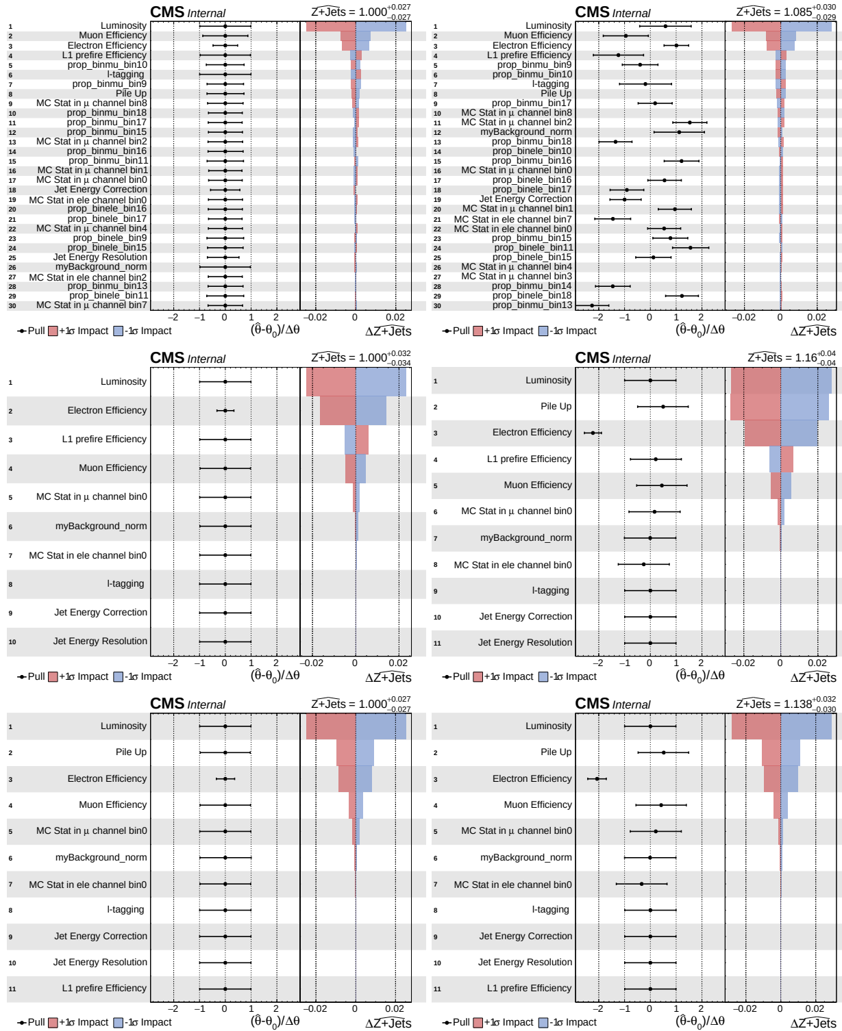
Figure 53: The impact plot shows postfit pulls and constraints on nuisance parameters for the Z + \text{jets} scale factor fit to Asimov data (left) and data (right) for 2016 (top), 2017 (middle), and 2017 (bottom), respectively.
