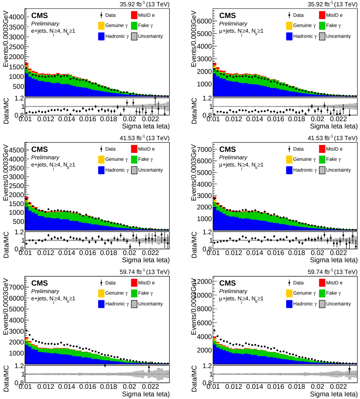
Figure 137: The distribution of the focused \sigma_{i\eta\eta} with no cut in Charge hadron isolation in the signal region ( N_j \geq 4, N_b \geq 1 ) split by photon category in e + \text{jets} (L) and \mu + \text{jets} (R) for 2016(top), 2017(middle), and 2018(bottom). The sideband region is defined as 0.011 \leq \sigma_{i\eta\eta} \leq 0.021 .
