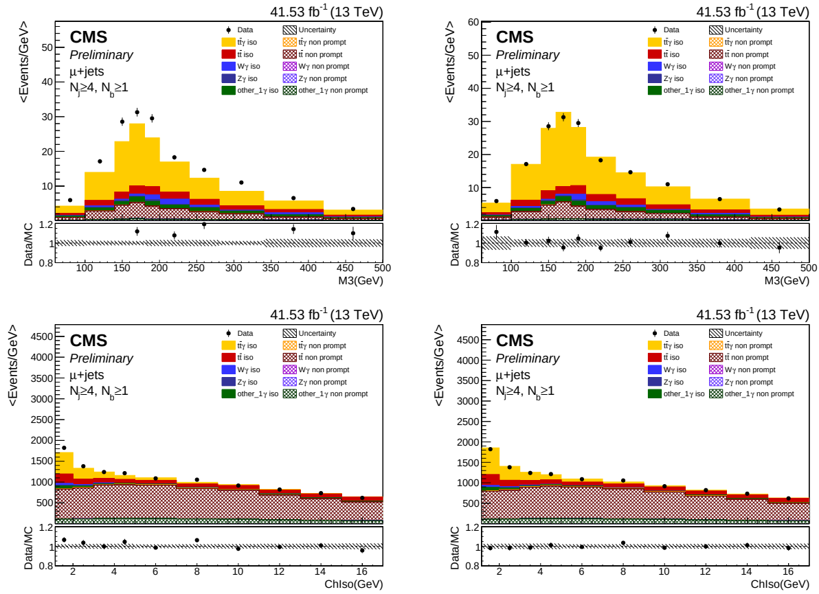
Figure 159: Pre-fit (left) and post-fit (right) plots for Data MC agreement for \sigma_{t\bar{t}\gamma} fitting in the signal region for M_3 (top) and ChIso (bottom) for \mu channel in 2017 data.
