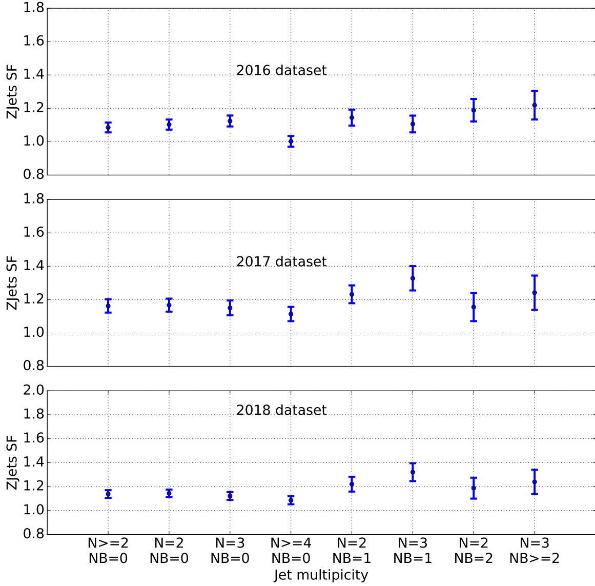
Figure 52: The comparison of the Z + \text{jets} scale factors from control regions with different number of jets and b-tagged jets for 2016, 2017, 2018. This is a graphical representation of Table 28.
