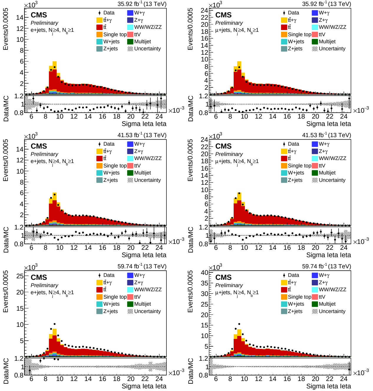
Figure 135: The distribution of the \sigma_{i\eta i\eta} with no cut in Charge hadron isolation in the signal region ( N_j \geq 4, N_b \geq 1 ) in e + \text{jets} (L) and \mu + \text{jets} (R) for 2016(top), 2017(middle), and 2018(bottom). The sideband region is defined as 0.011 \leq \sigma_{i\eta i\eta} \leq 0.021 .
