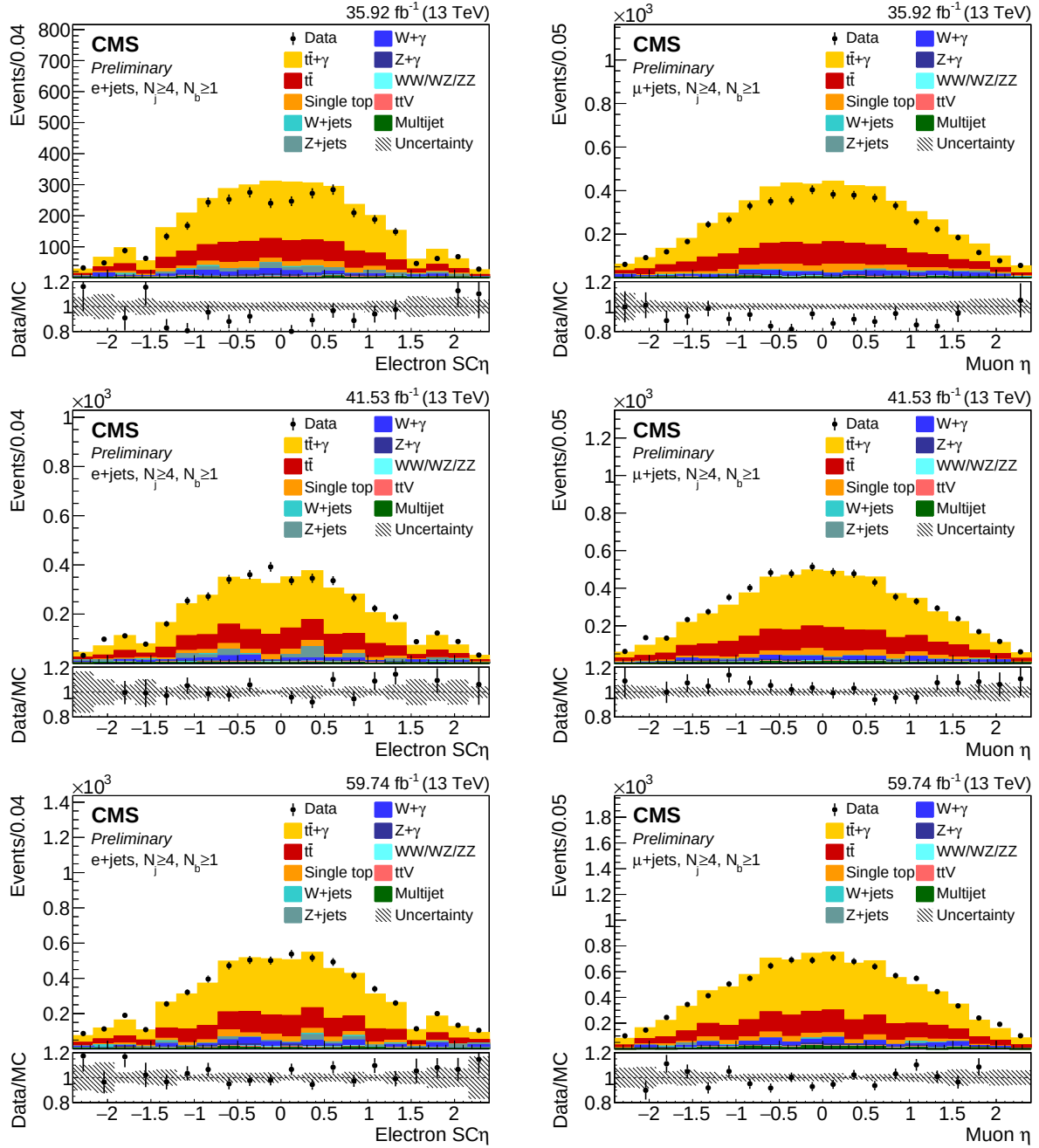
Figure 125: The electron(L) and muon(R) \eta distribution in the signal region ( N_j \geq 4, N_b \geq 1 ) in e + \text{jets} and \mu + \text{jets} for 2016(top), 2017(middle), and 2018(bottom).
