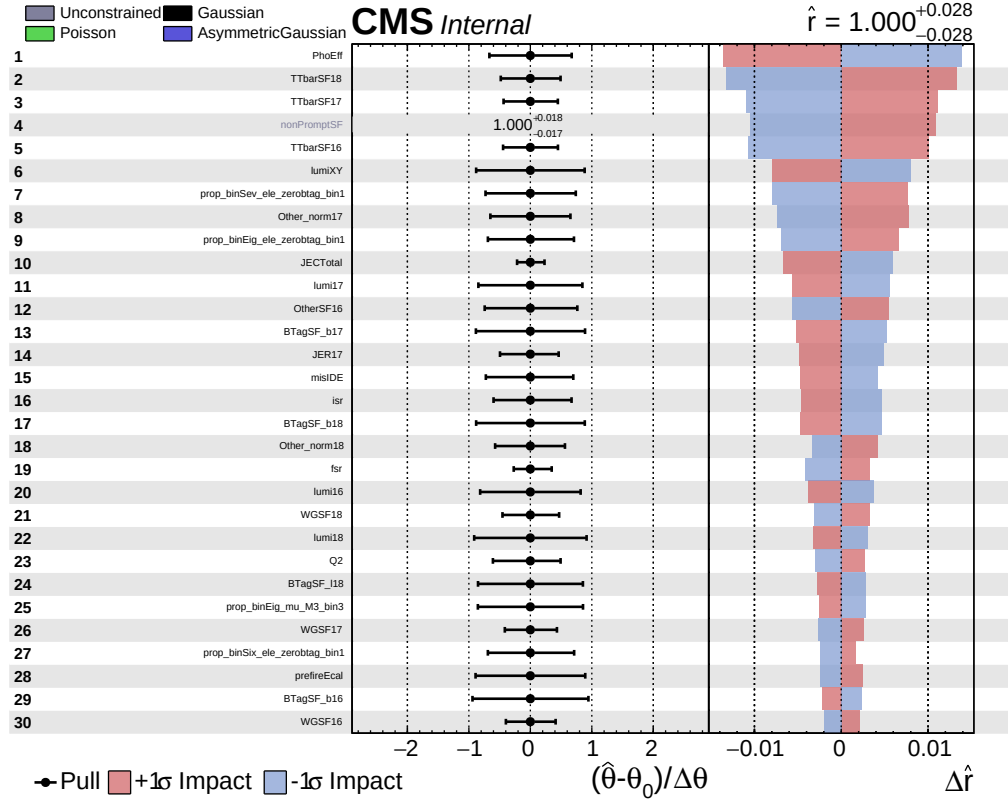
Figure 72: The impact plot that shows postfit pulls and constraints on nuisance parameters for t\bar{t}\gamma fit to Asimov data for full Run 2.
