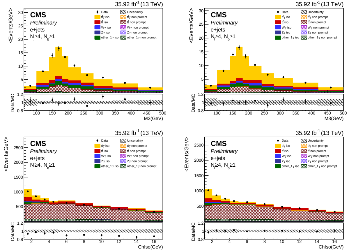
Figure 150: Pre-fit (left) and post-fit (right) plots for Data MC agreement for \sigma_{t\bar{t}\gamma} fitting in the signal region for M_3 (top) and ChIso (bottom) for e channel in 2016 data.
