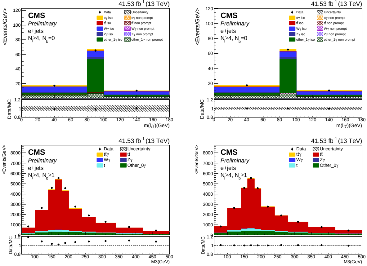
Figure 157: Pre-fit (left) and post-fit (right) plots for Data MC agreement for \sigma_{t\bar{t}\gamma} fitting in zero btag control region (top) and zero photon control region (bottom) for e channel in 2017 data.
