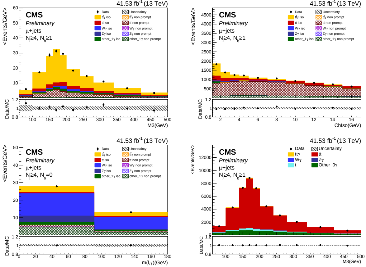
Figure 161: Post-fit plots for Data MC agreement in \frac{\sigma_{t\bar{t}\gamma}}{\sigma_{t\bar{t}}} fitting for M_3 and \text{ChIso} in the signal region (top left and top right, respectively), and zero btag control region and zero photon control region (bottom left and bottom right) for \mu channel in 2017 data.
