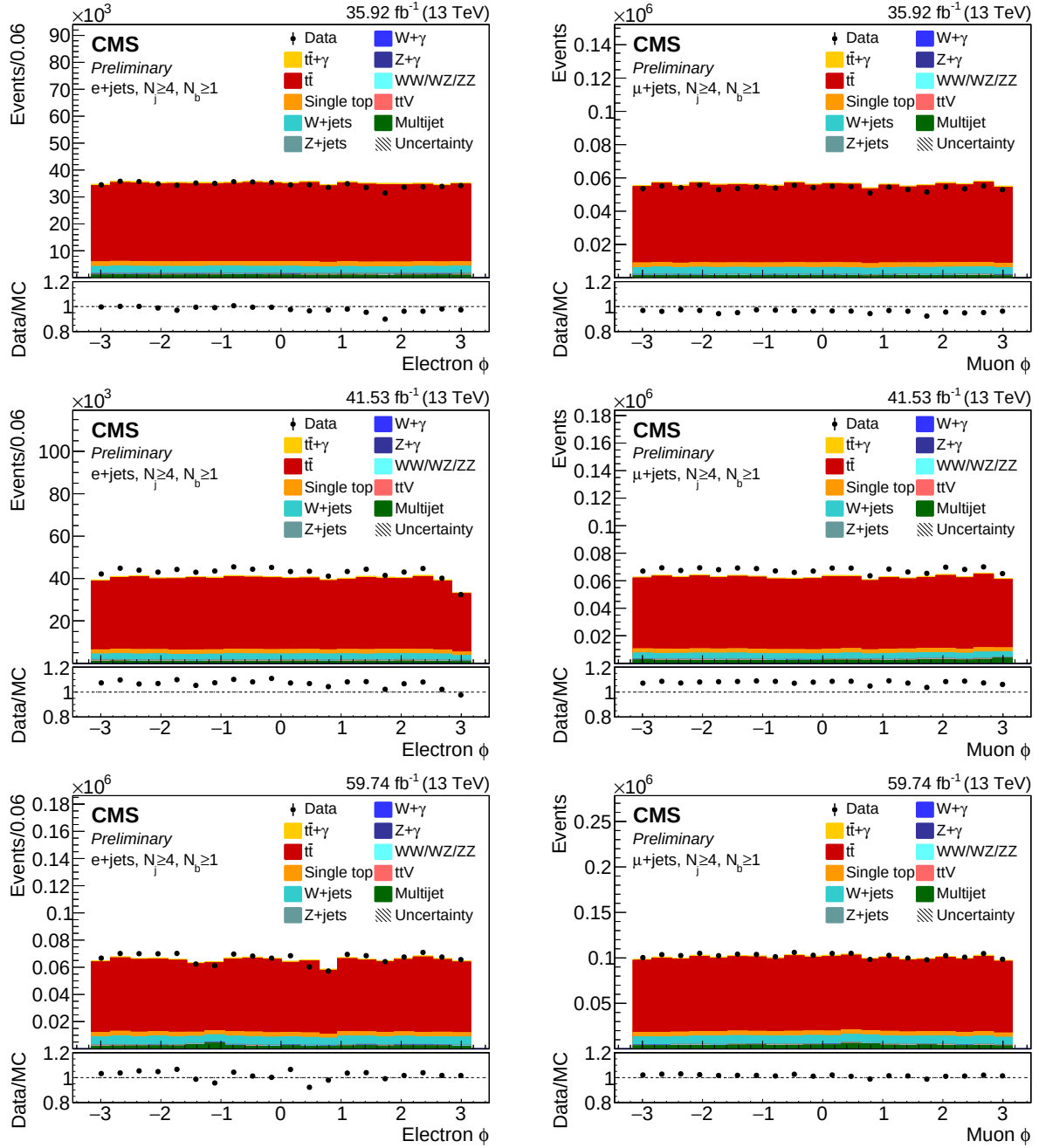
Figure 120: The electron(L) and muon(R) \phi distribution in 0 \gamma control region with N_j \geq 4 , N_b \geq 1 in e + jets and \mu + jets for 2016(top), 2017(middle), and 2018(bottom).
