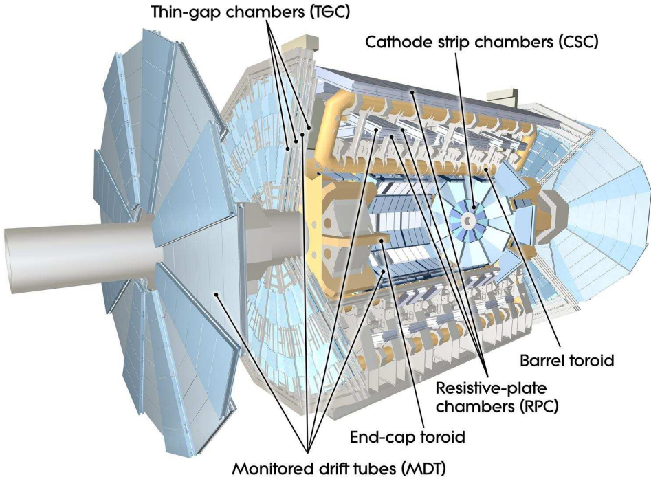
Figure 3.12: Overview of the muon chambers.
