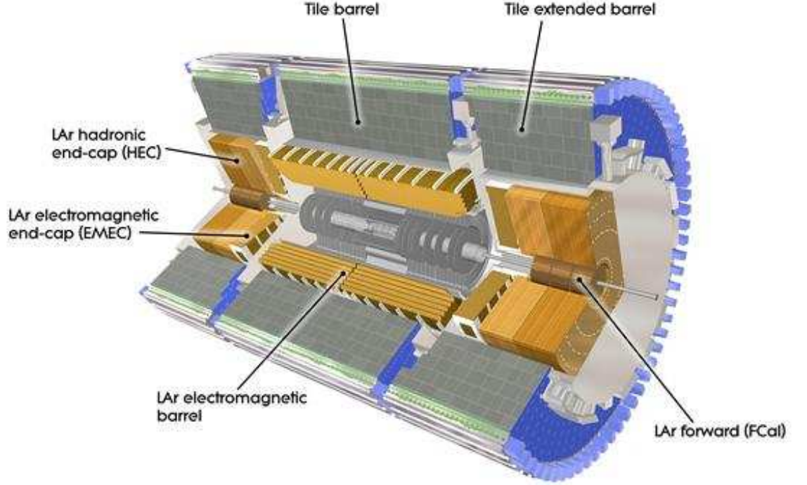
Figure 3.10: Schematic view of the calorimeters.
