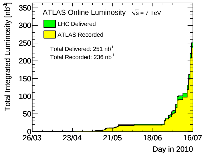
Figure 3.2: Daily update of the total integrated luminosity at ATLAS, since the LHC startup.
