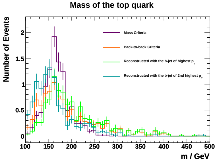
Figure 5.5: Top mass distributions reconstructed with the highest momentum b -jet (green), the second highest momentum b -jet (blue). The distributions chosen according to the “Mass Criteria” and the “Back-to-back Criteria” are represented in purple and orange respectively.
