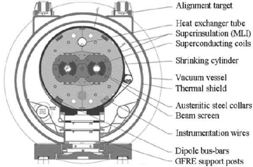
Figure 3.3: Dipole system of the LHC, extrated from reference [32]
