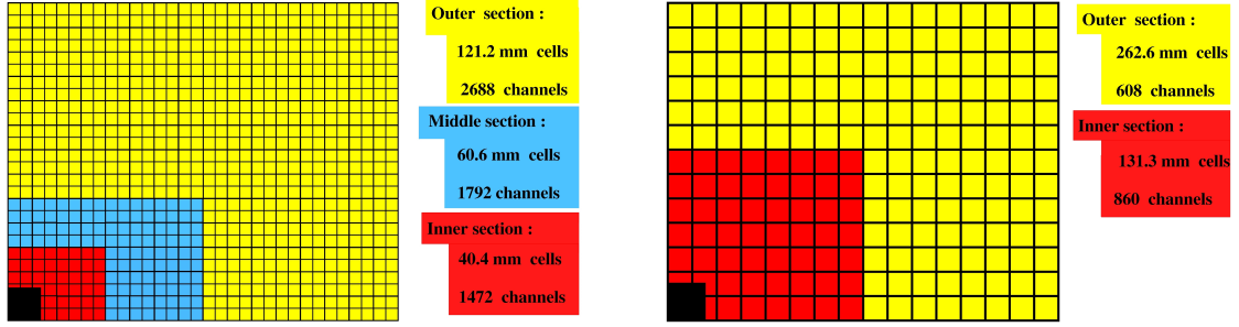
Figure 2.9: Cell pattern of SPD, PS and ECAL (left), and of HCAL (right).
