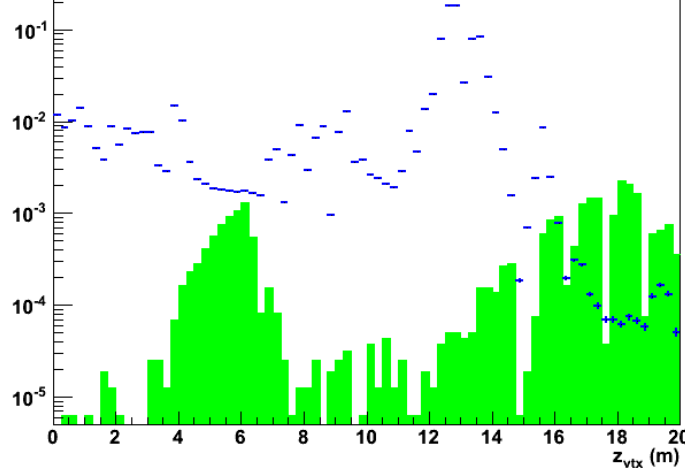
Figure 4.1: z -coordinate of the end vertex of the decay products of B_s^0 \rightarrow \mu^+\mu^- (green filled histogram) and B \rightarrow h^+h'^- (blue histogram), along the z axis. The tracking system of LHCb covers the range in z between the origin and 9.5 m, and the muon system starts at z \sim 15 m. All histograms are normalized to the respective fraction of decay products with z -coordinate of the end vertex below 20 m.
