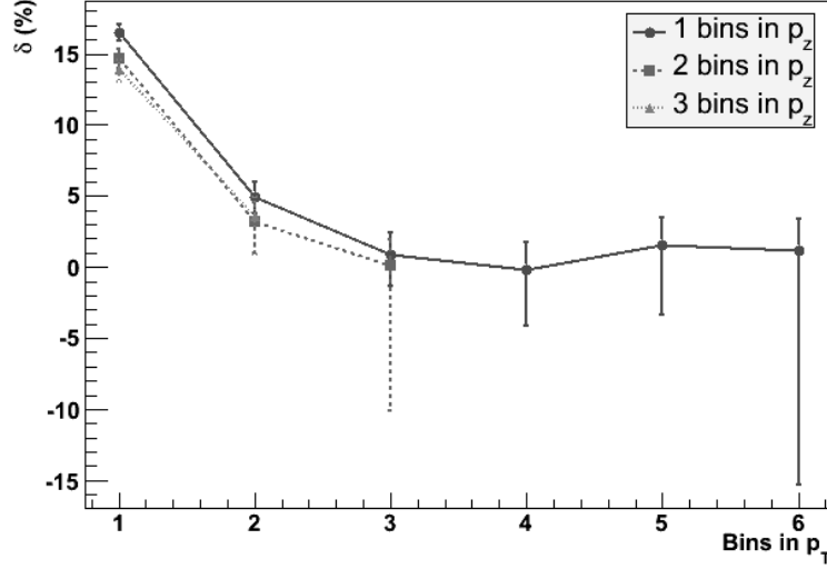
Figure 5.7: Relative bias in the efficiency estimation \delta as a function of the number of bins in p_T^B and for several numbers of bins in p_z^B , for B \rightarrow h^+h'^- , and having added and subtracted background from inclusive b\bar{b} . Vertical bars show the dispersion of the bias computed by the different MC toy-experiments, assuming 2 \text{ fb}^{-1} . The uncertainty on the bias is hence \sim \sqrt{2000} times smaller. Points having vertical bars of size above 20% are not displayed for visual reasons.
