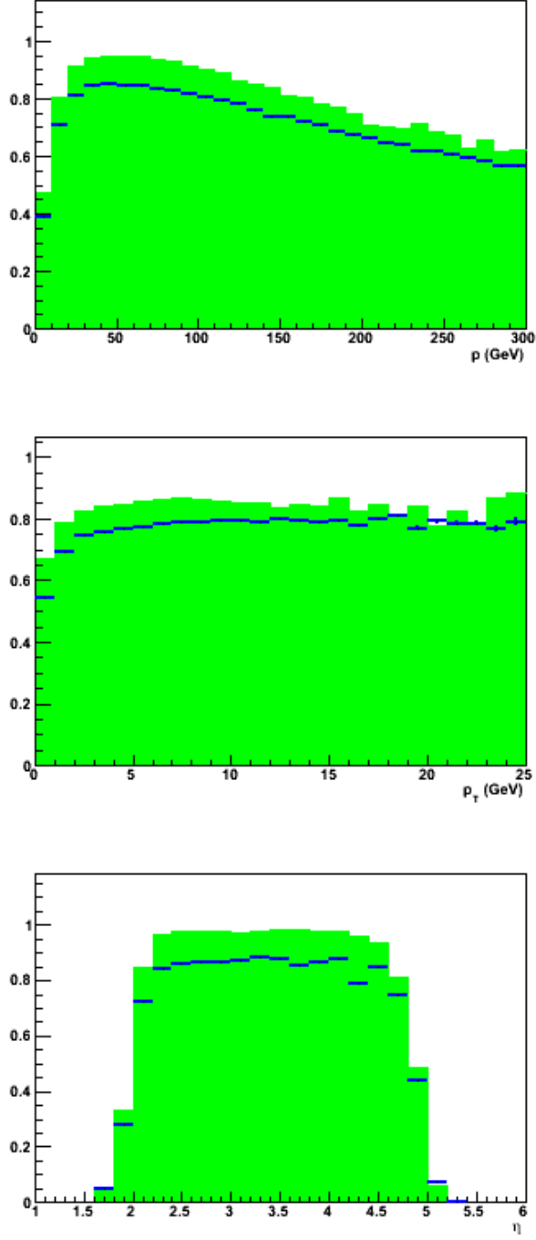
Figure 4.2: From top to bottom, track reconstruction efficiency of the decay products of B_s^0 \rightarrow \mu^+\mu^- (green filled histogram) and B \rightarrow h^+h'^- (blue histogram), as a function of the modulus of the momentum, the p_T and the pseudo-rapidity.
