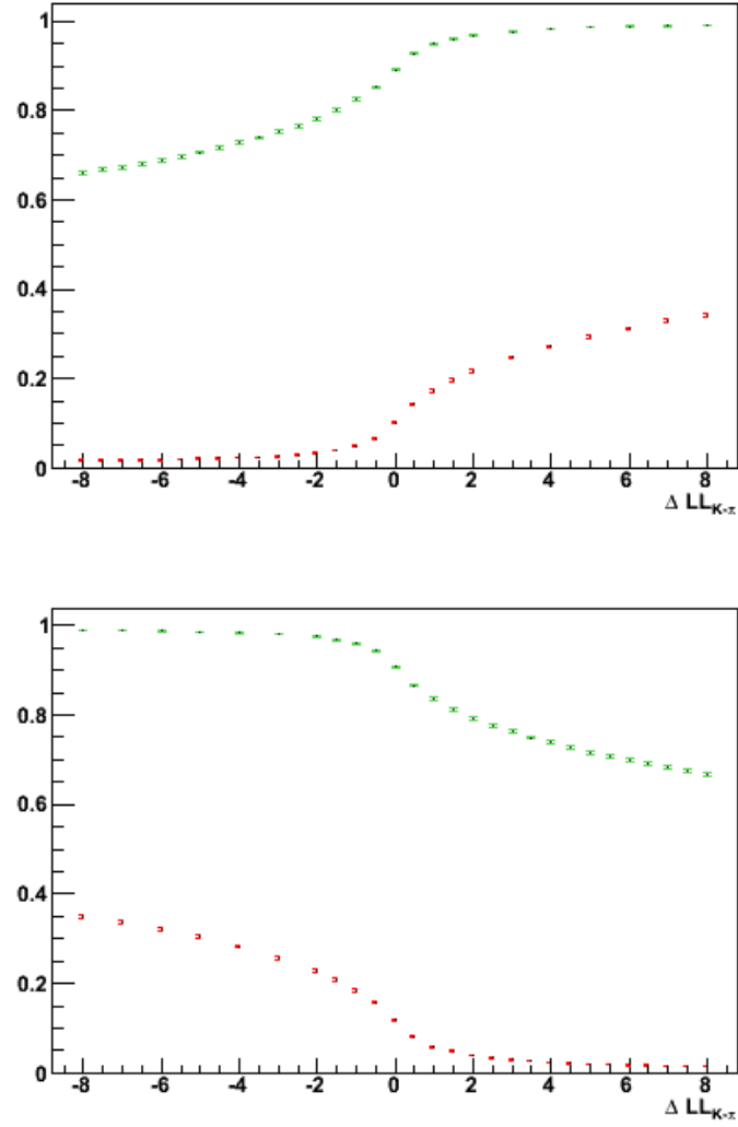
Figure 4.12: Efficiency (green points) and misidentification rate (red points) for hadrons produced in B \rightarrow h^+ h'^- decays identified as pions (top) and kaons (bottom), as a function of the threshold for \Delta LL_{K-\pi} . Events are required to satisfy the common selection.
