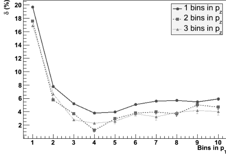
Figure 5.8: Relative bias in the efficiency estimation \delta as a function of the number of bins in p_T^B and for several numbers of bins in p_z^B , for B \rightarrow h^+h'^- satisfying GL > 0.25 , and having added and subtracted background from inclusive b\bar{b} . Vertical bars show the dispersion of the bias computed by the different MC toy-experiments, assuming 2 \text{ fb}^{-1} . The uncertainty on the bias is hence \sim \sqrt{2000} times smaller.
