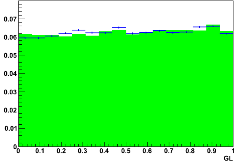
Figure 4.18: GL for B_s^0 \rightarrow \mu^+ \mu^- and B \rightarrow h^+ h'^- events passing the common selection. For B \rightarrow h^+ h'^- the cut on the IM is applied to the value computed using the most likely mass hypotheses. All histograms are normalized to unity.
