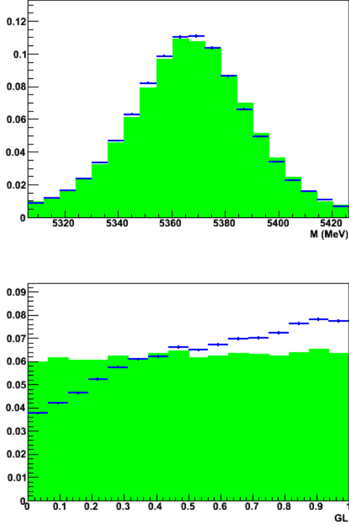
Figure 4.4: IM (top) and GL (bottom), for B_s^0 \rightarrow \mu^+\mu^- (green filled histogram) and B \rightarrow h^+h'^- (blue histogram), after the trigger and the original B_s^0 \rightarrow \mu^+\mu^- selection. The IM for each B \rightarrow h^+h'^- mode is computed assuming the mass hypotheses used at the generator level. In addition, the IM distribution of each B \rightarrow h^+h'^- mode has been shifted so that the true mass of the decaying B meson is situated at the mass of the B_s . All histograms are normalized to unity.
