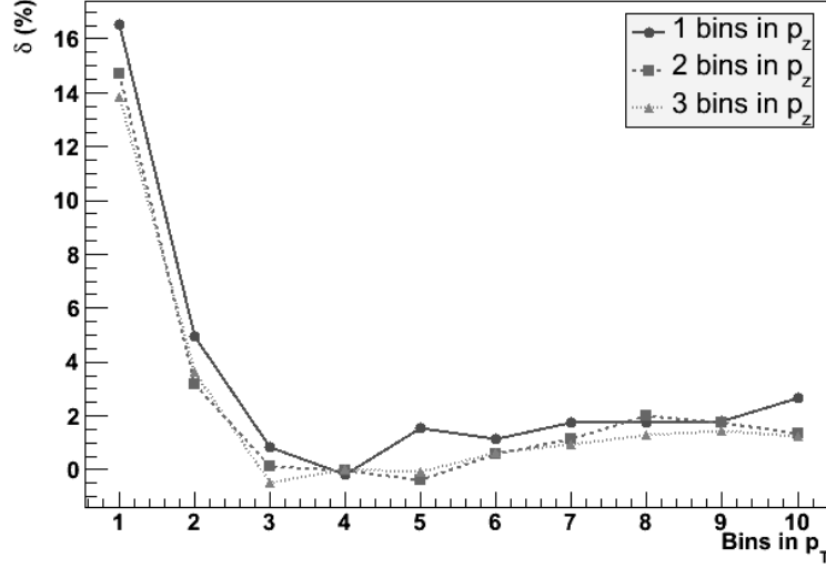
Figure 5.6: Relative bias in the efficiency estimation \delta , as defined in the text, as a function of the number of bins in p_T^B and for several numbers of bins in p_z^B , for B \rightarrow h^+ h'^- . Vertical bars showing the dispersion of the bias computed by the different MC toy-experiments assuming 2 \text{ fb}^{-1} are not displayed as they are smaller than the size of the points.
