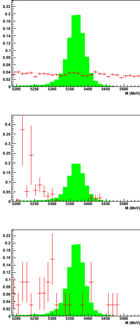
Figure 3.1: IM for events satisfying the offline selection, not including the trigger. Each plot represents signal (green filled histogram) against a specific background contribution (red histogram). From top to bottom: combinatorial dimuon background, misidentification from B^0 \rightarrow \pi^+\pi^- , and fake combination from B_c^+ \rightarrow J/\psi(\mu^+\mu^-)\mu^+\nu_\mu . All histograms are normalized to unity.
