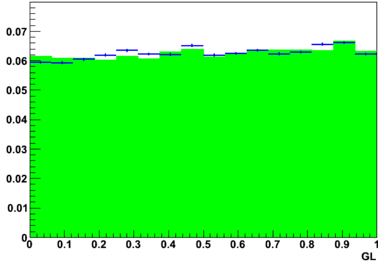
Figure 4.19: GL for B \rightarrow h^+h'^- passing the common selection, without including further cuts (green filled histogram), and requiring in addition both decay products to satisfy \Delta LL_{p-\pi} < 30 (blue histogram). All histograms are normalized to unity.
