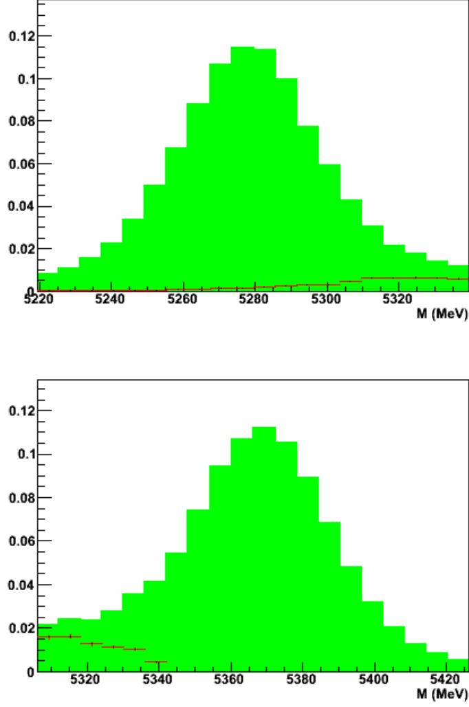
Figure 5.1: IM for B \rightarrow h^+ h'^- selected as B^0 \rightarrow K^+ \pi^- and B_s^0 \rightarrow K^+ K^- (top and bottom green filled histograms respectively), and for the respective background due to the cross-feed from B \rightarrow h^+ h'^- (red histograms). Events are required to satisfy the common selection. Signal histograms are normalized to unity, while background histograms are normalized respecting the ratio of yields.
