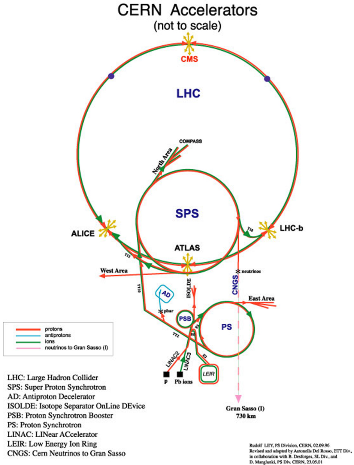
Figure 3.1: The layout of the accelerator complex at CERN (33).
