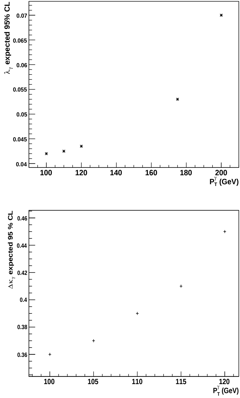
Figure 7.8: Top: The statistical sensitivity to the \lambda_\gamma anomalous coupling vs P_T^\gamma cut. Bottom: The statistical sensitivity to the \Delta\kappa_\gamma anomalous coupling vs P_T^\gamma cut.
