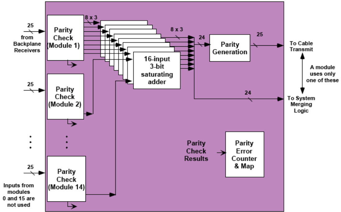
Figure 4.3: The flow of logical operation in a Cluster Processor Crate CMM(43).
