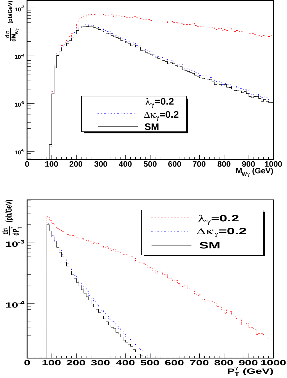
Figure 2.5: Top: a generator level plot of the M_{W\gamma} distribution at NLO for the SM, \lambda_\gamma = 0.2 and \Delta\kappa_\gamma = 0.2 cases. Bottom: a generator level plot of the P_T^\gamma distribution at NLO for the SM, \lambda_\gamma = 0.2 and \Delta\kappa_\gamma = 0.2 cases.
