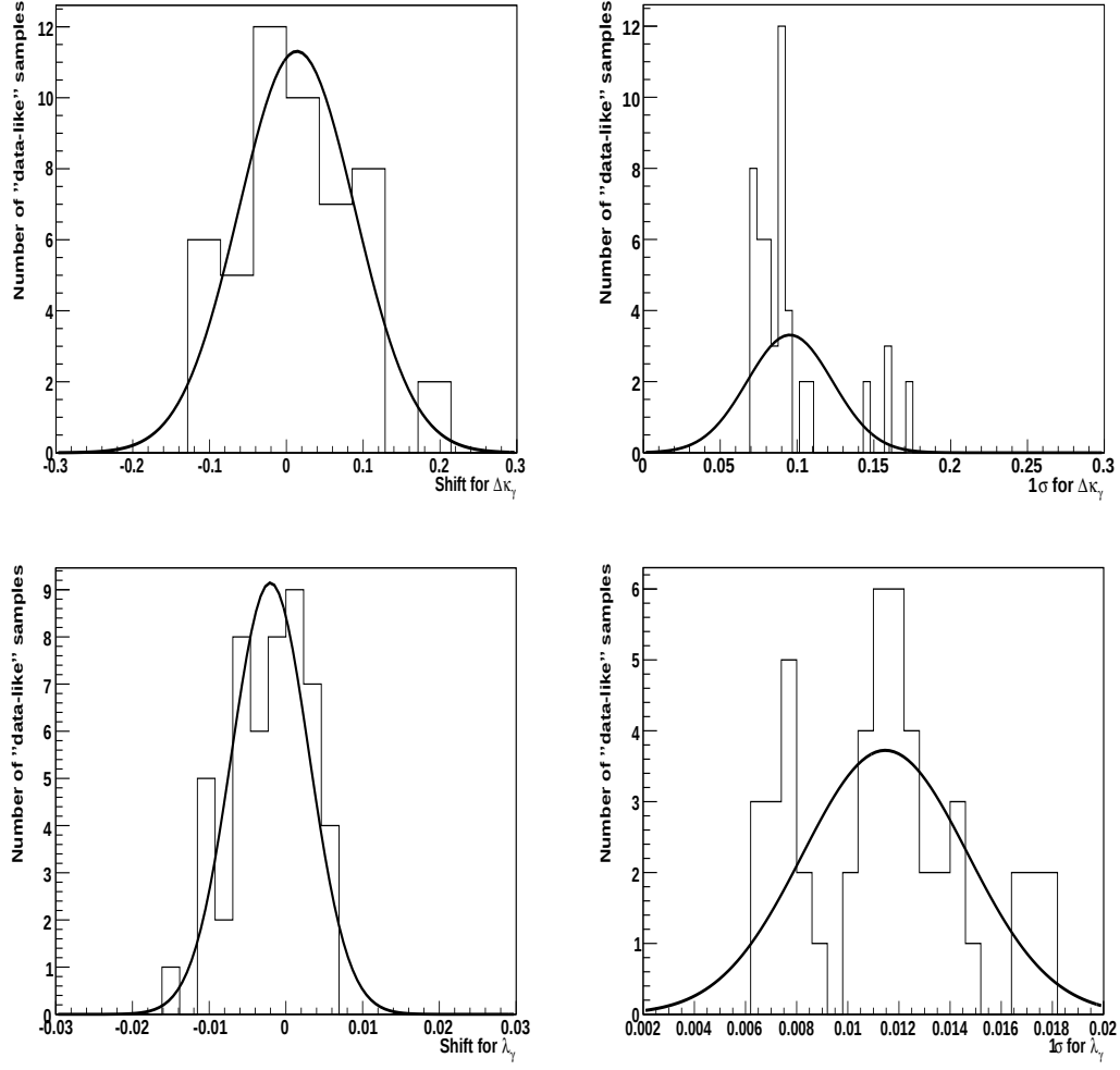
Figure 7.2: Top: The shift and 1\sigma standard deviation statistical error given by the fit from 50 “data-like” samples when fitting for \Delta\kappa_\gamma . The shift has a mean of 0.015\pm0.010 and an RMS of 0.072\pm0.008 . The 1\sigma standard deviation has a mean of 0.095\pm0.004 and an RMS of 0.028\pm0.003 . Bottom: The shift and 1\sigma standard deviation statistical error given by the fit from 50 “data-like” samples when fitting for \lambda_\gamma . The shift has a mean of -0.002\pm0.001 and an RMS of 0.0050\pm0.0005 . The 1\sigma standard deviation has a mean of 0.0115\pm0.0004 and an RMS of 0.0032\pm0.0003 . In all plots a Gaussian (solid line) has been fitted using a binned log-likelihood fit. The binning was chosen so that an acceptable goodness-of-fit, as reported by MINUIT (81), was found (see reference (80) for more details about goodness-of-fit).
