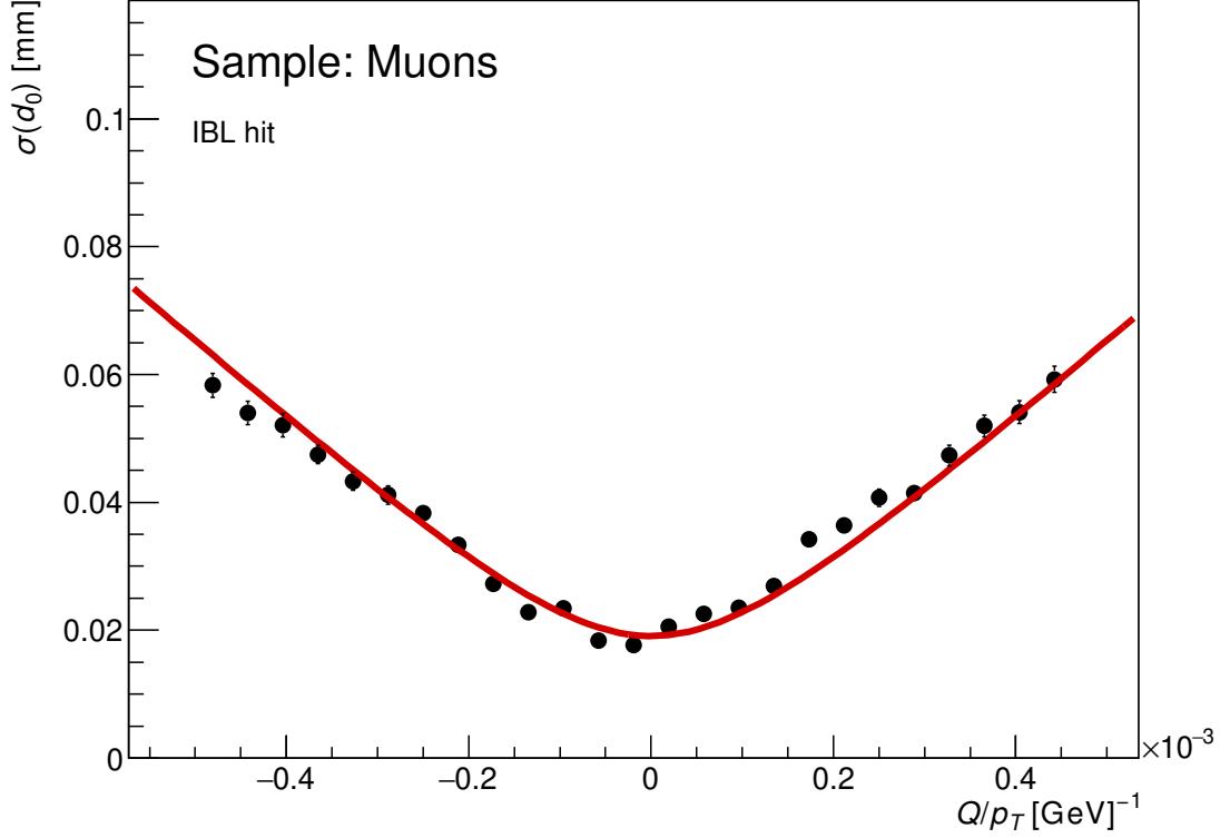
Figure 6.9: An example of a square root fit for the track parameter d_0 with a track having an IBL hit and |\eta| < 0.5 . The individual black points correspond to resolution of the Gaussian distribution of all tracks which have an IBL hit in |\eta| < 0.5 as shown in Figure 6.8
