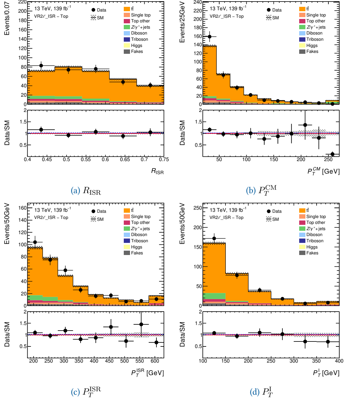
Figure 4.44: \text{VR}2\ell_{\text{ISR}}\text{-Top} : Modelling for R_{\text{ISR}} in (a). We show P_T^{\text{CM}} in (b). In (c) we show P_T^{\text{ISR}} . In (d) we show P_T^{\text{I}} .
