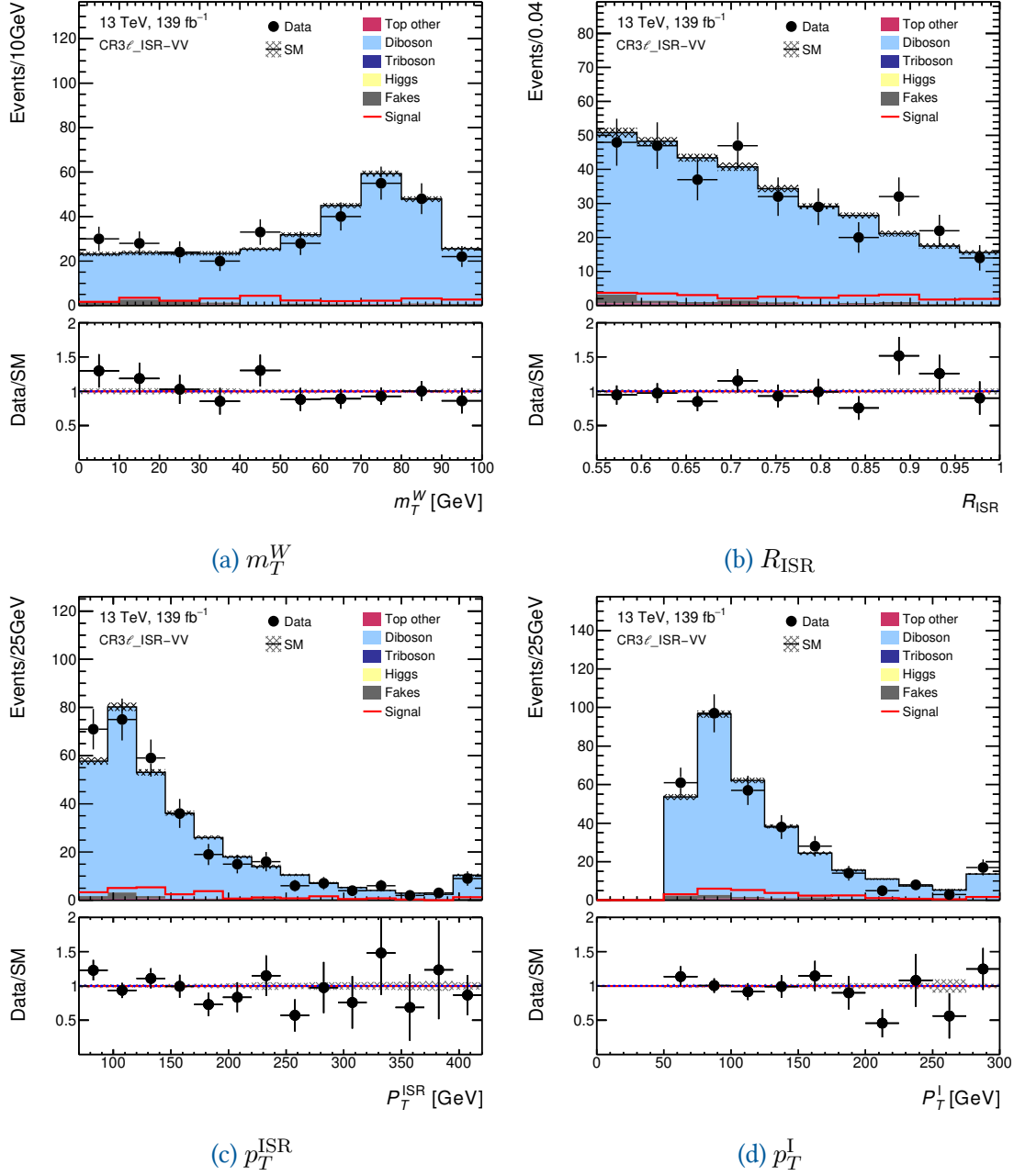
Figure 4.50: CR3 \ell _ISR-VV: Modelling for (a) m_T^W , (b) R_{\text{ISR}} , (c) p_T^{\text{ISR}} and (d) P_T^{\text{I}} .
