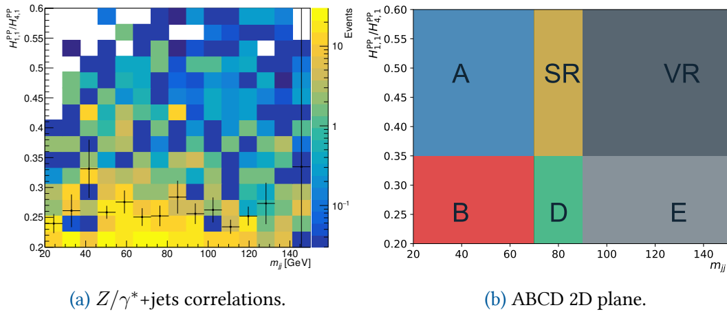
Figure 4.53: The ABCD regions for \text{SR}2\ell\_Low Z/\gamma^* +jets estimate. In (a), the black dots are a profile of each vertical slice. In (b), we have the regions labelled for the method.
