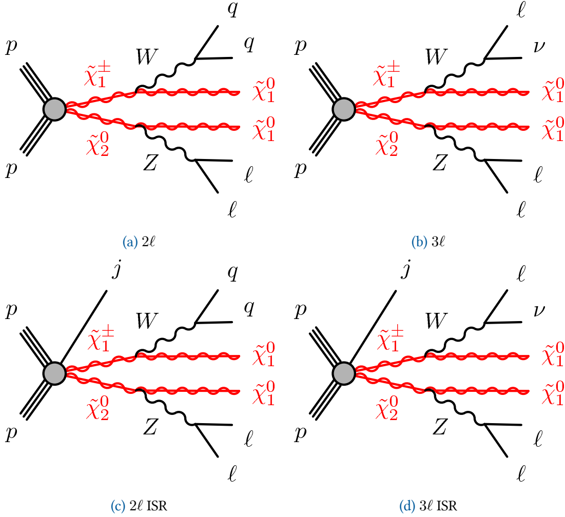
Figure 4.2: We sere signal models based on the W decaying either leptonically or hadronically, as well as the presence of initial state radiation. This naturally creates 2\ell and 3\ell signals, and ISR and non-ISR signals [65].
