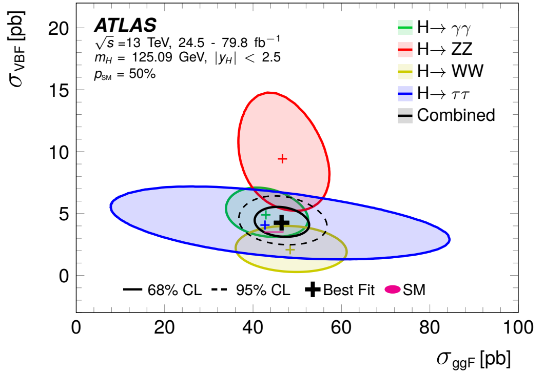
Figure 5.12: The summary of ggF and VBF Higgs production cross-sections as measured using different Higgs final states. For each measurement, the 68% CL is shown using a solid line, and the 95% CL, for the combined measurement is shown in a dotted line. The best fit for each measurement is shown with a cross. The combined measurement is shown in black, with the SM expectation being shown in magenta. The SM expectation is consistent with the combined 68% CL contour [134].
