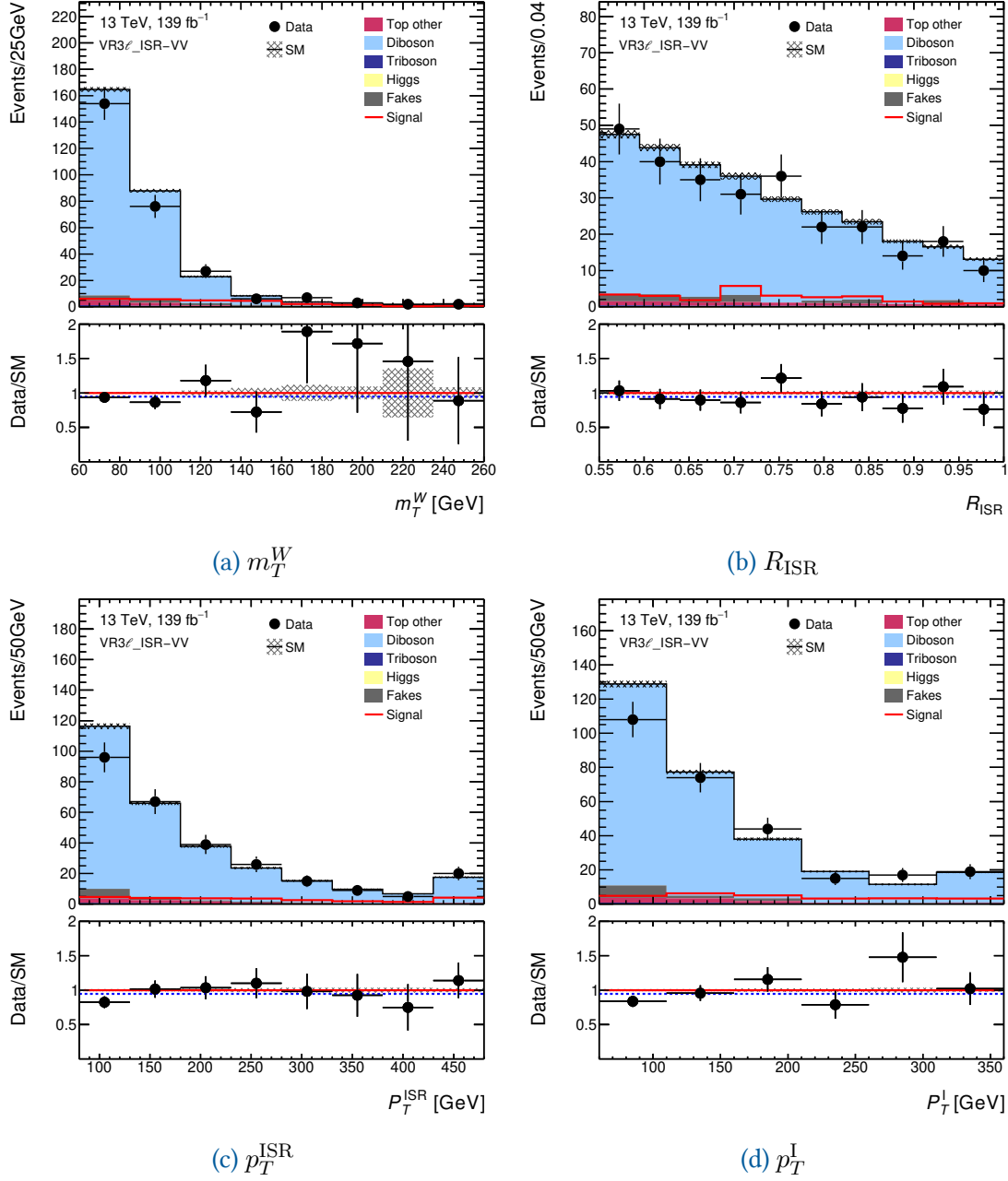
Figure 4.52: VR3 \ell _ISR-VV: Modelling for (a) m_T^W , (b) R_{\text{ISR}} , (c) p_T^{\text{ISR}} and (d) P_T^I .
