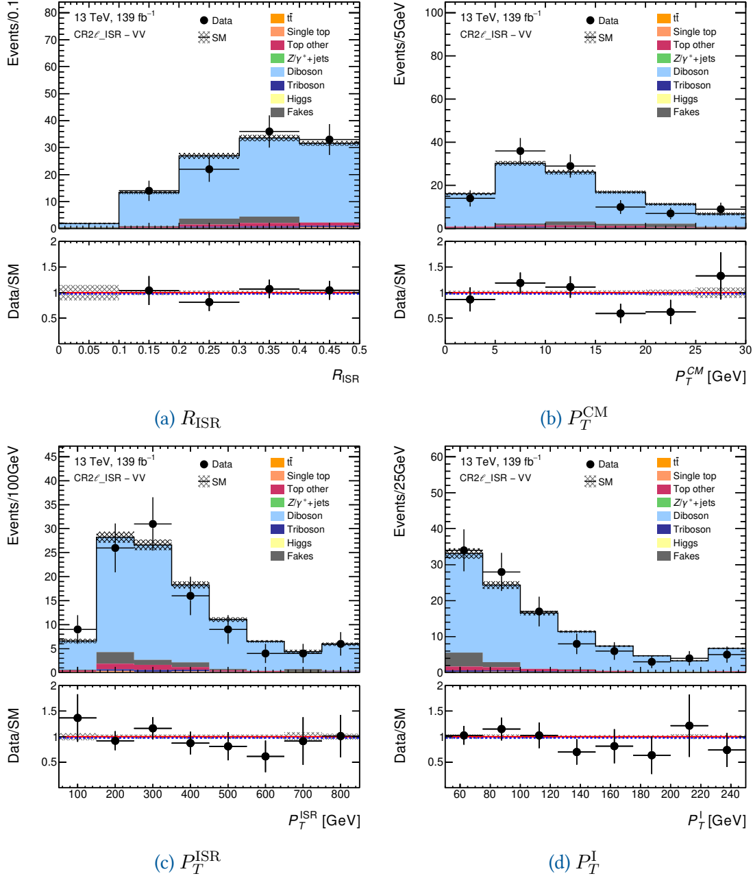
Figure 4.39: CR2 \ell_{\text{ISR}} -VV: Modelling for R_{\text{ISR}} in (a). We show P_T^{\text{CM}} in (b). In (c) we show P_T^{\text{ISR}} . In (d) we show P_T^{\text{I}} .
