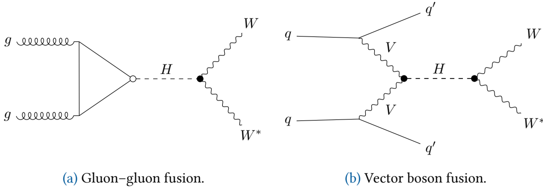
Figure 5.2: Diagrams for the leading production modes; (a) ggF and (b) VBF. Here we mark the VVH couplings with solid circle vertices and the qqH couplings with empty circles. The particle label “V” refers to a W/Z boson.
