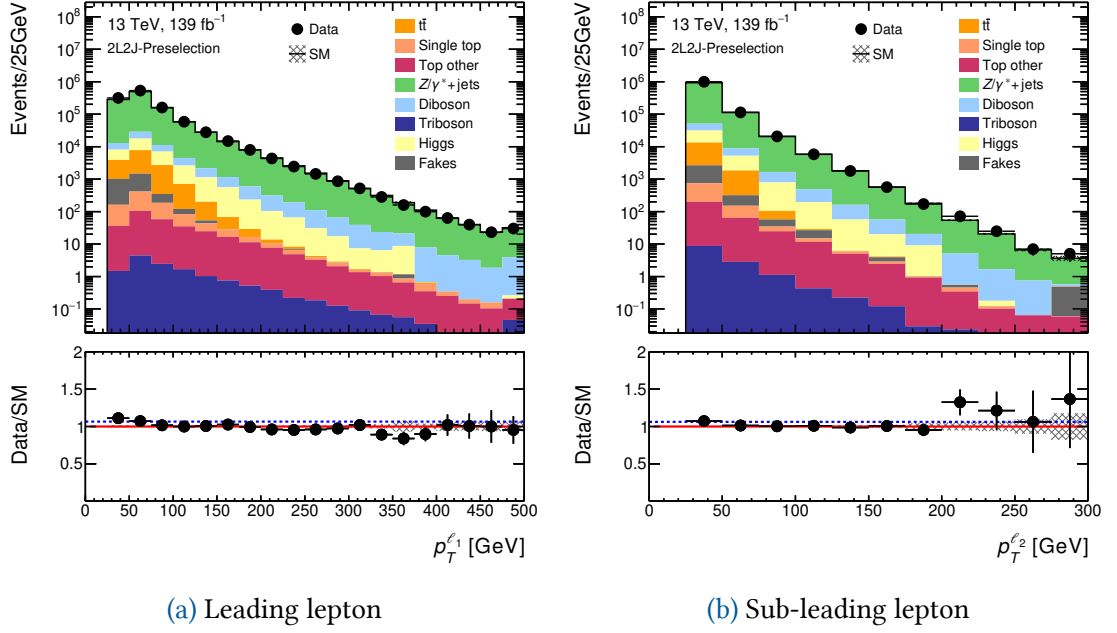
Figure 4.14: The lepton p_T modelling for preselection validation regions for RJ2 \ell A.
