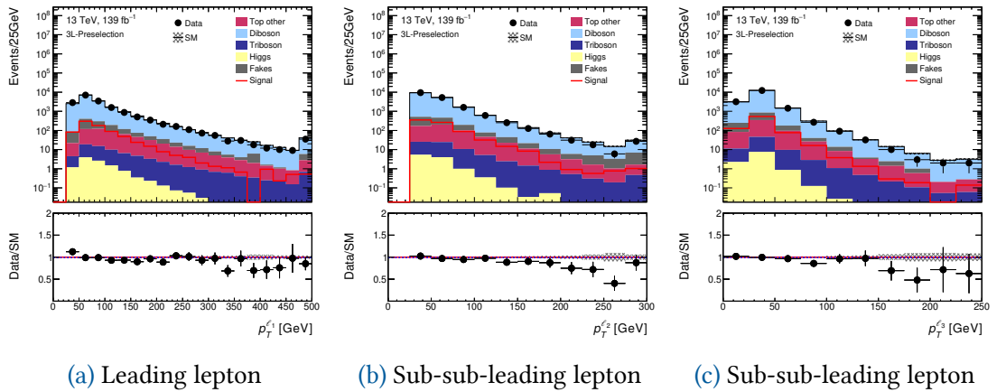
Figure 4.15: The lepton p_T modelling for preselection validation regions for RJ3 \ell A.
