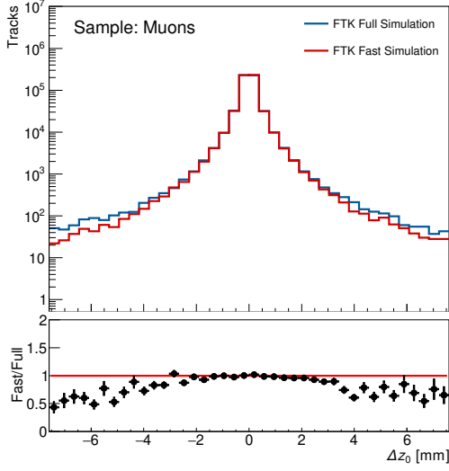
(a) Muon validation
