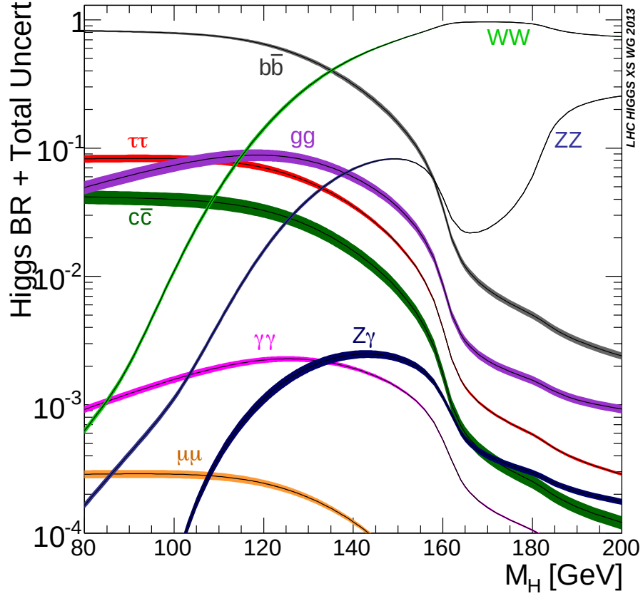
Figure 1.4: Branching ratios of SM Higgs boson vs m_H [11]
