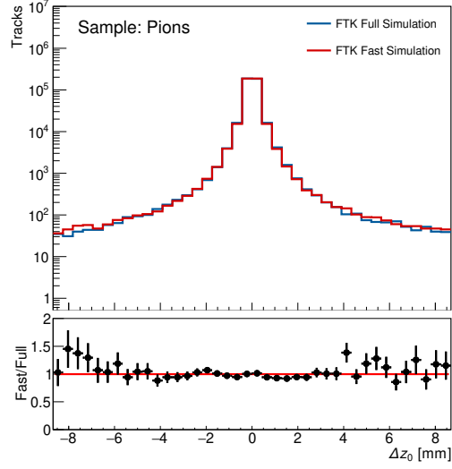
(b) Pion validation
