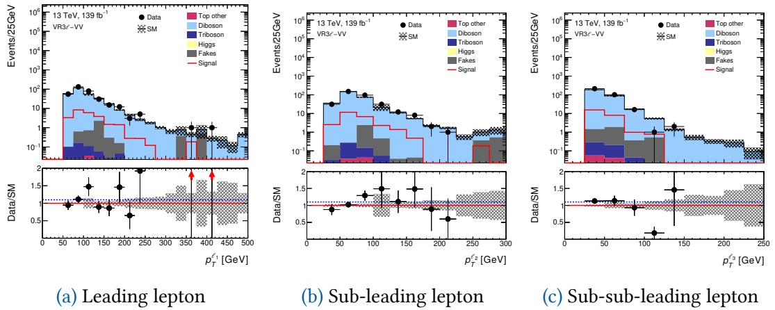
Figure 4.47: Validation of lepton momenta in VR3 \ell -VV. In (a) we show the leading lepton momentum. In (b) we show the sub-leading lepton momentum. In (c) we show the sub-sub-leading lepton momentum.
