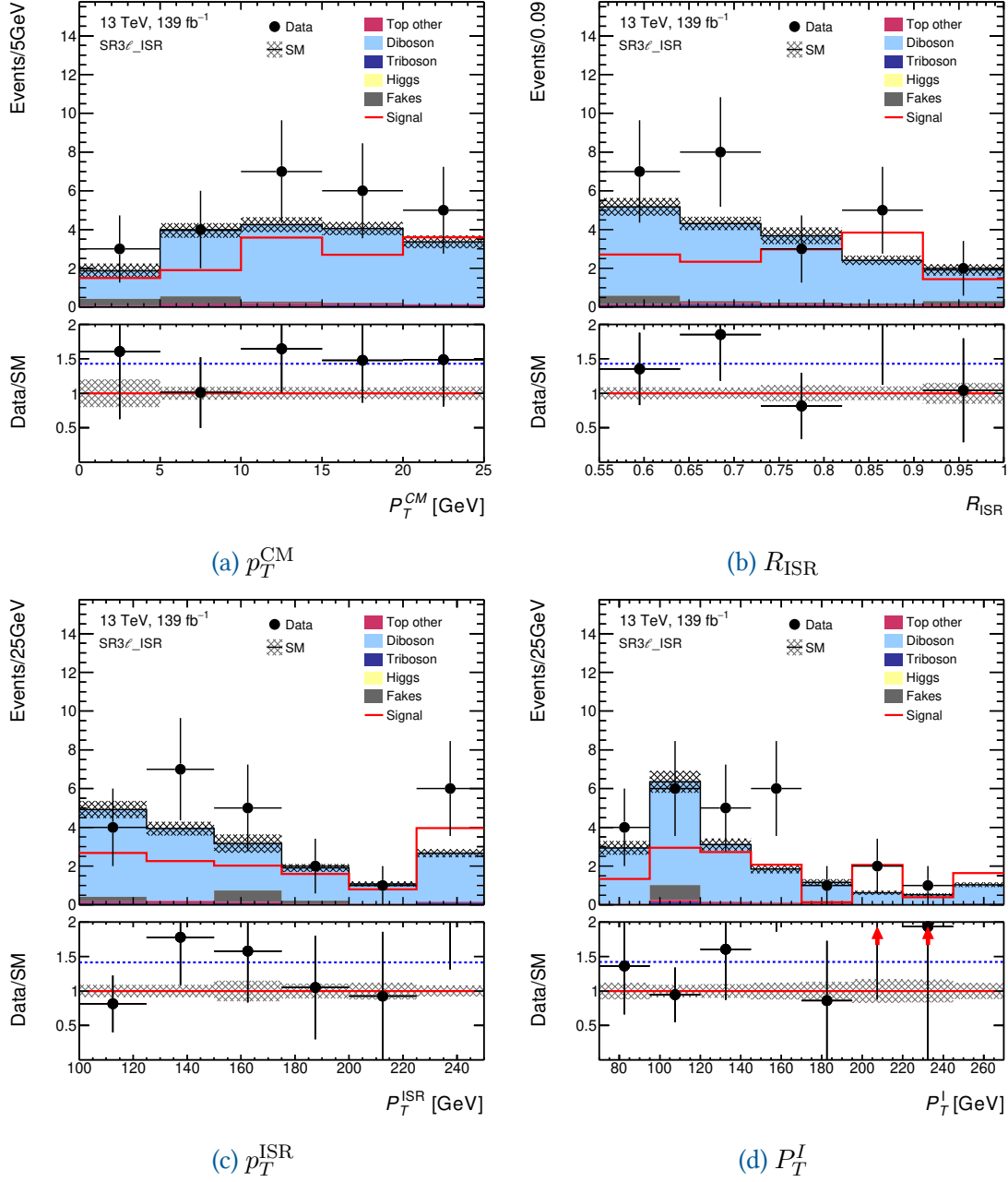
Figure 4.58: SR3 \ell _ISR: Modelling for (a) p_T^{\text{CM}} , (b) R_{\text{ISR}} , (c) p_T^{\text{ISR}} and (d) P_T^{\text{I}} .
