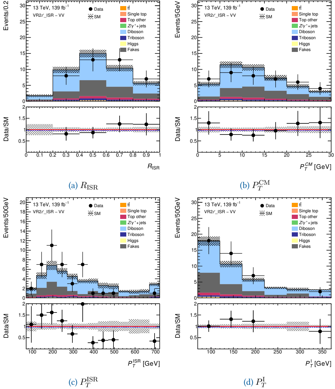
Figure 4.43: VR2 \ell_{\text{ISR}} -VV: Modelling for R_{\text{ISR}} in (a). We show P_T^{\text{CM}} in (b). In (c) we show P_T^{\text{ISR}} . In (d) we show P_T^{\text{I}} .
