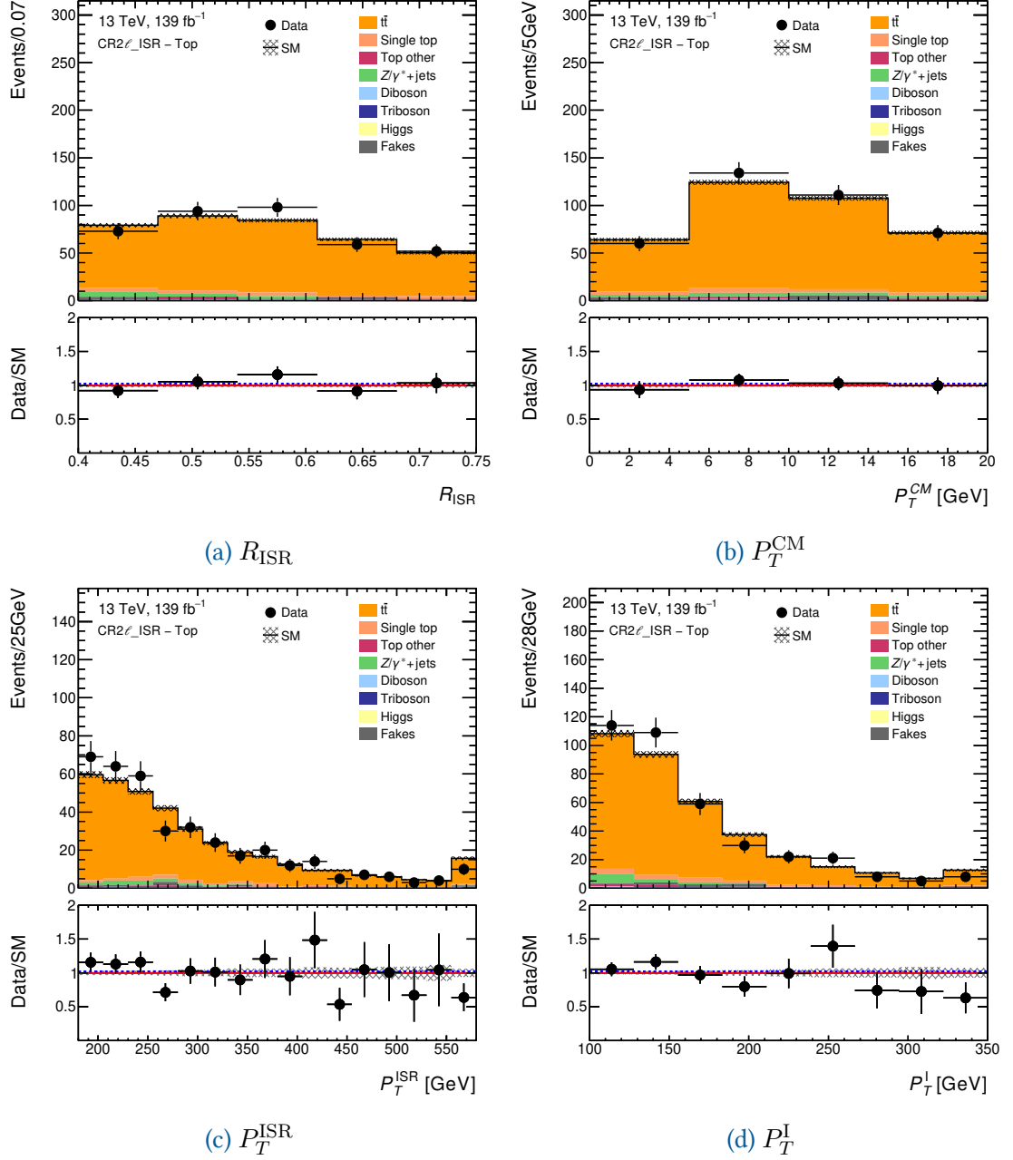
Figure 4.40: CR2ℓ_ISR-Top: Modelling for R_{\text{ISR}} in (a). We show P_T^{\text{CM}} in (b). In (c) we show P_T^{\text{ISR}} . In (d) we show P_T^{\text{I}} .
