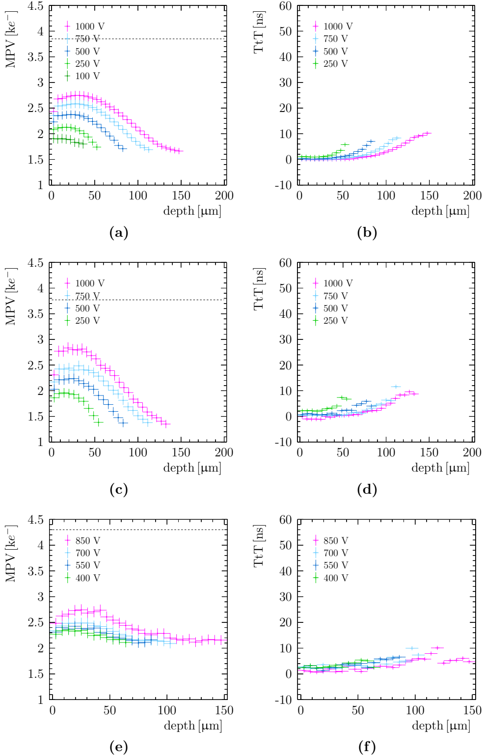
Figure 8.7: Charge collected (left) and time-to-threshold (right) as a function of depth for a 200 \mu m thick HPK n-on-p sensor (a)(b), a 200 \mu m thick Micron n-on-p sensor (c)(d) and a 150 \mu m thick Micron n-on-n sensor (e)(f). The 0 \mu m depth corresponds to the pixel electrodes side and 200 (top and middle) or 150 (bottom) \mu m to the backplane. The dashed line indicates the charge collected by a nonirradiated sensor of the same type. The sensors are uniformly irradiated to 8 \times 10^{15} \cdot 1 \text{ MeV } n_{eq} \text{ cm}^{-2} .
