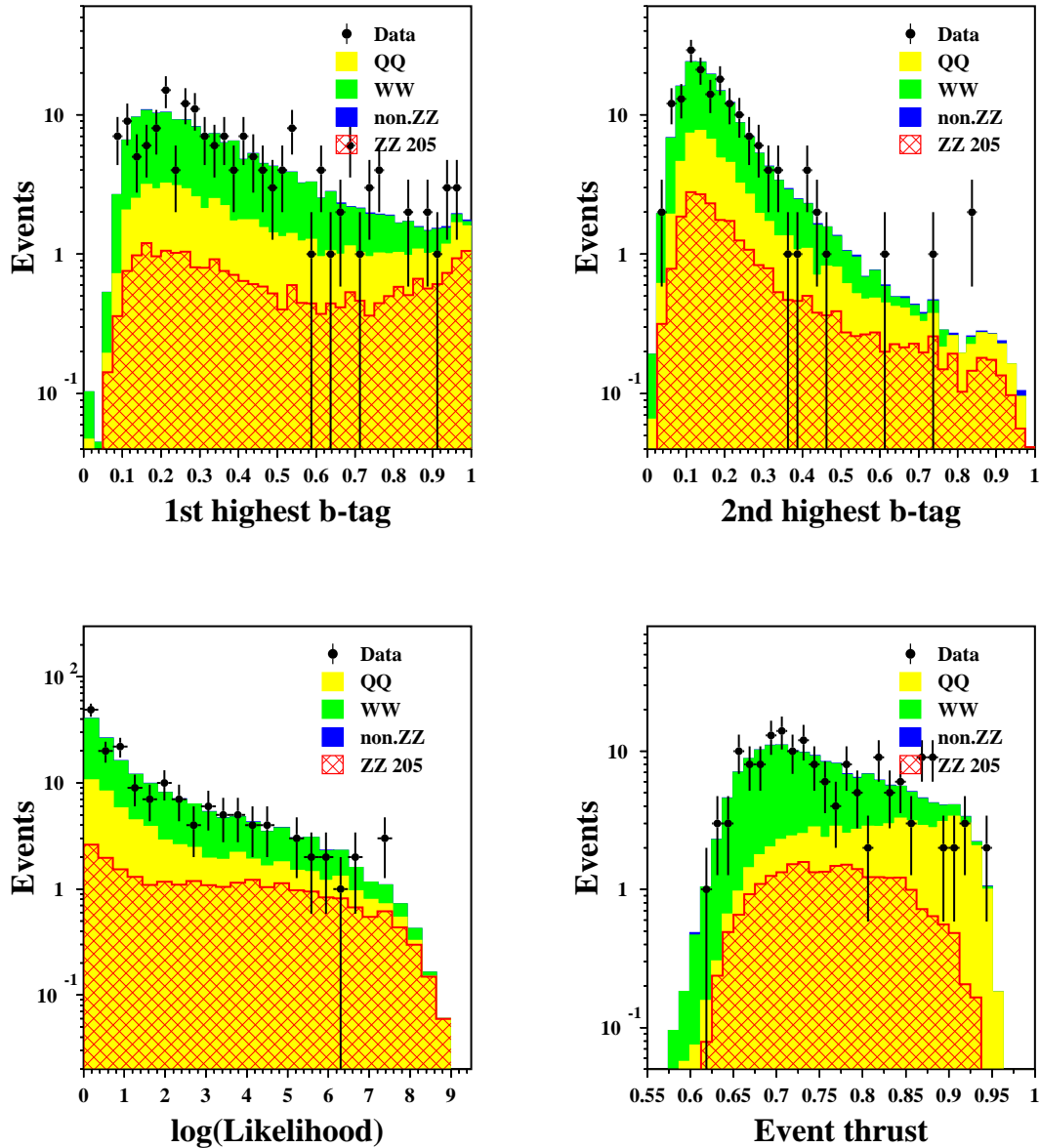
Figure 7.9: Distributions of variables used to construct the signal likelihood L_{ZZ} : 1st highest b-tag in the event (upper-left); 2nd highest b-tag in the event (upper-right); The logarithm of the selection likelihood after applying the cut, \log(L_{ZZ}) (lower-left); The event thrust (lower-right).
