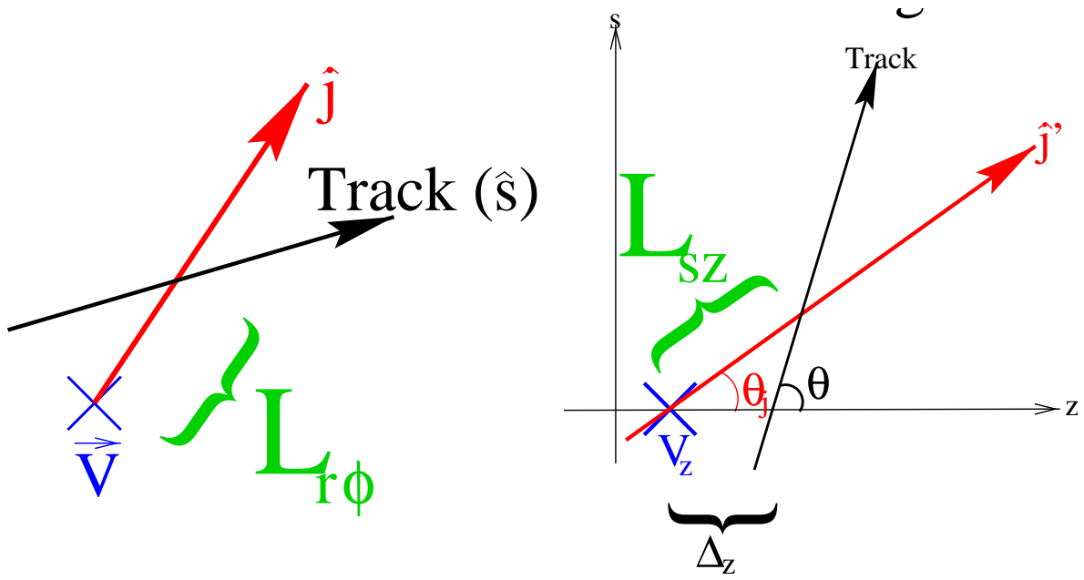
Figure 4.12: The definition of the tagging variable in the r - \phi plane, L_{r\phi} (left) and in s - z plane, L_{sz} , (right).
