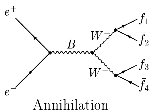
Figure 7.2: Topologies Feynman diagrams for the e^+e^- \rightarrow \bar{f}f\bar{f}'f' process. The curly lines represent any allowed gauge boson ( B = \gamma, Z^0, B_1, B_2, B_3 = Z^0, \gamma, W^\pm ).
