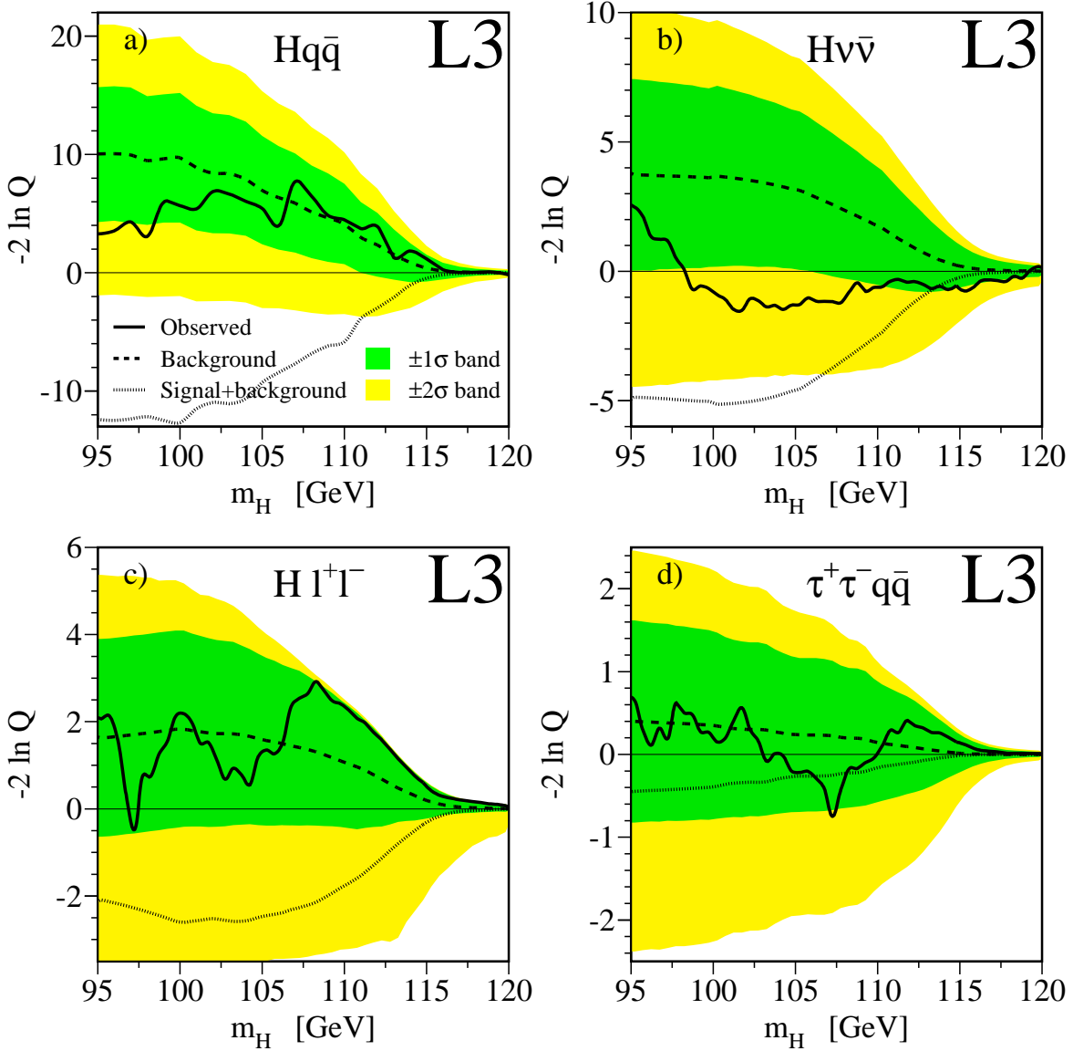
Figure 6.2: The log-likelihood ratio, -2\ln Q , as a function of the Higgs mass hypothesis, m_H , for the search channels a) Hq\bar{q} , b) H\nu\bar{\nu} [82], c) Hl^+l^- [82] and d) \tau^+\tau^-q\bar{q} [82]. The solid line shows the observed -2\ln Q . The dashed line shows the expected median value of -2\ln Q for the “background-only” hypothesis. The dark and the light shaded bands show the 68% and 95% probability intervals centered on the background expected median value. The dotted line is the median expected value for the “signal+background” hypothesis.
