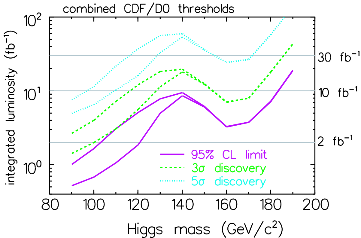
Figure 8.1: The sensitivity of the FNAL TEVATRON experiments to a light Higgs boson, as a function of its mass [134].
