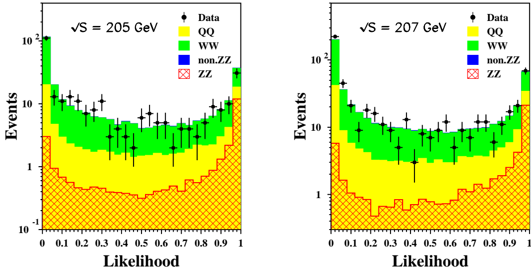
Figure 7.8: The Likelihood L_{ZZ} distribution for the signal and different background sources for the 205 GeV energy bin (left) and for 207 GeV energy bin (right).
