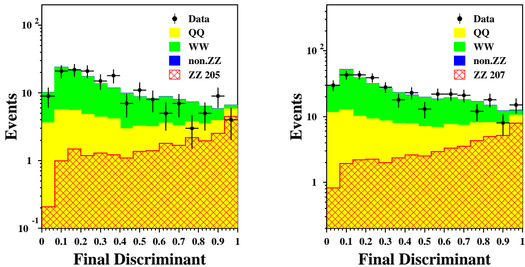
Figure 7.11: The final discriminant distribution for the data, signal and different background sources for the 205 GeV energy bin (left) and for 207 GeV energy bin (right) in the b -sensitive measurement including two highest jet b -tags.
