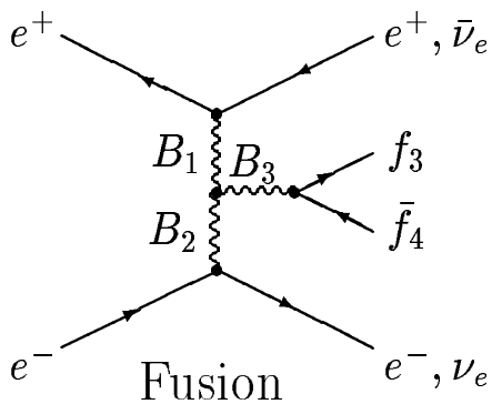
Figure 7.2: Topologies Feynman diagrams for the e^+e^- \rightarrow \bar{f}f\bar{f}'f' process. The curly lines represent any allowed gauge boson ( B = \gamma, Z^0, B_1, B_2, B_3 = Z^0, \gamma, W^\pm ).
