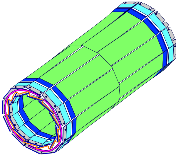
Figure 3.5: Perspective view of the Silicon Microvertex Detector. Overlap regions between the inner ladders are clearly seen.
