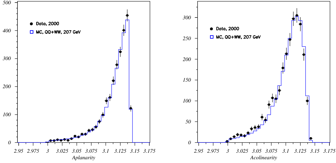
Figure 4.8: Aplanarity and acolinearity between two jets for data and Monte Carlo.
