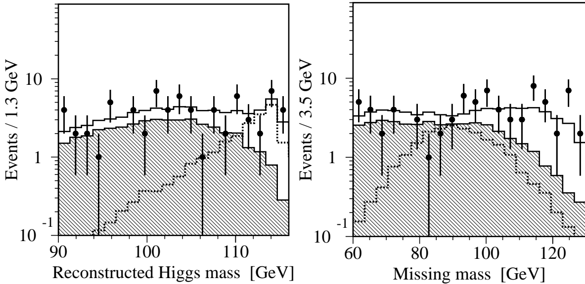
Figure 5.7: Distributions of the reconstructed Higgs mass after applying the 1C kinematic fit (left) and the missing mass, reconstructed from the measured quantities (right). The points represent the data collected as \sqrt{s} > 206 GeV. The open and hatched histograms are the expected backgrounds. The dashed line is the expected Higgs boson signal with m_H = 115 GeV, scaled by a factor of 30 [82].
