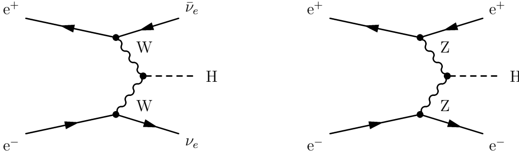
Figure 2.7: WW and ZZ fusion diagrams: They are suppressed by an additional power of the electroweak coupling with respect to the Higgs-strahlung process.
