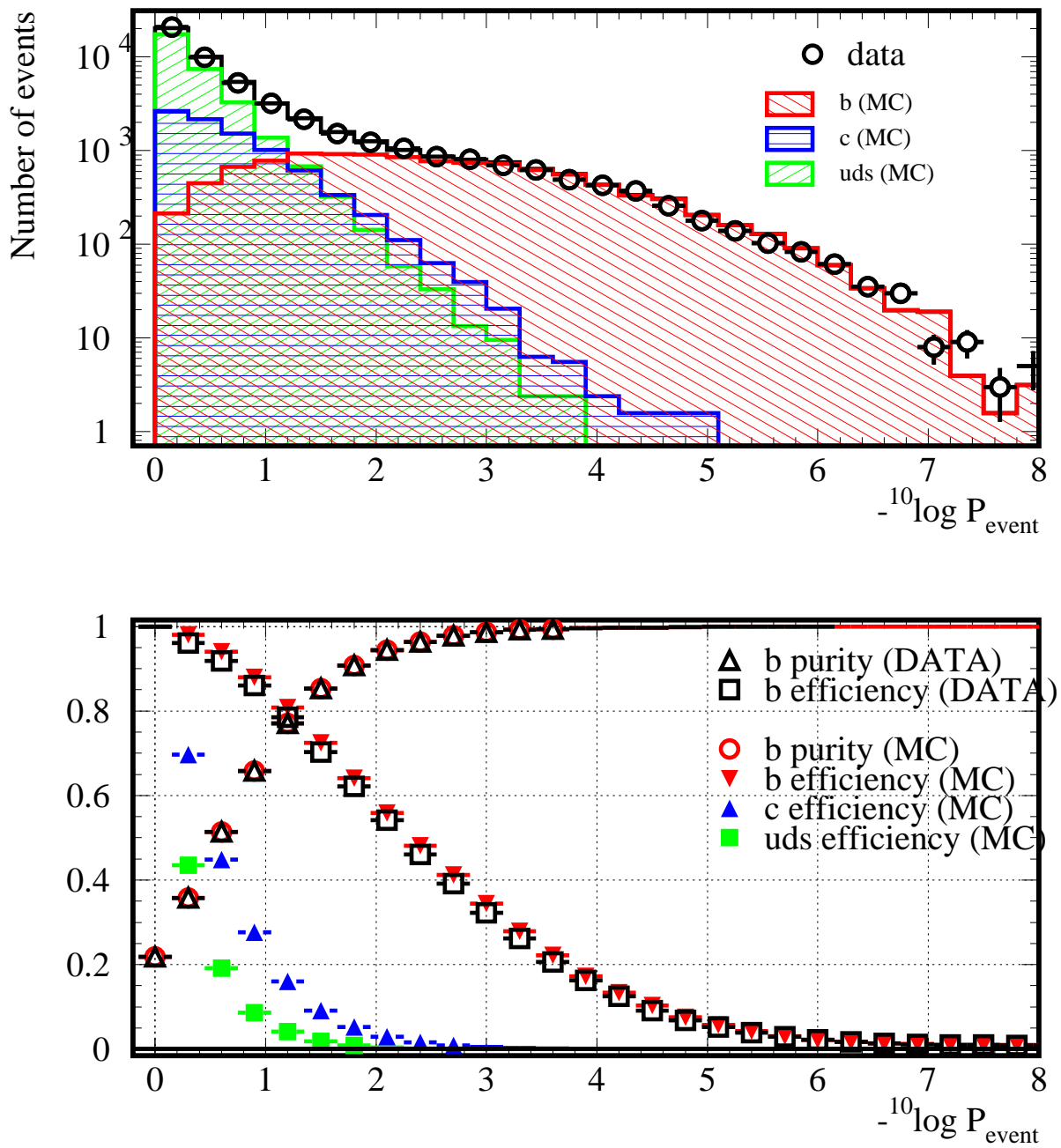
Figure 4.14: Event b-tagging discriminant distribution (upper plot) and tagging efficiency and purity as a function of cut on -\log(P_{\text{event}}) (lower plot) in 1999 Z-peak data and MC.
