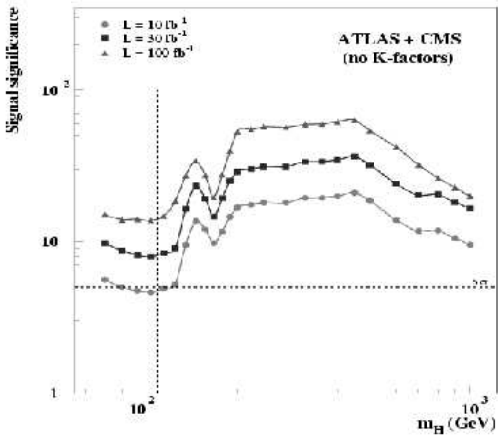
Figure 8.2: The sensitivity of the LHC experiments to a Higgs boson, as a function of its mass, for different accumulated luminosities [135].
