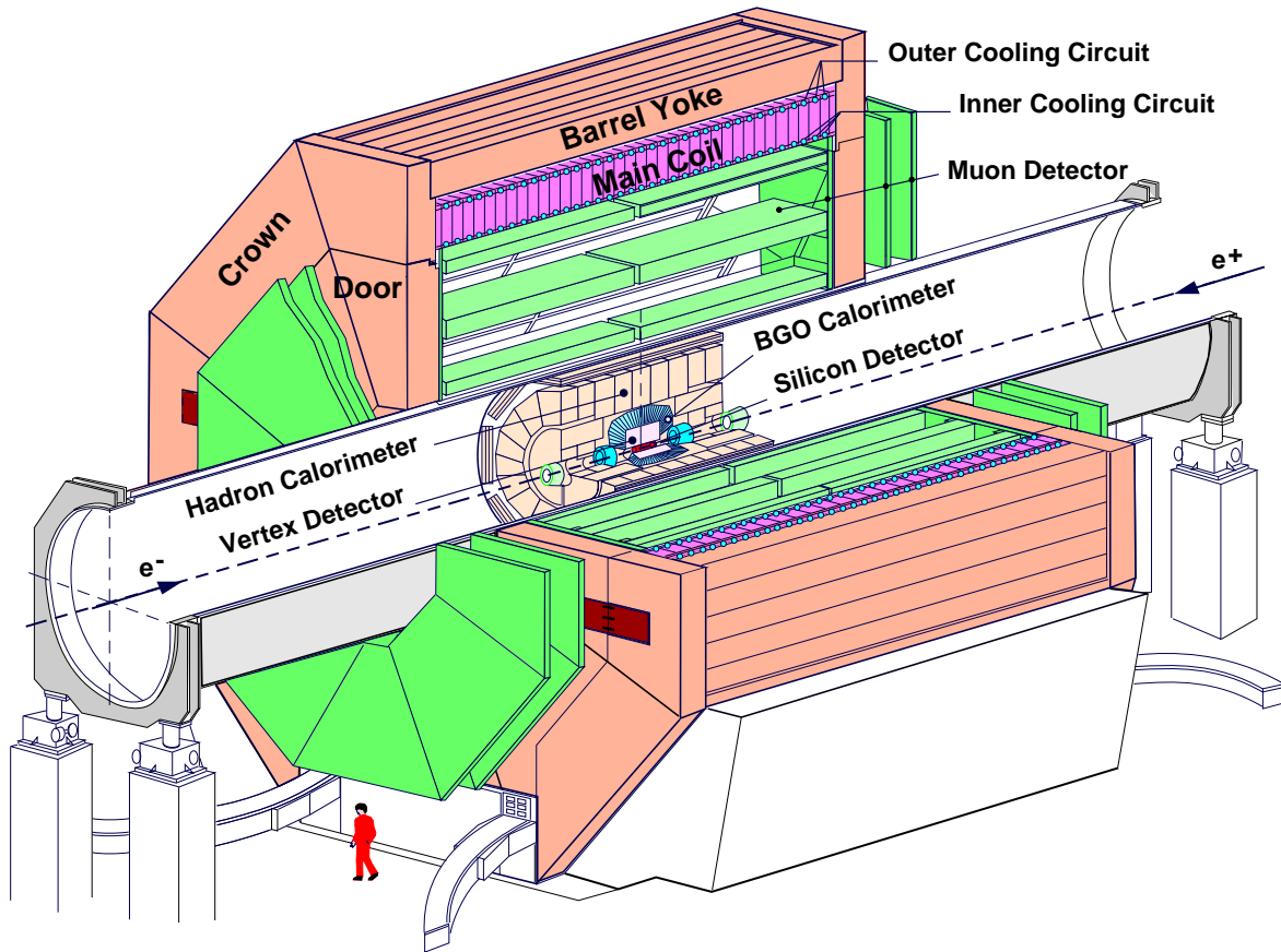
Figure 3.3: Perspective view of the L3 detector.
