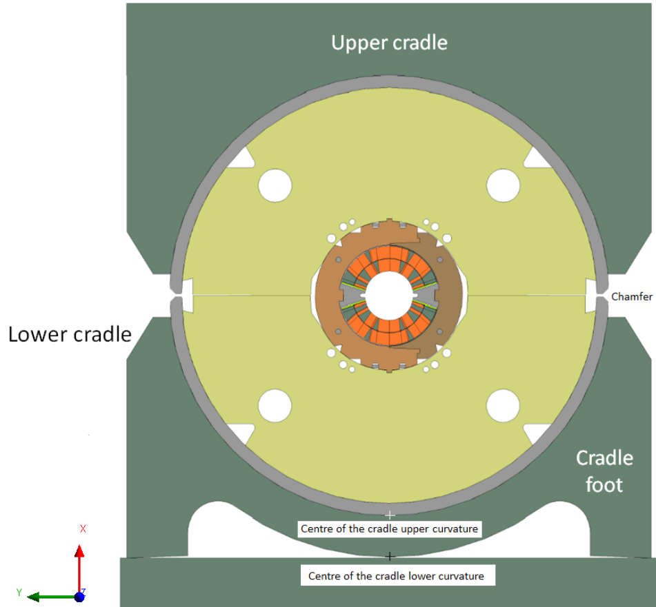
Figure 2.6: A Cradle assembly and single aperture 11-T dipole magnet (1-in-1) intersection. The magnet halves have been turned 90^\circ clockwise from Figure 2.2 for the welding position. [26]
