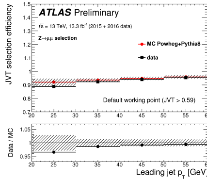
Figure 2.22: The hard-scatter jet selection efficiency measured in Z(\rightarrow \mu^+\mu^-)+\text{jets} events as a function of the leading jet p_T in data and MC simulation for JVT > 0.59. The uncertainties shown are the statistical uncertainty summed in quadrature with the systematic uncertainty. The bottom panels of each figure show the ratio of efficiencies measured in data and MC simulation [296].
