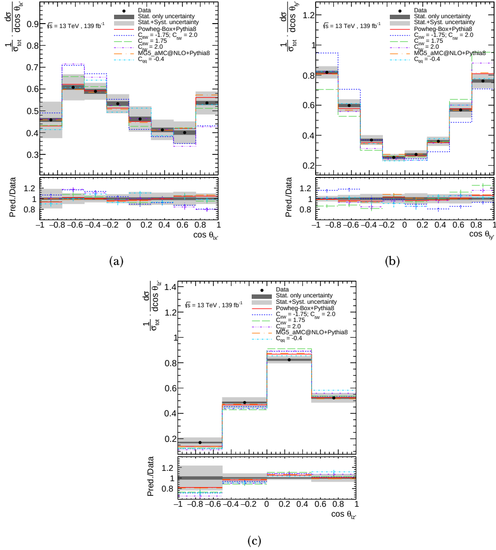
Figure 4.30: Normalised differential cross-sections as a function of (a) \cos \theta_{lx'} , (b) \cos \theta_{ly'} and (c) \cos \theta_{lz'} , for both top quarks and top antiquarks. The data, shown as the black points with statistical uncertainties, are compared to predictions using different MG5_AMC@NLO+PYTHIA8 samples, with different values for the real and the imaginary part of the dipole operator. A non-SM value for the four-fermion operator is also considered. The uncertainty bands include both the statistical and systematic uncertainties. The lower panels show the ratio of data to prediction in each bin.
