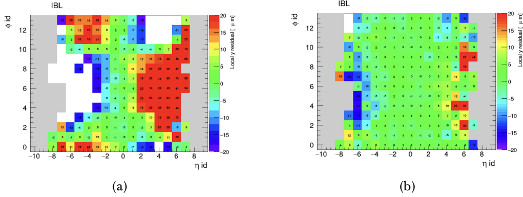
Figure 3.13: Residual maps in the y direction as a function of the \phi and \eta indexes for the IBL before (a) and after (b) a Level 3 alignment of this structure. The empty cells correspond to high \eta indexes which do not have enough statistics.
