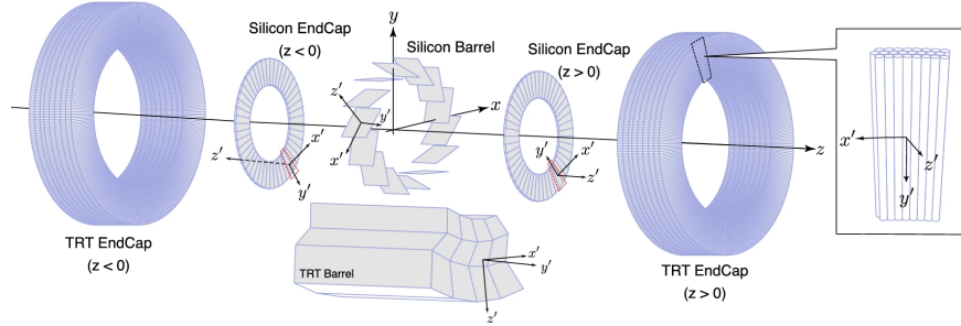
Figure 3.1: Schematic representation of the ATLAS global reference frame (x, y, z) . The local reference frame (x', y', z') of the different subdetectors is also displayed [1].
