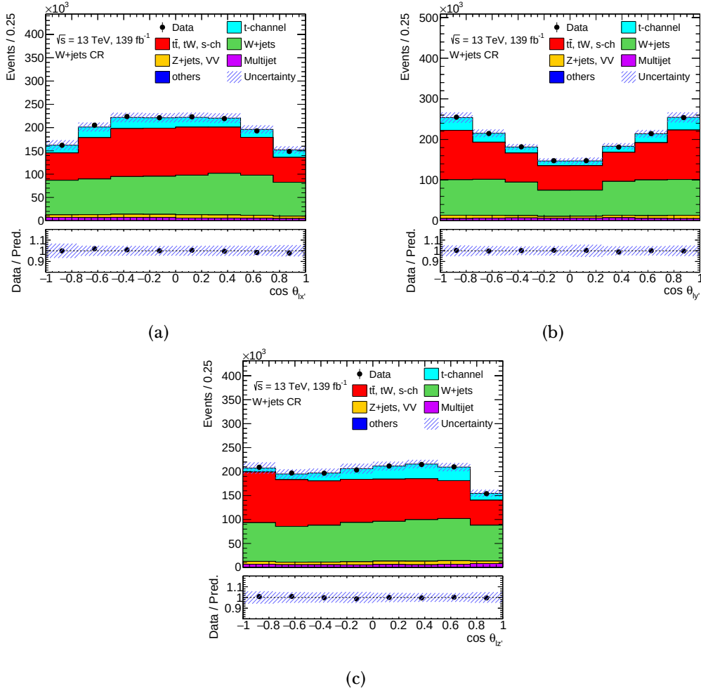
Figure 4.13: Post-fit distributions of (a) \cos \theta_{lx'} , (b) \cos \theta_{ly'} and (c) \cos \theta_{lz'} in the W +jets control region for the electron and muon channels merged, comparing observed data, shown as the black points with statistical uncertainties, to SM signal and background predictions. The multijet background is estimated using data-driven techniques, while contributions from simulated W +jets, top-quark backgrounds and t -channel event samples are normalised to the results of a maximum-likelihood fit to event yields in the signal and control regions. VV stands for the diboson background. The label "others" represents the t\bar{t}Z , t\bar{t}W , t\bar{t}H , tZq , tHq and tWZ productions. The uncertainty bands include both statistical and systematic uncertainties (described in Section 4.8.2). The lower panels show the ratio of data to prediction in each bin.
