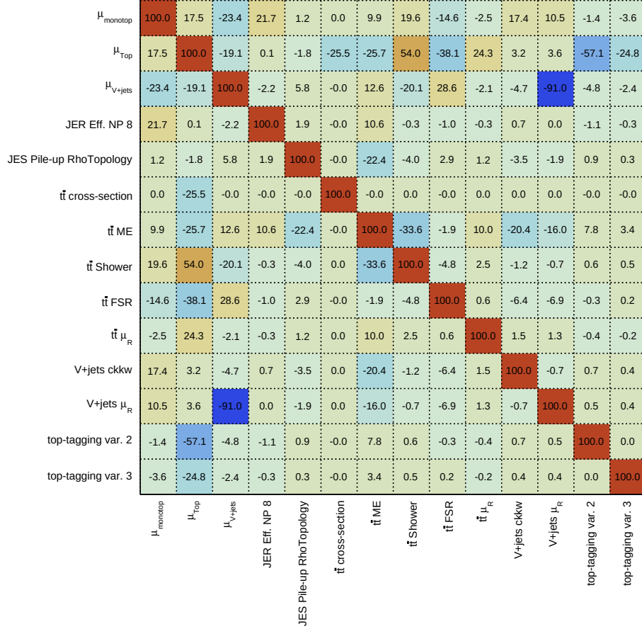
Figure 5.22: Correlation matrix of the free parameters and the NPs included in the data fit in the control regions and the DM resonant signal region under the signal-plus-background hypothesis. Only NPs with a correlation above 20% are displayed. The fit is performed using \lambda = 0.6 , y = 0.4 , m_\chi = 1 GeV and m_\phi = 4 TeV as parameters of the model.
