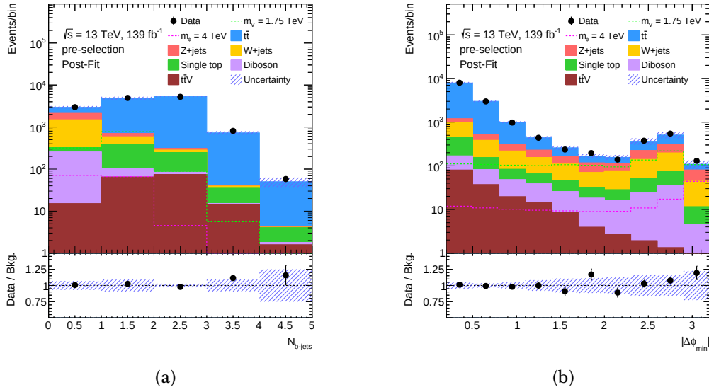
Figure 5.8: Comparison of data and SM predictions (post-fit) for (a) the N_{b\text{-jets}} and (b) the \Delta\phi_{\min} . The t\bar{t} and V -jets backgrounds are normalised to the results of a maximum-likelihood fit to data yields in the control regions. The expected distributions for the DM mono-top signal models are shown for the DM resonant model, assuming a mass of the mediation of m_\phi = 4 TeV and also for the DM non-resonant model, assuming a mass of the mediator of m_V = 1.75 TeV. In (a), the last bin of the distribution includes the overflow. The uncertainty bands correspond to the errors due to the limited size of the simulation samples. The lower panel shows the ratio of data to SM prediction.
