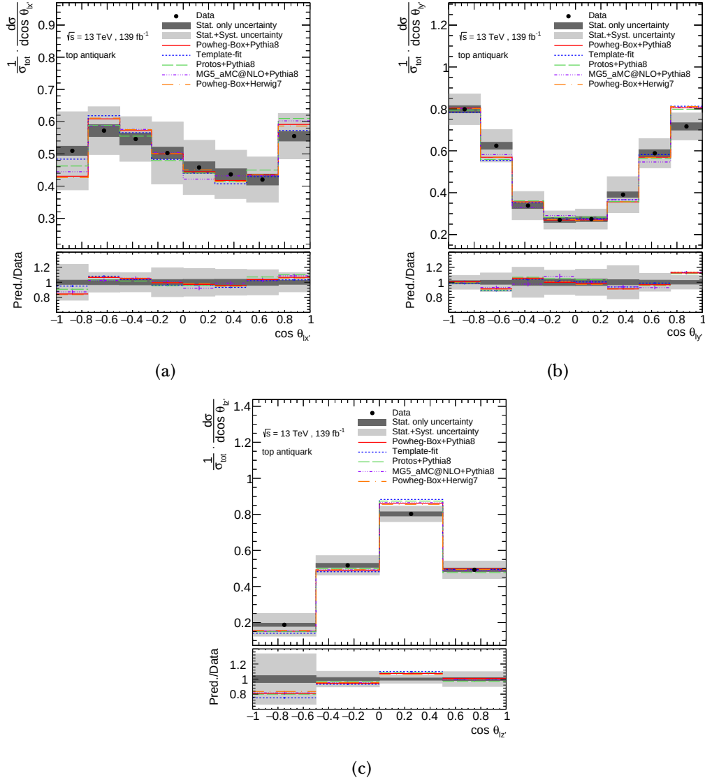
Figure 4.28: Normalised differential cross-sections as a function of (a) \cos \theta_{lx'} , (b) \cos \theta_{ly'} and (c) \cos \theta_{lz'} , along with various MC predictions of the t -channel signal for top antiquarks. The data, shown as the black points with statistical uncertainties, are compared to predictions using the POWHEG-BX+PYTHIA8, PROTOS+PYTHIA8, MG5_AMC@NLO+PYTHIA8, and POWHEG-BX+HERWIG7 setups. The results are also compared with the direct measurement of the top-antiquark polarisation vector, labelled template-fit. The uncertainty bands include both the statistical and systematic uncertainties. The lower panels show the ratio of data to prediction in each bin.
