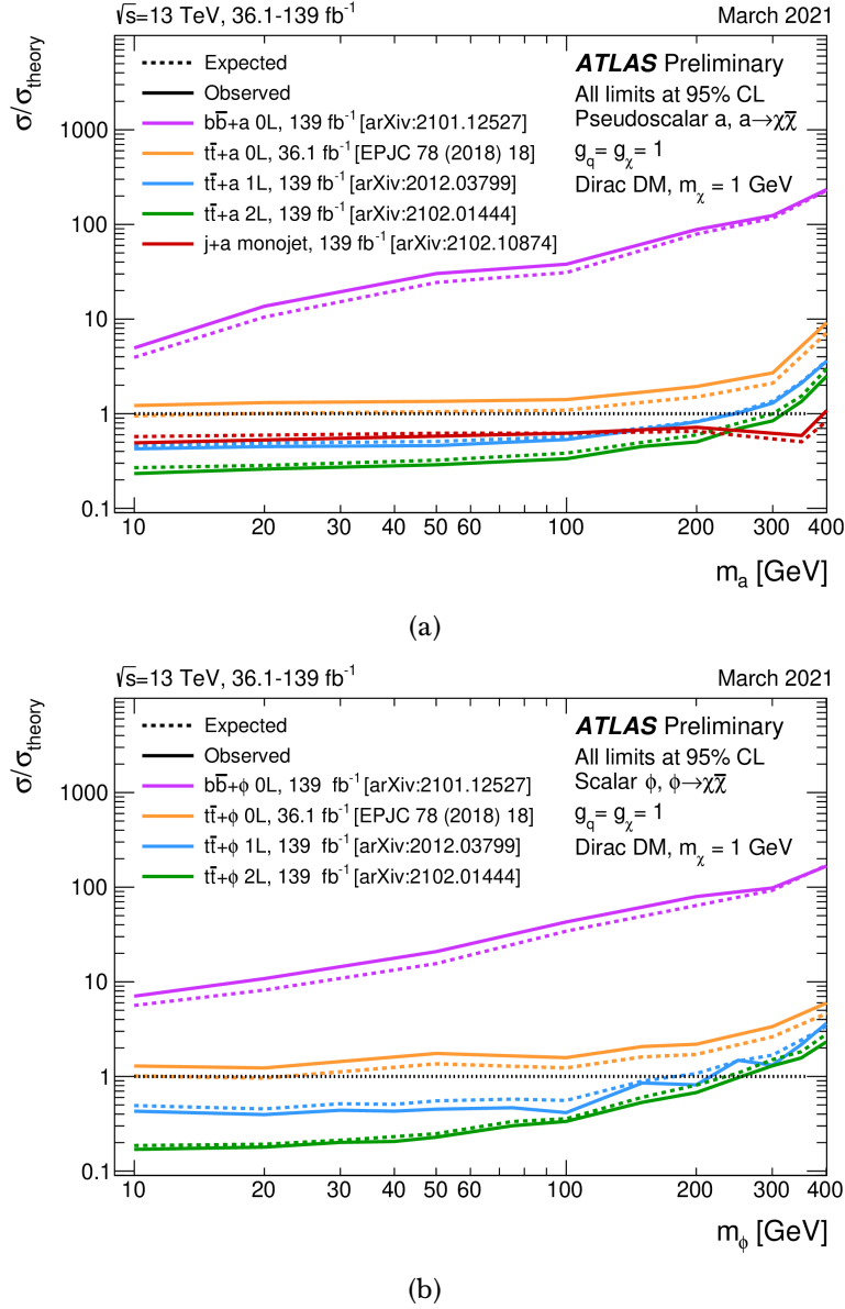
Figure 1.17: Exclusion limits for colour-neutral (a) pseudoscalar and (b) scalar mediator DM models from ATLAS as a function of the mediator mass (a) m_a and (b) m_\phi for a DM mass m_\chi of 1 GeV. The limits are calculated at 95% C.L. and are expressed in terms of the ratio of the excluded cross-section to the nominal cross-section for a coupling assumption of g = g_q = g_\chi = 1 . The solid (dashed) lines show the observed (expected) exclusion limits for different analyses [221].
