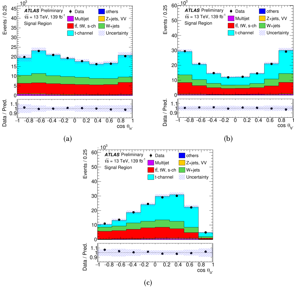
Figure 4.15: Post-fit distributions of (a) \cos \theta_{lx'} , (b) \cos \theta_{ly'} and (c) \cos \theta_{lz'} in the signal region for the electron and muon channels merged, comparing observed data, shown as the black points with statistical uncertainties, to SM signal and background predictions. The multijet background is estimated using data-driven techniques, while contributions from simulated W +jets, top-quark backgrounds and t -channel event samples are normalised to the results of a maximum-likelihood fit to event yields in the signal and control regions. VV stands for the diboson background. The label "others" represents the t\bar{t}Z , t\bar{t}W , t\bar{t}H , tZq , tHq and tWZ productions. The uncertainty bands include both statistical and systematic uncertainties (described in Section 4.8.2). The lower panels show the ratio of data to prediction in each bin.
