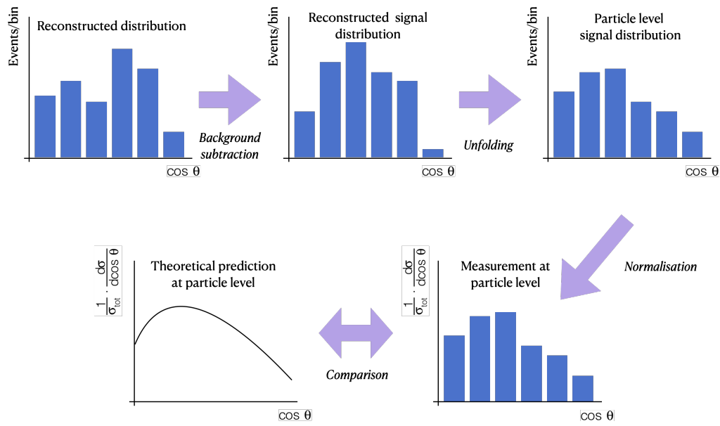
Figure 4.16: Schematic view summarising the different steps to provide the normalised differential cross-section measurements: The estimated background is subtracted from the measured distribution at reconstruction level. The unfolding to particle level technique is applied to the background-subtracted data to obtain the unfolded distributions. These distributions are provided as normalised differential cross-section measurements, which can finally be compared with theoretical predictions.
