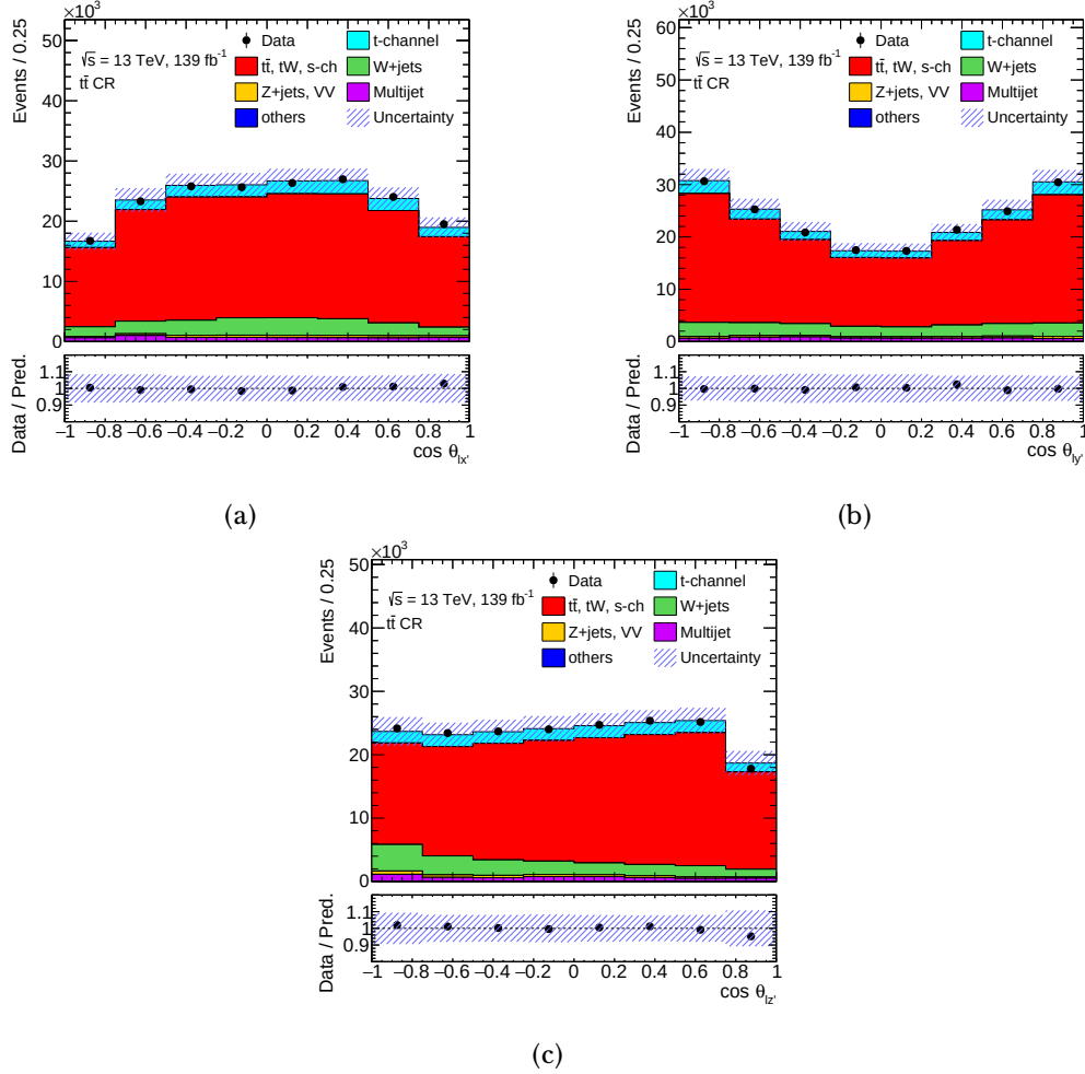
Figure 4.14: Post-fit distributions of (a) \cos \theta_{lx'} , (b) \cos \theta_{ly'} and (c) \cos \theta_{lz'} in the t\bar{t} control region for the electron and muon channels merged, comparing observed data, shown as the black points with statistical uncertainties, to SM signal and background predictions. The multijet background is estimated using data-driven techniques, while contributions from simulated W +jets, top-quark backgrounds and t -channel event samples are normalised to the results of a maximum-likelihood fit to event yields in the signal and control regions. VV stands for the diboson background. The label "others" represents the t\bar{t}Z , t\bar{t}W , t\bar{t}H , tZq , tHq and tWZ productions. The uncertainty bands include both statistical and systematic uncertainties (described in Section 4.8.2). The lower panels show the ratio of data to prediction in each bin.
