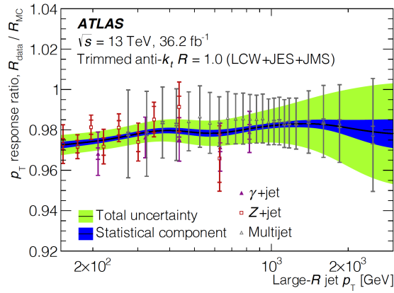
Figure 2.27: Data-to-simulation ratio of the average jet p_T response as a function of large- R jet p_T . The combined result (band) is based on three in situ techniques: the Z+jet balance method (open squares), \gamma +jet balance method (closed triangles), and the multijet balance (open triangles). The errors represent the statistical (inner error bars) and the total uncertainty (statistical and systematic uncertainties added in quadrature, outer error bars). The results apply to trimmed anti- k_t jets with R = 1.0 . The lines shown are smoothed using a sliding Gaussian kernel [306].
