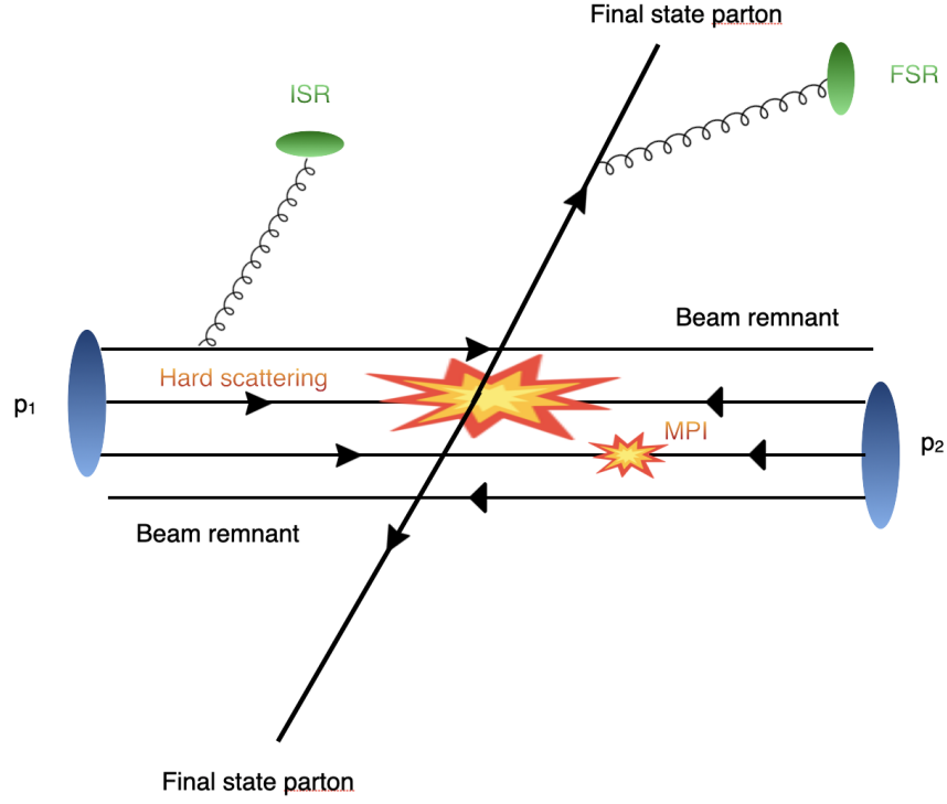
Figure 2.4: Schematic representation of a pp interaction with special emphasise on the underlying event. The collision includes the hard scattering interaction between two partons and the two final state partons resulting from this interaction. The underlying event includes an additional multiple particle interaction, the initial and the final state radiation and the beam remnants.
