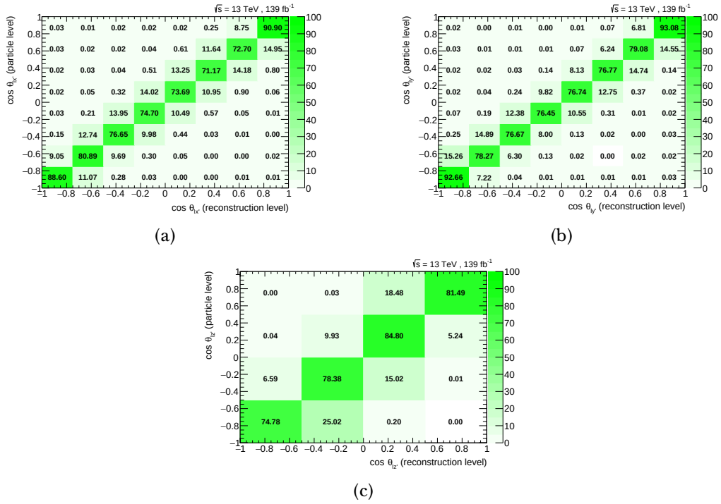
Figure 4.17: Migration matrices for (a) \cos \theta_{lx'} , (b) \cos \theta_{ly'} and (c) \cos \theta_{lz'} . The angular variable at particle level is shown on the y' -axis while the reconstructed angular variable is shown on the x' -axis. The numbers are normalised per row and given in percentage. They have been computed from the baseline POWHEG-BOX+PYTHIA8 FS sample.
