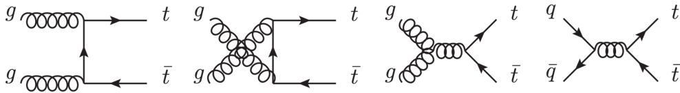
Figure 1.4: Feynman diagrams for t\bar{t} production at LO. The first three diagrams correspond to the gg initial state, whereas the last diagram corresponds to the q\bar{q} initial state.
