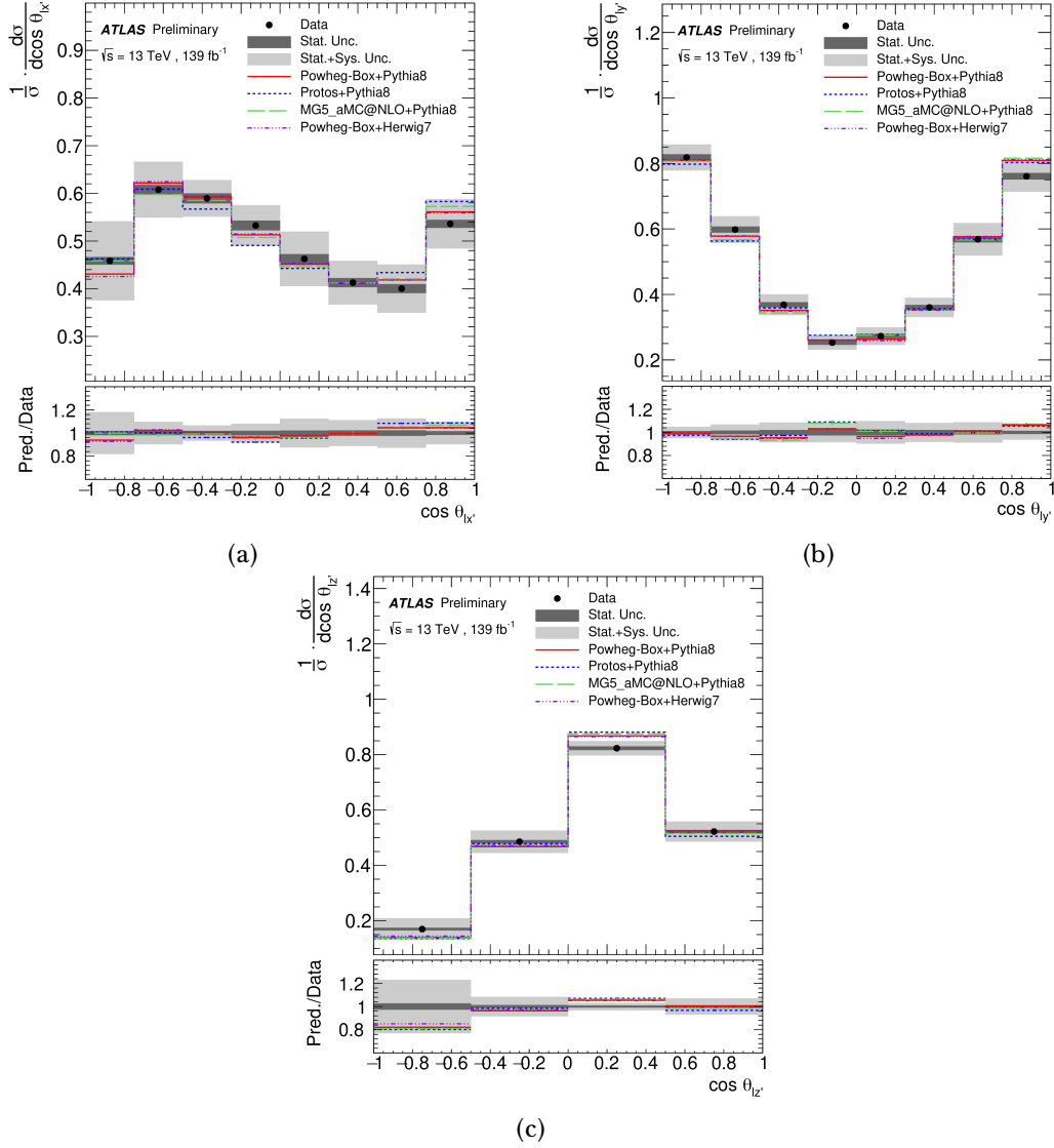
Figure 4.26: Normalised differential cross-sections as a function of (a) \cos\theta_{lx'} , (b) \cos\theta_{ly'} and (c) \cos\theta_{lz'} , along with various MC predictions of the t -channel signal for both top quarks and top antiquarks. The data, shown as the black points with statistical uncertainties, are compared to predictions using the POWHEG-BOX+PYTHIA8, PROTOS+PYTHIA8, MG5_AMC@NLO+PYTHIA8, and POWHEG-BOX+HERWIG7 setups. The uncertainty bands include both the statistical and systematic uncertainties. The lower panels show the ratio of data to prediction in each bin.
