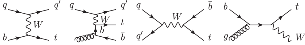
Figure 1.5: Feynman diagrams for single-top-quark production at LO. The first two correspond to the t -channel production, the next diagram corresponds to the s -channel and the last diagram corresponds to the production of a top quark in association with a W boson.
