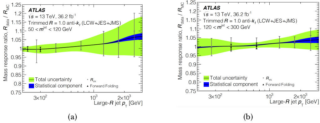
Figure 2.28: Data-to-simulation ratio of the average jet mass response as a function of the large- R jet p_T . Corrections using a combination of two in situ methods, the R_{trk} and forward-folding approaches, are applied. The fit is performed for large- R jet mass in the W mass range 50–120 GeV (a), and the top mass range 120–300 GeV (b). The error bars represent the statistical and systematic uncertainties added in quadrature. The results apply to anti- k_t jets with R = 1.0 calibrated with the LCW+JES+JMS scheme. The lines shown are smoothed using a sliding Gaussian kernel [306].
