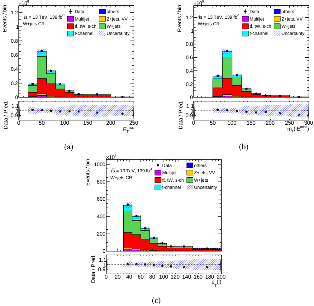
Figure 4.10: Post-fit distributions of (a) the E_T^{\text{miss}} , (b) the m_T(l, E_T^{\text{miss}}) and (c) the p_T(l) in the W +jets control region for the electron and muon channels merged, comparing observed data, shown as the black points with statistical uncertainties, to SM signal and background predictions. The multijet background is estimated using data-driven techniques, while contributions from simulated W +jets, top-quark backgrounds and t -channel event samples are normalised to the results of a maximum-likelihood fit to event yields in the signal and control regions. VV stands for the diboson background. The label "others" represents the t\bar{t}Z , t\bar{t}W , t\bar{t}H , tZq , tHq and tWZ productions. The uncertainty bands include both statistical and systematic uncertainties (described in Section 4.8.2). The lower panels show the ratio of data to prediction in each bin. The last bin of the distributions includes the overflow.
