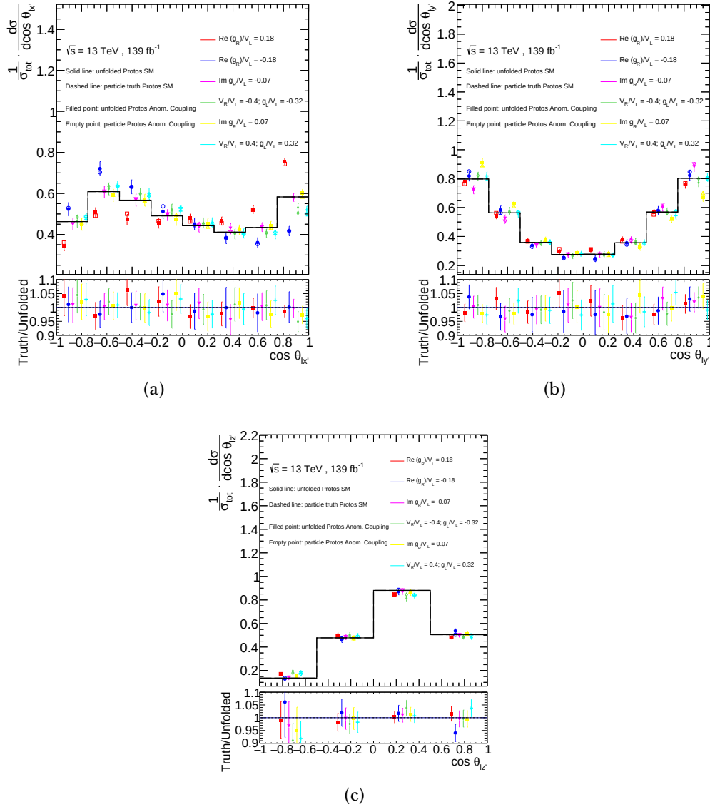
Figure 4.22: Normalised differential cross-sections as a function of (a) \cos\theta_{lx'} , (b) \cos\theta_{ly'} and (c) \cos\theta_{lz'} using different new physics samples. The dashed line represents the truth SM values while the solid line represents the unfolded values. The empty dots represent the truth values from different beyond the SM effects in terms of anomalous couplings, while the filled dots represent the unfolded values of the beyond the SM sample using the migration matrix and corrections factors from the SM sample. The uncertainty bands include the statistical error of the unfolded histograms. The lower panels show the ratio between the truth and the unfolded distributions for the SM and the beyond the SM samples considered.
