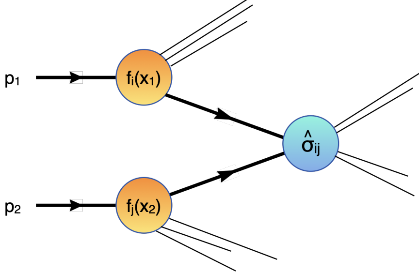
Figure 2.3: Schematic description of a hard process in hadronic collisions using the factorisation theorem.
