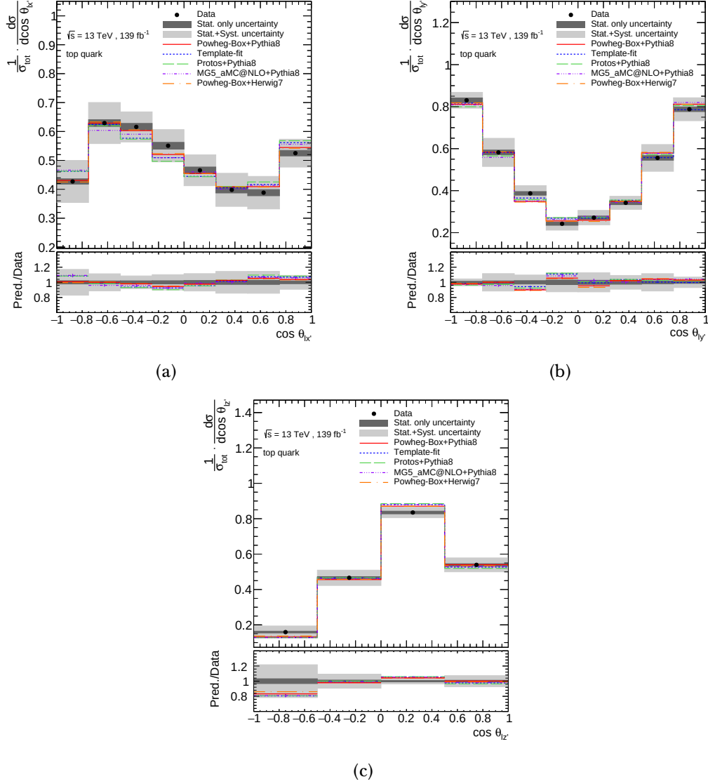
Figure 4.27: Normalised differential cross-sections as a function of (a) \cos\theta_{lx'} , (b) \cos\theta_{ly'} and (c) \cos\theta_{lz'} , along with various MC predictions of the t -channel signal for top quarks. The data, shown as the black points with statistical uncertainties, are compared to predictions using the POWHEG-BOX+PYTHIA8, PROTOS+PYTHIA8, MG5_AMC@NLO+PYTHIA8, and POWHEG-BOX+HERWIG7 setups. The results are also compared with the direct measurement of the top-quark polarisation vector, labelled template-fit. The uncertainty bands include both the statistical and systematic uncertainties. The lower panels show the ratio of data to prediction in each bin.
