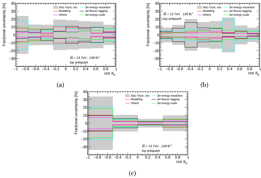
Figure 4.25: Breakdown of the different systematic contributions for the three angular distributions for top antiquarks: (a) \cos \theta_{l_{x'}} , (b) \cos \theta_{l_{y'}} and (c) \cos \theta_{l_{z'}} . The category 'Others' includes all the uncertainties which are not included in any other group.
