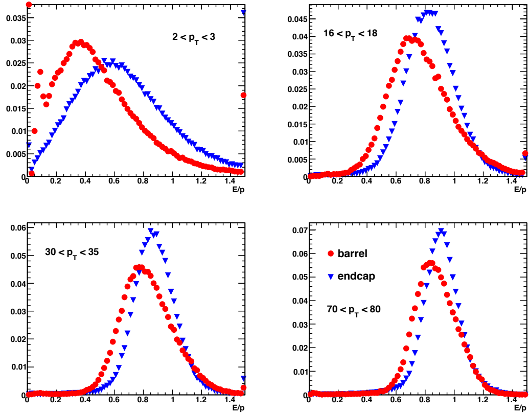
Figure 2.5: Calorimeter response for charged pions, separately in the barrel and endcap, for several different p_T intervals. The response is systematically better in the endcap than in the barrel and improves with increasing pion p_T .
