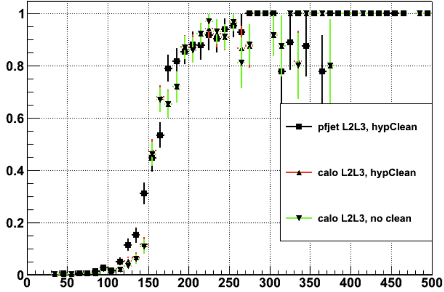
Figure 6.1: Turn-on curve for the H_T requirement of the DoubleMu3_HT150 and DoubleMu3_HT160 triggers measured using dimuon events near the Z mass. The distributions are shown as a function of H_T computed using L2L3-corrected particle-flow jets not overlapping with either of the muons (box), L2L3-corrected calorimeter jets not overlapping with either of the muons (up triangle) and L2L3-corrected calorimeter jets allowed to overlap with the two muons. In all cases, the jets are required to have p_T > 30 GeV and |\eta| < 2.5 .
