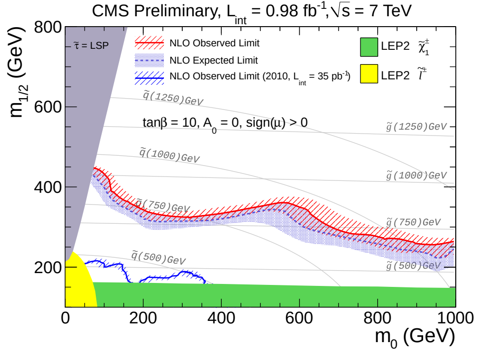
Figure 7.4: Exclusion region in the CMSSM corresponding to the observed upper limit of 3.0 events in the high- p_T signal region defined by H_T > 400 GeV and \cancel{E}_T > 120 GeV. The result of the previous analysis [32] is shown to illustrate the improvement since.
