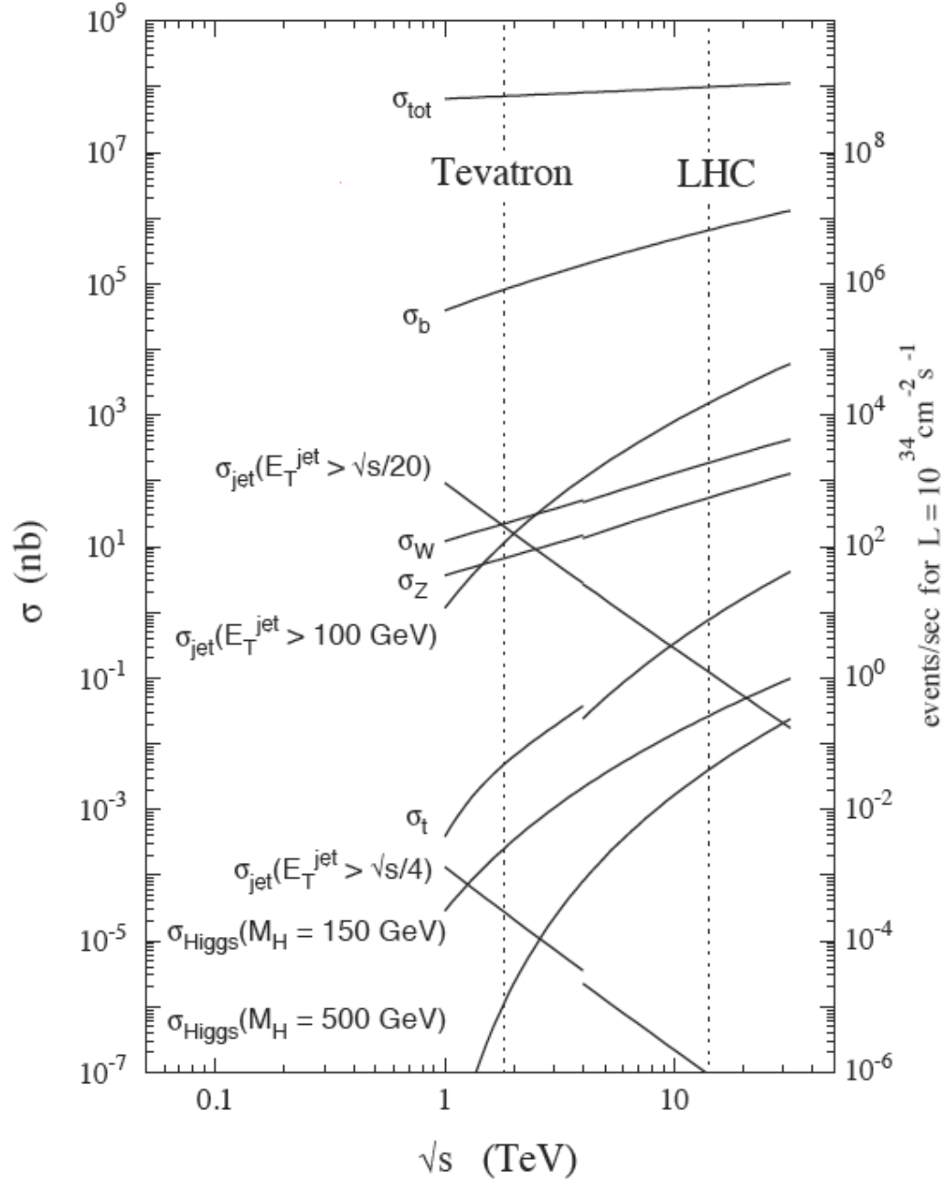
Figure 1.2: Cross sections for some Standard Model processes and for different potential Higgs masses. The production rate for new physics (i.e., Higgs production) is much smaller than that for SM electroweak and t\bar{t} production, the main backgrounds to new physics searches in dilepton final states. The cross sections of SM processes giving final state leptons are in turn many orders of magnitude smaller than QCD cross sections. From [4].
