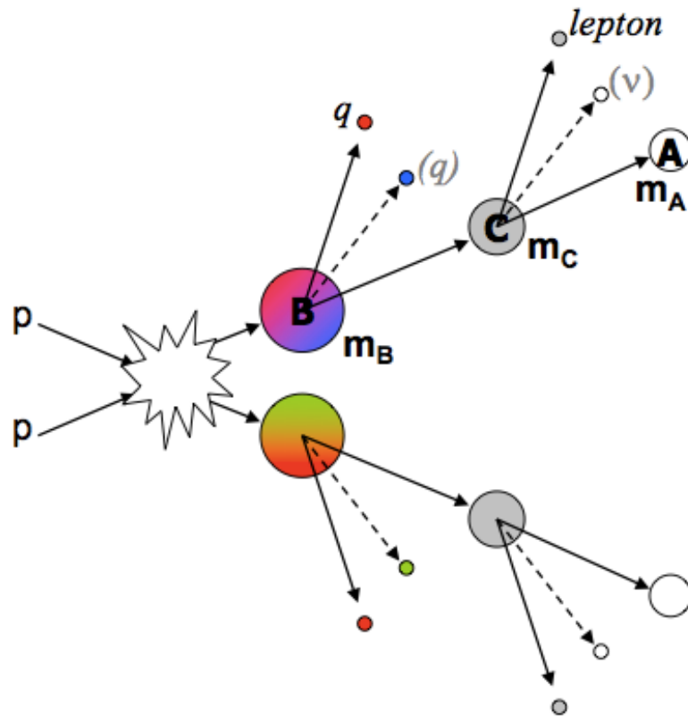
Figure 7.1: A depiction of a decay chain typically observed in SUSY models.
