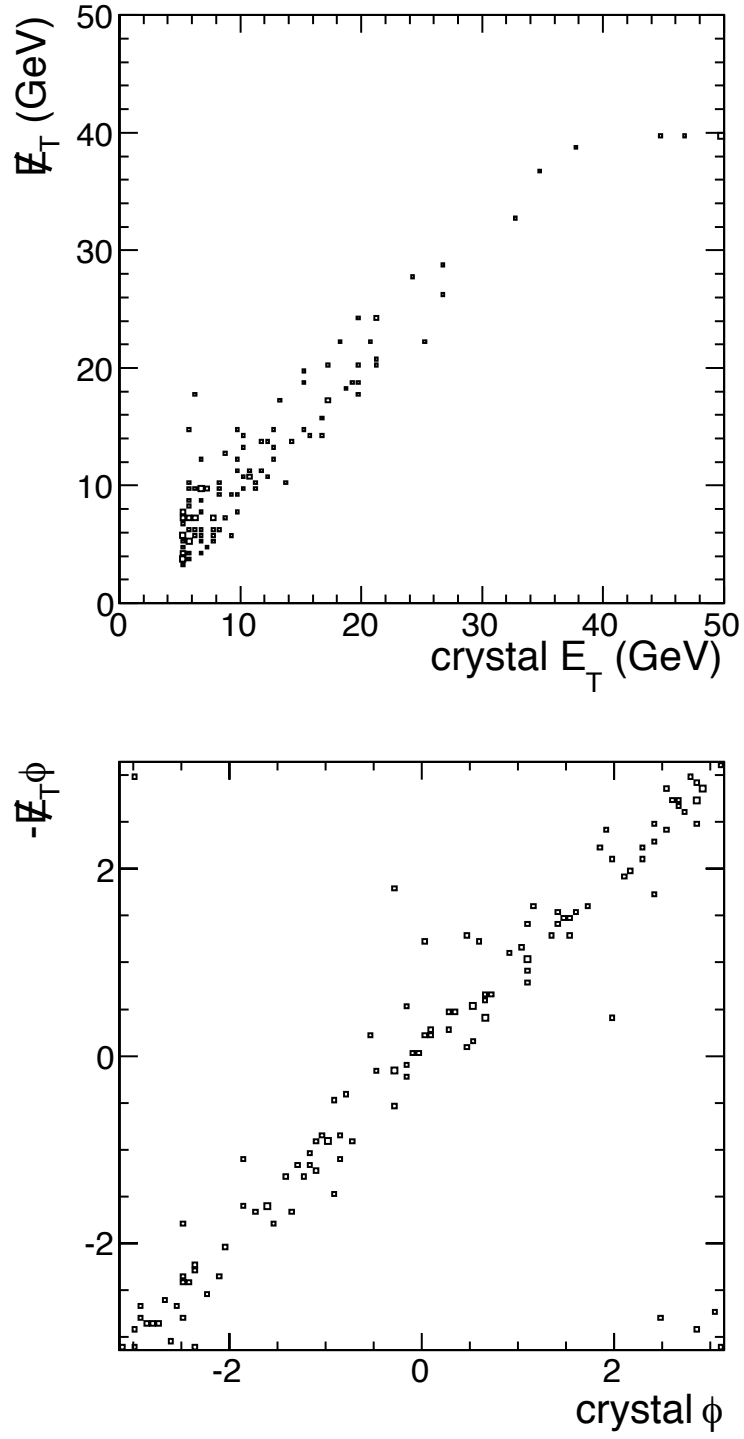
Figure 2.23: Correlation of the magnitude (top) and direction (bottom) between ECAL spikes and the \vec{E}_T .
