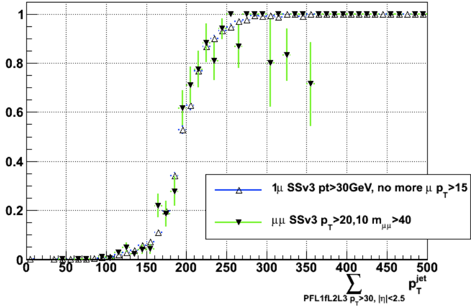
Figure 6.2: H_T trigger turn-on curves for the HT150/HT160 triggers as a function of the L1FastL2L3-corrected particle-flow jets. The jets are required to pass a selection of p_T > 30 GeV and |\eta| < 2.5 . The curve measured for the single-muon+ H_T trigger in event with only one muon (open triangles) represent the efficiency in W +jets events. The curve measured for the dimuon H_T trigger in events with two muons (filled triangles) represents the efficiency in Z +jets events.
