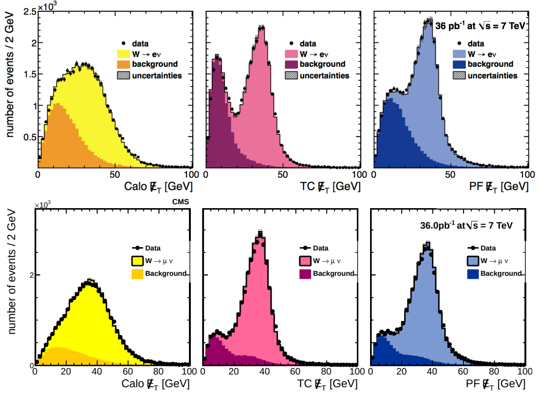
Figure 2.26: Comparison of \cancel{E}_T distributions for different algorithms in W \rightarrow e\nu (top) and W \rightarrow \mu\nu (bottom) candidate events. The distributions correspond to the corrected calo \cancel{E}_T , tc \cancel{E}_T and pf \cancel{E}_T algorithms (left to right). Good agreement is observed between data and simulation for all algorithms. Both tc \cancel{E}_T and pf \cancel{E}_T show significant improvement compared to the baseline calorimeter-based \cancel{E}_T [18].
