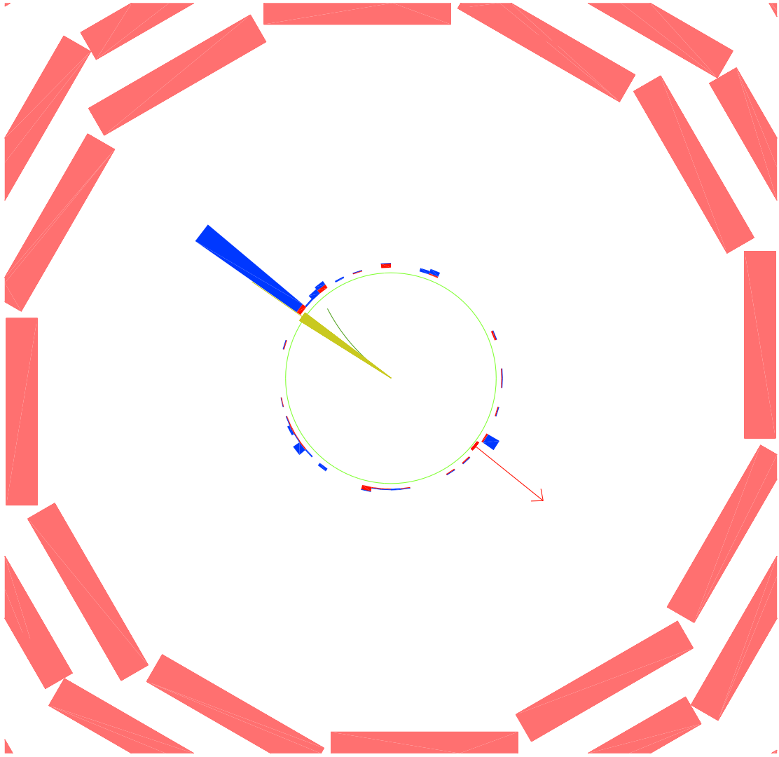
Figure 2.12: Visualization in the r - \phi plane of an event from 2009 data showing clear evidence of a high energy calorimeter deposit that is anti-aligned with the \vec{E}_T .
