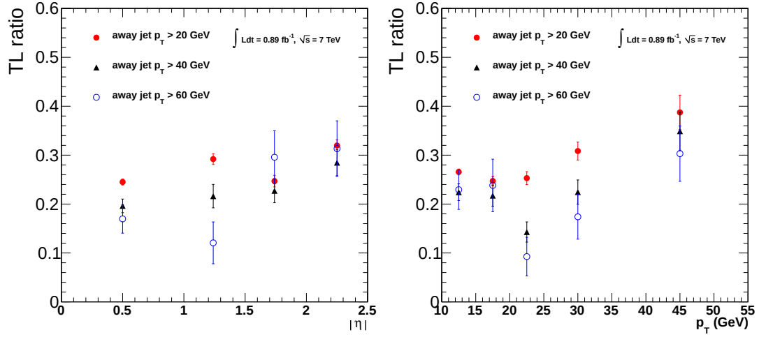
Figure 5.9: Projection in \eta and p_T of the electron fake rate measured in data for different away-jet p_T requirements. The away-jet is a corrected particle-flow jet and is required to be at least \Delta R > 1.0 away from the electron candidate. The electron fake rate is measured using triggers without an online isolation requirement.
