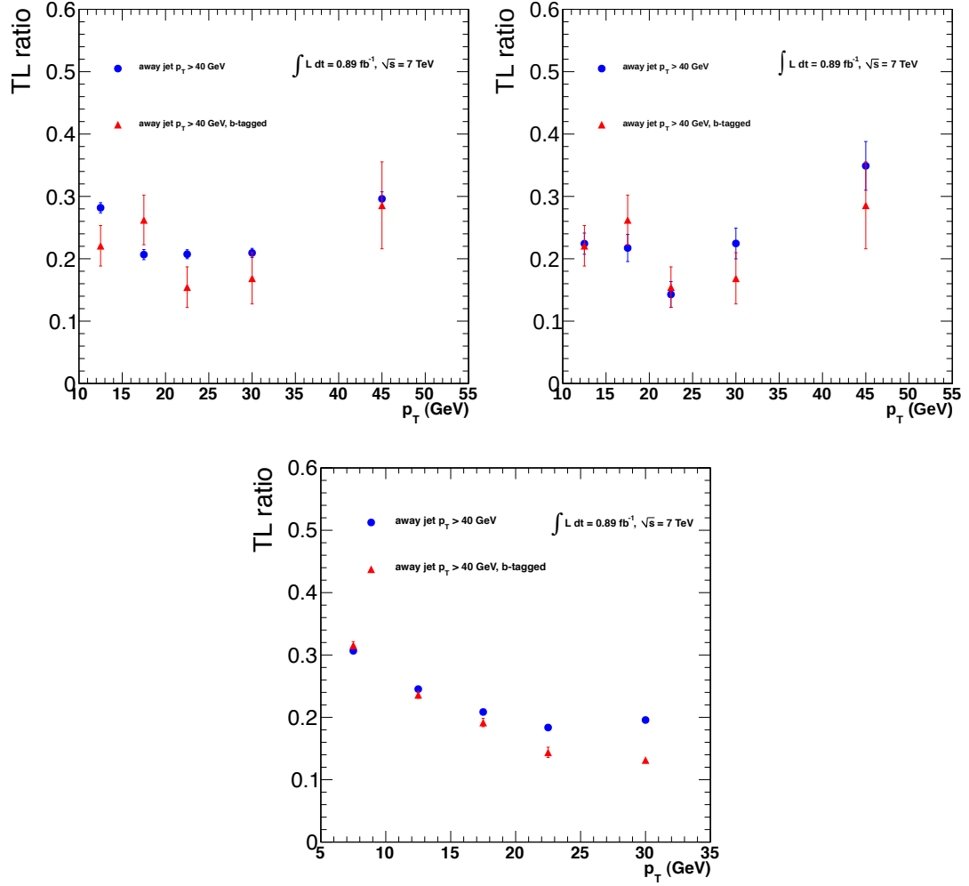
Figure 5.10: Projection in p_T of the lepton fake rates measured in data for different away-jet requirements. The away-jet is a corrected particle-flow jet with p_T > 40 GeV, is required to be at least \Delta R > 1.0 away from the lepton, with (filled triangle) and without (filled circle) a b -tagging requirement. We use the simple secondary vertex high efficiency (SSVHE) algorithm and require the discriminant have a value of at least 1.74. The top row shows the electron fake rate for triggers with (left) and without (right) an online isolation requirement. The bottom row shows the muon fake rate. Neither the fake rate for electrons nor muons shows a strong dependence on the heavy flavor content of the sample.
