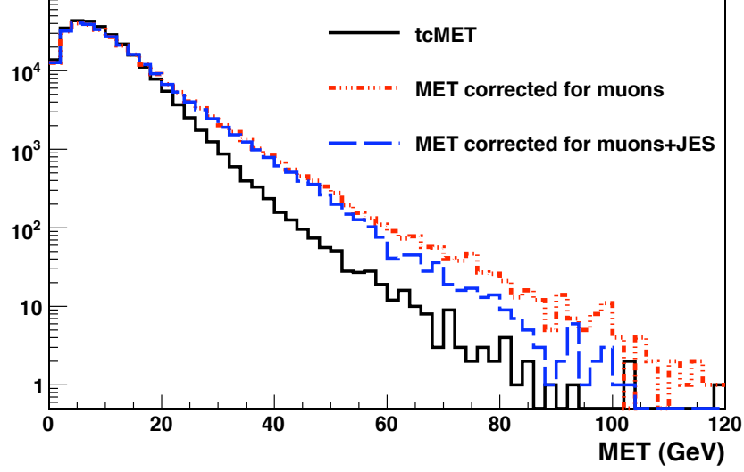
Figure 2.6: Distribution for tc\cancel{E}_T and corrected calo\cancel{E}_T objects in Z \rightarrow \ell^+\ell^- events, where the leptons are required to have p_T > 20 GeV. The tc\cancel{E}_T algorithm reduces the number of events with \cancel{E}_T > 30 (50) GeV by a factor of 3.4 (6.8) compared to caloMET corrected for muons only. The reduction is a factor of 3.0 (4.3) when compared to caloMET corrected for both muons and the JES.
