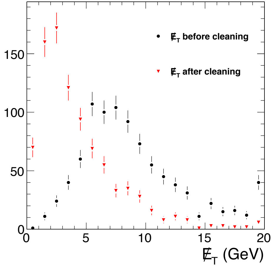
Figure 2.17: Distribution of E_T before and after cleaning HF spikes. Only the subset of events in data containing a HF tower identified as a spike is shown.
