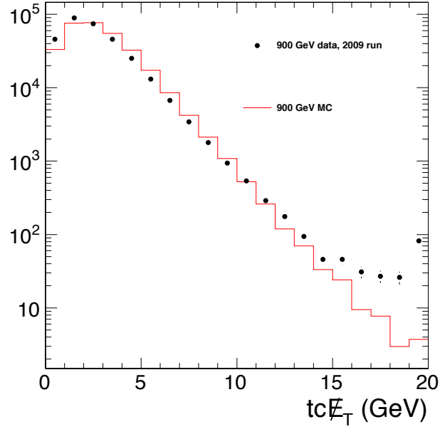
Figure 2.11: Distribution of tc\cancel{E}_T in data and MC at the start of the commissioning of 2009 data.
