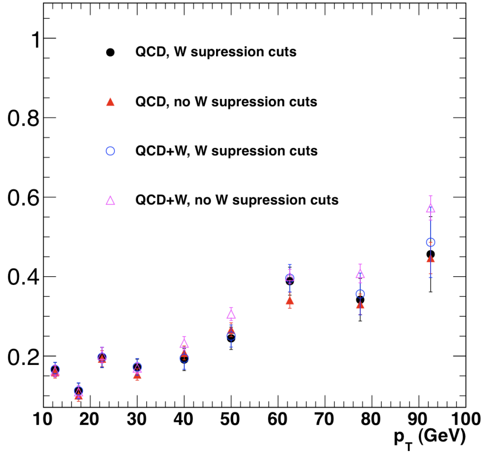
Figure 5.1: Electron fake rate as a function of the electron p_T measured over a range of selections enhancing the contribution from W/Z events. The fake rate measured in simulation is shown for the nominal measurement using only QCD samples (filled circles), and that with the W sample included (open circles), as well as for the selection without the W suppression measured in the QCD sample alone (filled triangles) and that with the W sample included (open triangles). Removing the W suppression cuts results in little increase in the value of the fake rate.
