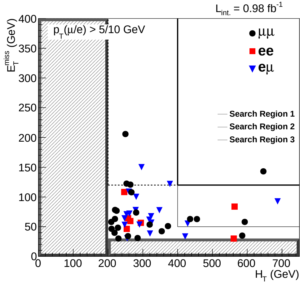
Figure 7.3: Distribution of events in the H_T - E_T^{\text{miss}} plane passing the analysis selections for the inclusive dilepton control region. From [45]
