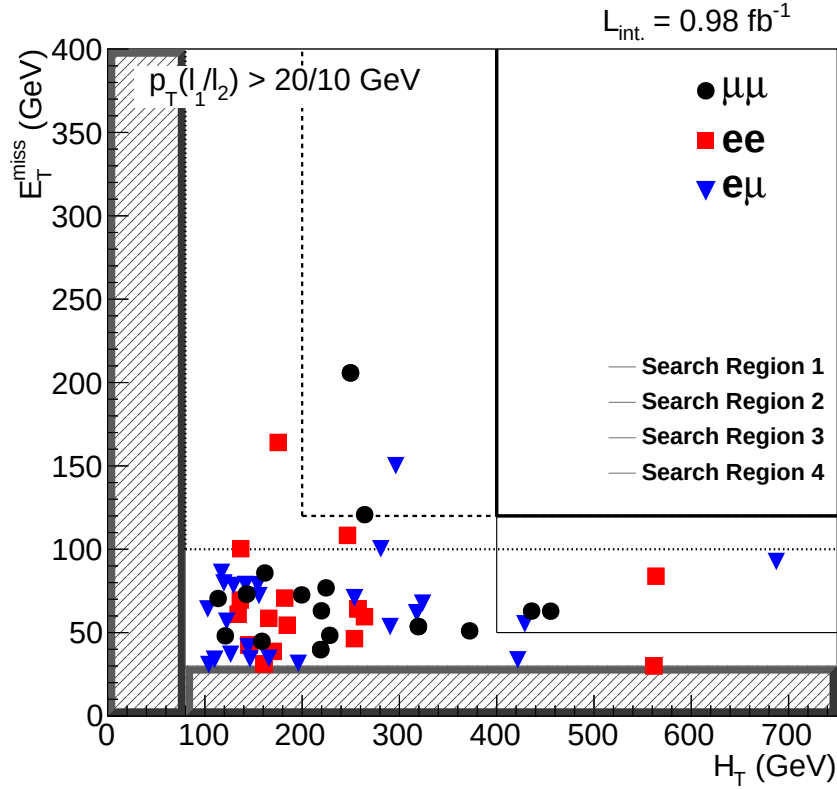
Figure 7.2: Distribution of events in the H_T - \cancel{E}_T plane passing the analysis selections for the high- p_T control region. From [45]
