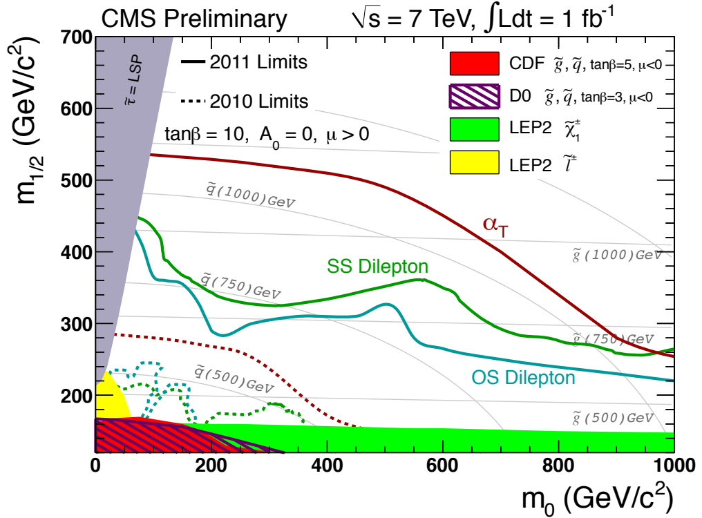
Figure 7.5: Observed limits for several 2011 CMS SUSY searches plotted in the CMSSM (m_0, m_{1/2}) plane. From [48].
