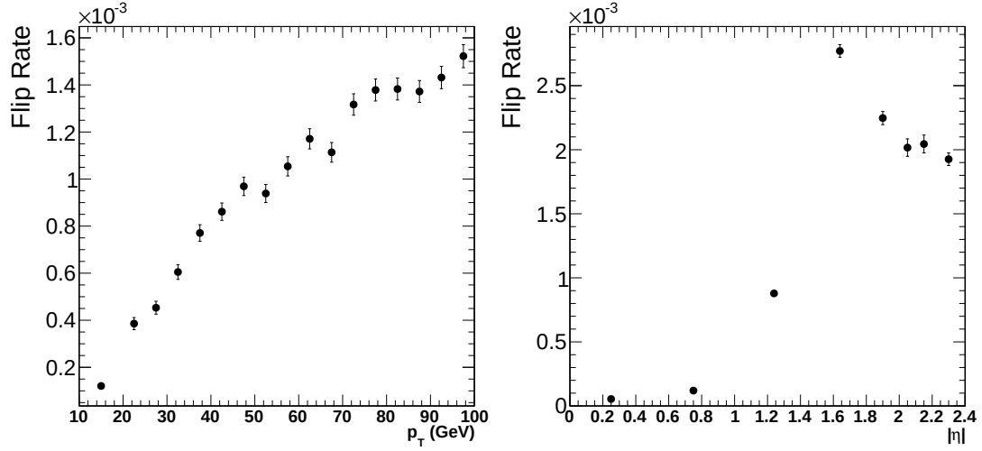
Figure 5.11: Charge mis-reconstruction rate projected in p_T (left) and \eta (right) measured using a single electron Monte Carlo sample. The rate is measured after requiring consistency amongst the three reconstructed electron charges.
