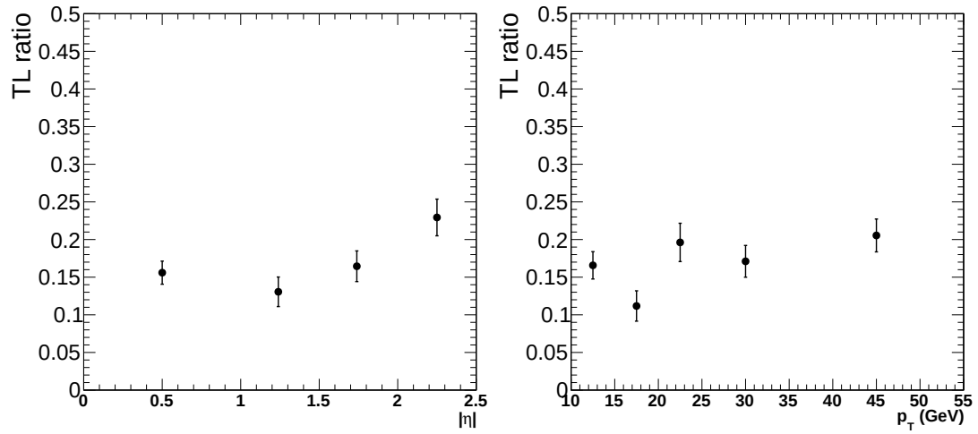
Figure 5.6: Projection in \eta and p_T of the electron fake rate measured in simulation.
