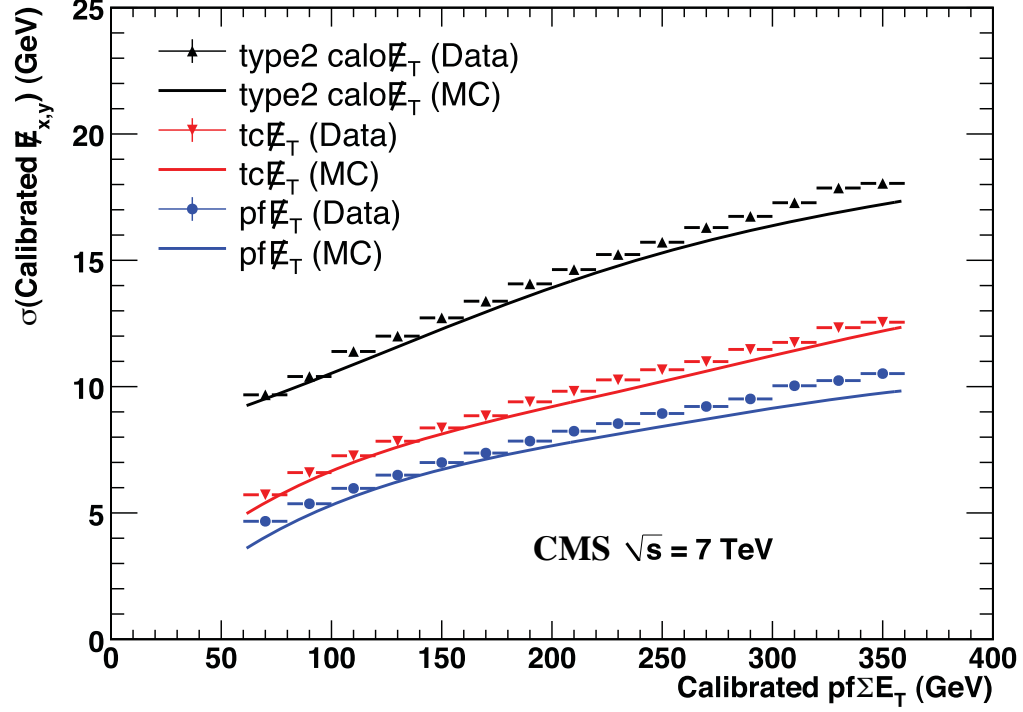
Figure 2.27: Resolution of the \cancel{E}_T components for \text{calo}\cancel{E}_T , \text{tc}\cancel{E}_T and \text{pf}\cancel{E}_T as a function of the calibrated sum E_T of particle-flow candidates [17].
