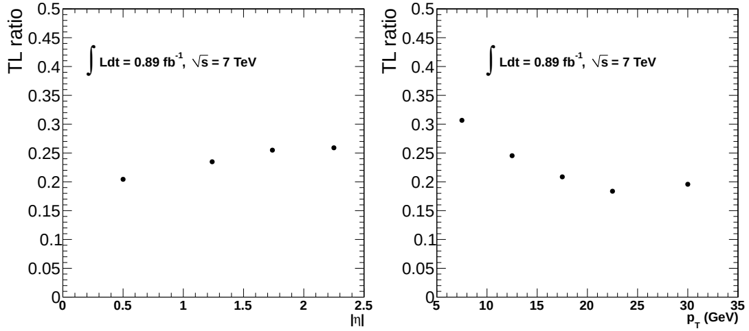
Figure 5.3: Projection in \eta and p_T of the muon fake rate measured in data. This fake rate is used for the high- p_T and inclusive dilepton analyses.
