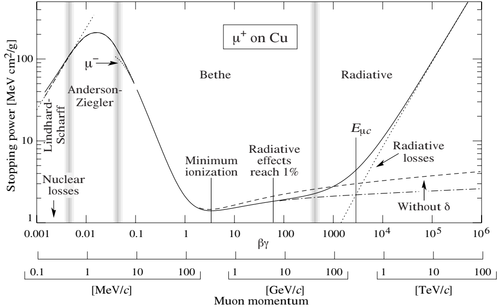
Figure 2.1: Stopping power of Cu for positively charged muons [3]. Muons from electroweak processes are typically produced with momenta of \mathcal{O}(100) GeV. This momentum scale is still in the region where muons are approximately minimum ionizing, before radiative effects become significant.
