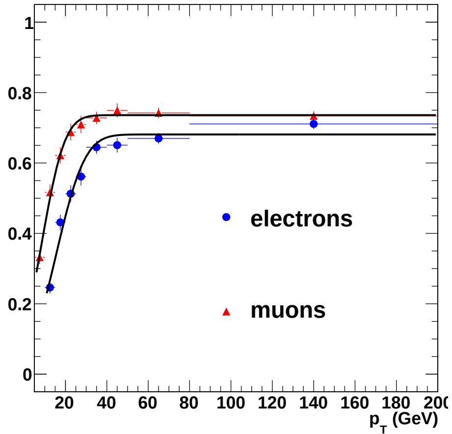
Figure 6.3: Lepton selection efficiency for electrons and muons as a function of p_T . The efficiencies were determined at the hard scatter level using simulated events for the mSUGRA point LM6. The displayed efficiencies include data-to-simulation scale factors for lepton identification and isolation determined using tag-and-probe in Z events as well as trigger efficiencies. The simulation has been re-weighted to reflect the pile-up distribution observed in the data.
