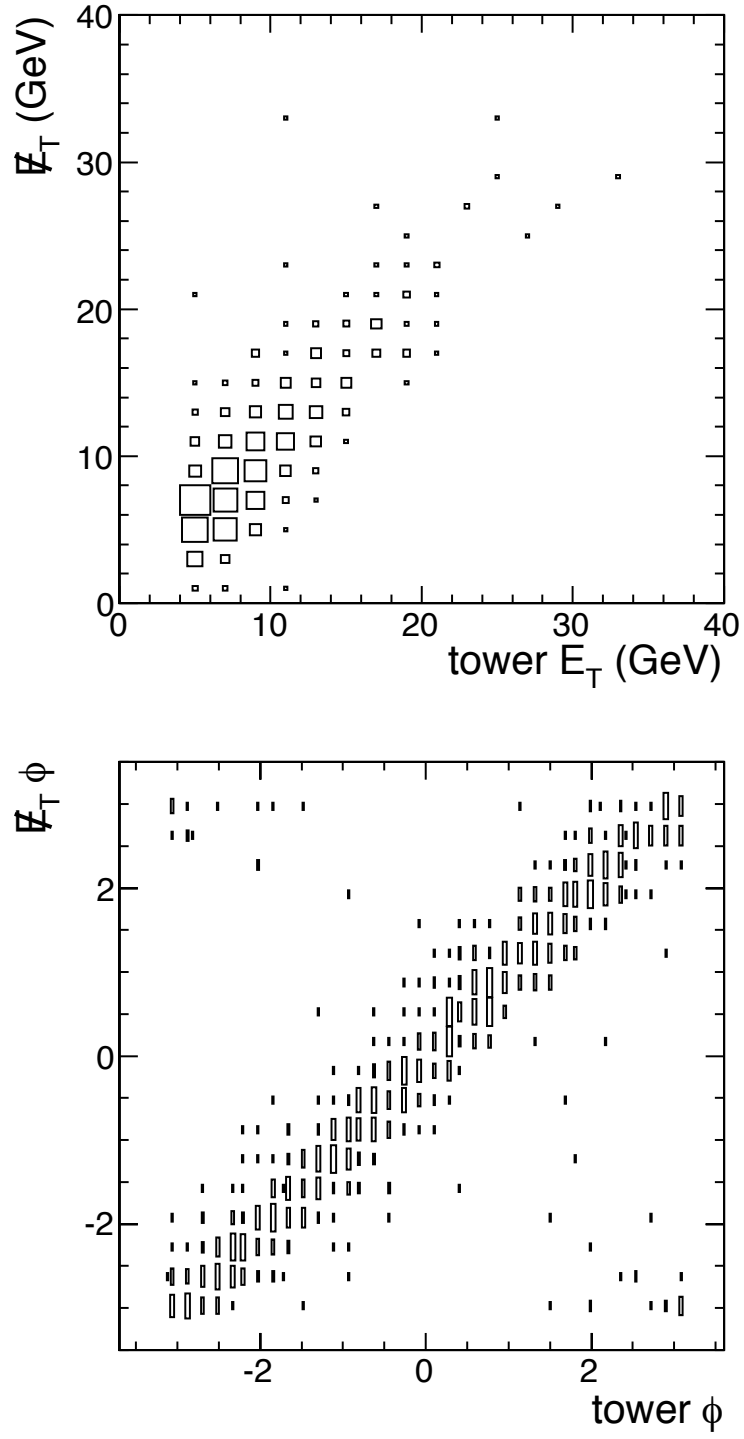
Figure 2.16: Correlation of the magnitude (top) and direction (bottom) between HF spikes and the \vec{E}_T .
