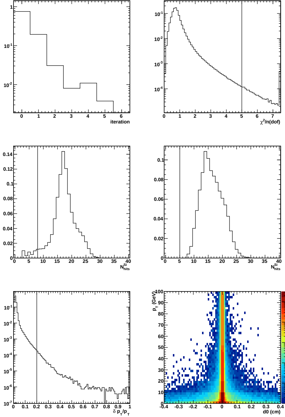
Figure 2.3: Tracking distributions made from a single pion Monte Carlo sample. Vertical lines indicate the selections used by the tc\cancel{E}_T algorithm. The distribution in each panel is made after applying all selections in Table 2.3 but omitting selection on the plotted quantity.
