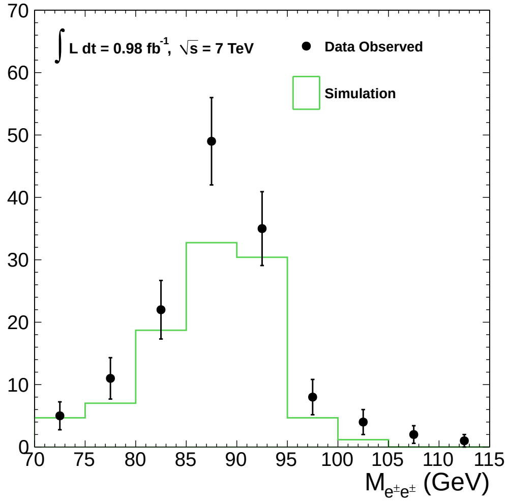
Figure 5.12: Invariant mass distribution of e^\pm e^\pm pairs in data compared with Z \rightarrow ee Monte Carlo expectations. To reduce backgrounds from W +jets, we require p_T^{\text{miss}} < 20 GeV and M_T < 25 GeV. The highest p_T electron is used in the calculation of the transverse mass.
