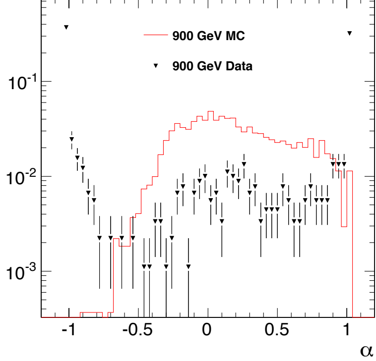
Figure 2.15: Distribution of \alpha = \frac{L-S}{L+S} used to characterize energy deposits in the forward hadron calorimeter. There is an excess of towers in data near \alpha = \pm 1 , which is indicative of anomalous signals in the HF. Only towers with E_T > 5 GeV are shown as towers with smaller E_T do not contribute significantly to the \cancel{E}_T tails.
