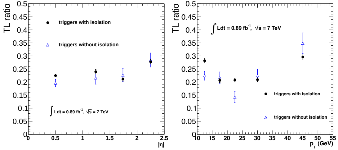
Figure 5.4: Projection in \eta and p_T of the electron fake rate measured in data using triggers with (filled circle) and without (open triangle) an online isolation requirement. The fake rate measured using triggers with an online isolation requirement is used for the high- p_T analysis in the dielectron final state. Triggers without an online isolation requirement are used to measure the fake rate for the inclusive dilepton analysis, as well as the e\mu final state of the high- p_T analysis.
