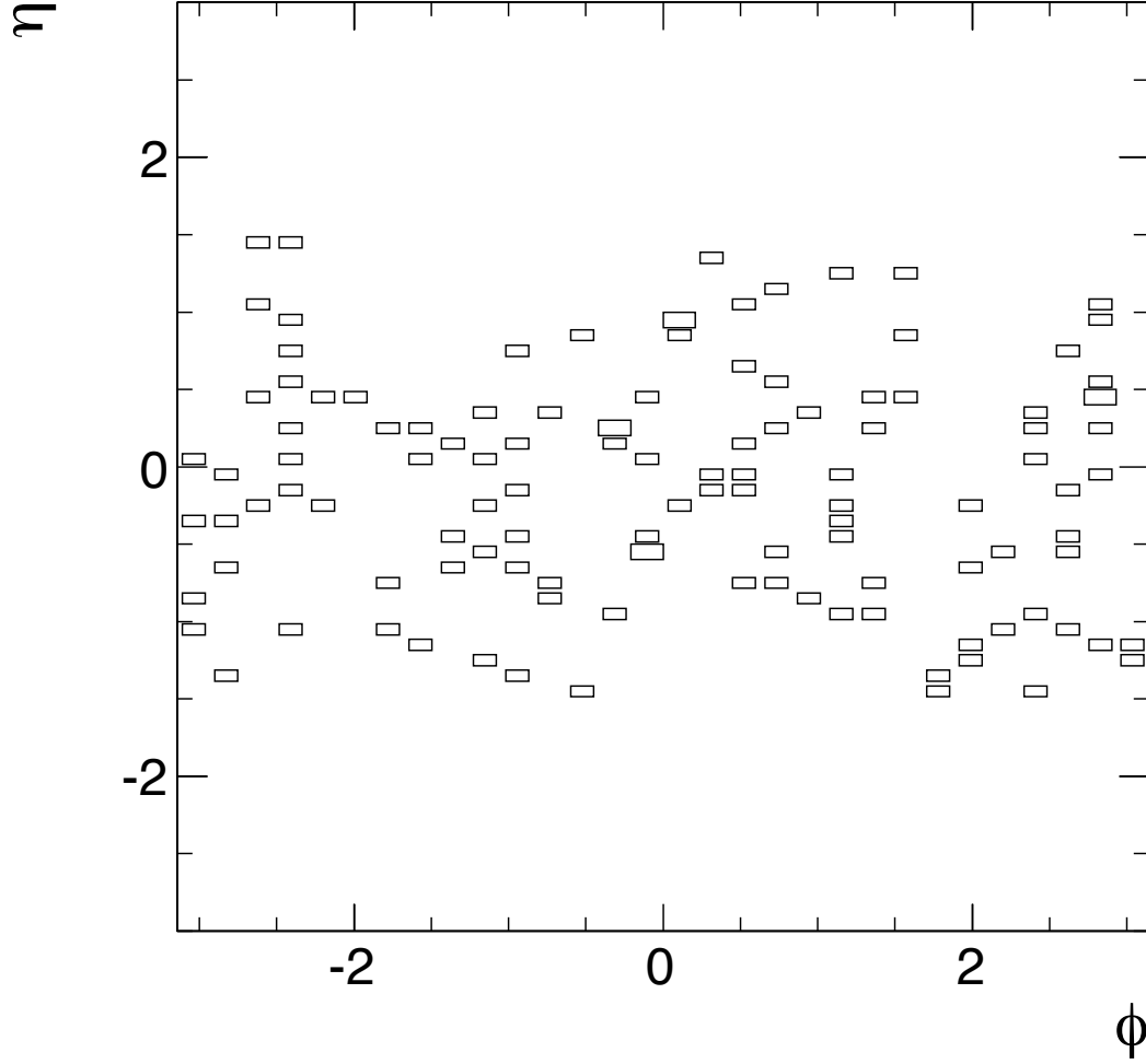
Figure 2.22: ECAL spikes are uniformly distributed throughout the barrel.
