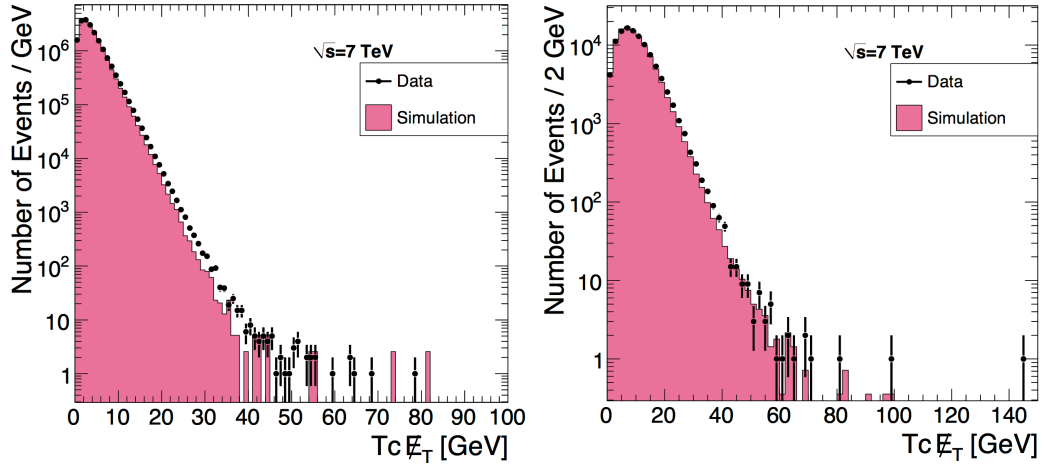
Figure 2.25: Comparison of tc\cancel{E}_T distributions in data and simulation for minimum bias events (left) and di-jet events (right). Distributions were made using approximately 11.7 \text{ nb}^{-1} of \sqrt{s} = 7 TeV data [17].
