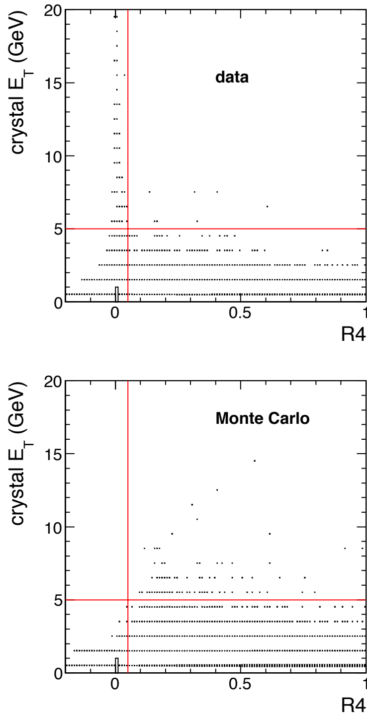
Figure 2.21: Distribution of R4 used to characterize energy deposits in the ECAL barrel. There is an excess of towers in data with E_T > 5 GeV and R4 < 0.05 which is indicative of anomalous signals in the ECAL.
