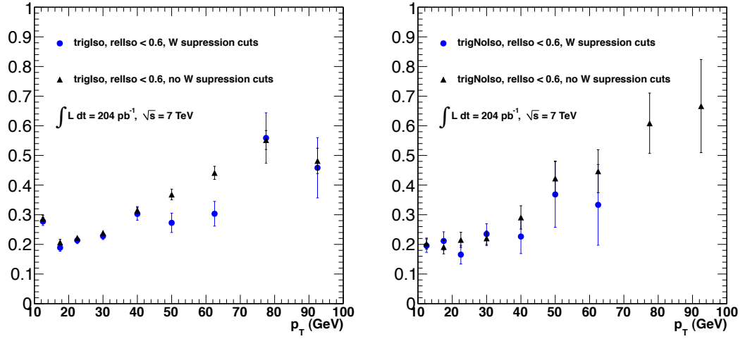
Figure 5.2: Electron fake rate as a function of the electron p_T measured with (filled circles) and without (filled triangles) W suppression cuts in data. Removing the W suppression cuts results in a small change in the fake rate for triggers with an online isolation cut. The fake rate measured in events selected using triggers with an online isolation cut shows more sensitivity to W contamination, as expected, although the value of the fake rate remains stable with p_T after applying rejection cuts. Based on these observations and those from simulation, the electron fake rate is measured out to a p_T of 55 GeV, and take to be a constant value at higher p_T .
