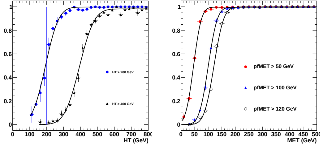
Figure 6.4: Efficiency for an event to pass a given reconstructed \cancel{E}_T ( H_T ) threshold as a function of the \cancel{E}_T^{\text{gen}} ( H_T^{\text{gen}} ). The curves are shown for \cancel{E}_T thresholds of 50, 100 and 120 GeV. The thresholds for H_T are 200 and 400 GeV.
