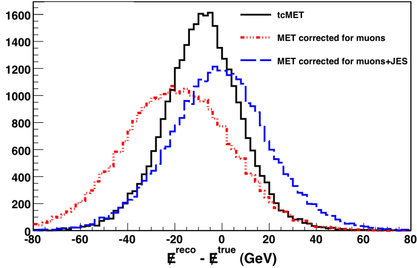
Figure 2.7: Distribution of \Delta\cancel{E}_T = \cancel{E}_T^{\text{reco}} - \cancel{E}_T^{\text{true}} for t\bar{t} \rightarrow \ell^+\ell^- + X events with \cancel{E}_T^{\text{true}} > 50 GeV. The \cancel{E}_T resolution is improved nearly 25% (20%) for \text{tc}\cancel{E}_T compared to \text{calo}\cancel{E}_T corrected for muons ( \text{calo}\cancel{E}_T corrected for muons + JES).
