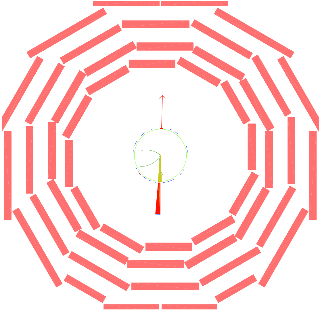
Figure 2.18: Visualization in the r - \phi plane of an event from 2009 data showing clear evidence of a high energy calorimeter deposit that is anti-aligned with the -\vec{E}_T .
