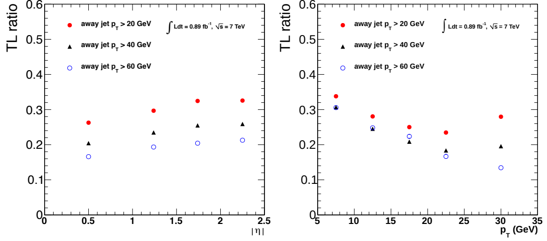
Figure 5.7: Projection in \eta and p_T of the muon fake rate measured in data for different away-jet p_T requirements. The away-jet is a corrected particle-flow jet and is required to be at least \Delta R > 1.0 away from the muon candidate.
