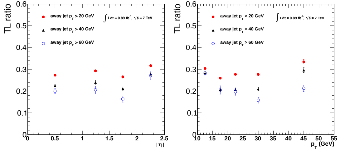
Figure 5.8: Projection in \eta and p_T of the electron fake rate measured in data for different away-jet p_T requirements. The away-jet is a corrected particle-flow jet and is required to be at least \Delta R > 1.0 away from the electron candidate. The electron fake rate is measured using triggers with an online isolation requirement.
