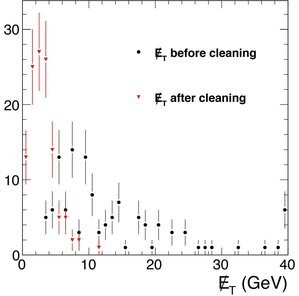
Figure 2.24: Distribution of \cancel{E}_T before and after cleaning ECAL spikes. Only the subset of events in data containing an ECAL crystal identified as a spike is shown.
