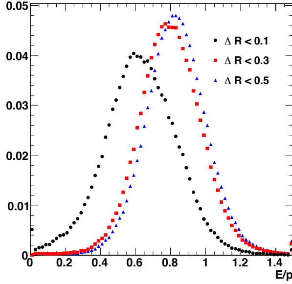
Figure 2.4: Response of simulated charged pions with |\eta| < 1 and p_T between 20 and 30 GeV using cones of size \Delta R = 0.1, 0.3 and 0.5 .
