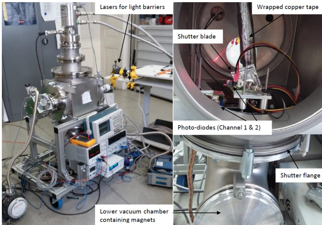
Figure 4.5.: Left: The complete setup. On the white table two yellow bench vices hold the lasers for the light barriers. Right: The shutter installed in the vacuum chamber. In the fore ground one of the photo diodes is visible on an amplifier board. The cabling of the amplifiers includes the power supply in black and red and ground in yellow. The amplifier signal is transmitted with a BNC cable whose feed-through is visible left above the window. The second amplifier board is half visible on the left hand side of the other one. Due to the very limited space in the chamber it had to be mounted upside down. Through the window a laser diode is visible that shines red light on one of the photo-diodes. Wrapped in super insulation foil the cooper tape connects the shutter with the cold finger on top. Shutter flange.
