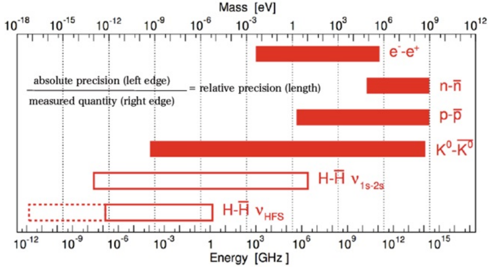
Figure 1.1.: Precision of some CPT tests compared with envisaged precision of \bar{\text{H}} experiments. The right edge of the red bars indicates the measured quantity and the left edge the absolute precision of this measurement. The dashed line for \text{H}-\bar{\text{H}} \nu_{\text{HFS}} shows the theoretical potential of ground state hyperfine spectroscopy experiments. First generation experiments of this kind aim at the left edge of the solid bar which is slightly above 10^{-7} GHz. Taken from [29]
