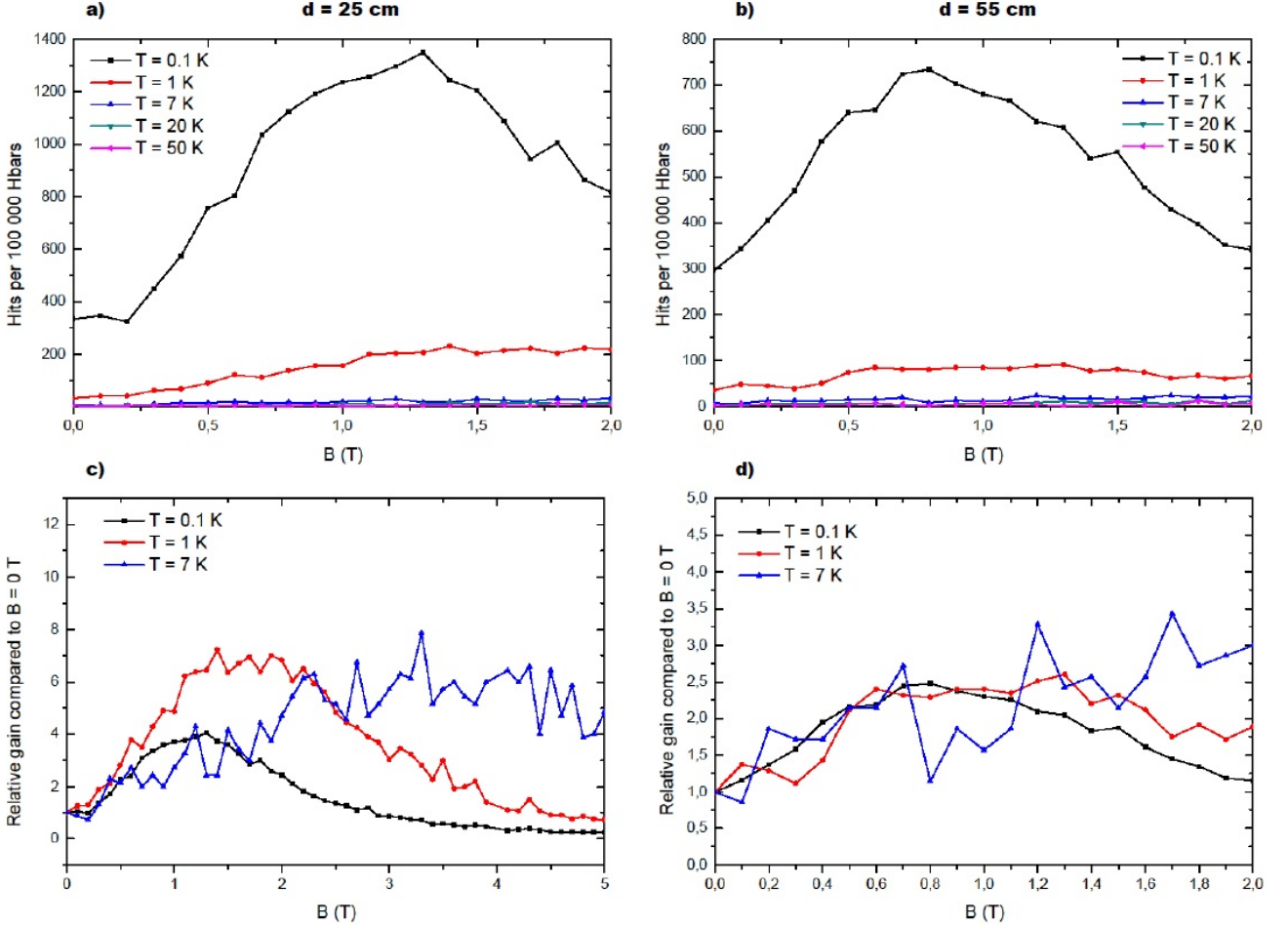
Figure 3.7.: The number of counts per 100 000 \bar{\text{H}} 's in the gravity experiment is shown in a) with the sextupole at d = 25 cm and in b) with d = 55 . c) ( d = 25 ) and d) ( d = 55 ) show the relative gain in counts \frac{n(B)}{n(B)|_{B=0\text{T}}} , that is attainable by the implementation of a sextupole magnet.
