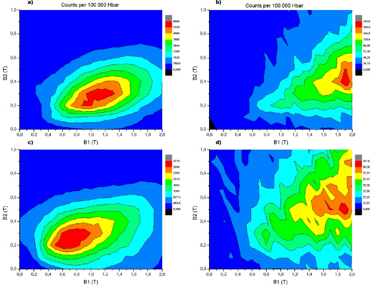
Figure 3.5.: Number of counts per 100 000 \bar{H} 's in dependence of the field strengths of the sextupole magnets. The four plots belong to simulations with differing values for \bar{H} temperature and distance of the first sextupole from the source: a) 0.1 K, 25 cm b) 7 K, 25 cm c) 0.1 K, 55 cm d) 7 K, 55 cm.
